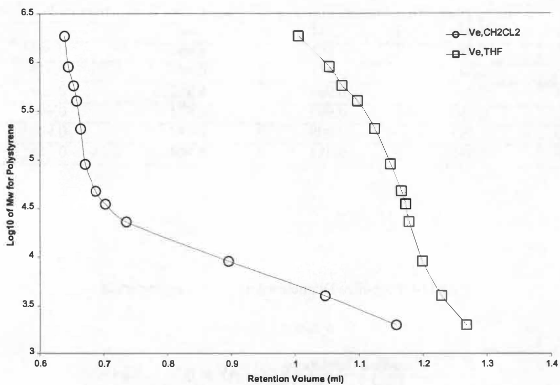
Figure 11. ISEC Calibration Curve for the standard packing material for column (1).
