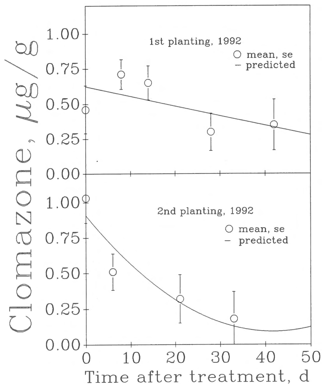
Figure 2. Field dissipation of clomazone with time after treatment in Sequatchie soil in two plantings at Knoxville in 1992. Regression equations: first planting: \hat{Y} = -0.007(\text{days}) + 0.62 , r^2 = 0.86 ; second planting: \hat{Y} = 0.95 - 0.05(\text{days}) + 0.001(\text{days})^2 , r^2 = 0.92 .
