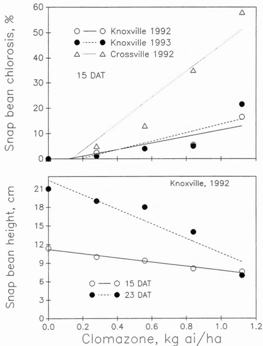
Figure 2. Effect of clomazone rate on snap bean injury and height. Injury data are pooled over plantings and height data for Knoxville are pooled over plantings. Regression equations for snap bean injury: Knoxville 1992, \hat{Y} = 12.9(\text{rate}) - 1.5 , r^2 = 0.80 ; Knoxville 1993, \hat{Y} = 16.8(\text{rate}) - 3.1 , r^2 = 0.72 ; Crossville 1992, \hat{Y} = 52.1(\text{rate}) - 7.0 , r^2 = 0.92 . Regression equations for snap bean height: 15 DAT, \hat{Y} = -3.4(\text{rate}) + 11.2 , r^2 = 0.98 ; 23 DAT, \hat{Y} = -11.8(\text{rate}) + 22.4 , r^2 = 0.89 .
