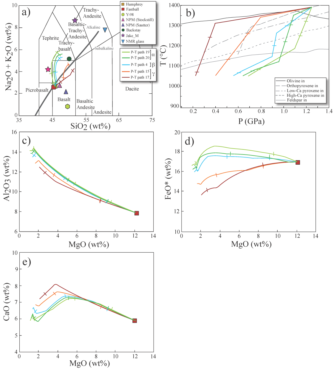
Figure A8. a) Total alkali-silica diagram showing liquid lines of descent calculated with pMELTS for the fractional crystallization of the Fastball composition with 0.5 wt% \text{H}_2\text{O} at FMQ-1 and P-T paths displayed in b). b) P-T paths used to calculate liquid lines of descent in 8a and c-e). Olivine, orthopyroxene, low-Ca pyroxene, high-Ca pyroxene, and feldspar liquidus are shown as black and gray solid and dashed lines, respectively. Plots of c) \text{Al}_2\text{O}_3 , d) \text{FeO}^* , and e) \text{CaO} versus \text{MgO} for liquid lines of descent. Tick marks delineate 20% fractionation increments.
