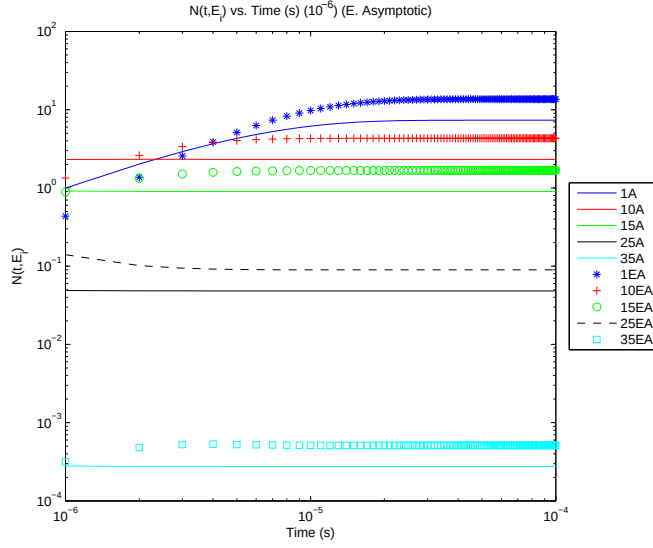
Figure 23: Explicit Asymptotic approximation (EA): Numerical/Analytic solution showing Neutrino density vs. Time at time step of 10^{-6} .
