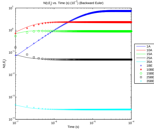
Figure 11: Backward-Euler method: Analytic vs. Numerical solution showing Neutrino density vs. Time at time step of 10^{-7} . As the time step ( dt ) increases, the amount of results decreases.
