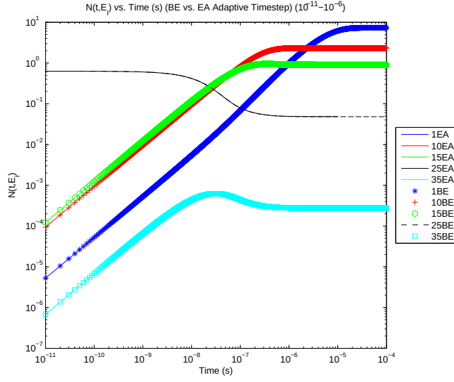
Figure 30: Explicit Asymptotic approximation (EA) vs. Backward Euler method (BE): Numerical solutions of both methods showing Neutrino density vs. Time at a varying time step of 10^{-11} to 10^{-6} seconds.
