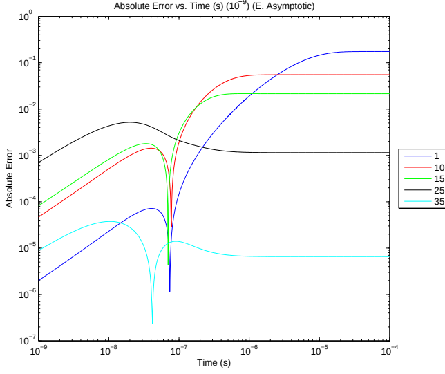
Figure 25: Explicit Asymptotic approximation (EA): Absolute error vs. Time at time step of 10^{-9} . Prior to reaching equilibrium, the absolute error increases before leveling for every energy bin group.
