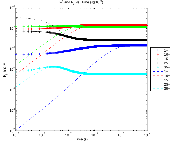
Figure 14: F_i^+ = F_i^- [Backward-Euler method]: Numerical solution showing Neutrino density vs. Time at time step of 10^{-9} . At the lowest time step, the earliest equilibrium time is reached by the (35) energy bin group while the latest time is reached by the (1) energy bin group.
