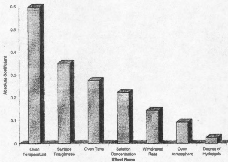
Figure 4.6 Pareto Charts for Epitaxial #
