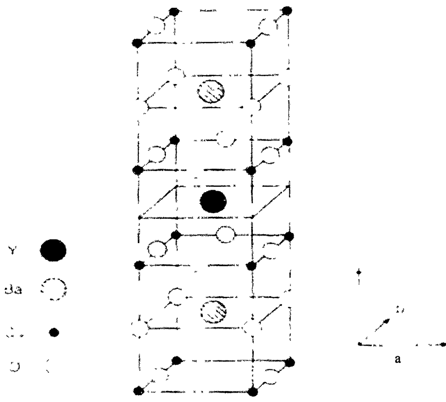
Figure 2.5 YBCO ( \text{YBa}_2\text{Cu}_3\text{O}_7 )
