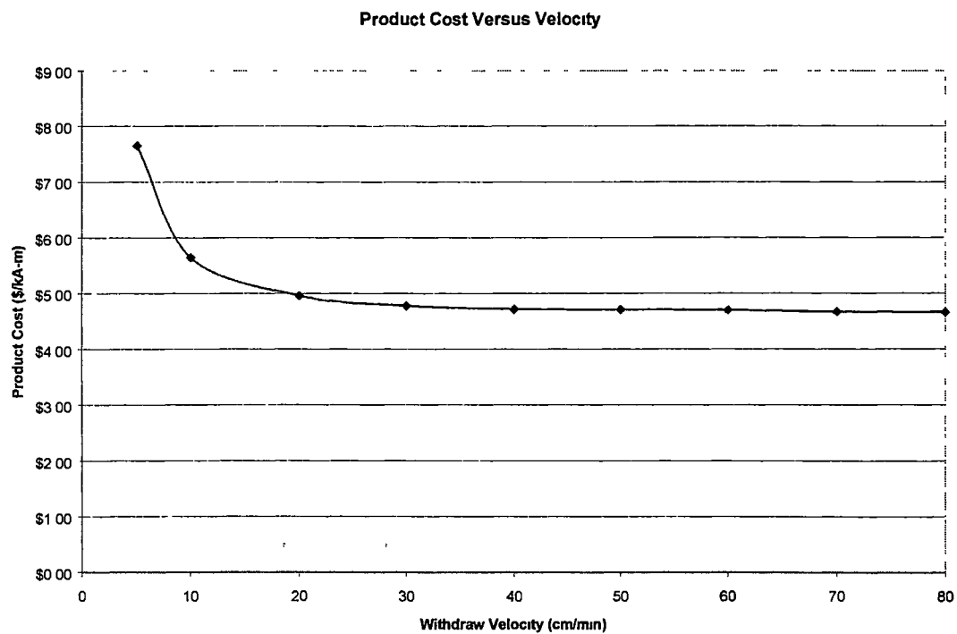
Figure 5.7 Product Cost Versus Withdrawal Velocity
