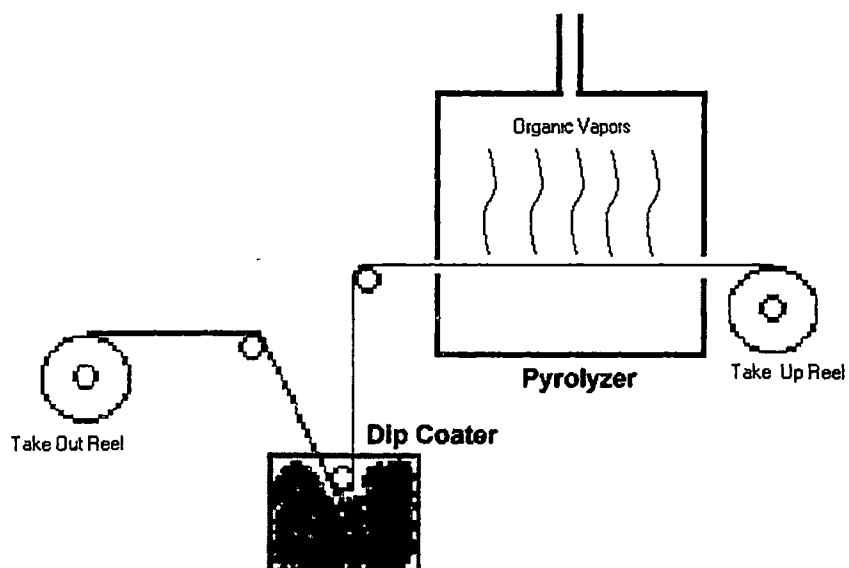
Figure 5.1 Continuous Dip-Coater
