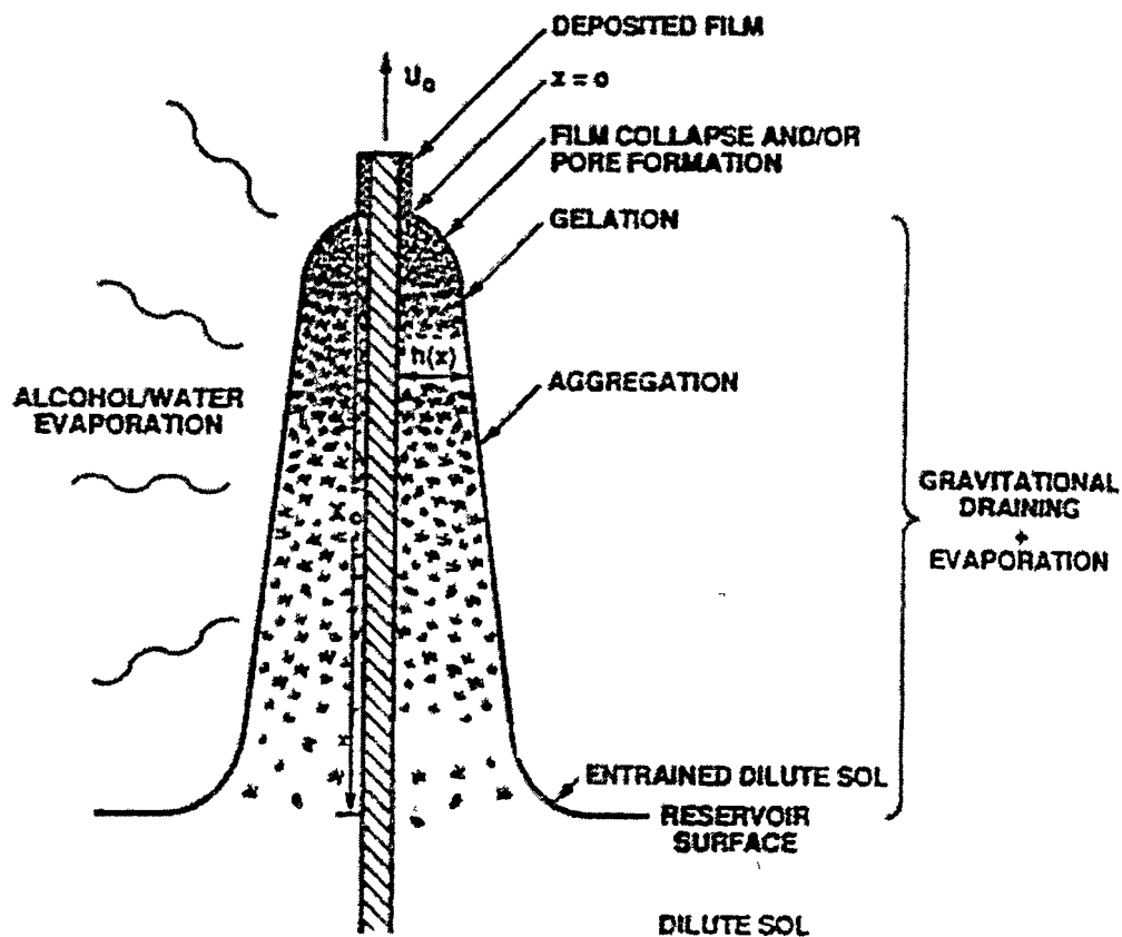
Figure 2.13 Gel Formation in Dip Coating
