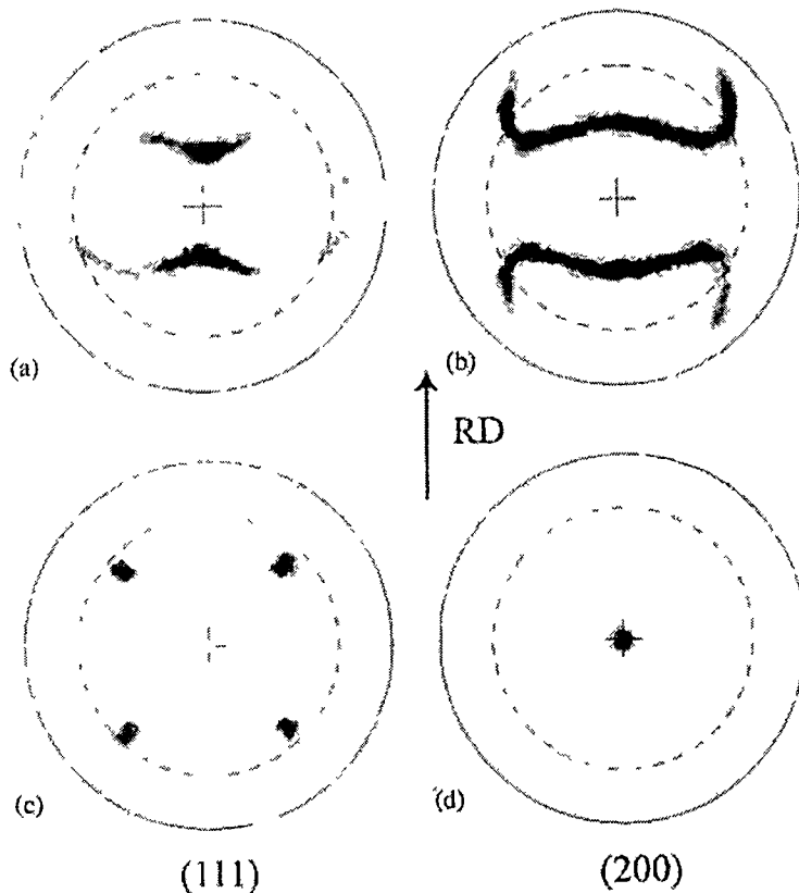
Figure 2.7 Improvement in Texture with Recrystallization
