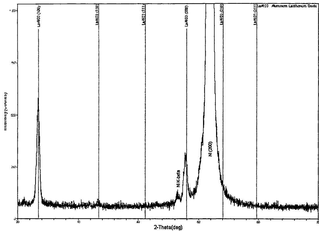
Figure 3.4 Typical Phase Scan of \text{LaAlO}_3 on Nickel Substrate
