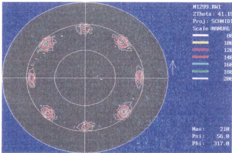
Figure 4.7 (111) Pole Figure of \text{LaAlO}_3 on Ni
