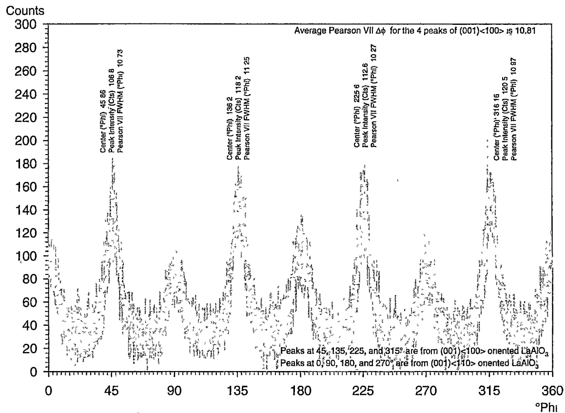
Figure 3 6 Typical (111) \text{LaAlO}_3 Phi Scan
