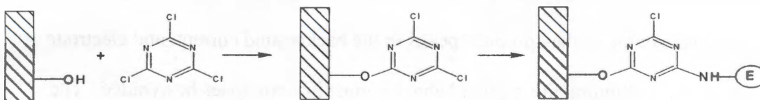
Figure 2.5: Common covalent immobilization techniques for enzymes.
