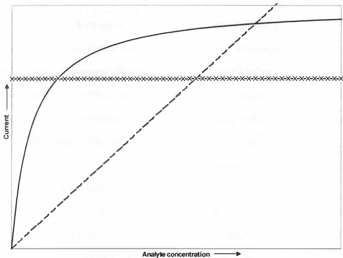
Figure 2.7: Apparent enzyme kinetics of a biosensor for different rate-determining steps.
