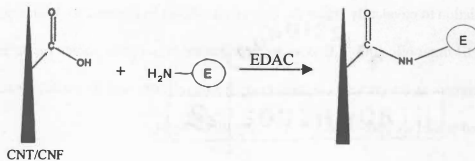
Figure 2.9: Covalent attachment of an enzyme to CNTs/CNFs via EDAC-activated amidation.
