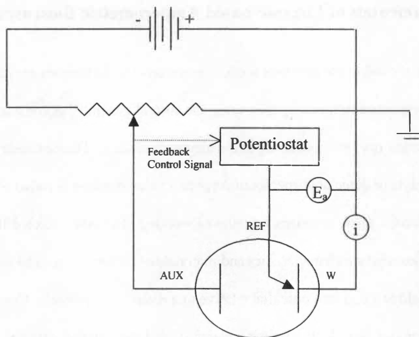
Figure 2.2: Schematic representation of a potentiostat and three-electrode cell.
