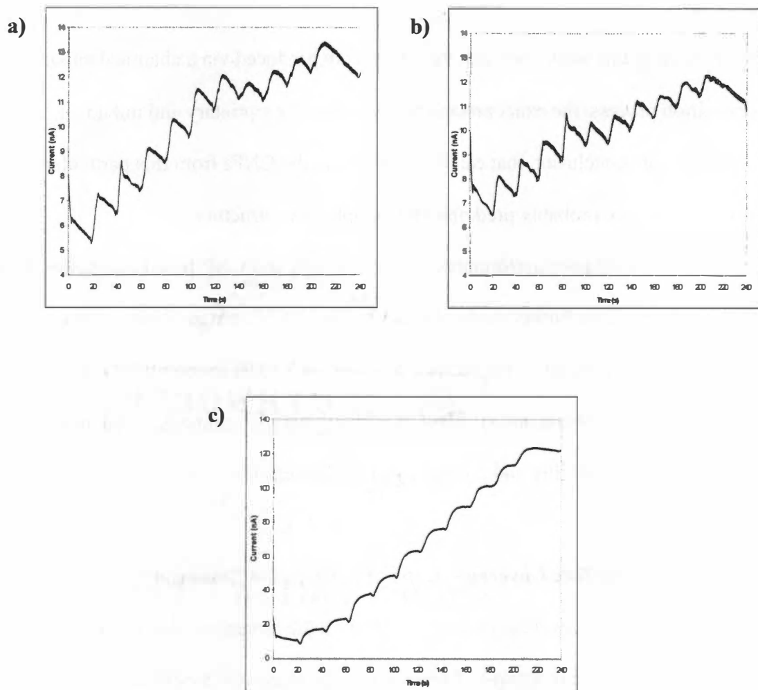
Figure 4.8: Individual responses of different biosensors to ethanol additions.
