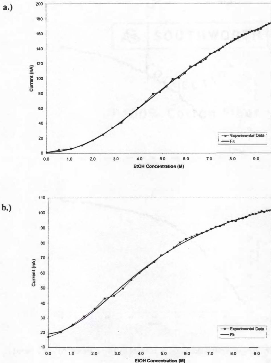
Figure 4.10: Current as a function of ethanol concentration for two different MWNT-based biosensors.
