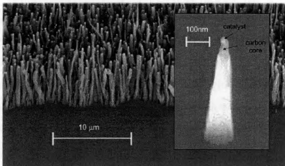
Figure 2.8: Scanning electron micrograph of CNFs grown on a silicon support.
