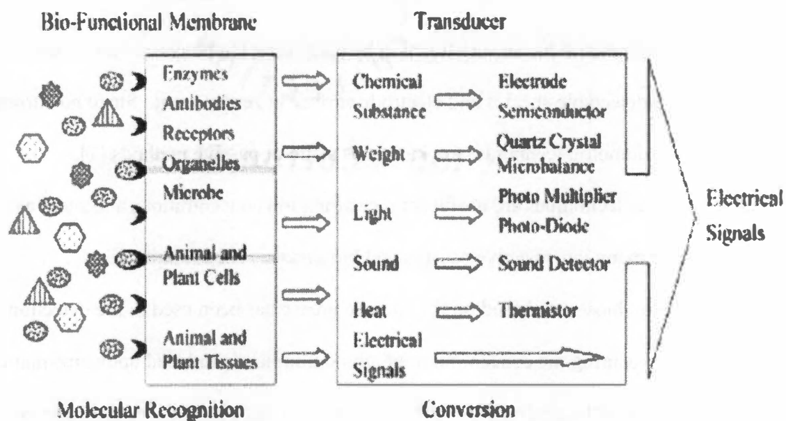
Figure 2.1: The different kinds of biological elements and transducers used in biosensors and the general principles of how they function.
