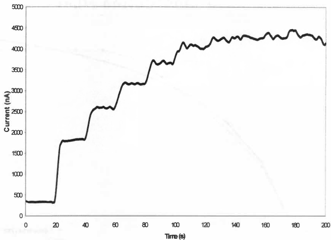
Figure 4.11: Amperometric detection of ethanol by the MWNT-modified electrode with YADH and \text{NAD}^+ in free solution.
