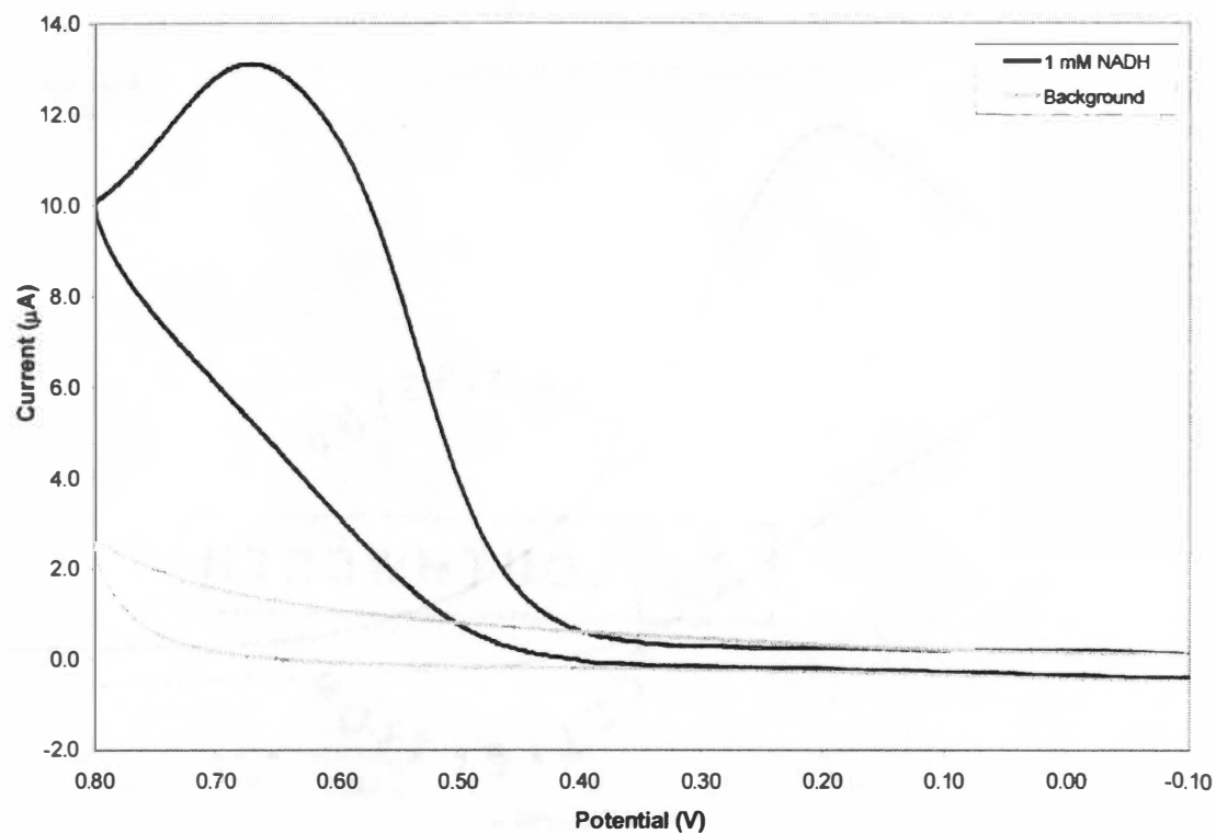
Figure 4.1: Cyclic voltammogram for an unmodified GC electrode in 1 mM NADH.
