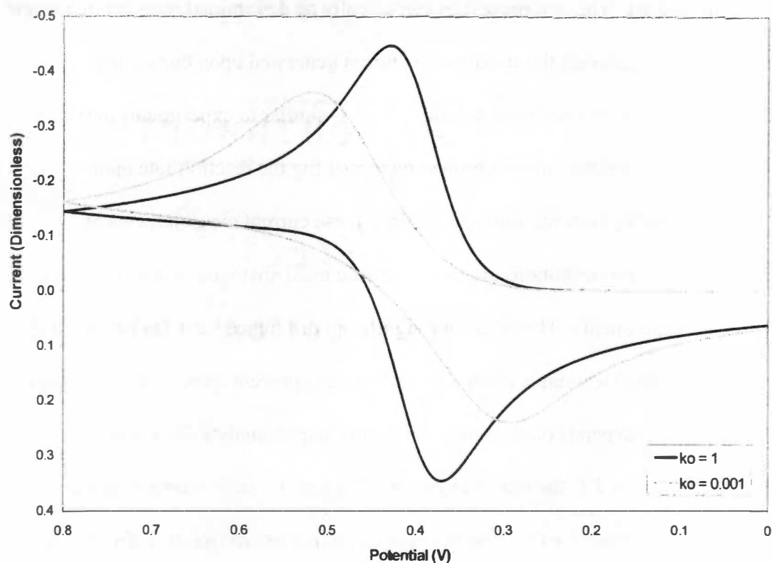
Figure 2.6: Hypothetical cyclic voltammograms for two materials.
