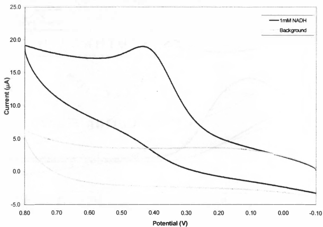
Figure 4.4: Cyclic voltammogram for a MWNT-modified GC electrode in 1 mM NADH.
