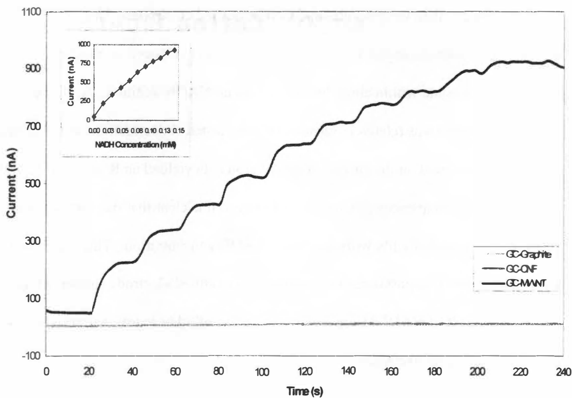
Figure 4.6: Amperometric detection of NADH at graphite-, CNF- and MWNT-modified GC electrodes.
