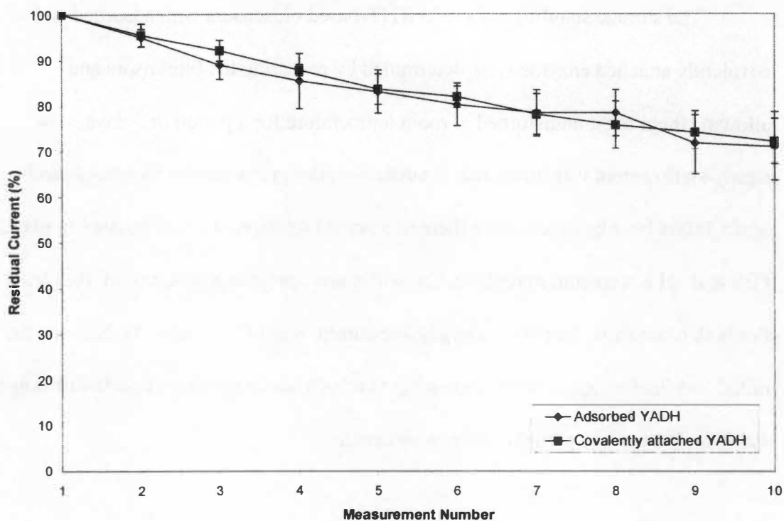
Figure 4.13: Reusability of two different MWNT-based biosensors.
