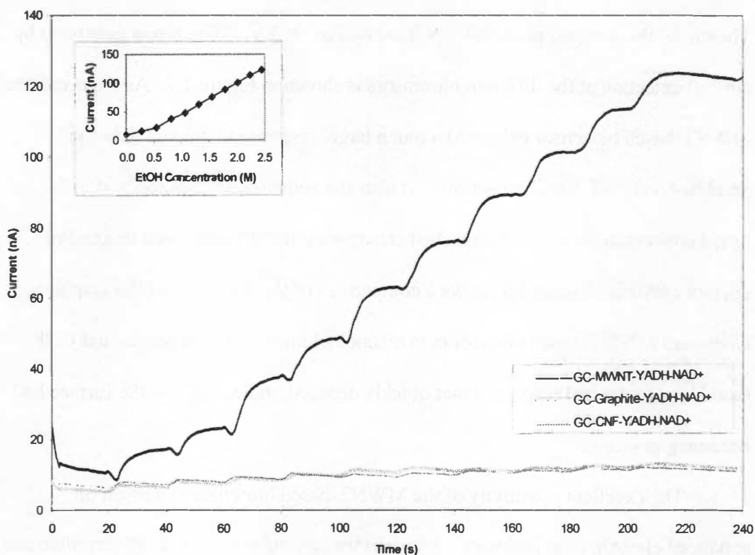
Figure 4.7: Amperometric detection of ethanol by graphite-, CNF- and MWNT-based biosensors.
