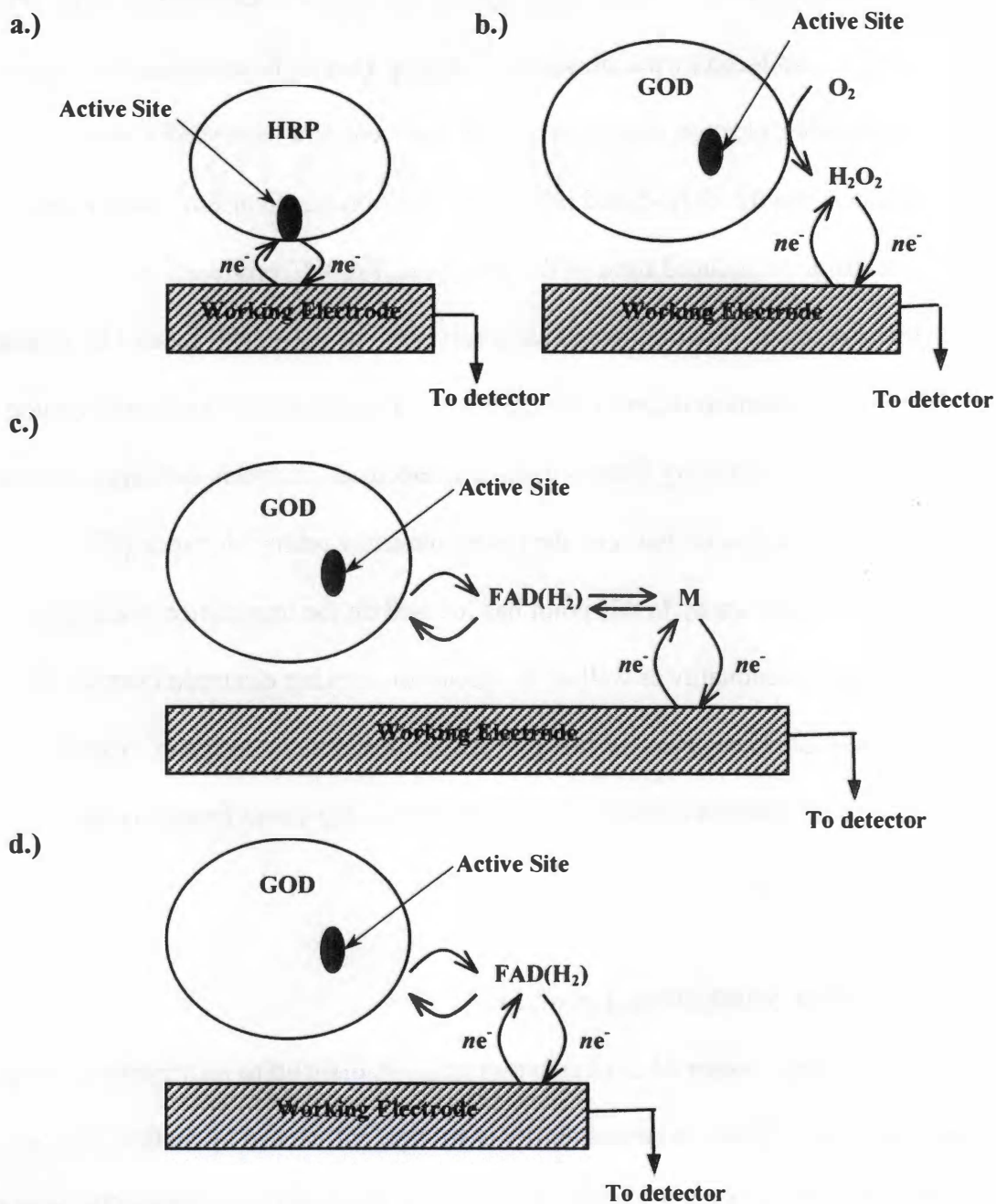
Figure 2.4: Examples of indirect analyte detection techniques.
