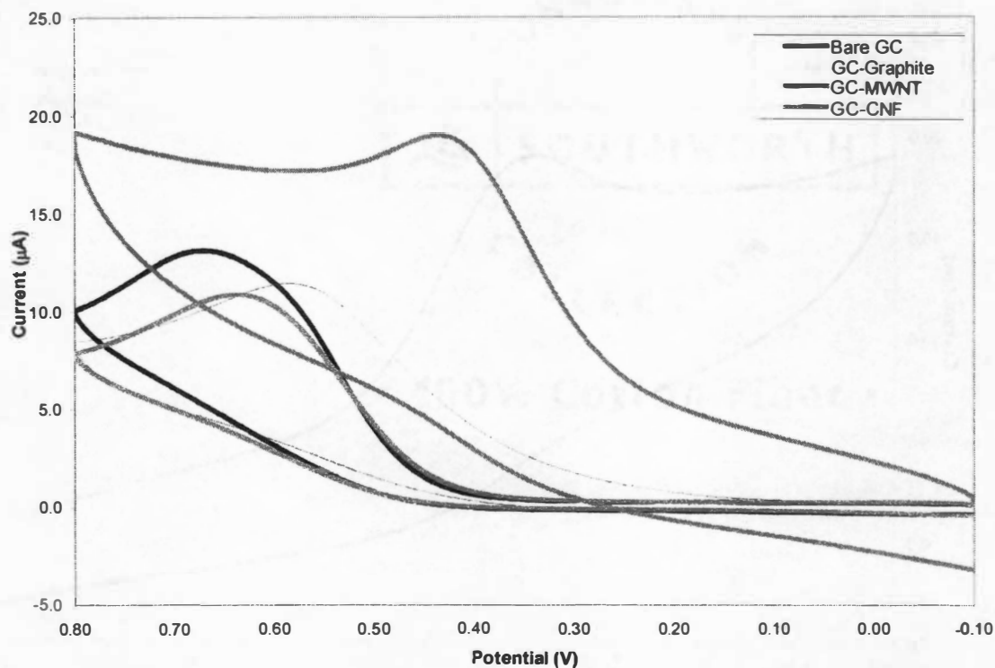
Figure 4.5: Cyclic voltammograms for unmodified, graphite-, CNF- and MWNT-modified GC electrodes in 1 mM NADH.
