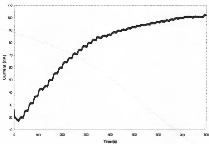
Figure 4.9: Amperometric detection of ethanol by two different MWNT-based biosensors.
