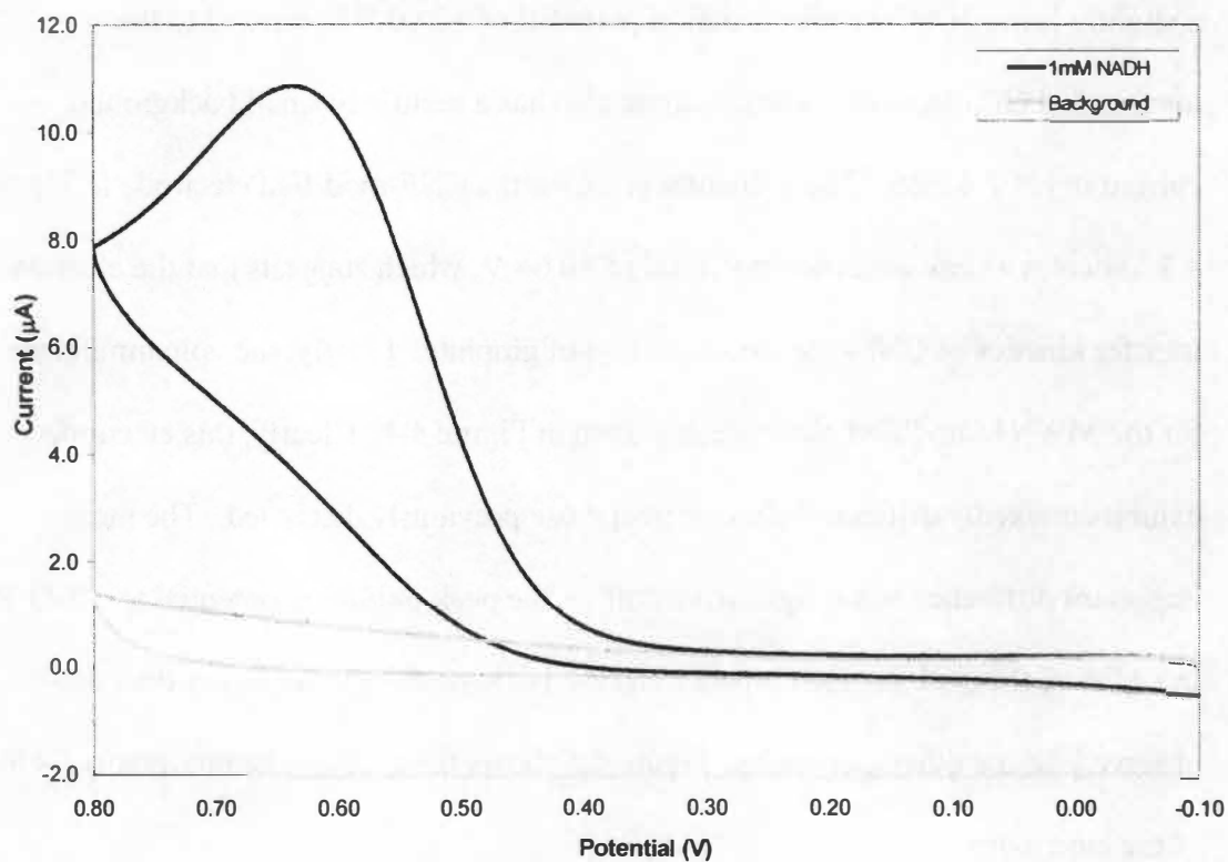
Figure 4.3: Cyclic voltammogram for a CNF-modified GC electrode in 1 mM NADH.
