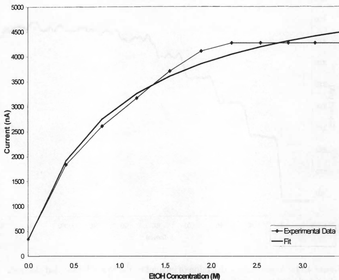
Figure 4.12: Current as a function of ethanol concentration for the MWNT-modified electrode with YADH and \text{NAD}^+ in free solution
