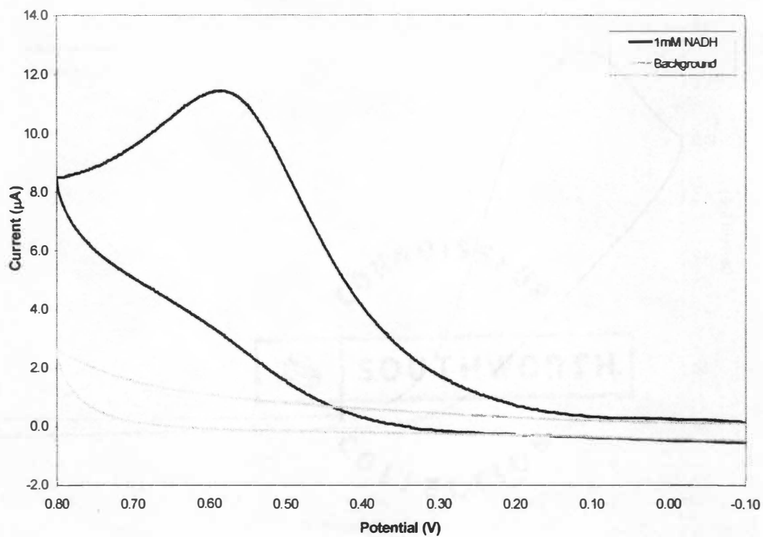
Figure 4.2: Cyclic voltammogram for a graphite-modified GC electrode in 1 mM NADH.
