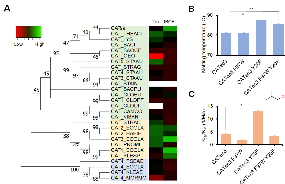
Figure 2-9: Bioprospecting and protein engineering of CATs. (A) A phylogenetic tree of 28 CATs and heat map of their melting temperatures ( T_m ) and activities towards isobutanol (IBOH). The numbers in the phylogenetic tree represent bootstrapping values (%) from 1000 bootstrap replicates. (B) Melting temperatures of CAT3_ECOLX (CATec3) variants. Student's t-test: *p-value = 4.34E-08 (df = 13), **p-value = 3.43E-06 (df = 13). Each value represents mean \pm 1 stdev from at least three biological replicates. (C) Catalytic efficiencies of CATec3 and its variants towards isobutanol. Student's t-test: *p-value = 4.46E-05 (df = 6). Each value represents mean \pm 1 stdev from at least three biological replicates.
