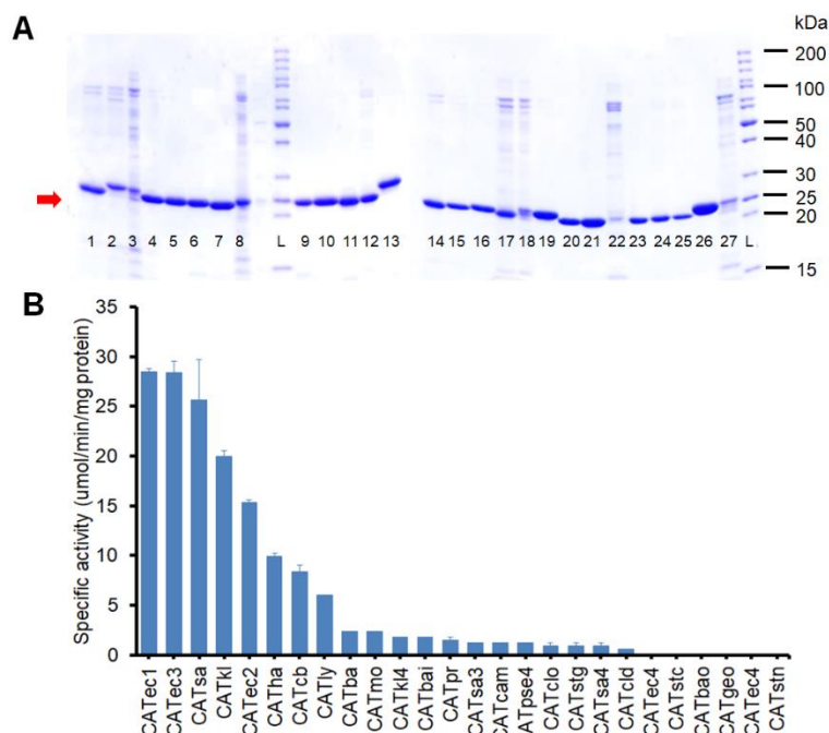
Figure 2-7: Screening of CATs for activity towards isobutanol. (A) SDS-PAGE of His-tag purified CATs. The protein samples were loaded at 500 ng per lane. From 1 to 27; CATsa, CAT_STRAC, CAT2_ECOLX, CAT_THEACI, CAT_BACI, CAT4_STAAU, CAT_BAOCl, CAT3_STAAU, CAT_PROMI, CAT_BACPU, CAT1_ECOLIX, CAT_KLEPS, CAT_CLOBU, CAT_GEO, CAT_CAMCO, CAT4_ECOLIX, CAT4_PSEAE, CAT_CLODI, CAT_LYSI, CAT4_MORMO, CAT1_CLOPF, CAT5_STAAU, CAT3_ECOLX, CAT4_KLEAE, CAT_STRAG, CAT2_HAEIF, and CAT_VIBAN. The red arrow indicates the average size of the CATs (24.9kDa). CAT_STAIN was not included because of unsuccessful expression. (B) Specific activity of CATs towards 100 mM isobutanol (mean \pm 1 stdev from two biological replicates).
