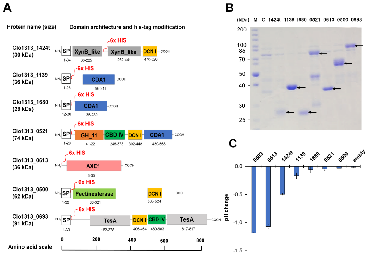
Figure 4-2: Identification of esterases responsible for isobutyl acetate hydrolysis in C. thermocellum . (A) Seven O-deacetylases in C. thermocellum and their domain architectures. The locations tagged with the histidine residues were marked as 6xHis in red. Clo1313_1424t is a truncated version of Clo1313_1424 which is derived from removal of the signal peptide and one XynB_like domain located at 36-225 residues that is identical to the other located at 252-441 residues. Abbreviation – SP: signal peptide, DCN: dockerin, CDA: carbohydrate deacetylase family, GH: glycosyl hydrolases family, CBD: cellulose binding domain, AXE: acetyl xylan esterase, and TesA: thioesterase A (lysophospholipase L1 or related esterase). (B) SDS-PAGE of purified His-tagged proteins expressed in the recombinant E. coli strains. Abbreviations – M: protein marker ladder and C: E. coli harboring an empty backbone plasmid. (C) In vitro screening of isobutyl acetate hydrolysis activities by endogenous CEs of C. thermocellum . The error bars represent standard deviation of three biological replicates.
