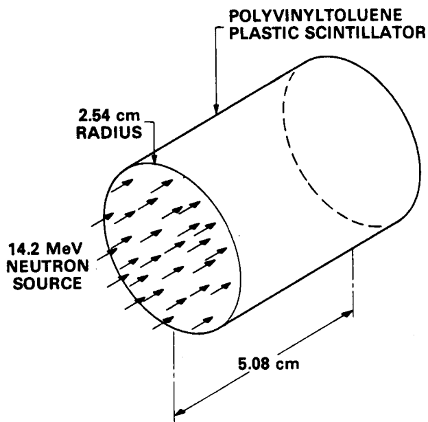
Figure 4-10. Geometry Configuration for the BC501 Polyvinyltoluene Plastic Scintillator.
