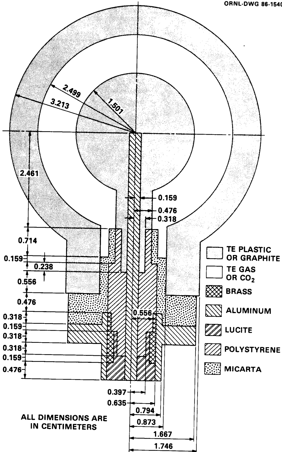
Figure 4-16. Geometry Configuration for the Armed Forces Radiobiology Research Institute (AFRI) 50 cm 3 Ionization Chamber.
