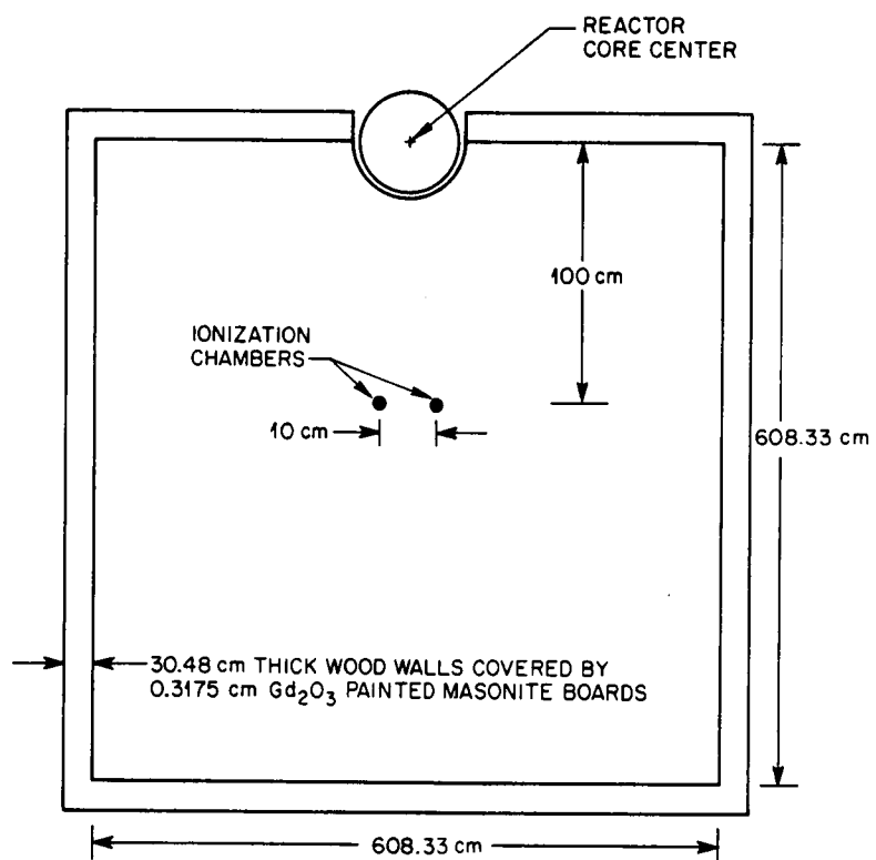
Figure 4-20. Schematic Top View of the Armed Forces Radiobiology Research Institute (AFRRI) Experimental Room One Free Field (ER1 FF) Experiment.
