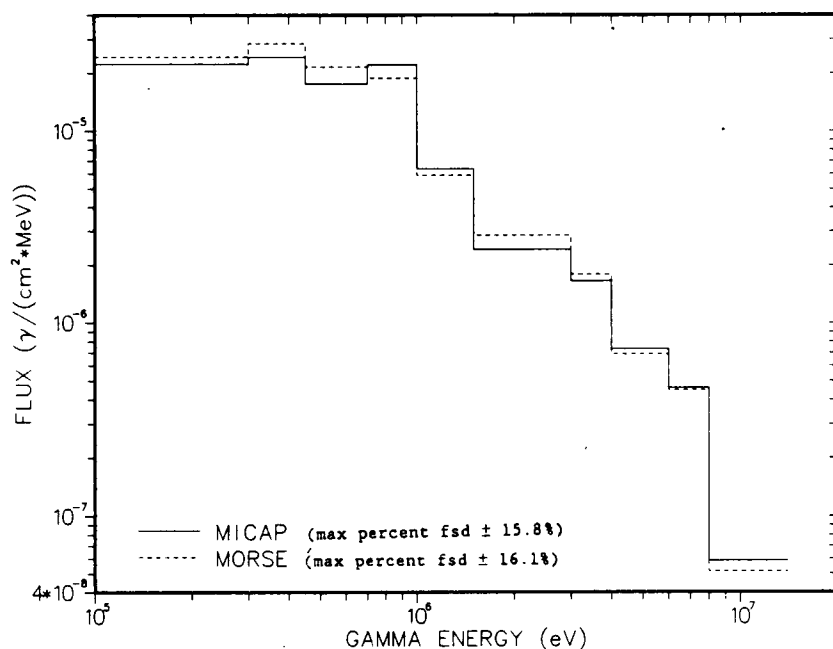
Figure 4-7. Comparison of MICAP and MORSE Photon Leakage Flux Spectra out the Back Face of a 50 cm x 50 cm x 20 cm Iron Slab with a Point Isotropic 14.0 MeV Neutron Source.
