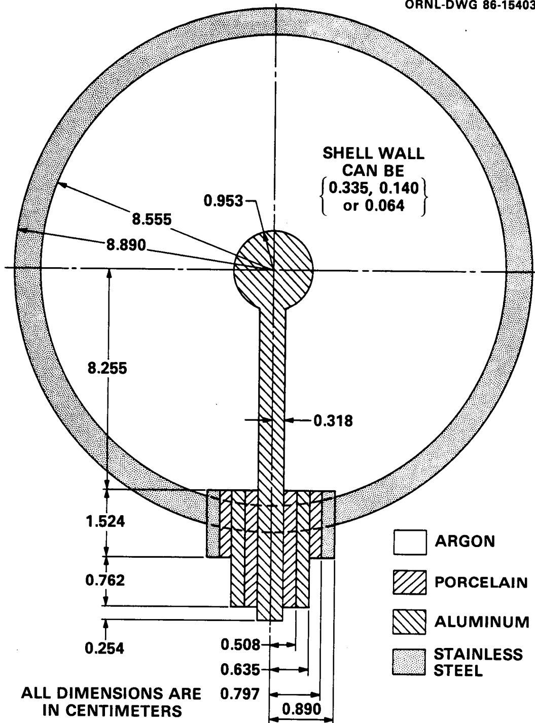
Figure 4-15. Geometry Configuration for the Health and Safety Laboratory (HASL) High Pressure Argon Ionization Chamber.
