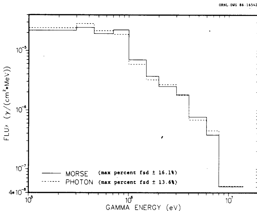
Figure 4-9. Comparison of PHOTON and MORSE Photon Leakage Flux Spectra out the Back Face of a 50 cm x 50 cm x 20 cm Iron Slab with a Point Isotropic 14.0 MeV Neutron Source using the MORSE Generated Secondary Photon Production Data.
