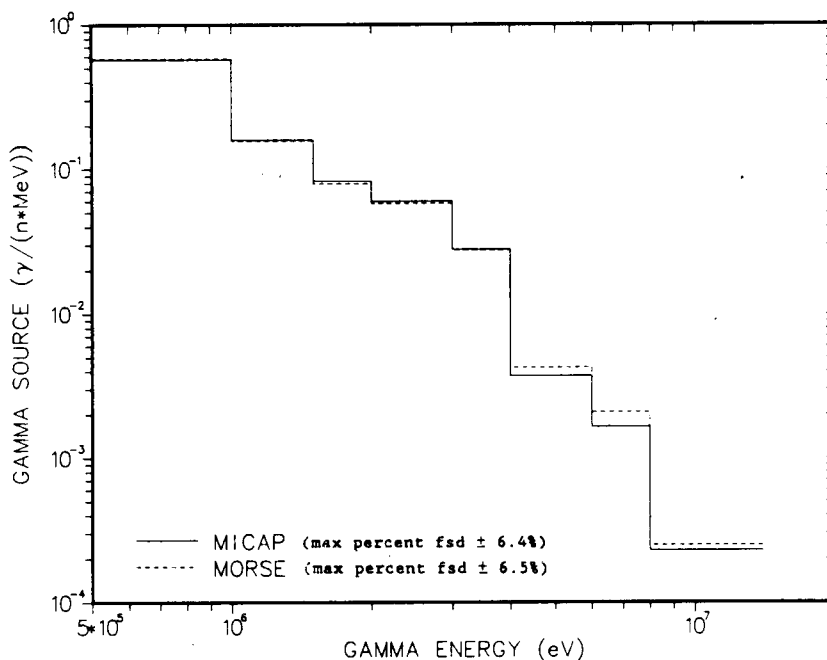
Figure 4-5. Comparison of MICAP and MORSE Secondary Photon Production Spectra in a 50 cm x 50 cm x 10 cm Iron Slab with a Point Mono-Directional Fission Neutron Source.
