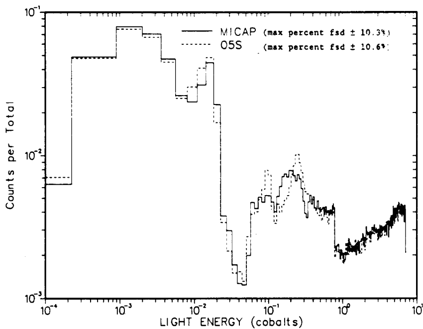
Figure 4-11. Comparison of MICAP and O5S Pulse Height Distributions for a BC501 Polyvinyltoluene Plastic Scintillator with a Mono-Directional 14.2 MeV Neutron Source.
