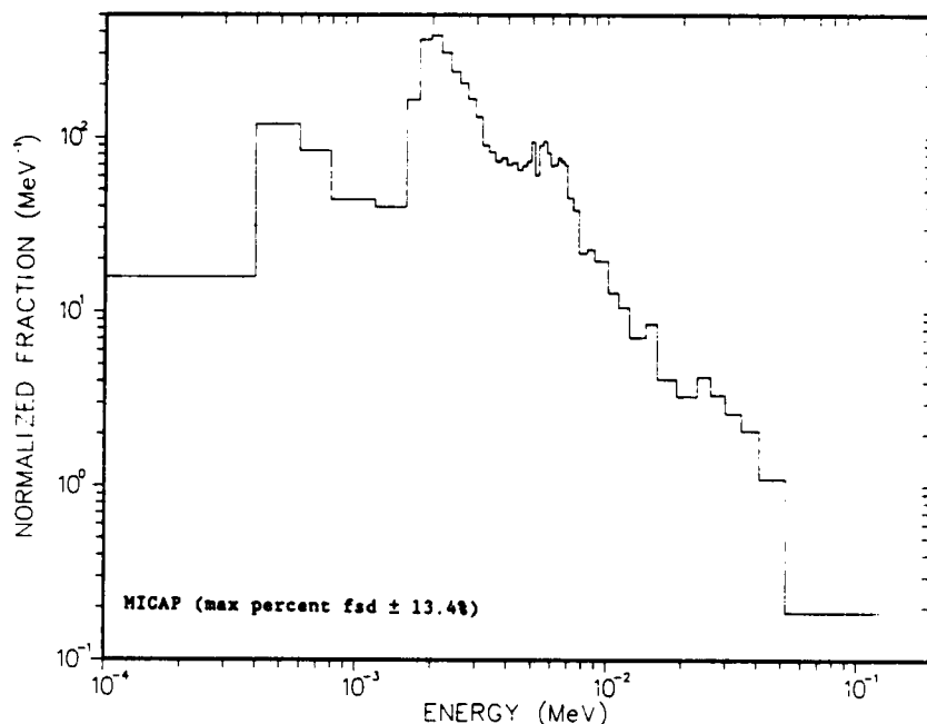
Figure 4-19. Pulse Height Distribution for the Armed Forces Radiobiology Research Institute (AFRRI) TE/TE 50 cm 3 Ionization Chamber due to a Mono-Directional 60 Co Photon Source.
