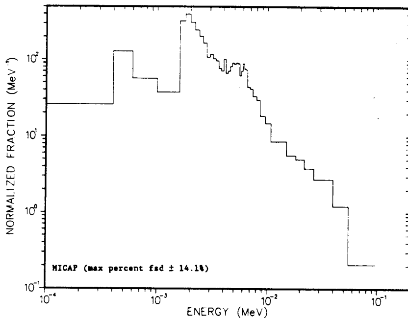
Figure 4-22. Pulse Height Distribution for the Armed Forces Radiobiology Research Institute (AFRRI) TE/TE 50 cm 3 Ionization Chamber due to a Mono-Directional 252 Cf Neutron Source.
