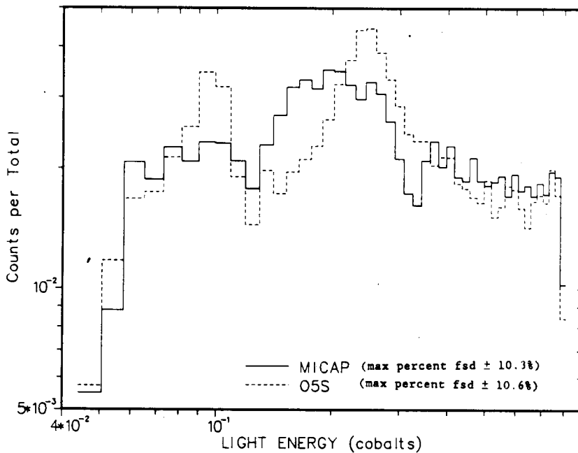
Figure 4-13. Comparison of MICAP and O5S Pulse Height Distributions due Predominantly to Alpha Recoil for a BC501 Polyvinyltoluene Plastic Scintillator with a Mono-Directional 14.2 MeV Neutron Source.
