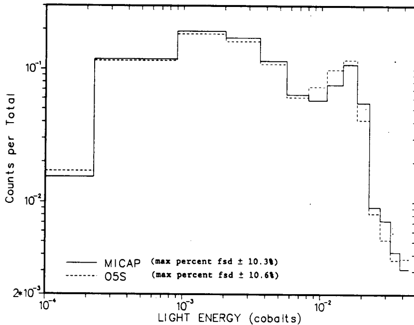
Figure 4-12. Comparison of MICAP and O5S Pulse Height Distributions due Predominantly to Carbon Recoil for a BC501 Polyvinyltoluene Plastic Scintillator with a Mono-Directional 14.2 MeV Neutron Source.
