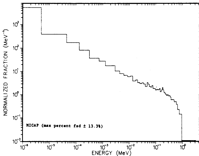
Figure 4-23. Pulse Height Distribution for the Armed Forces Radiobiology Research Institute (AFRRI) TE/TE 50 cm 3 Ionization Chamber due to a Mono-Directional 252 Cf Photon Source.
