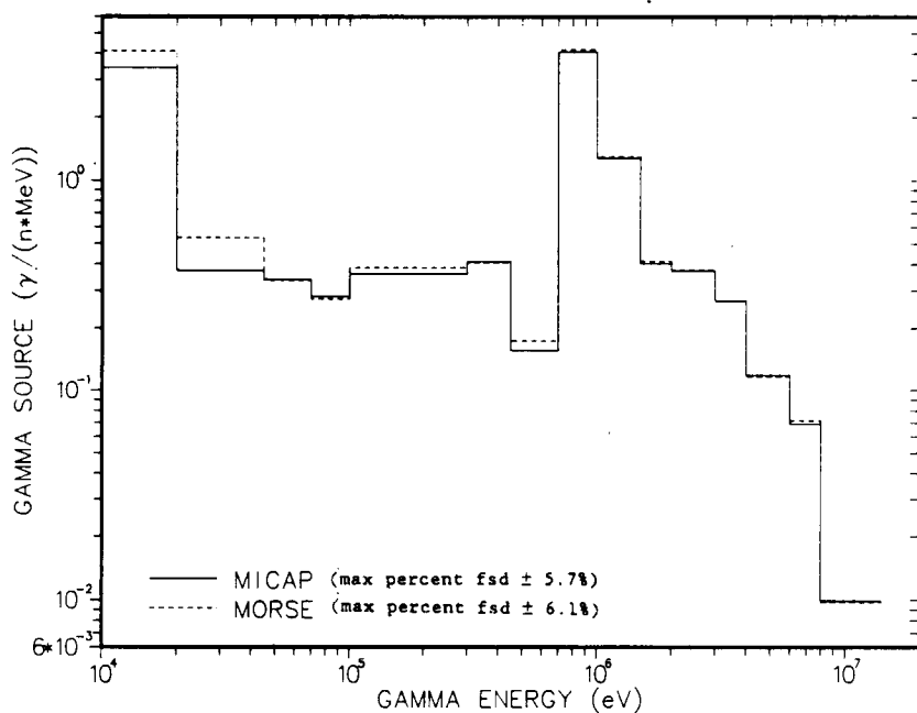
Figure 4-8. Comparison of MICAP and MORSE Secondary Photon Production Spectra in a 50 cm x 50 cm x 20 cm Iron Slab with a Point Isotropic 14.0 MeV Neutron Source.
