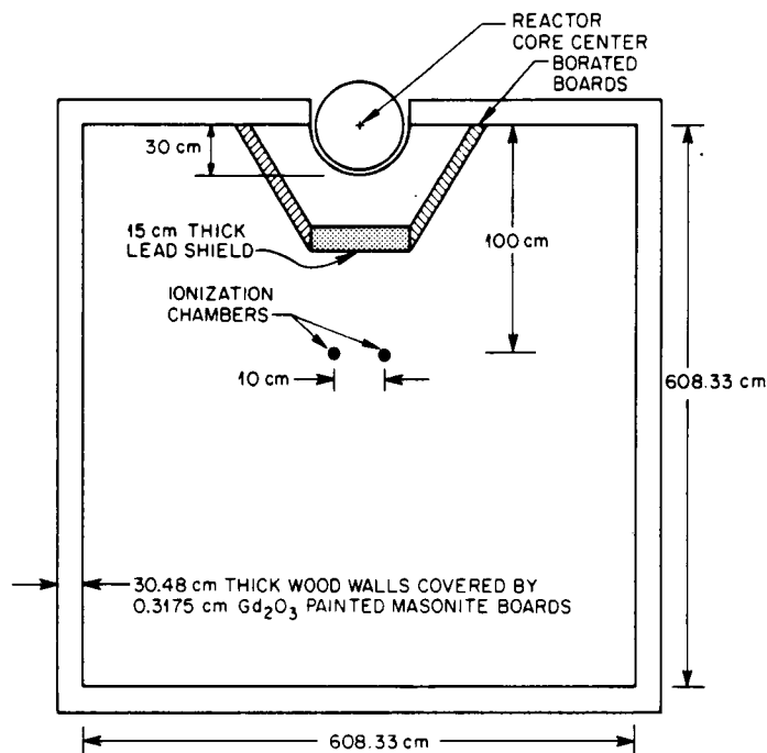
Figure 4-21. Schematic Top View of the Armed Forces Radiobiology Research Institute (AFRRI) Experimental Room One 15 cm Lead Shield (ER1 15 cm Pb) Experiment.
