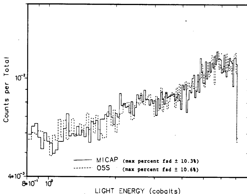
Figure 4-14. Comparison of MICAP and O5S Pulse Height Distributions due Predominantly to Proton Recoil for a BC501 Polyvinyltoluene Plastic Scintillator with a Mono-Directional 14.2 MeV Neutron Source.
