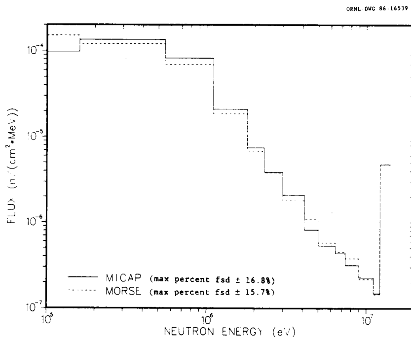
Figure 4-6. Comparison of MICAP and MORSE Neutron Leakage Flux Spectra out the Back Face of a 50 cm x 50 cm x 20 cm Iron Slab with a Point Isotropic 14.0 MeV Neutron Source.
