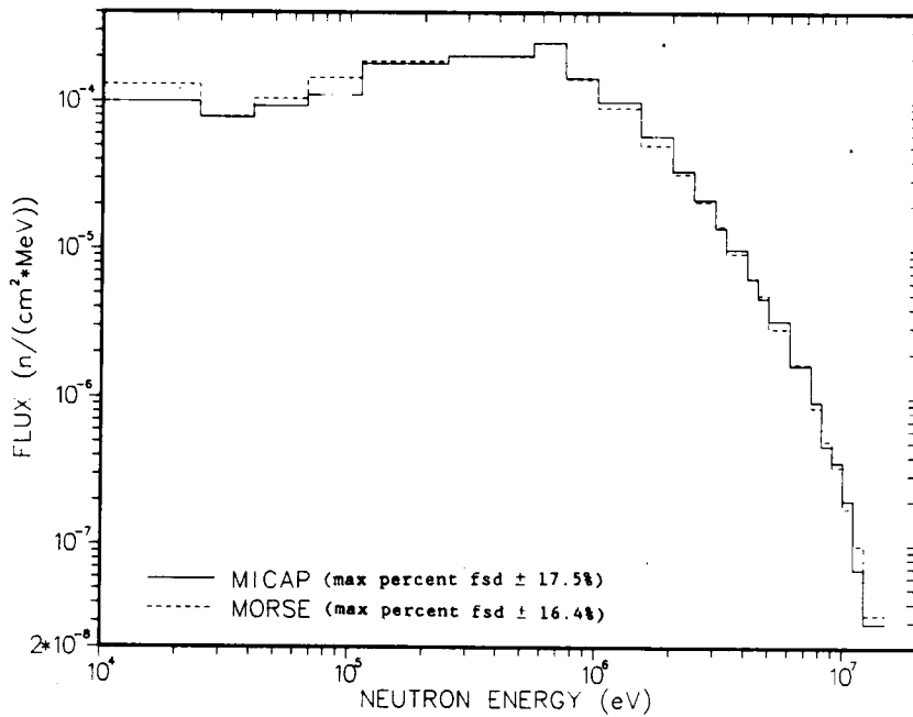
Figure 4-3. Comparison of MICAP and MORSE Neutron Leakage Flux Spectra out the Back Face of a 50 cm x 50 cm x 10 cm Iron Slab with a Point Mono-Directional Fission Neutron Source. (max percent fsd represents maximum percent fractional standard deviation)
