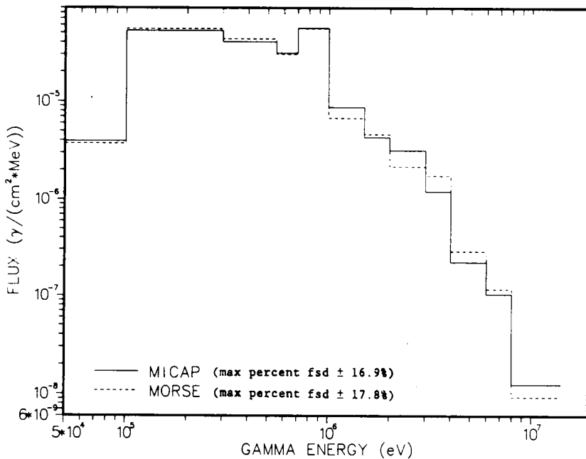
Figure 4-4. Comparison of MICAP and MORSE Photon Leakage Flux Spectra out the Back Face of a 50 cm x 50 cm x 10 cm Iron Slab with a Point Mono-Directional Fission Neutron Source.
