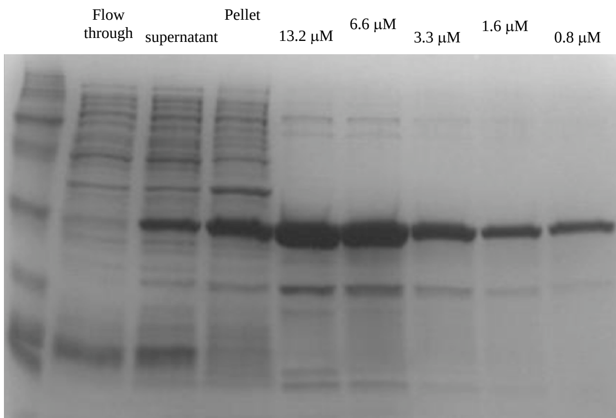
Figure 2-4: SDS-PAGE of different concentrations of purified EGFP
