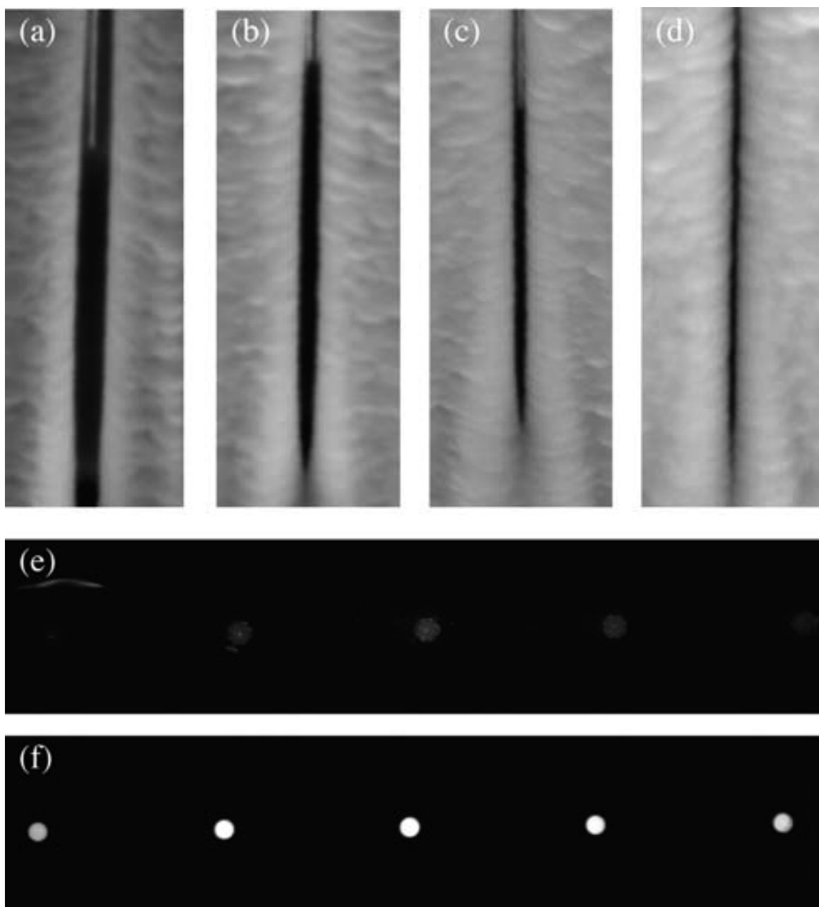
Figure 2-8: The deposition of silicon dioxide on membrane structures can be used to reduce pore width. Pores are shown after (a) 2, (b) 4, (c) 6, and (d) 8 min of PECVD silicon dioxide deposition. The retention of green fluorescent protein was observed after 5 min in reaction vessels coated with silicon dioxide for (e) 4 min (100 ms digital camera exposure) and (f) 6 min (50 ms digital camera exposure). Each of the devices shown was filled with the same concentration of EGFP.
