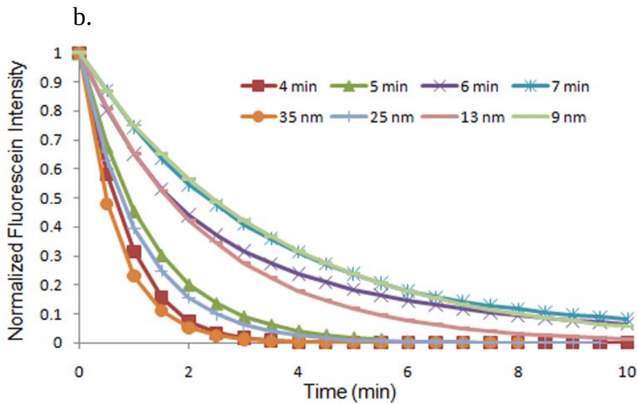
Figure 2-11: Experimental diffusion data vs. the diffusion model. a) Normalized EGFP diffusion data for devices that have undergone 4, 5, 6 and 7 minute PECVD vs. the diffusion model for pore widths of 35, 25, 13 and 4 nm. b) Normalized fluorescein diffusion data for devices that have undergone 4, 5, 6 and 7 minute PECVD vs. the diffusion model for pore widths of 35, 25, 13 and 9 nm.
