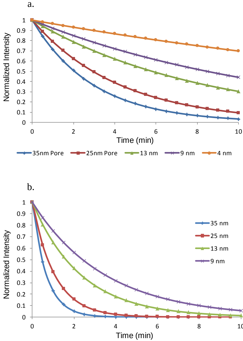
Figure 2-10: Lumped Capacitance Diffusion model (a) EGFP and (b) fluorescein for predicting transient changes in concentration within the cell mimic device with different pore widths of 35, 25, 13 and 9 nm under moderate external flow.
