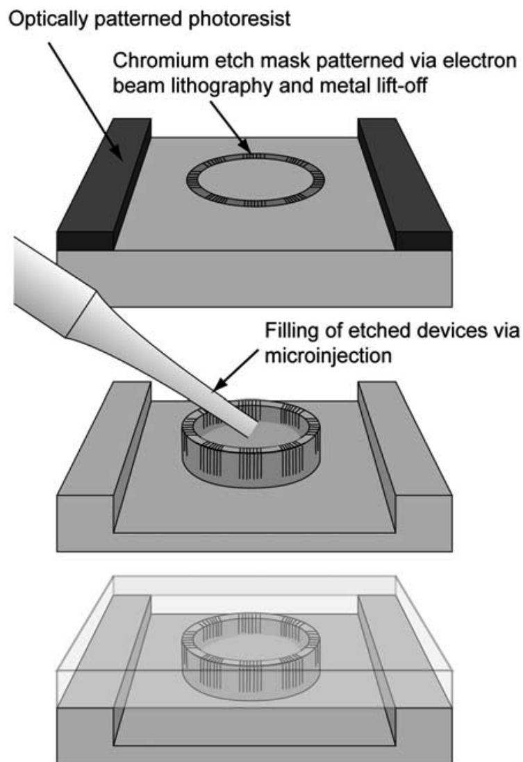
Figure 2-3: Nanoporous reaction devices are fabricated within microfluidic channels by combining electron beam lithography and metal lift-off techniques with contact photolithography to define the reaction vessel and channel geometries (top). The pattern is transferred into the exposed silicon using cryogenic silicon etching and individual vessels are filled with reactants via microinjection (middle). The entire chip is then sealed with PDMS (bottom) [159].
