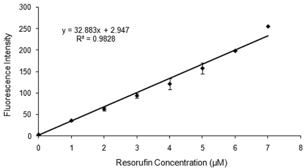
Figure 3-2: Resorufin standard curve. A standard curve showing the fluorescent intensity according to the resorufin concentration in the device. Error bars are \pm 1 SD.
