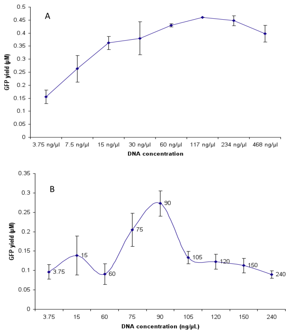
Figure 4-8: Cell-free protein expression in (a) plate reader and (b) no slit device. The graph represents the protein concentration, corresponding to the observed fluorescence intensity, from three protein synthesis experiments (3 individual devices on 3 separate chips). Error bars represent +/- one standard deviation.
