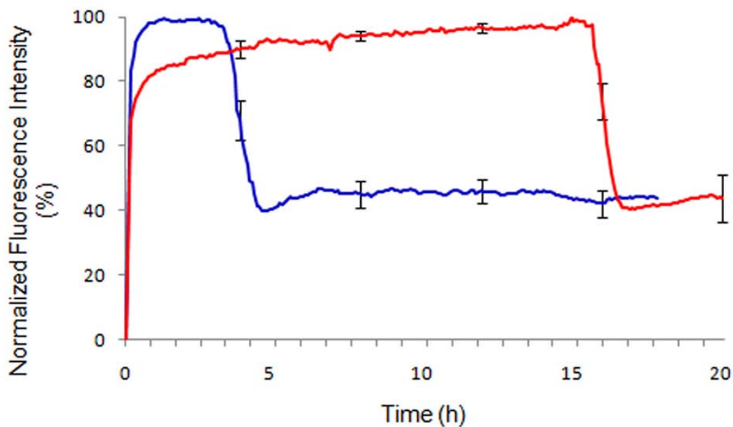
Figure 5-5: Blockage of protein synthesis by antibiotic treatment, . Adding chloramphenicol at selected time points blocked the protein synthesis reaction allowing estimation of protein loss from the device. Chloramphenicol was introduced in the reaction after 3 and 15 hours by switching to an alternate flow stream, upstream of the fluidic chamber that contains the array of cell mimic devices. The graph represents the average normalized intensity recorded from 3 individual reaction containers during 3 separate experiments. Error bars representing \pm one standard deviation are shown at 4 hour intervals for clarity.
