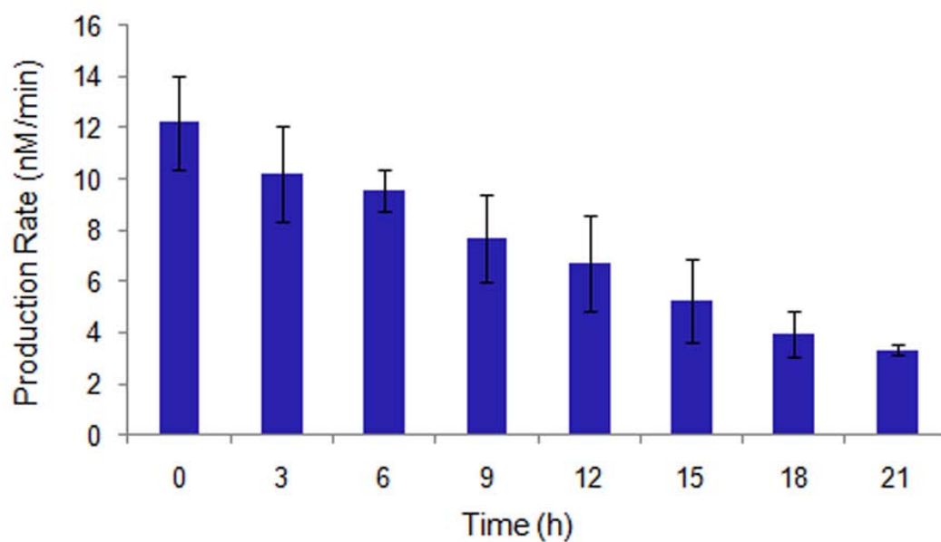
Figure 5-4: Fluorescence recovery rates. A steady decrease in the production rate, the rate of new protein synthesis as measured by the increase in fluorescence, is observed as reaction time progresses. Recovery rates were calculated by measuring the slope of photobleaching recovery curves for the first five minutes following the photobleach pulse. Error bars represent +/- one standard deviation
