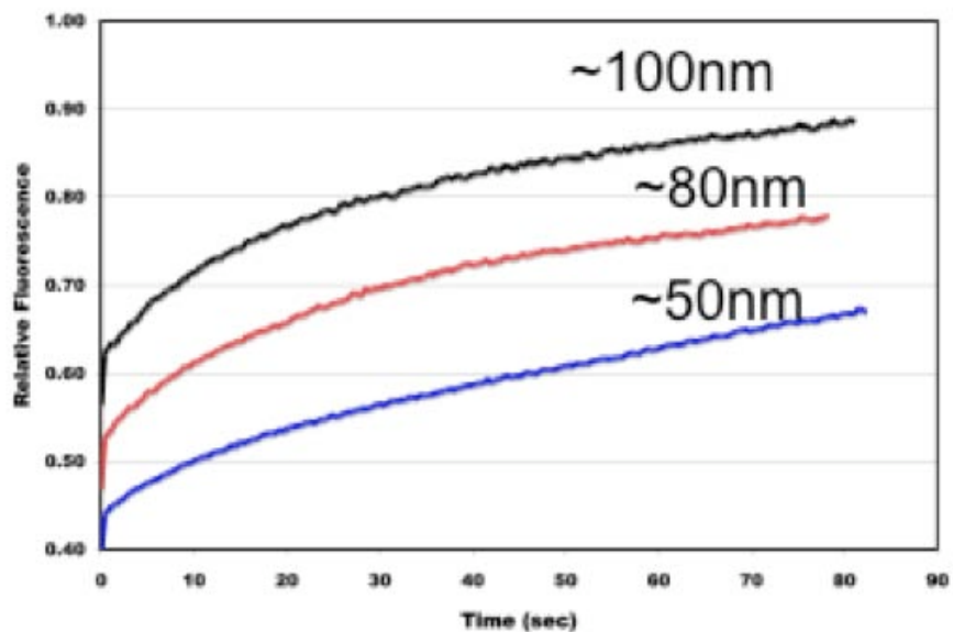
Figure 2-5: Fluorescence Recovery After Photobleaching. (a) Presentation of data collected during a FRAP experiment. Fluorescence is collected before and after photobleaching occurs. Over time, the unbleached molecules diffuse into the photobleached area and the amount of fluorescence increases [161]. (b) Fluorescent recovery of reaction vessels with different nominal pore sizes.
