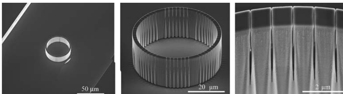
Figure 2-1: Scanning electron micrographs of containment vessels for assessing diffusive loss taken prior to filling and sealing show the integration of porous vessels within a microfluidic channel (left), the overall device size and pore locations (center) and nominal pore size (right). Images were taken at a 30° stage tilt.
