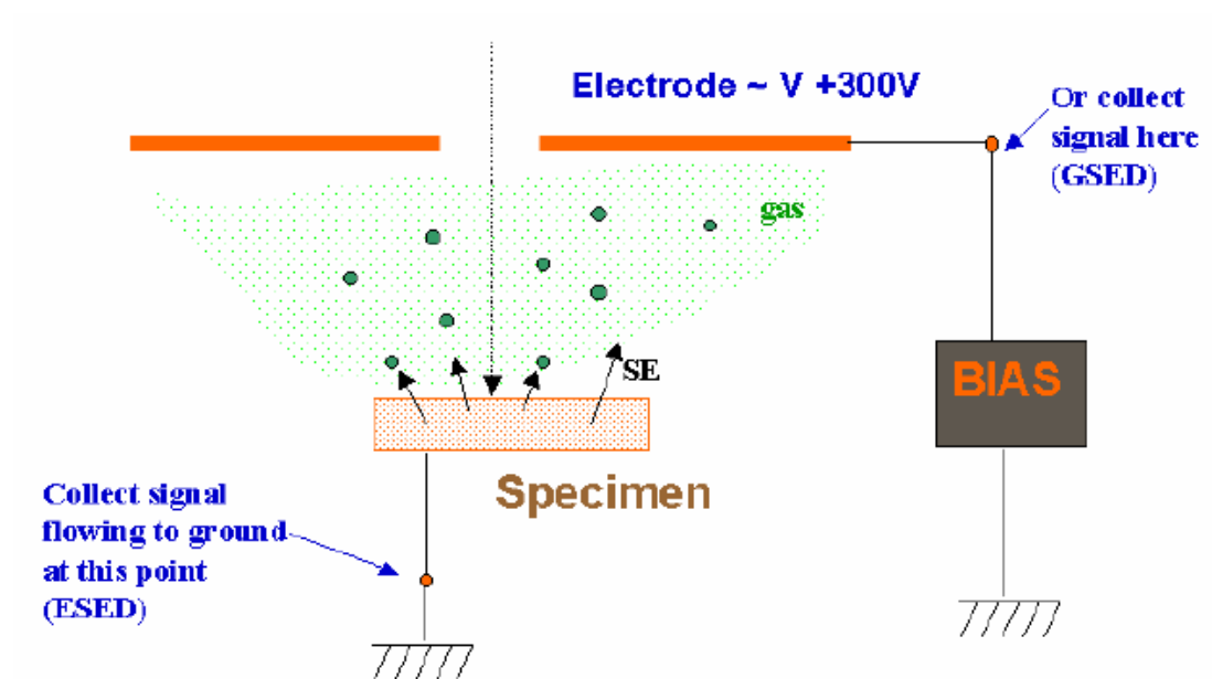
Figure 1-13: Schematic diagram of signal detection for SE imaging on VPSEM. Image courtesy of Joy D.C. [30].
