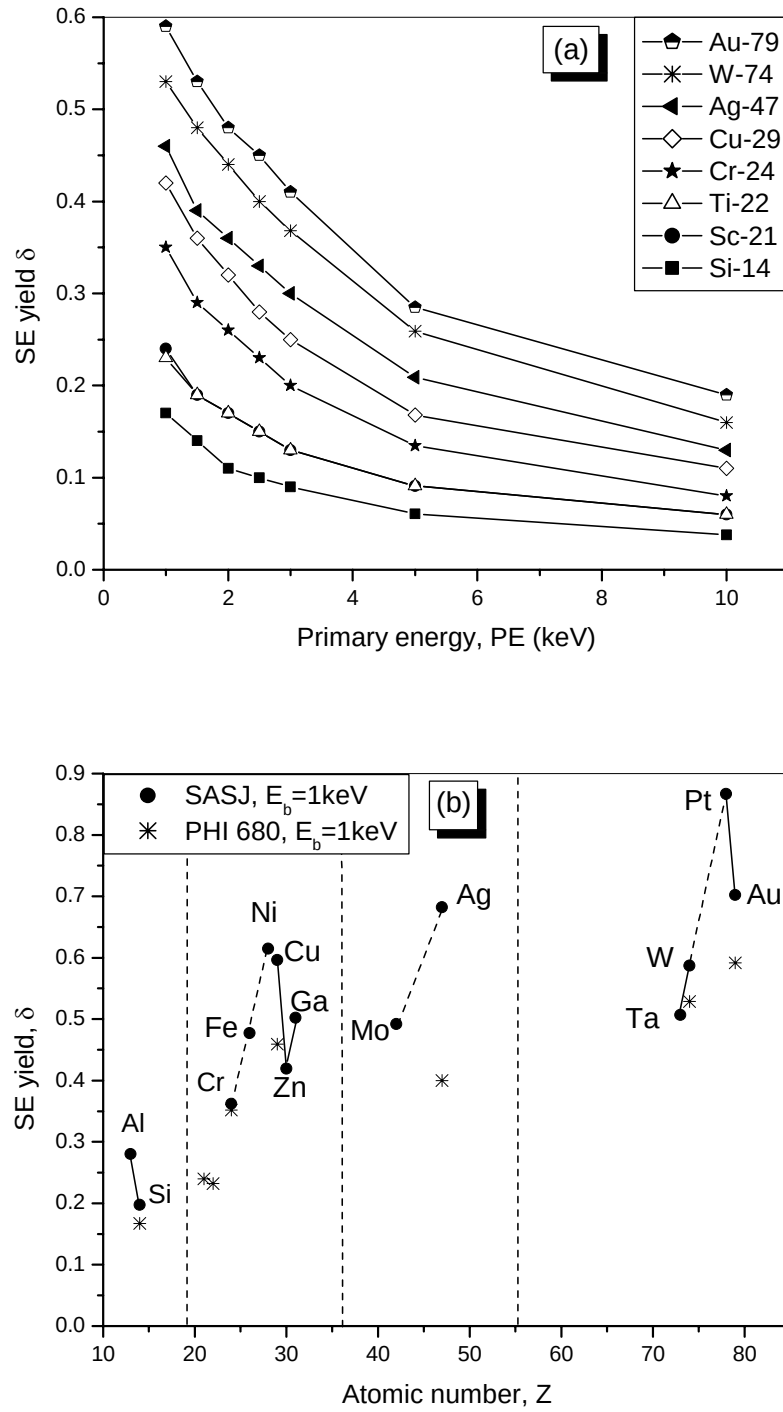
Figure 5-5: (a) The SE yields of elements measured on PHI 680 SAN vary with beam energy. (b) Comparison of the SE yields at beam energy of 1 keV measured on the PHI 680 SAN and that of SASJ as a function of atomic number demonstrates an atomic shell filling effect.
