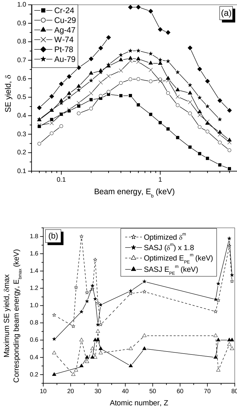
Figure 5-3: (a) SE yields \delta calculated from the SASJ database varying with the beam energy E_b . (b) Comparison of the maximum SE yield \delta^m and the corresponding beam energy E_{PE}^m varying with atomic number with the optimized data in chapter 3.
