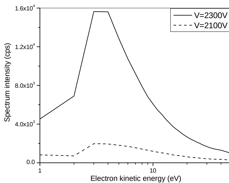
Figure 4-11: Comparison of a SE spectrum under 2300 V and 2100 V MCP voltage shows that increasing the multiplier voltage produces a much higher output count rate for weak electron signal in PHI 680.
