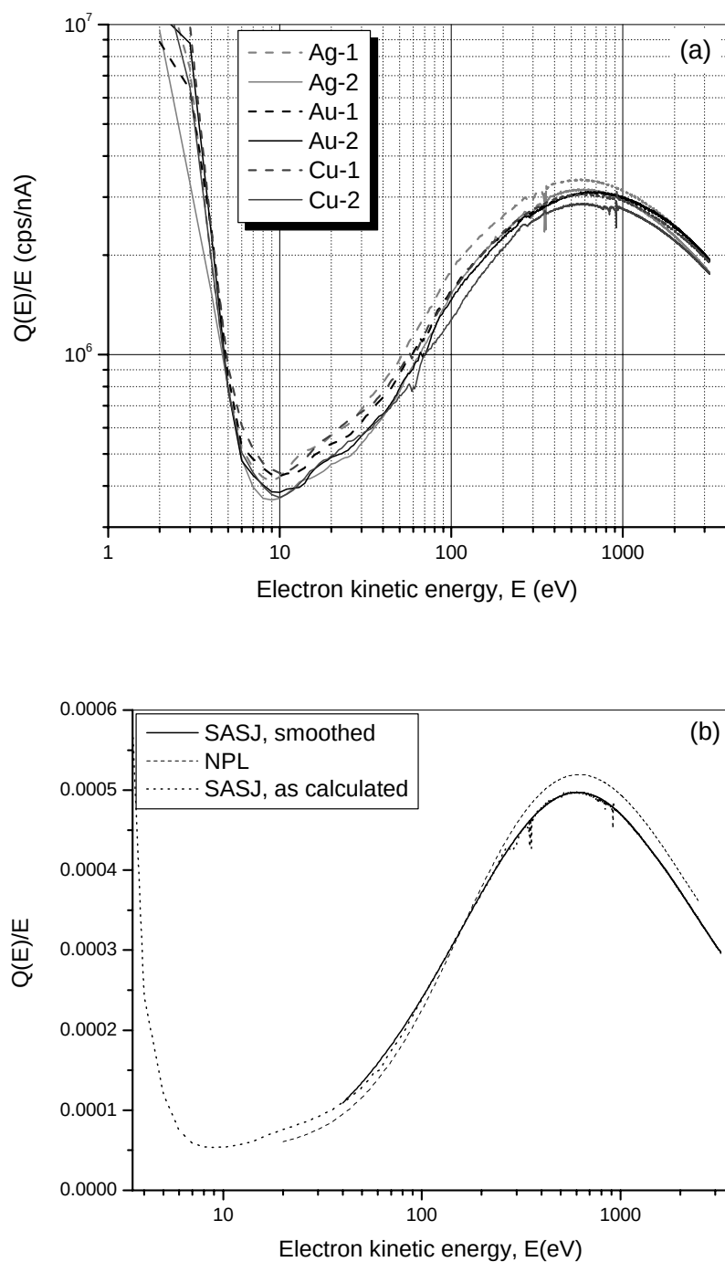
Figure 4-16: The Q(E)/E for PHI 680 SAN. (a) Calibration based on Goto's absolute spectra on the SASJ data bank. The Q(E)/E lines are for two sets of measurement on Ag, Au and Cu. (b) Q(E)/E produced by the two institutes agree well with each other. The Q(E)/E are converted to be unitless. The smoothed SASJ data are presented in the range of 40~3200 eV.
