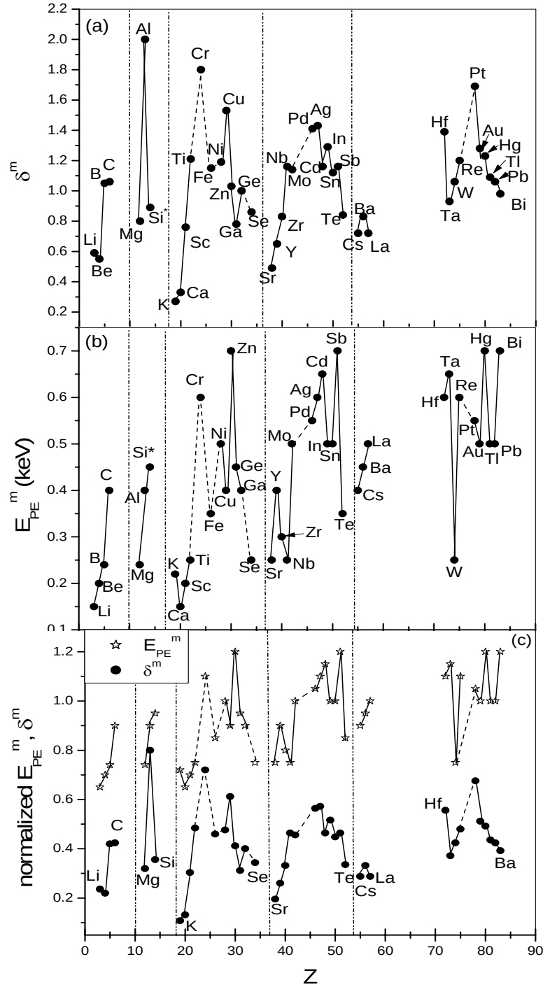
Figure 3-8: Maximum SE yield \delta^m (a) and corresponding primary energy E^m_{PE} (b) as functions of atomic number Z . (c) E^m_{PE} normalized to 1keV and \delta^m normalized to 2.5 show recognizable similar shape and shell filling effect. Solid lines connect neighboring elements, dashed lines connect non-consecutive atomic number. Normalized E^m_{PE} are shifted 0.5 up to make plot clear.
