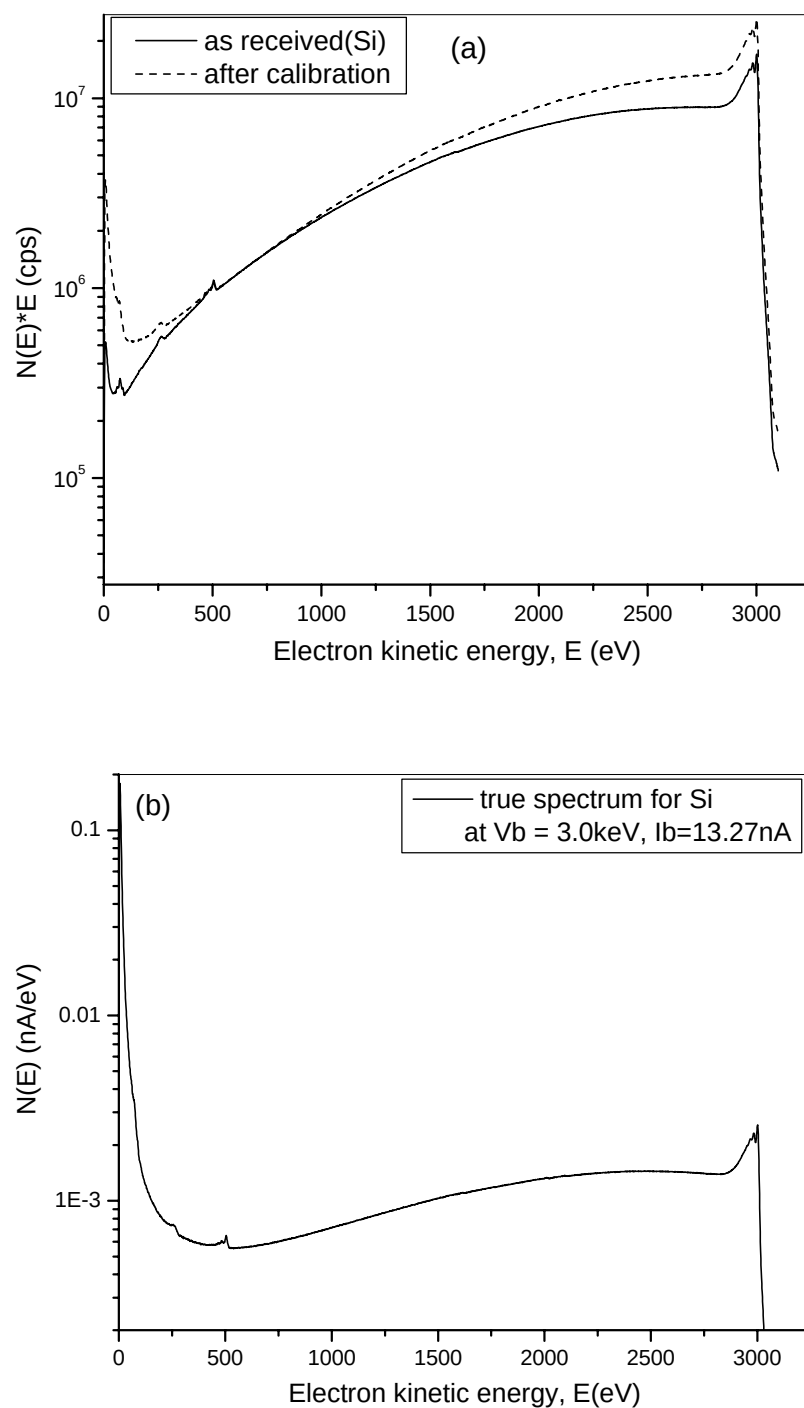
Figure 4-17: (a) Comparison of spectra for Si collected on PHI 680 SAN before and after intensity calibration. The calibrated spectrum has much higher intensity at low and high energies. (b) The calibrated Si spectrum corrected for the CMA transmission efficiency.
