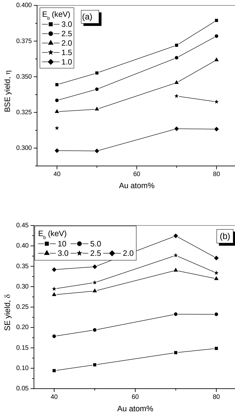
Figure 5-11: The variation of yields with element gradient in the Cu-Au binary alloys. (a) BSE yield linearly increases with Au atomic percent. (b) SE yield almost linearly increases with Au atomic percent.
