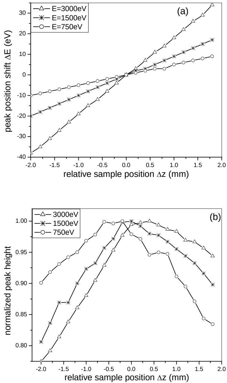
Figure 4-7: Deviation of sample position from CMA focus point in the axis direction in PHI 680 SAN cause spectrum distortion. Legends note the energy of the electrons forming the peak. The sample position is relative to the one calibrated with the 1000 eV elastic peak, (a) Peak position shift \Delta E with sample position \Delta z . (b) Peak intensity reduction with \Delta z . Noted that electrons with different energies show different CMA focus positions.
