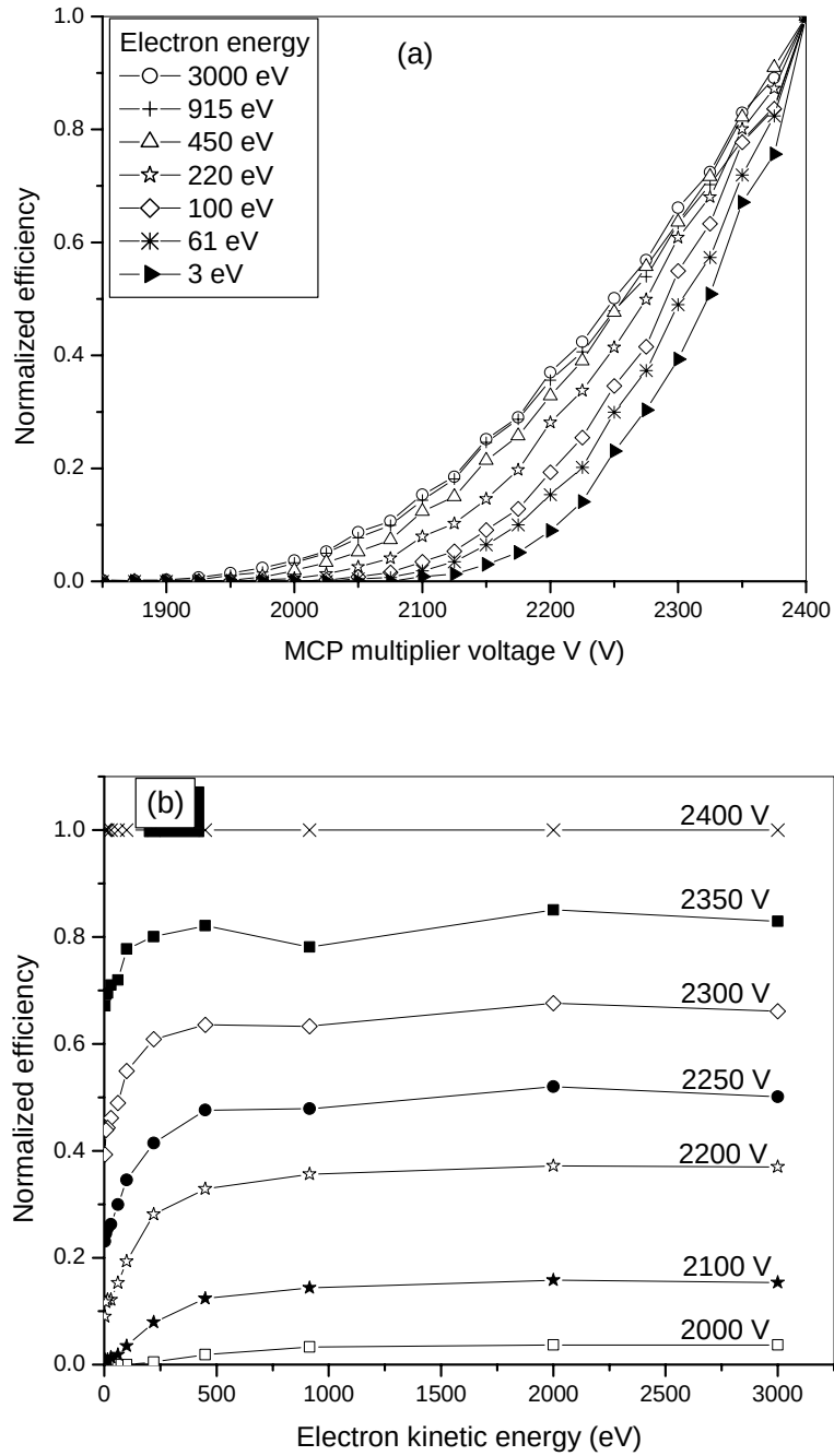
Figure 4-10: Responses of the detection efficiency for MCP in PHI 680 SAN to the multiplier voltage V and the electron energy. (a) Detection efficiency as a function of multiplier voltage V . The increasing tendency at high V indicates that the MCP is operated below saturation point. (b) Detection efficiency as a function of electron kinetic energy increase with multiplier voltage.
