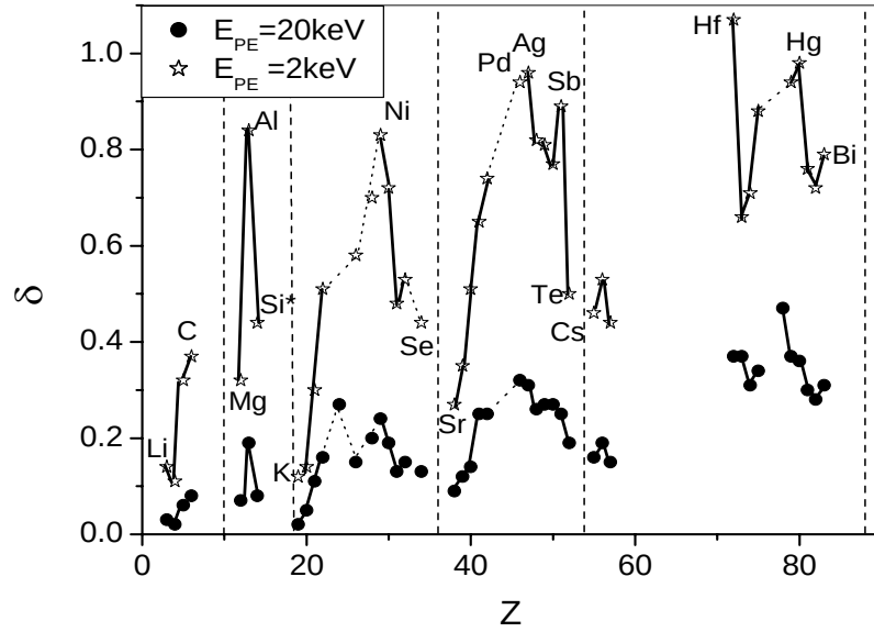
Figure 3-6: SE yield \delta as a function of atomic number Z has similar trends for beam energy E_{PE} at 2 keV and 20 keV. Solid lines connect neighboring elements; dashed lines connect elements with uncontinuous atomic number.
