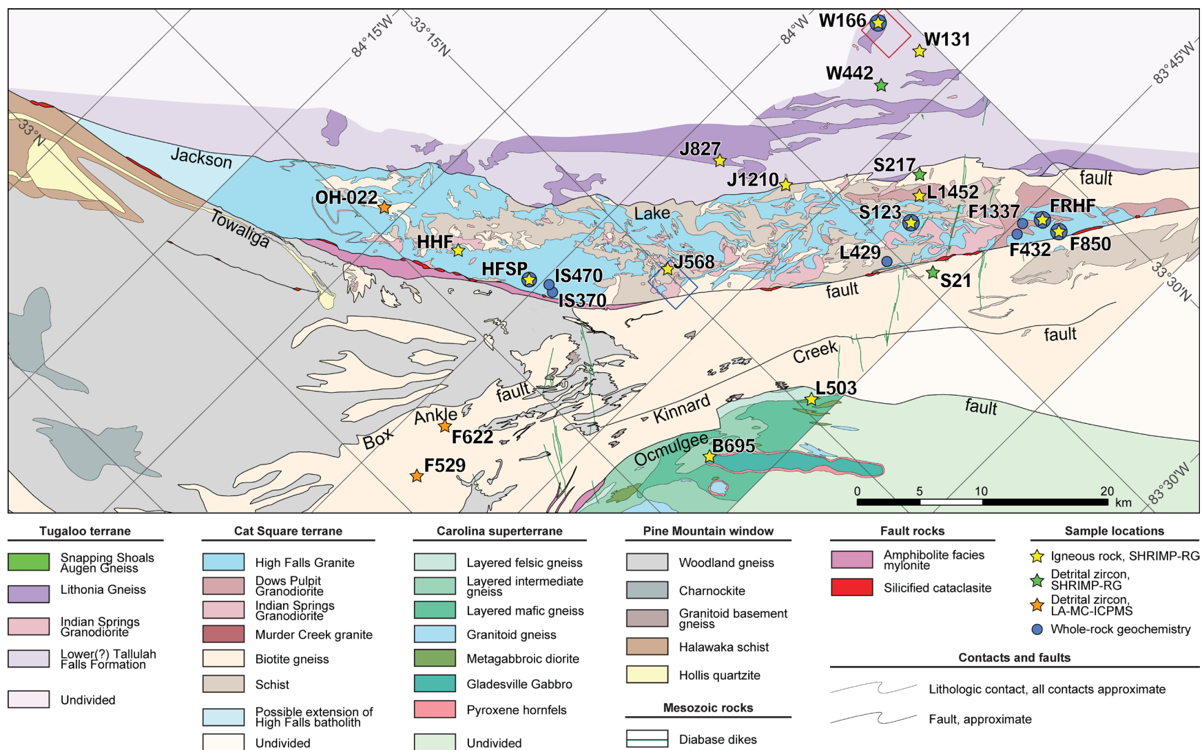
Figure 2-4: Compiled geologic map of the central Georgia portion of the Inner Piedmont with geochronologic and geochemical sample locations. Sources of geochemical data listed in appendix III. LA-MC-ICPMS detrital zircon data from J.R. Rehrer, unpublished data. The red and blue boxes indicate the locations of maps in figures 3-6 and 3-8, respectively. Location of map is shown in Fig. 2-1.
