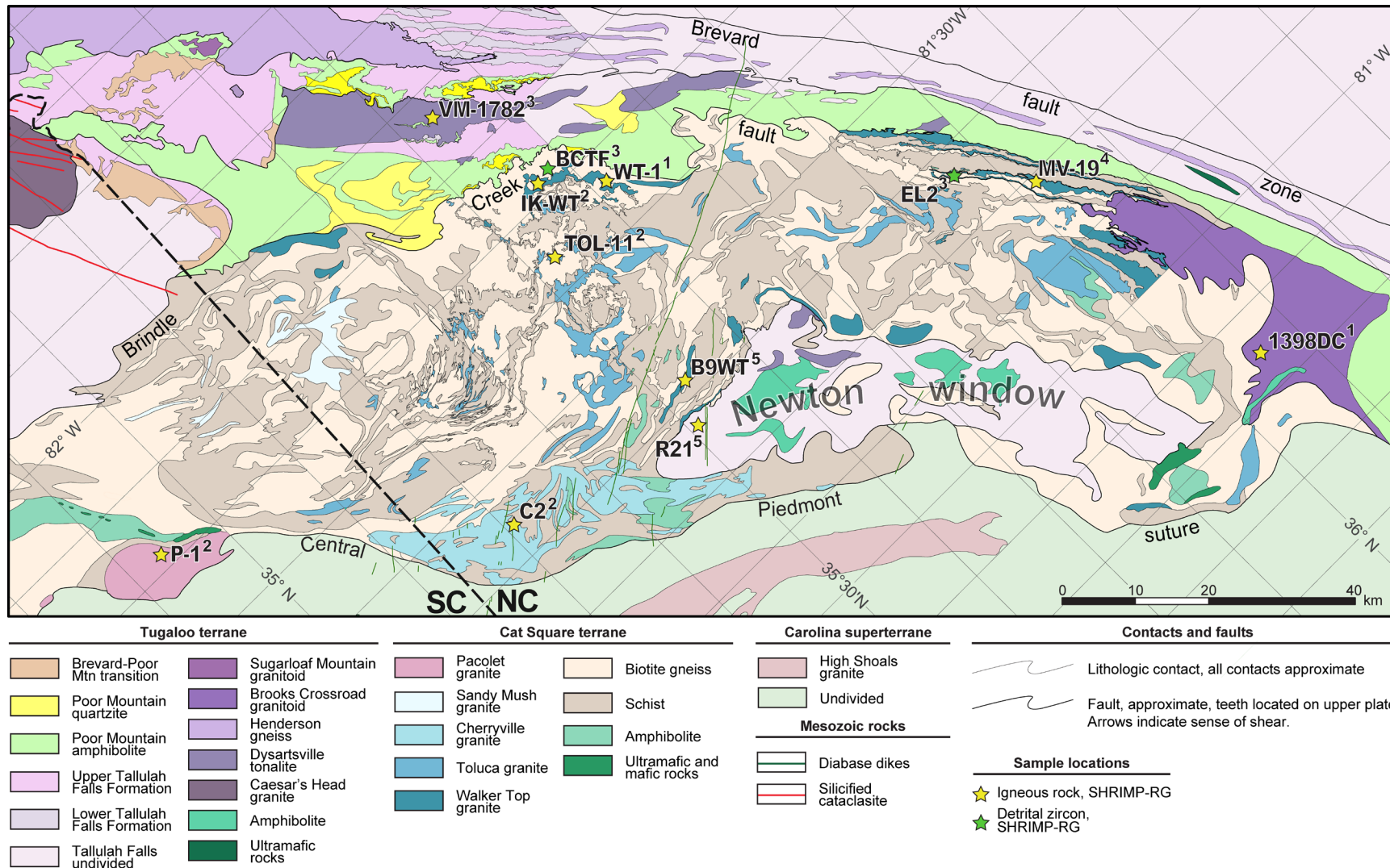
Figure 2-2: Geologic map of the Carolina portion of the Inner Piedmont (modified from Mersch, ms, 2009) with sample locations of compiled U-Pb ion microprobe granitoid ages and detrital zircon analyses. Ages summarized in table 2. Data sources: 1 Vinson (ms, 1999); 2 Mapes (ms, 2002); 3 Bream (ms, 2003); 4 Gatewood (ms, 2007); 5 Byars (ms, 2010). Location of map is indicated in Fig. 1.
