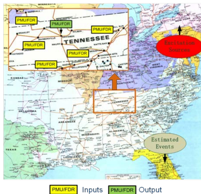
Figure 5-8 Illustration of Dynamic Response Estimation
