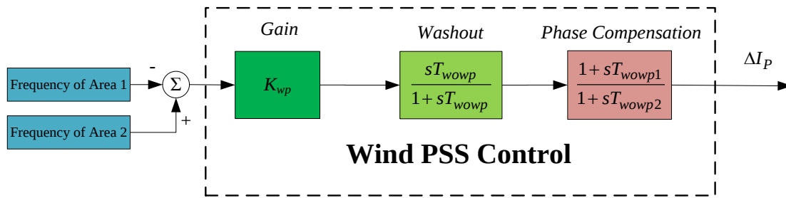
Figure 3-15 Wind PSS Control Structure
