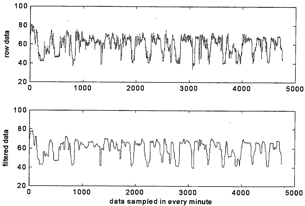
Figure 6.3 Measured and filtered Combustion Air Flow (Pct) (WinSize = 25)
