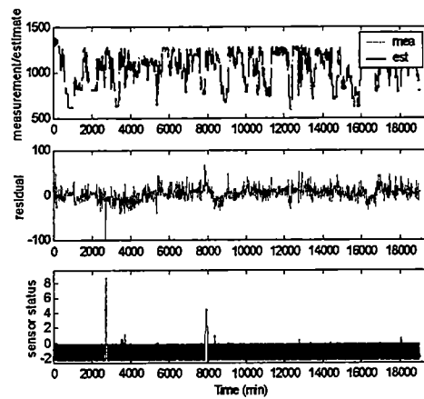
Figure C12 Prediction on First Stage Pressure B (psig)
