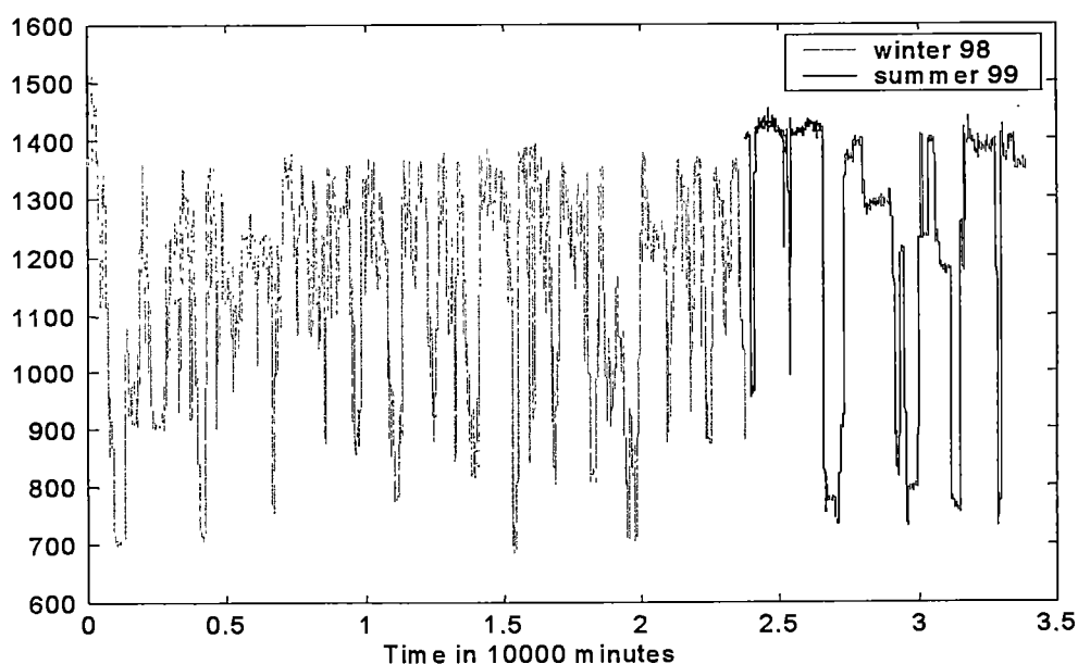
Figure 6.6 Operating condition change of Feedwater Flow (Klb/hr)
