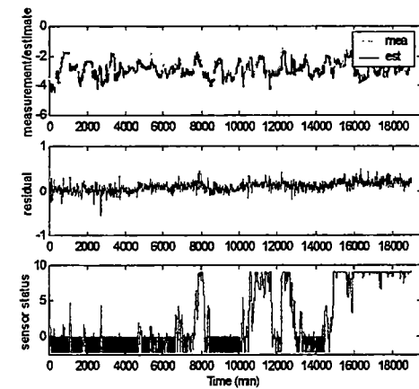
Figure C30 1%/day drift on RH Furnace Pres. after Econ (InH2O)
