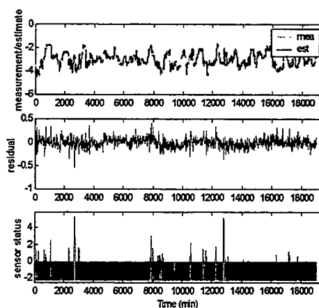
Figure C16 Prediction on RH Furnace Pres. after Econ (InH2O)
