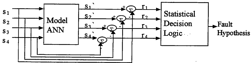
Figure 3.2 AANN-based Sensor monitoring module
