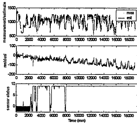
Figure C25 1%/day drift on First Stage Pressure A (psig)
