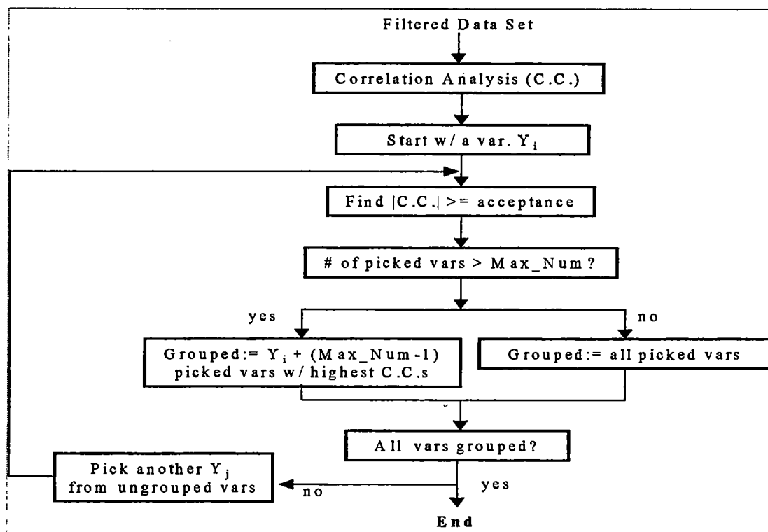
Figure 4.5 Variable inclusion algorithm
