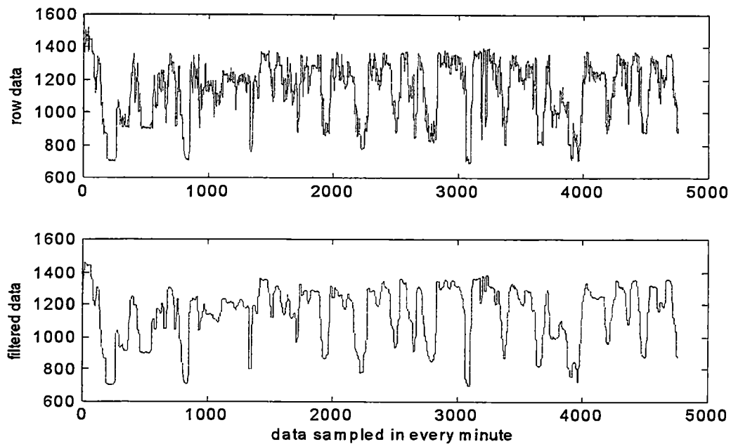
Figure 6.4 Measured and filtered Feedwater Flow (Klb/hr) (WinSize = 25)
