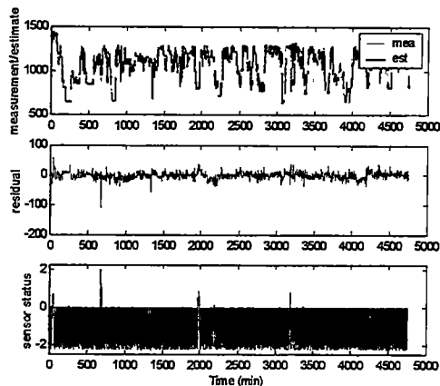
Figure C4 Recall on Measured Steam Flow (Klb/hr)
