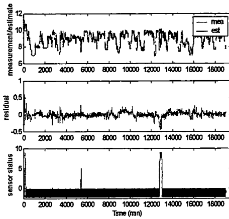
Figure C10 Prediction on Station Service Load (MW)
