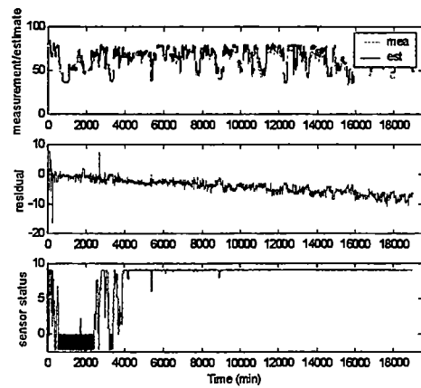
Figure C27 1%/day drift on Deaerator Pressure (psig)
