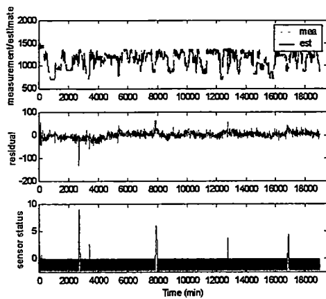
Figure C39 FW Flow (Klb/hr) after recovery
