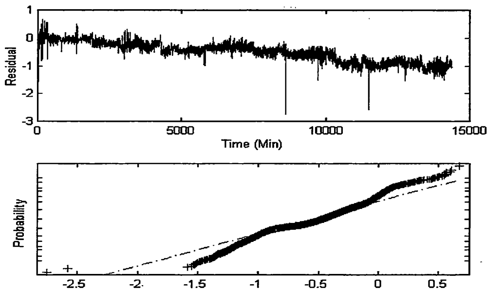
Figure 5.7 Residual normal probability plot
