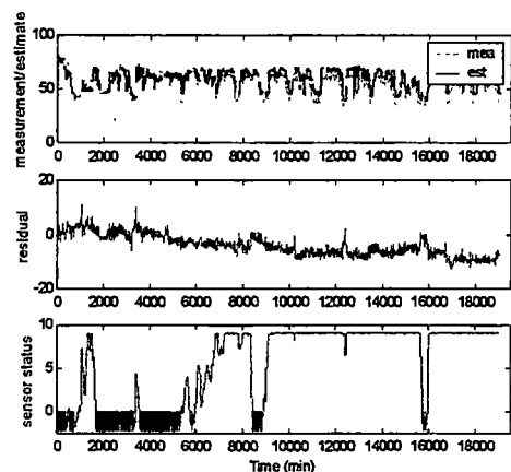
Figure C21 1% /day drift on Combustion Air Flow A1 (Klb/hr)
