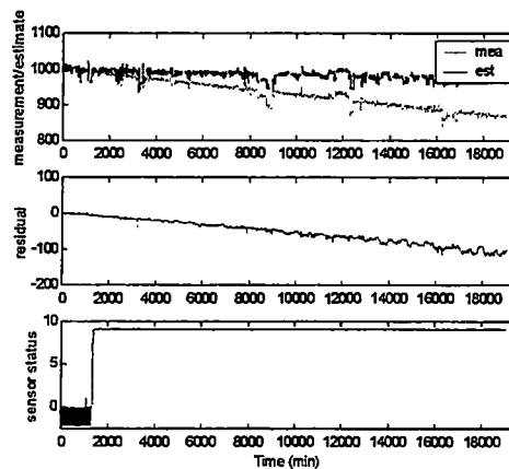
Figure C32 1%/day drift on SH Outlet Temp. #2 (DegF)
