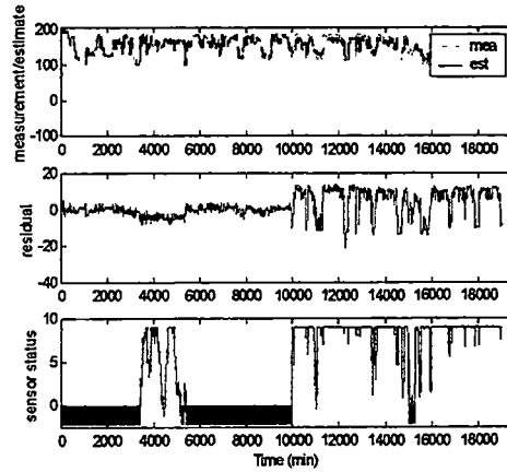
Figure C40 Predicted Unit Gross Gen. (MW) w/ faulty FW Flow #1
