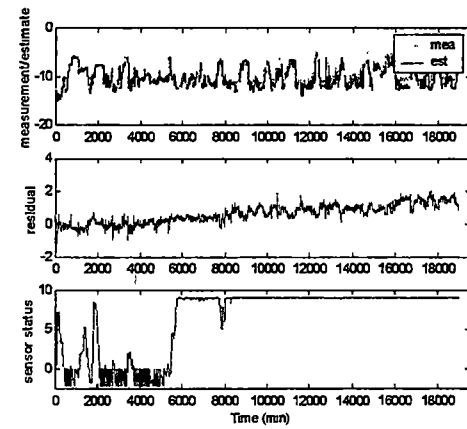
Figure C28 1%/day drift on ID Fan A Suction Pressure (InH2O)
