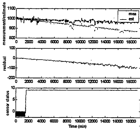
Figure C31 1%/day drift SH Outlet Temp. #1 (DegF)
