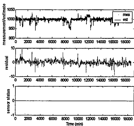
Figure C17 Prediction on SH Outlet Temp. #1 (DegF)
