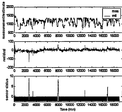
Figure C43 Corrected FW Flow #1 with 20% drop
