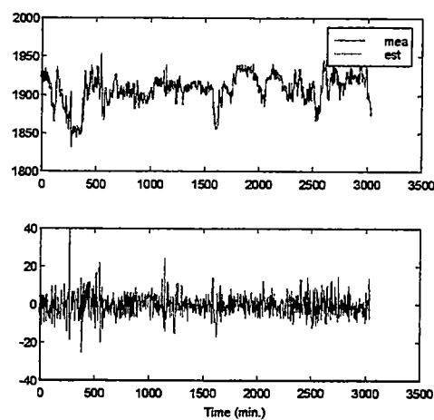
Figure B4 TDNN recall on Selected Drum Pressure (psig)
