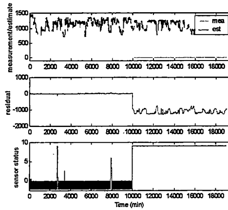
Figure C37 Predicted Unit Gross Gen. (MW) w/ bad FW Flow #1 Figure C38 Predicted lost FW Flow (Klb/hr) starting at 10000 th min.
