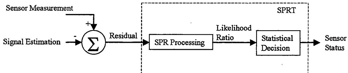
Figure 3.4 SPRT algorithm block diagram
