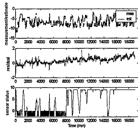
Figure C29 1%/day drift on ID Fan B Suction Pres. (InH2O)
