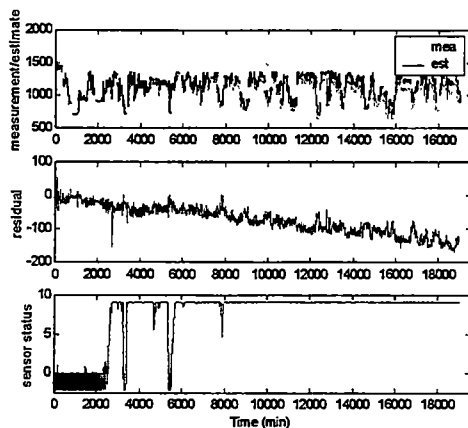
Figure C19 1%/day drift on FW Flow (Klb/hr)
