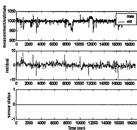
Figure C18 Prediction on SH Outlet Temp. #2 (DegF)
