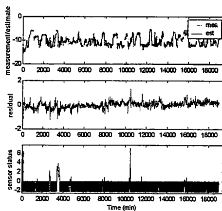
Figure C14 Prediction on ID Fan A Suction Pres. (InH2O)
