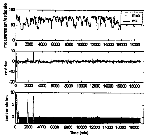
Figure C13 Prediction on Deaerator Pressure (psig)
