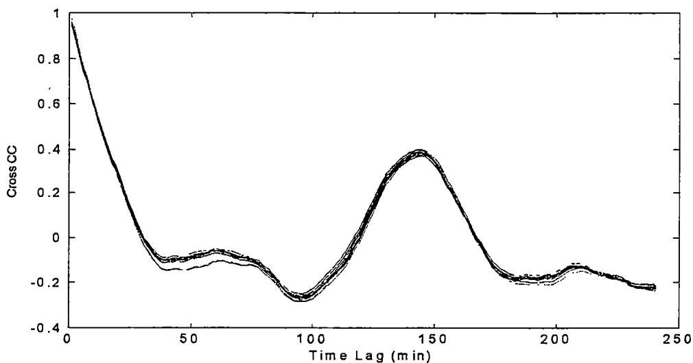
Figure 5.3 Cross correlation between Combustion Air Flow A1 and others
