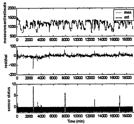
Figure C42 Corrected FW Flow #1 after replacement
