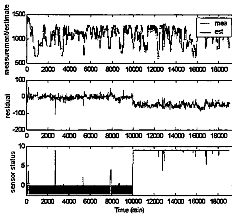
Figure C34 5% step drop on Measured Steam Flow (Klb/hr)
