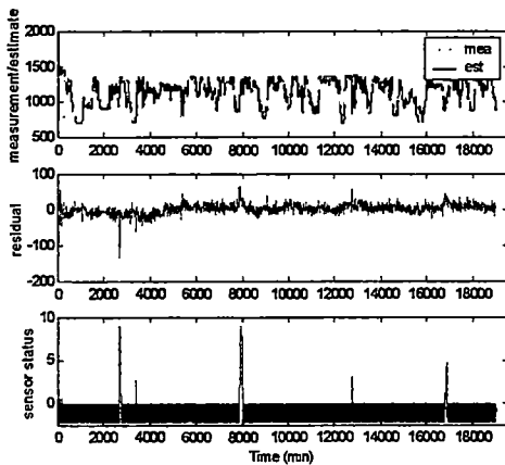
Figure C45 Recovered lost FW Flow #1
