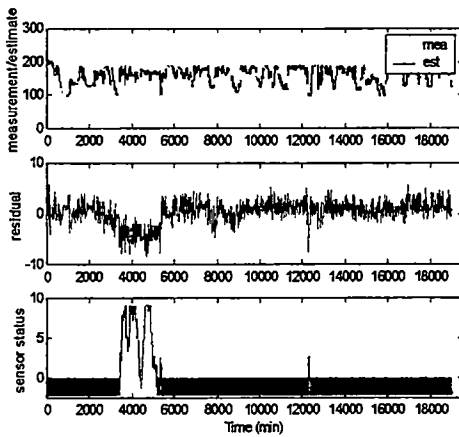
Figure C9 Prediction on Unit Gross Generation (MW)
