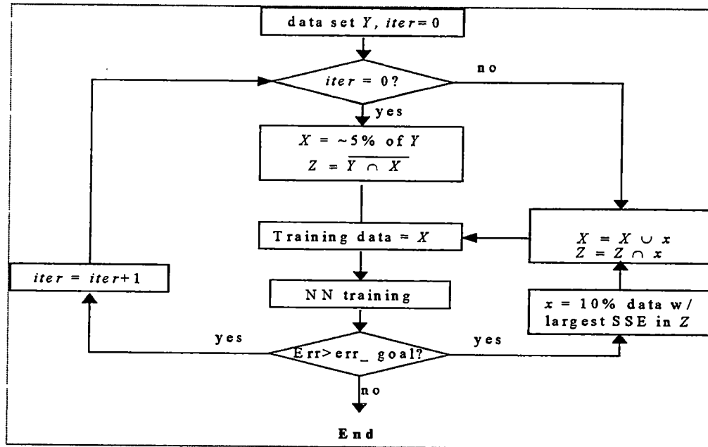
Figure 5.6 Network training paradigm
