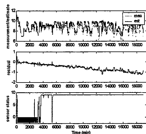
Figure C24 1%/day drift on Station Service Load (MW)
