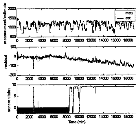
Figure C41 1%/day drift on FW Flow #1 (Klb/hr)
