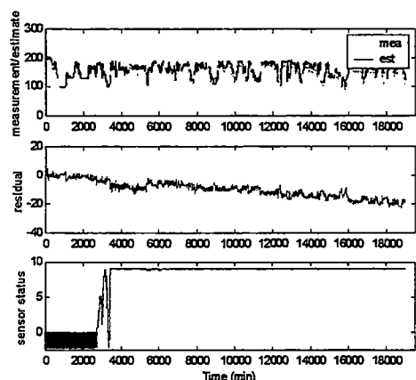
Figure C23 1%/day drift on Unit Gross Generation (MW)
