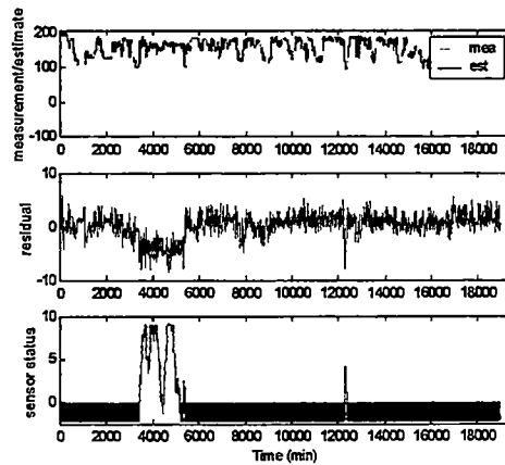
Figure C46 Predicted Unit Gross Gen. w/ recovered FW Flow #1
