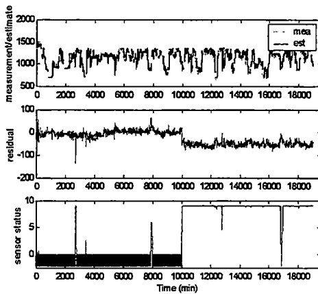
Figure C33 5% step drop on FW Flow (Klb/hr)
