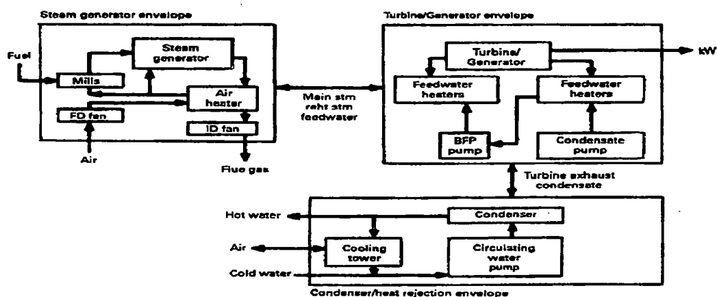
Figure 4.1 Fossil power generation system (ASME PTC PM-193)
