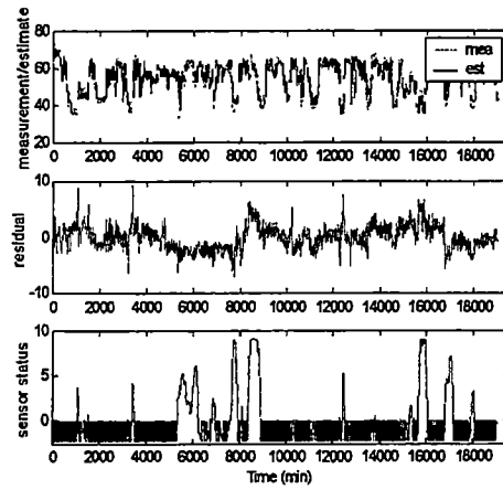
Figure C8 Prediction on Combustion Air Flow B1 (Pct)
