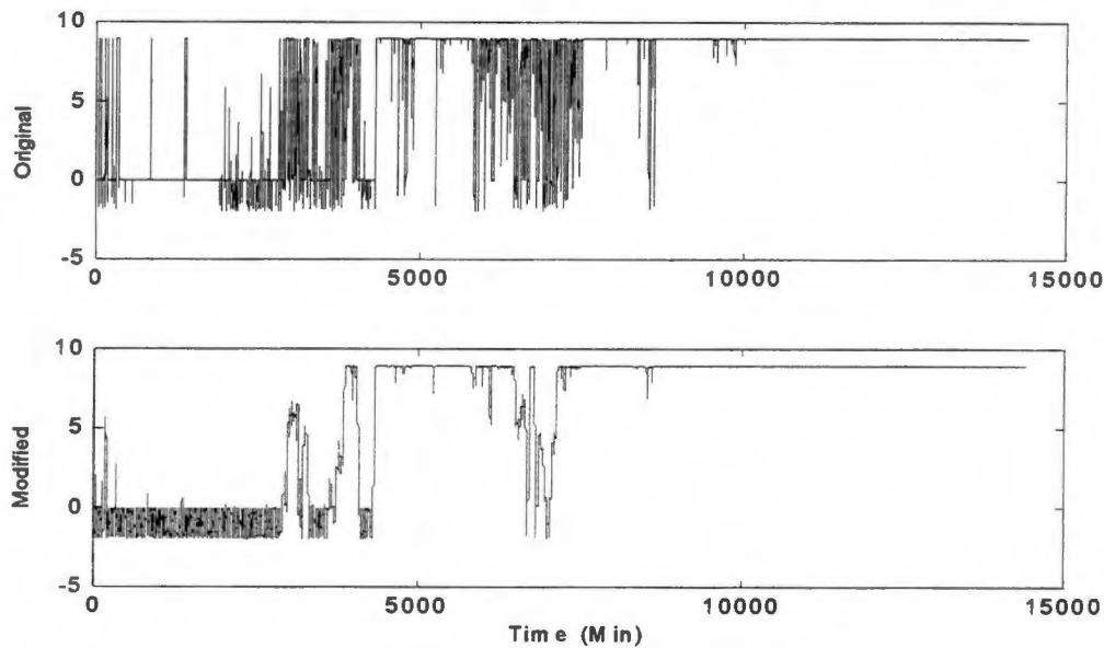
Figure 5.8 SPRT vs. MSPRT
