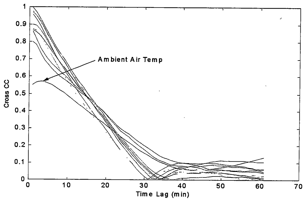
Figure 6.1 Cross correlation between Measured Steam Flow and others
