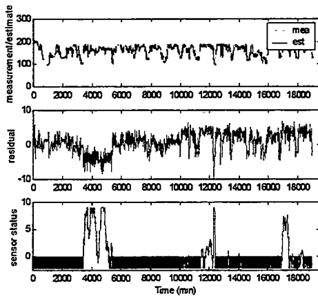
Figure C37 Predicted Unit Gross Gen. (MW) w/ bad FW Flow #1 Figure C38 Predicted lost FW Flow (Klb/hr) starting at 10000 th min.
