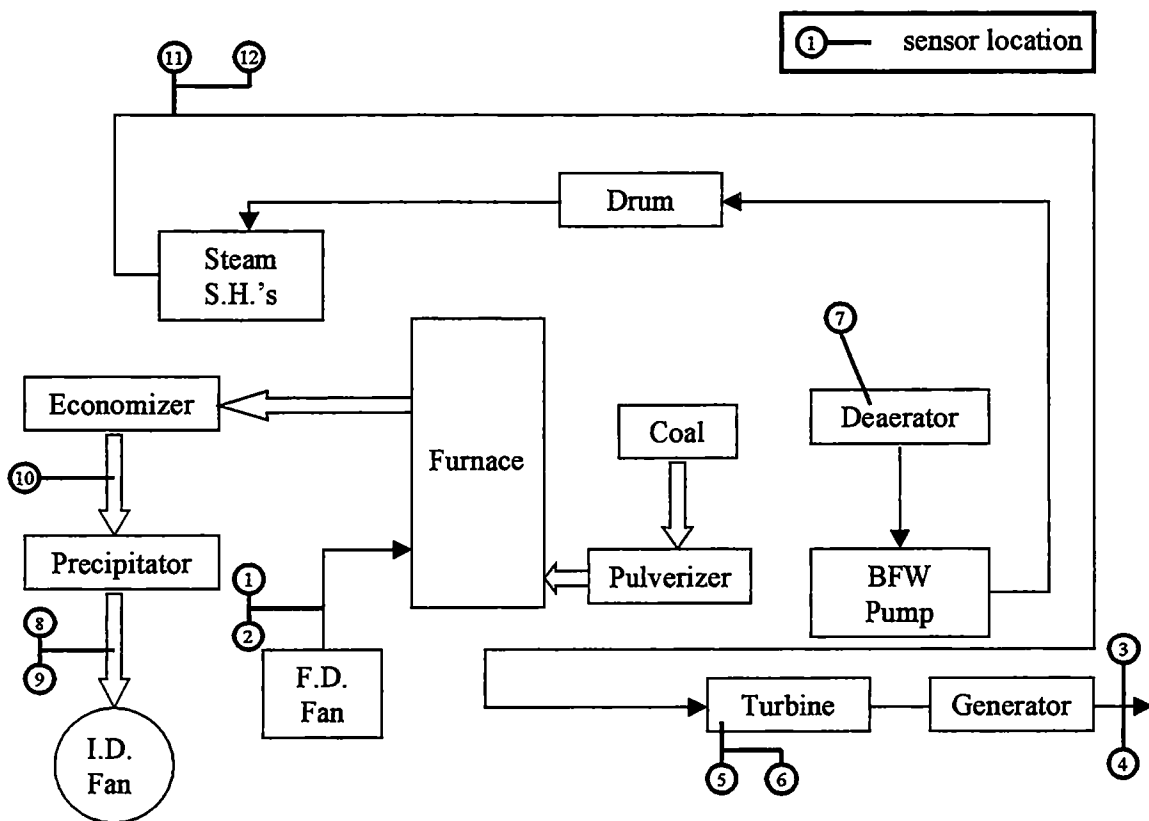
Figure 4.3 Kingston power plant Unit 9 Schematic
