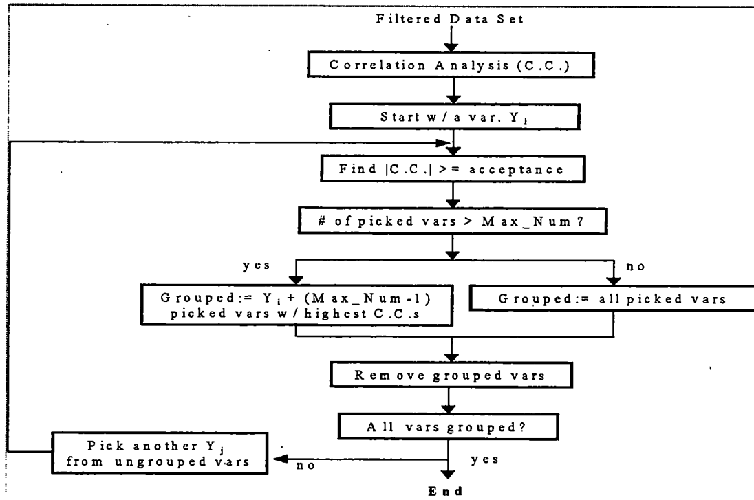
Figure 4.4 Variable exclusion algorithm
