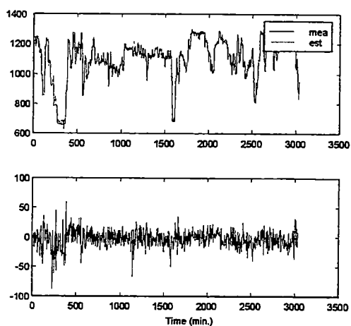
Figure B3 TDNN recall on Measured Steam Flow (Klb/hr)
