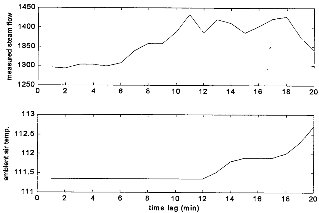
Figure 6.2 Measured Steam Flow and Ambient Air Temp. vs. time lag
