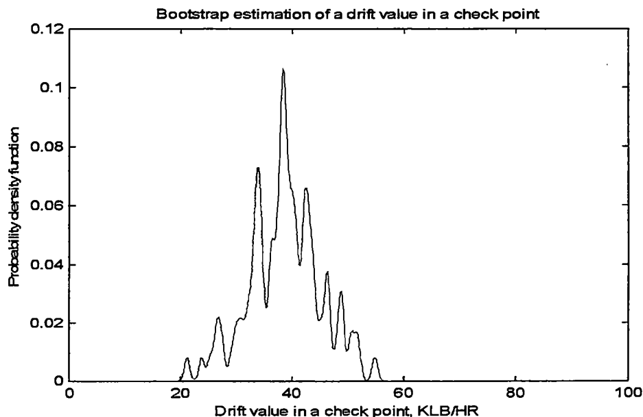
Figure 5.4 Instability of drift estimation due to perturbations (Gribok, et al. , 1999)
