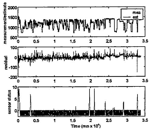
Figure C48 Predicted FW Flow (Klb/hr) after retuning
