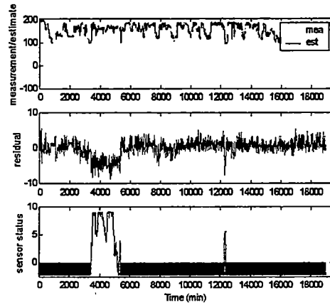
Figure C44 Predicted Unit Gross Gen. (MW) after replacement
