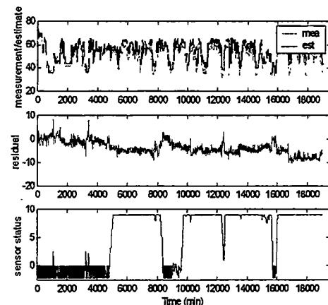
Figure C22 1% per day drift on Combustion Air Flow B1 (Klb/hr)
