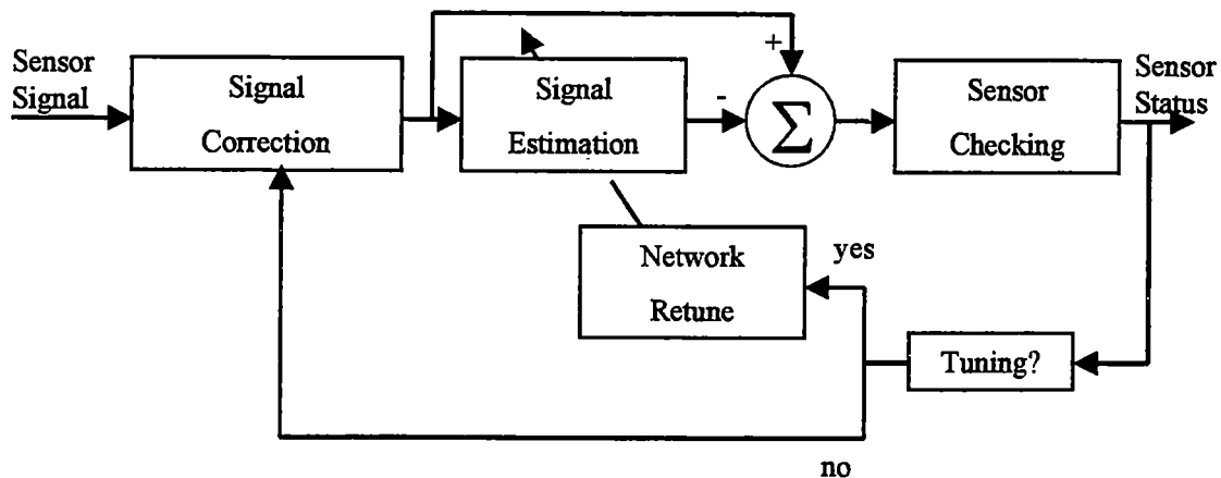
Figure 3.1 Sensor calibration system block diagram
