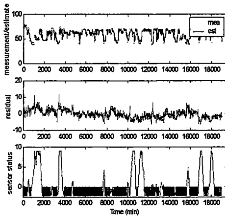
Figure C7 Prediction on Combustion Air Flow A1 (Pct)
