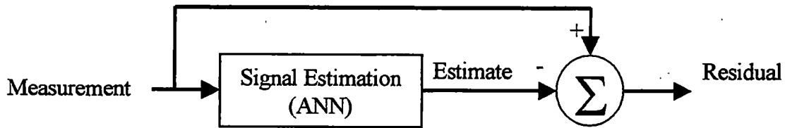
Figure 3.3 Simplified ANN signal error detection schematic
