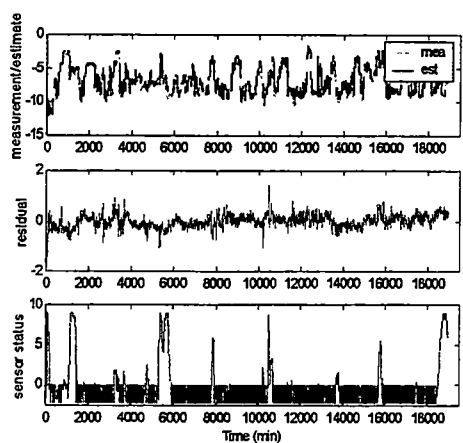
Figure C15 Prediction on ID Fan B Suction Pres. (InH2O)
