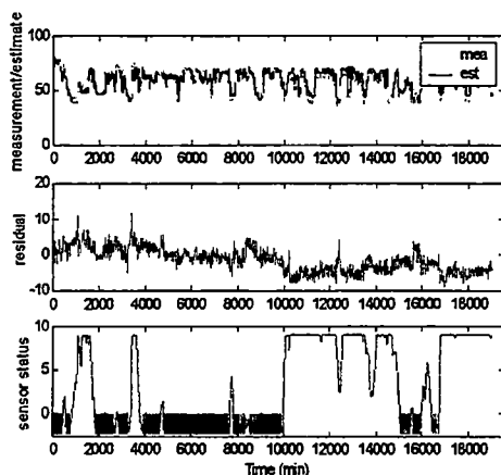
Figure C35 5% step drop on Combustion Air Flow (Pct)
