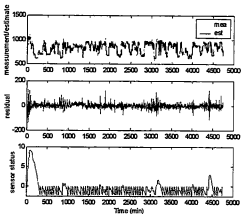
Figure C3 Recall on Hotwell Pump Discharge Flow (Klb/hr)
