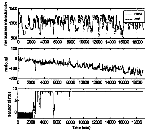
Figure C26 1%/day drift on First Stage Pressure B (psig)
