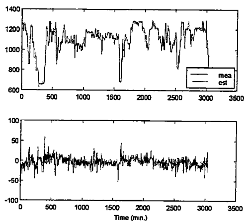
Figure B1 AANN recall on Measured Steam Flow (Klb/hr)
