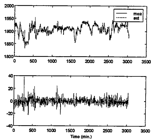
Figure B2 AANN recall on Selected Drum Pressure (psig)
