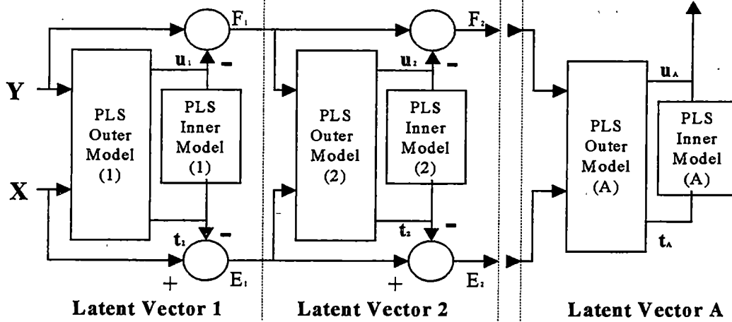
Figure 4.2 PLS model (Qin and McAvoy, 1992)
