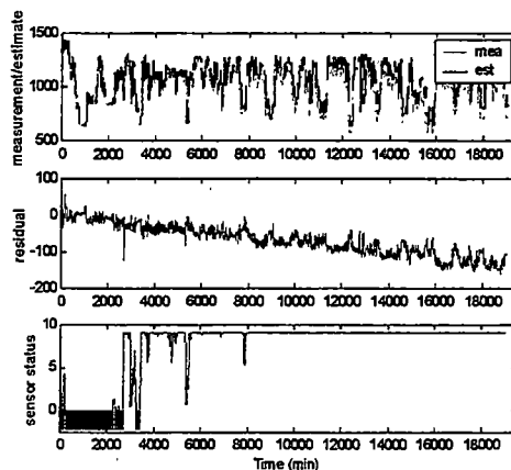
Figure C20 1%/day drift on Mea. Steam Flow (Klb/hr)
