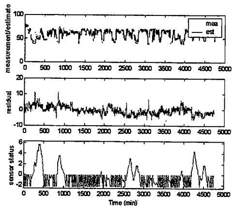
Figure C1 Recall on Combustion Air Flow (Pct)
