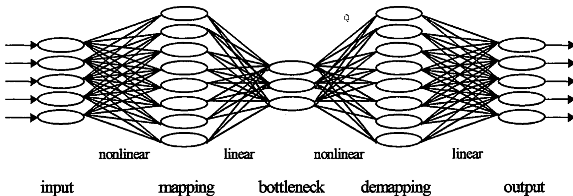
Figure 3.5 NLPCA-typed AANN structure
