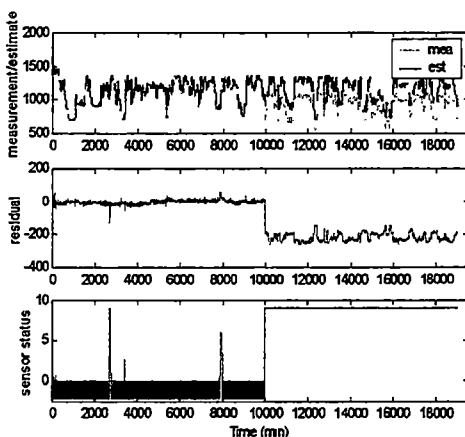
Figure C36 A 20% drop in FW Flow #1 (Klb/Hr)
