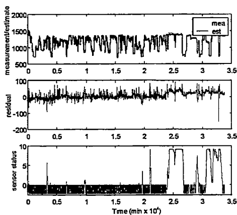
Figure C47 Predicted FW Flow (Klb/hr) before retuning
