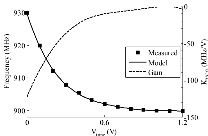
Fig. 5.2. Variation of tuning gain of the fabricated GB-LC described in Section 2.5.3.
