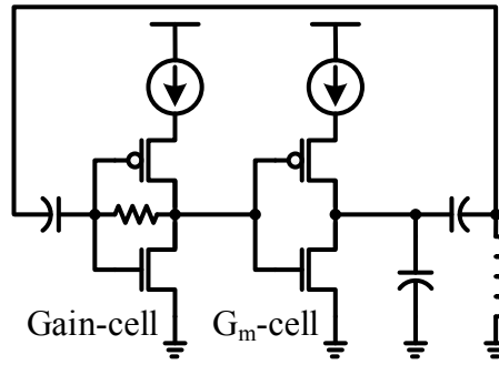
Fig. 2.8. Simplified structure of the developed GB-LC VCO topology.
