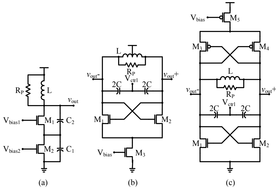
Fig. 2.2. Typical structures of (a) common-gate Colpitts oscillator, (b) cross-coupled oscillator and (c) complementary cross-coupled oscillator.
