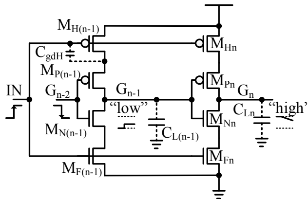
Fig. 3.8. Two stages of the ring structure of the proposed divider showing the situation where sub-threshold leakage limits the low frequency operation.
