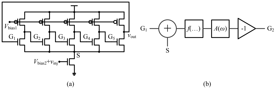
Fig. 3.4. (a) Ultra-low-power divide-by-5 ILFD reported in [49] and (b) analytical model for one stage of the ILFD.
