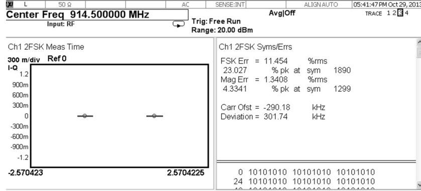
Fig. 2.20. Constellation diagram and FSK error results of the GB-LC VCO output. The oscillator is tuned to 914.5 MHz and is 2-FSK modulated with a 100 kHz, 50% square wave simulating ‘01010101’ bitstream at 200 kbps rate. RMS FSK error is about 11.5%.
