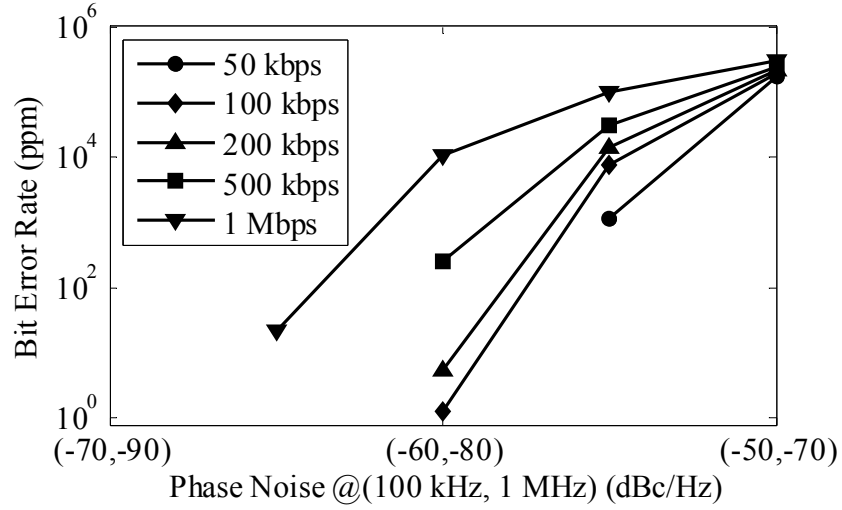
Fig. 2.6. Bit error rate (BER) of 2-FSK system with 500 kHz frequency shift for different data rates and carrier phase noise levels.
