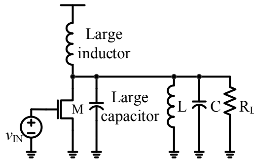
Fig. 4.1. General power amplifier model.
