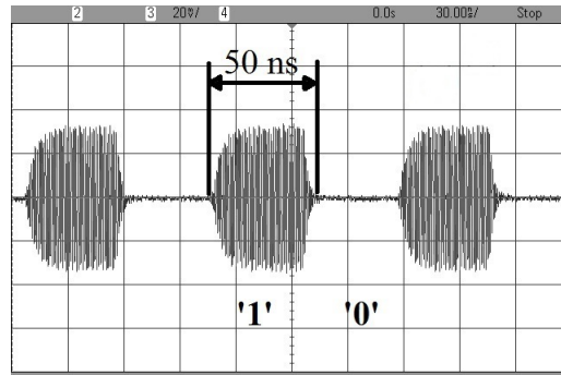
Fig. 6.14. 925 MHz carrier OOK-modulated by continuous '01010101' bitstream at 20 Mbps speed.
