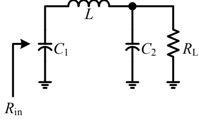
Fig. 4.5. Pi network for impedance transformation.
