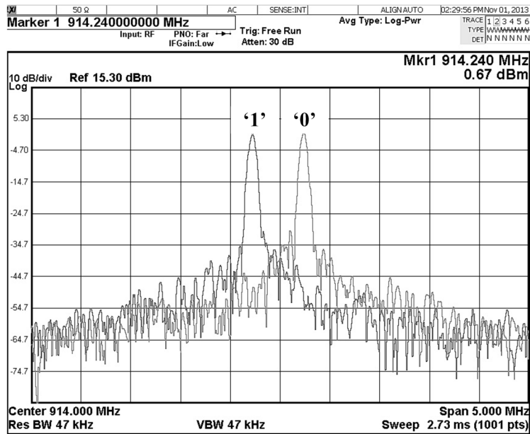
Fig. 2.18. Measured output spectra of the the BFSK GB-LC VCO showing about 550 kHz frequency shift around 914.5 MHz center frequency.
