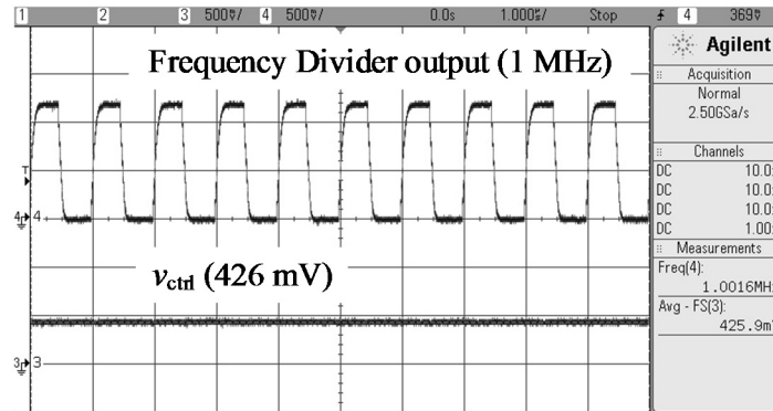
Fig. 6.4. VCO signal divided down to 1 MHz and CP-LF generated control voltage.
