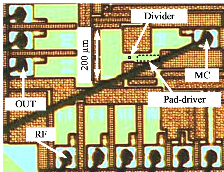
Fig. 3.10. Microphotograph of the fabricated dual-modulus divider.
