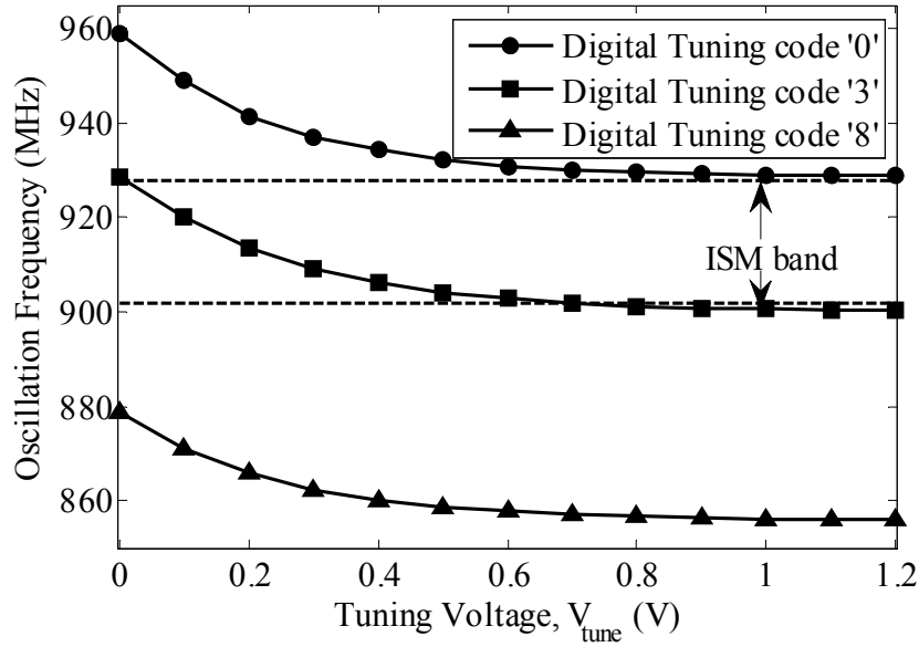
Fig. 2.21. Tuning range of the GB-LC VCO. The digital tuning system has a range of 80 MHz which is sufficient to cover for process variations and the analog tuning range varies from 22.5 MHz to 30.2 MHz, corresponding to digital tuning code ‘0’ to code ‘8’.
