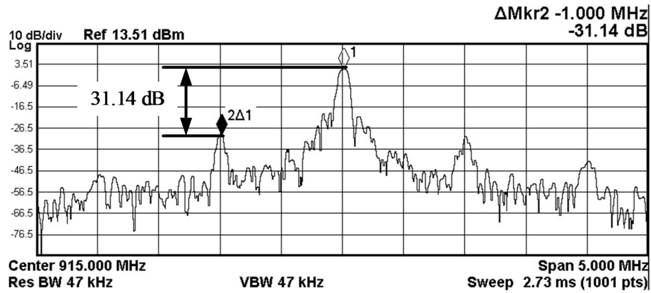
Fig. 6.3. Spectrum of unmodulated 915 MHz carrier generated by the PLL.
