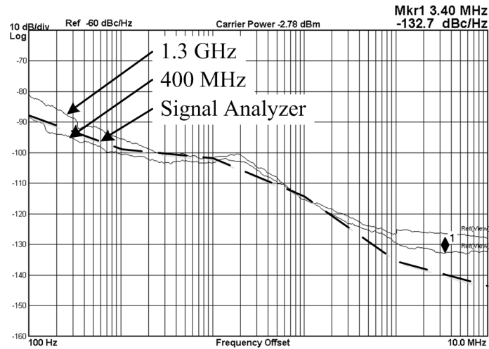
Fig. 3.12. Phase noise spectra of divider output in \div 4 mode, locked by 1.3 GHz and 400 MHz input frequencies. The dashed curve shows the base phase noise of the signal analyzer.
