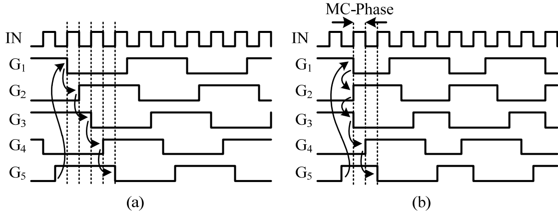
Fig. 3.7. (a) Divide-by-5 and (b) divide-by-4 operations of the designed divider. The arrows indicate propagated transitions controlled by input signal.
