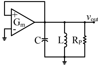
Fig. 2.1. Typical structure of an LC oscillator.
