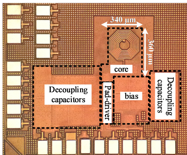
Fig. 2.17. Microphotograph of the fabricated GB-LC VCO in a bare die. The core occupies 360 \times 340 \mu\text{m}^2 chip area. The bias circuit occupies 245 \times 345 \mu\text{m}^2 chip area.
