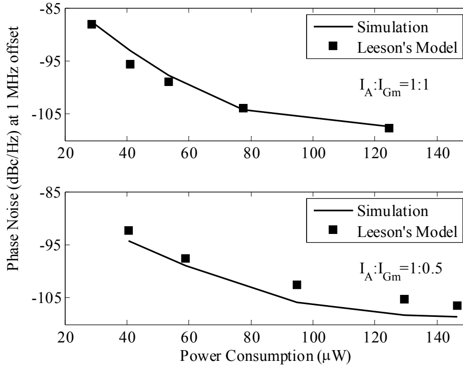
Fig. 2.16. Simulated (pre-layout) phase noise of the proposed GB-LC VCO at different power consumptions. Phase noise can be predicted using Leeson's model with F=5 . Two different structures of the VCO are simulated – one where the ratios of device sizes and bias currents between the A-cell and the Gm-cell are both 1:1 and another where the ratios are both 1:0.5.
