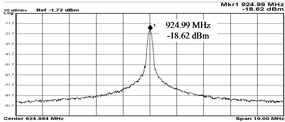
Fig. 6.10. Spectrum of unmodulated 925 MHz carrier signal, with PA at maximum output power, -18.6 dBm.
