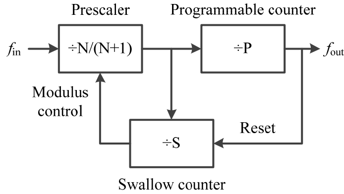
Fig. 3.1. Topology of the commonly used Pulse Swallow frequency divider [39].
