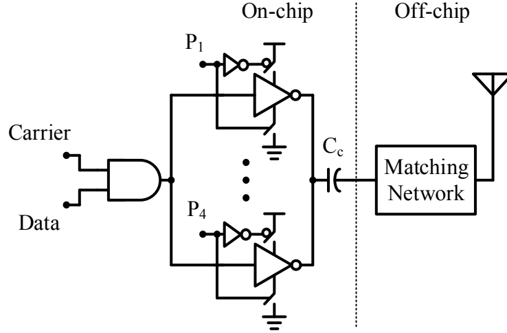
Fig. 4.4. Schematic of low-power power amplifier with OOK modulation, used in this work.
