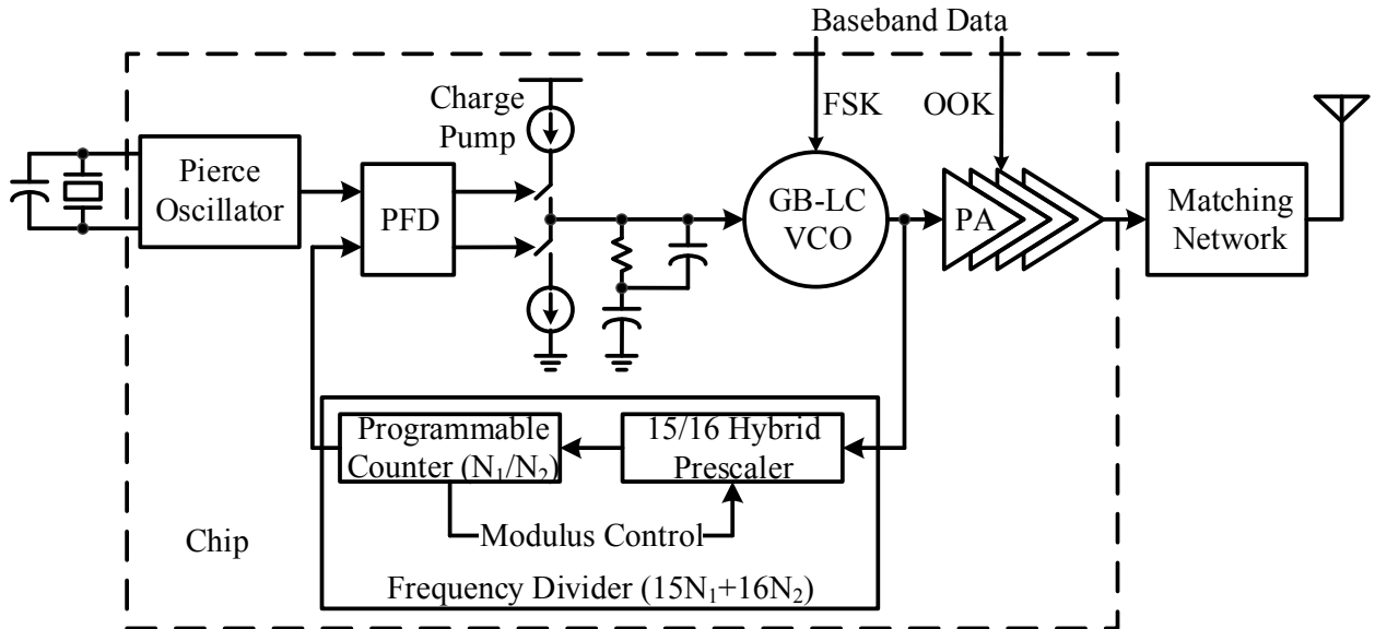
Fig. 5.1. Topology of the proposed low-power 915 MHz transmitter.
