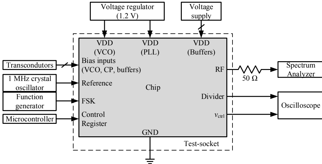
Fig. 6.2. Test setup for the 3 rd order PLL in the first phase.
