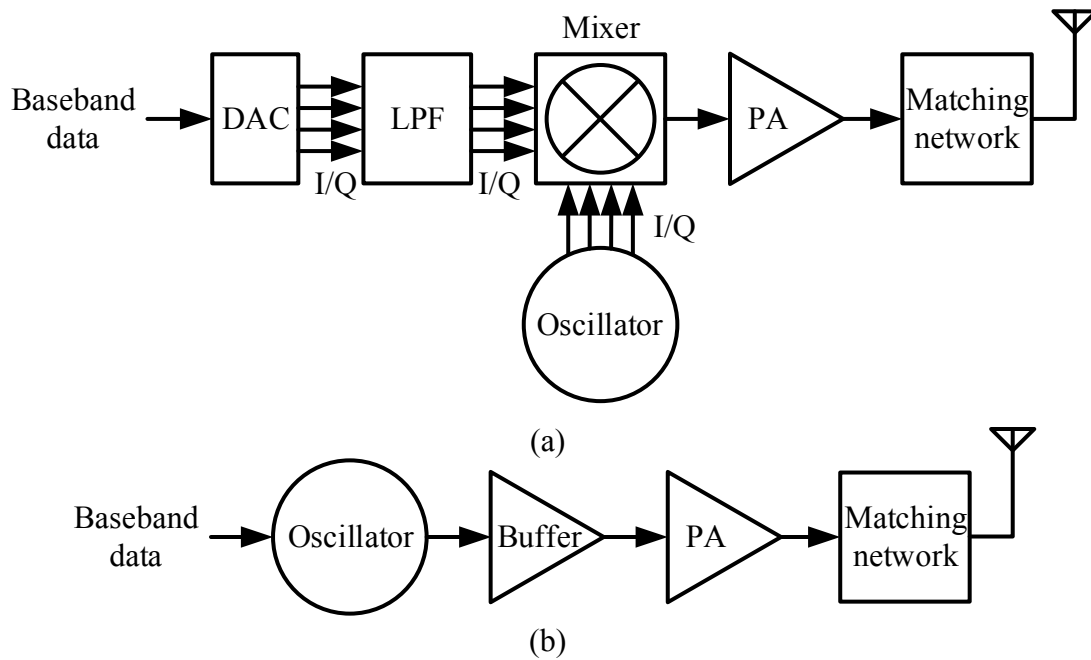
Fig. 1.2. Typical (a) direct-conversion and (b) direct-modulation transmitter structures.
