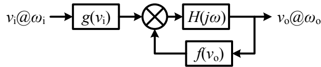
Fig. 3.3. Miller-type model for injection-locked frequency divider [45].
