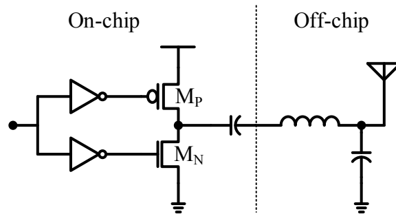
Fig. 4.3. A voltage-mode Class D power amplifier [68].
