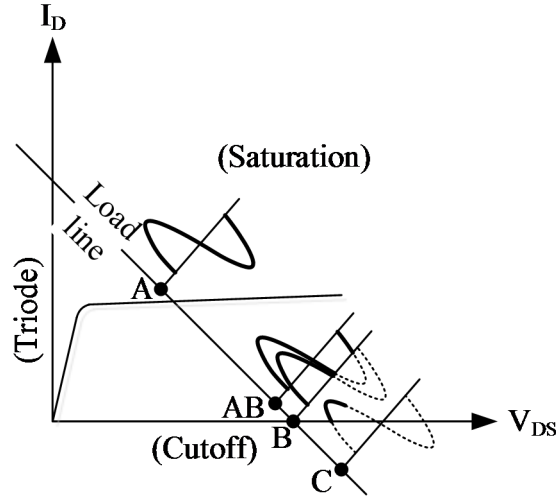
Fig. 4.2. Bias points of Class A, AB, B and C power amplifiers.
