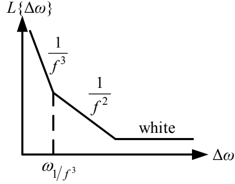
Fig. 2.4. Typical plot of the phase noise of an oscillator versus frequency offset from carrier.
