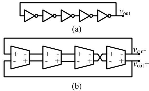
Fig. 2.3. Typical structures of (a) five-stage single-ended ring oscillator and (b) four-stage differential ring oscillator.
