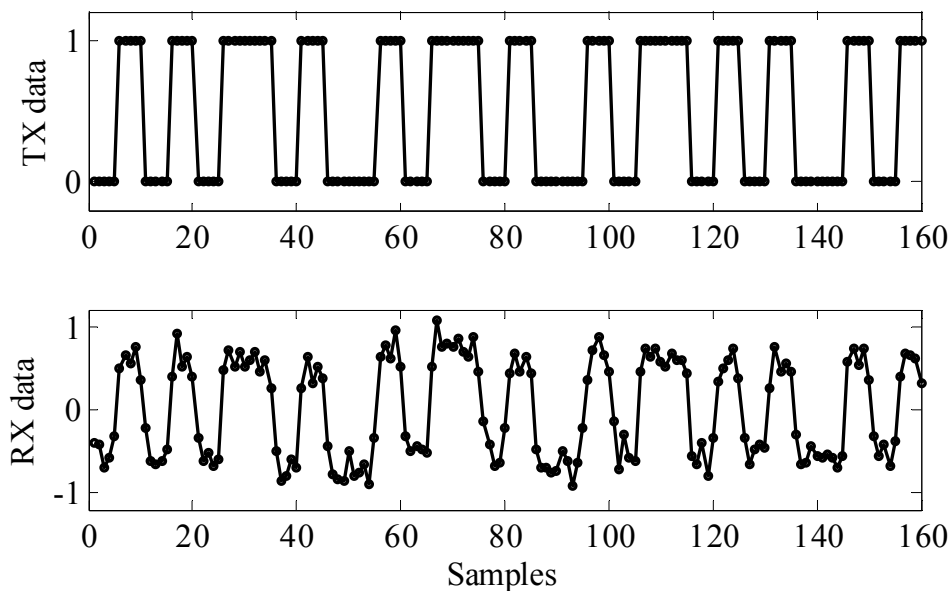
Fig. 6.13. Two bytes from a pseudo-random data (Manchester encoded) set transmitted and received at 400 kbps speed through FSK modulation system. Data is sampled at 4 MHz by the receiver.
