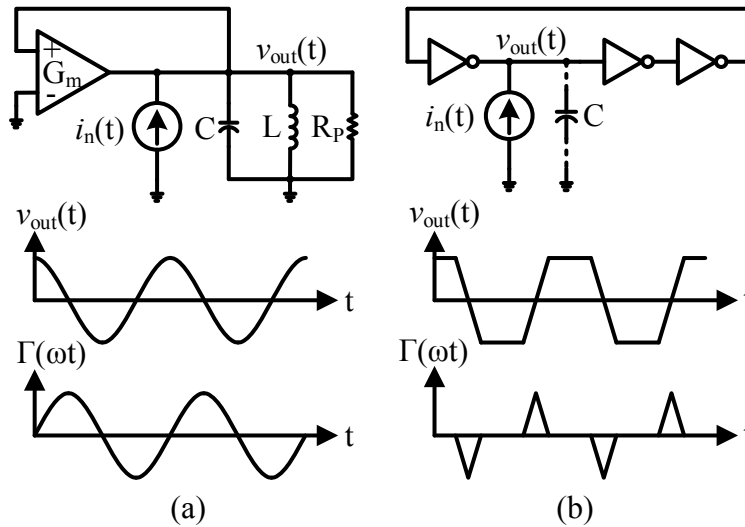
Fig. 2.5. Typical structures with noise-current injection source, i_n(t) , shown at a node, waveforms and impulse sensitivity functions of (a) an LC oscillator and (b) a ring oscillator [19].
