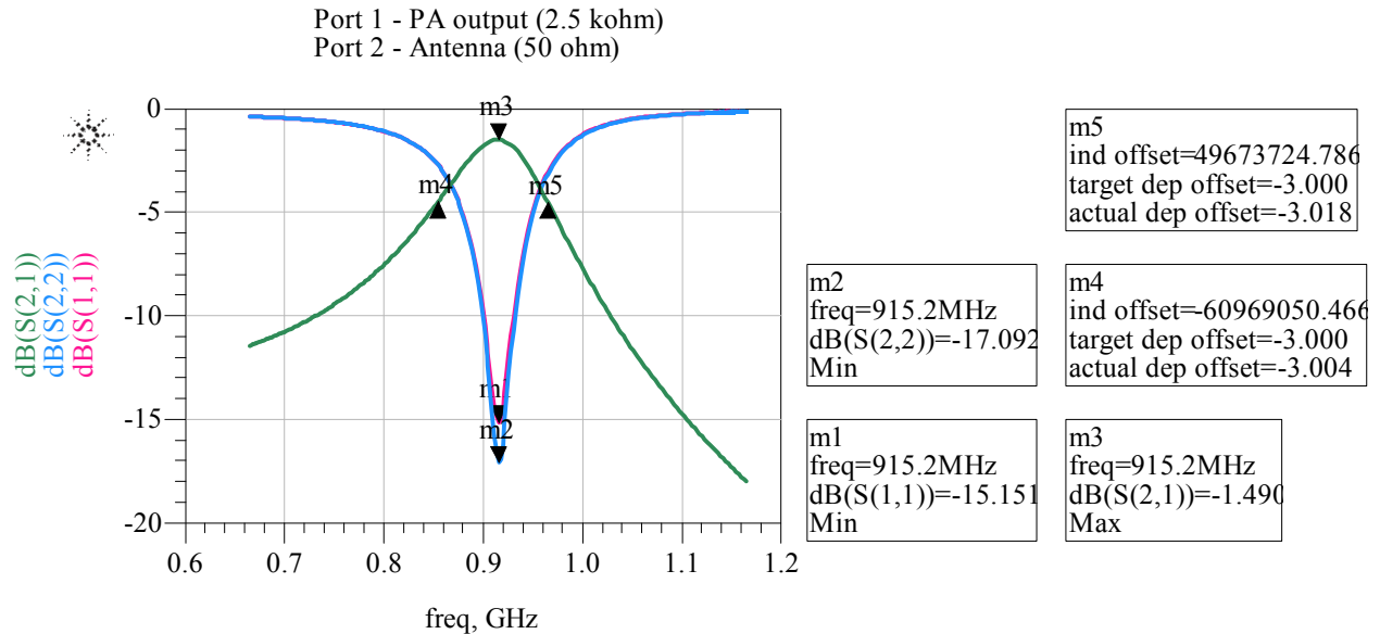
Fig. 4.7. Impedance transformation simulation with non-idealities, including short PCB trace between PA output and off-chip matching network using ADS.
