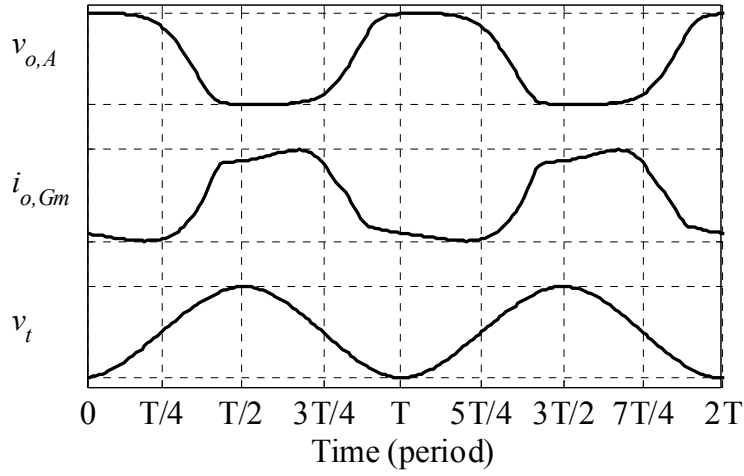
Fig. 2.15. Normalized waveforms of the GB-LC oscillator in post-layout simulation.
