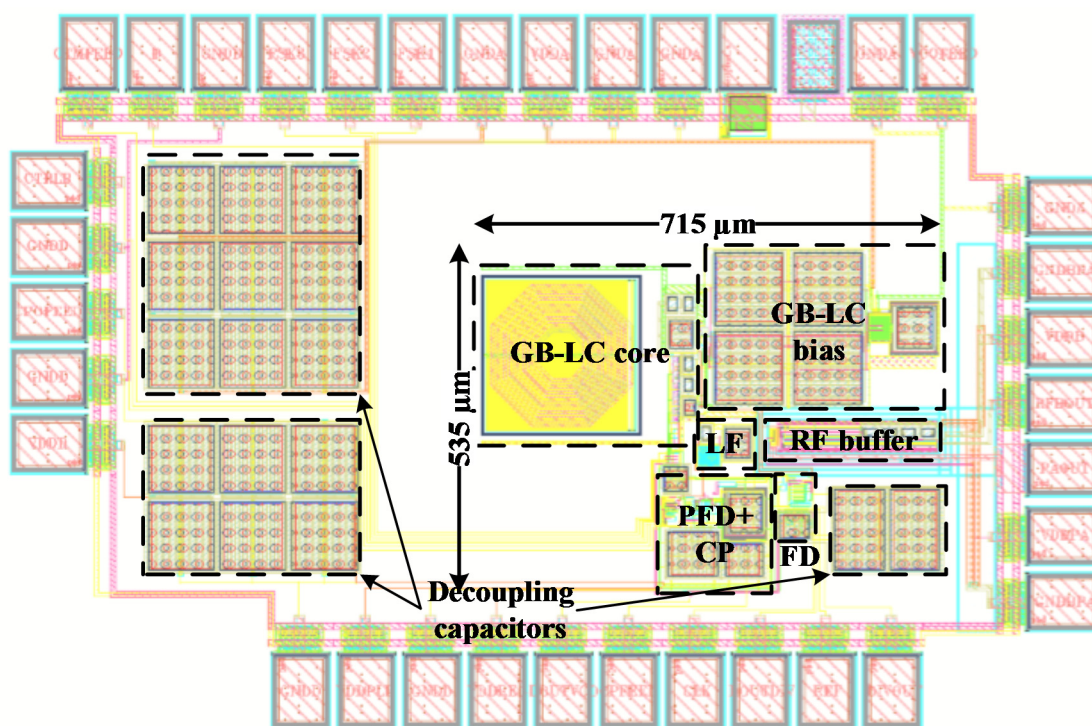
Fig. 6.1. Layout of the 3 rd order PLL in the first phase of proposed transmitter implementation.
