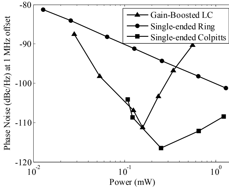
Fig. 2.9. Simulated phase noise of 1 GHz signals, at 1 MHz offset from generalized structures of a single-ended, 5-stage ring oscillator, a single-ended Colpitts oscillator and a GB-LC oscillator for different core power consumptions from 1.2 V supply.
