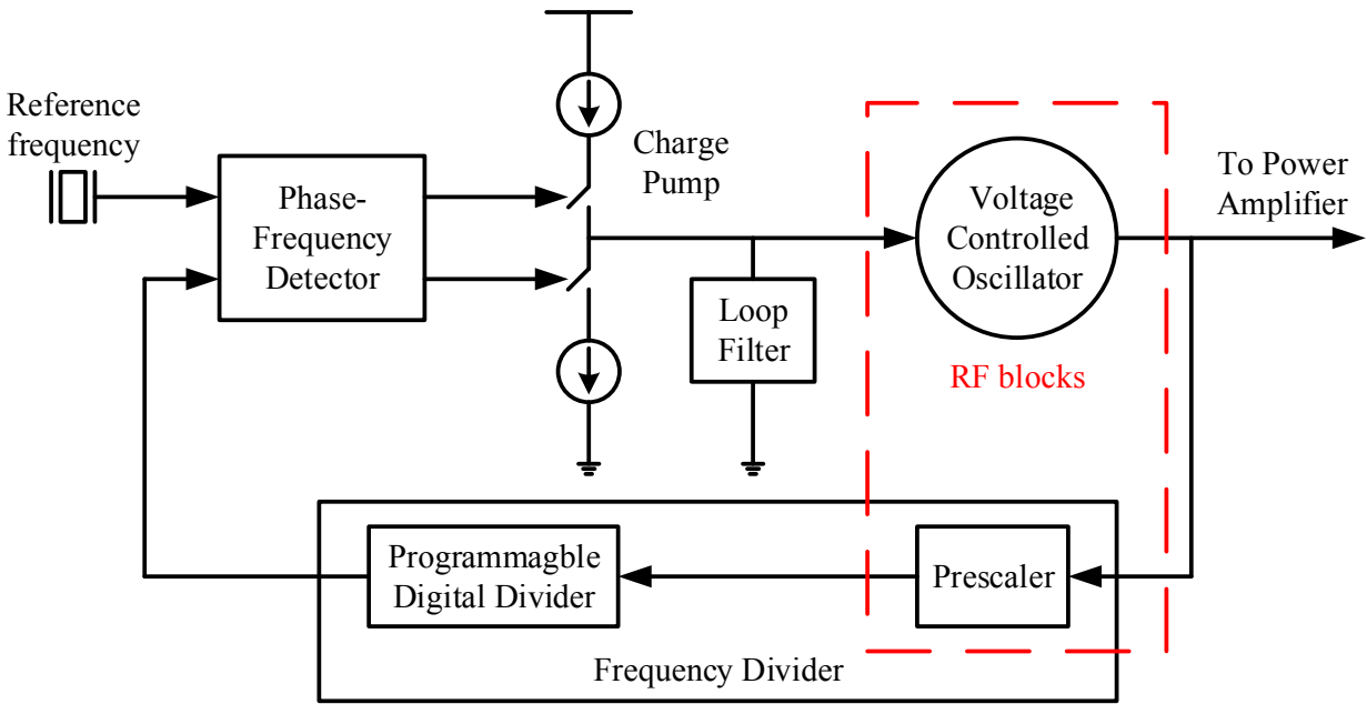
Fig. 1.3. The structure of a typical PLL.
