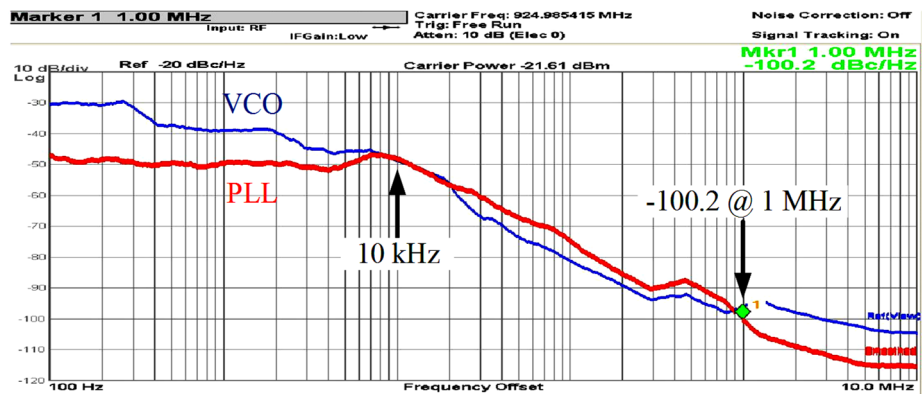
Fig. 6.11. Overlaid phase noise spectra of the PLL and the free-running VCO. Phase noise of PLL is -100.2 dBc/Hz at 1 MHz offset.
