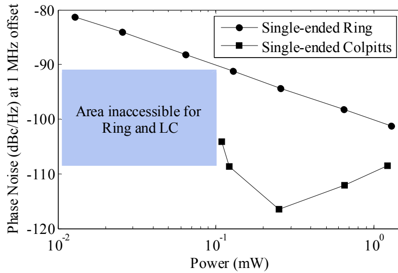
Fig. 2.7. Simulated phase noise of 1 GHz signals, at 1 MHz offset from generalized structures of a single-ended, 5-stage ring oscillator and a single-ended Colpitts oscillator for different core power consumptions from 1.2 V supply.
