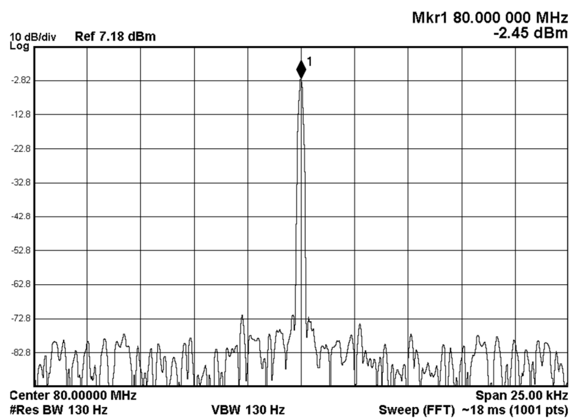
Fig. 3.11. Output spectrum of the divider at \div 5 mode locked by 400 MHz input frequency.
