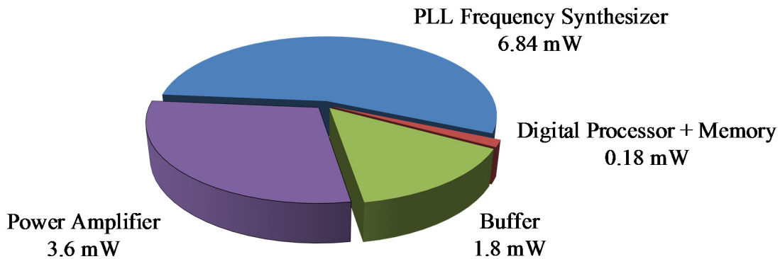
Fig. 1.1. Power distribution in the 2.4 GHz PLL-based transmitter reported in [6].
