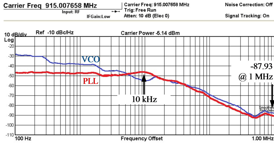
Fig. 6.5. Overlaid phase noise spectra of the VCO and PLL. This shows 10 kHz PLL bandwidth and unsuppressed phase noise of -87.93 dBc/Hz at 1 MHz offset.
