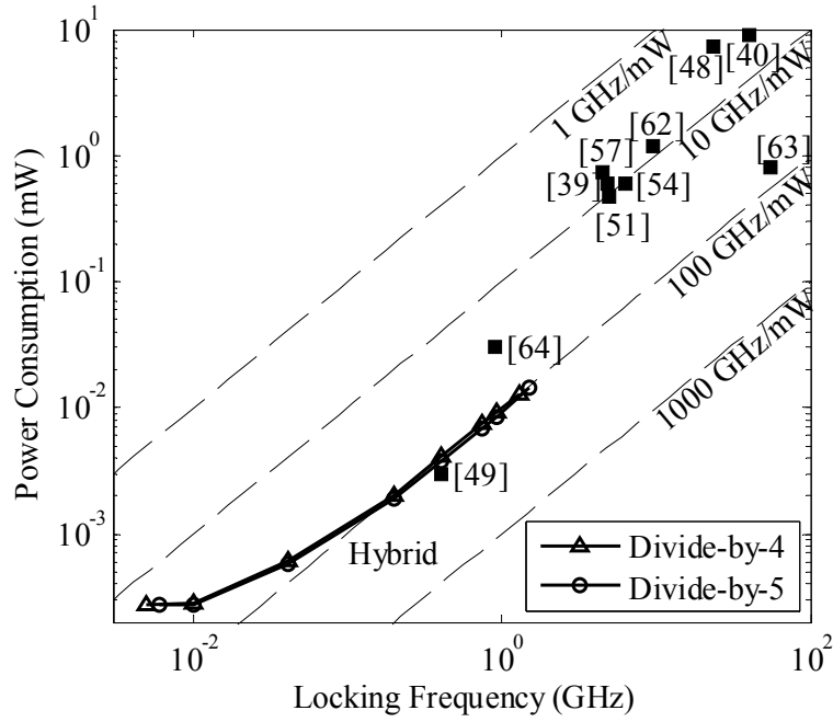
Fig. 3.13. Power consumption of the dual-modulus hybrid divider across locking range and a comparative overview with the state-of-the-art.
