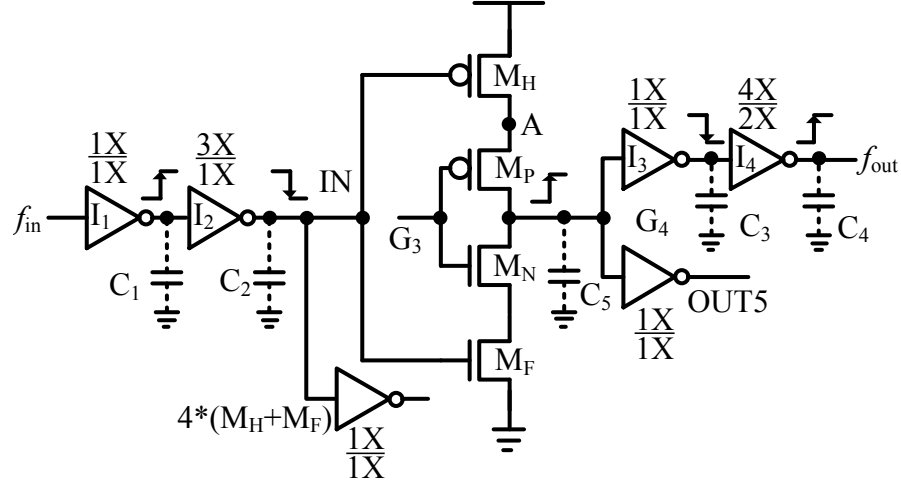
Fig. 3.9. Critical portion of divider for maximum locking frequency and phase noise estimation.
