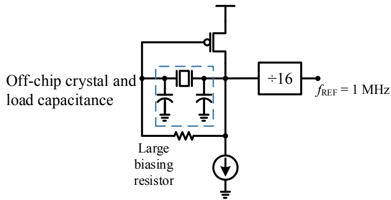
Fig. 5.8. Schematic of Pierce crystal oscillator for generating reference frequency for PLL.
