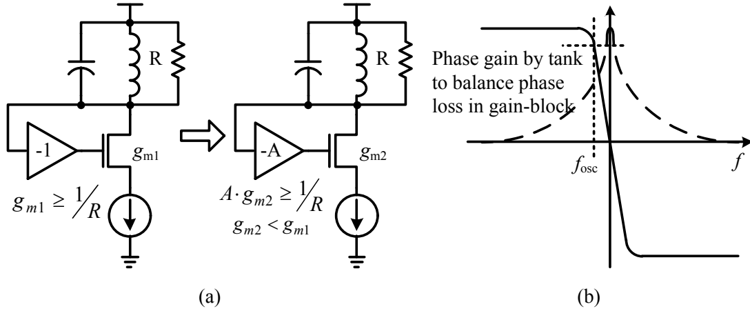
Fig. 2.11. (a) Derivation of core structure of the proposed VCO and (b) frequency of oscillation.
