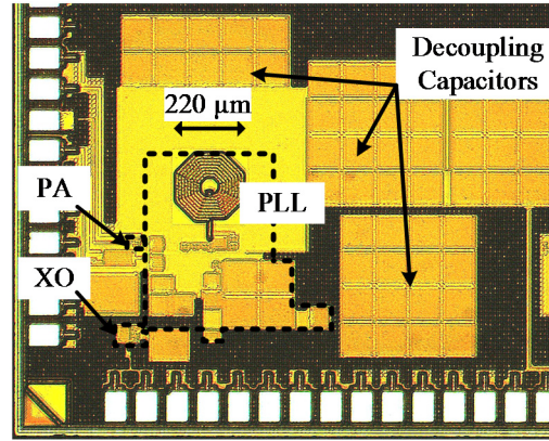
Fig. 6.7. Microphotograph of the transmitter die.
