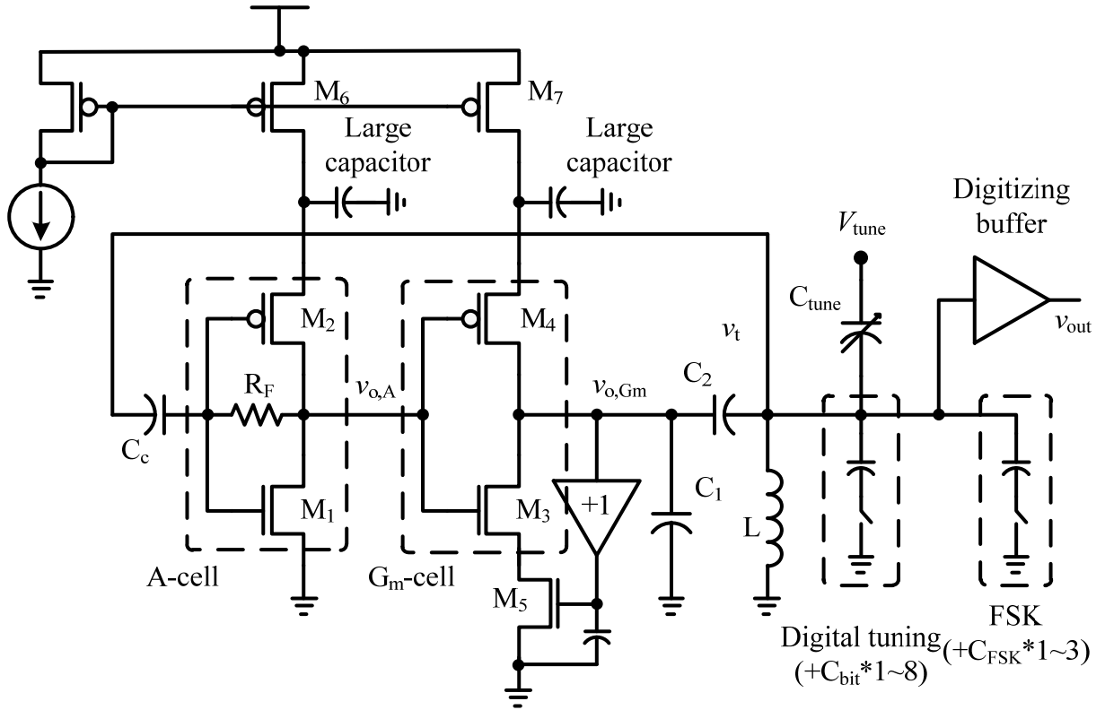
Fig. 2.12. Detailed schematic of the gain-booster LC VCO.
