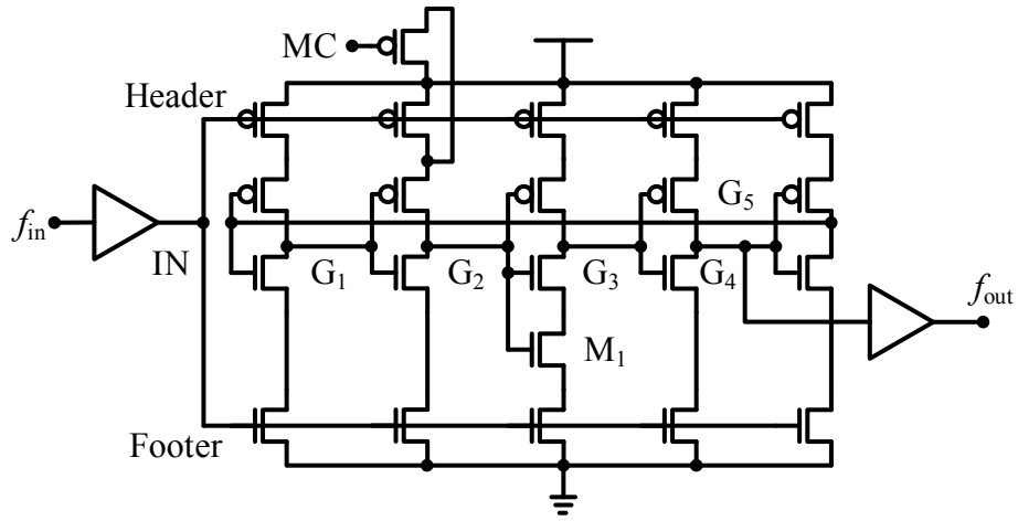
Fig. 3.6. Topology of the divide-by-4/5 hybrid frequency divider for this work.
