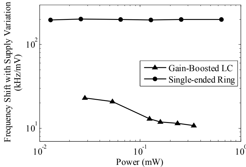
Fig. 2.10. Simulated supply sensitivity of generalized structures of a single-ended, 5-stage ring oscillator and a GB-LC oscillator, running at 1 GHz, using a 1.2 V supply.
