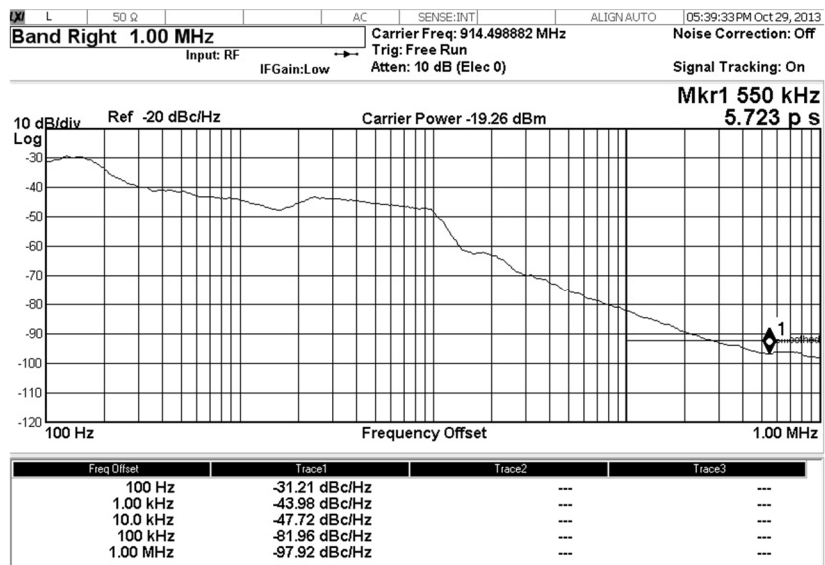
Fig. 2.19. Phase noise spectrum of the GB-LC VCO output at 914.5 MHz. Phase noise is -97.9 dBc/Hz at 1 MHz offset.
