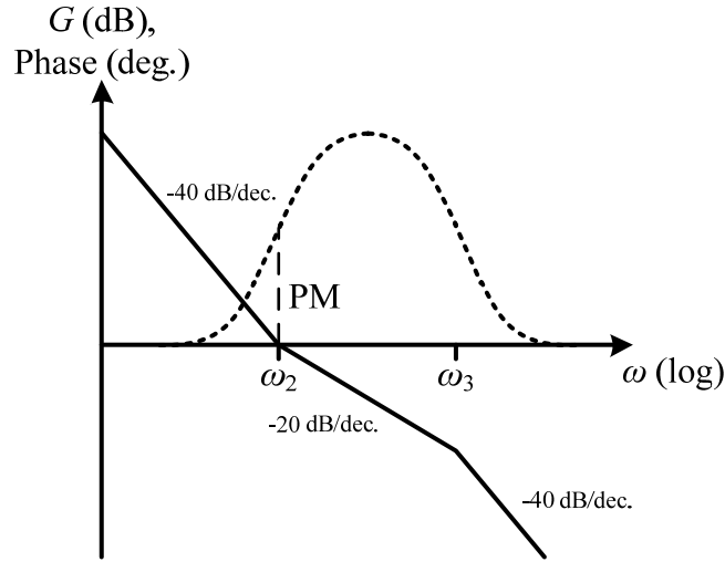
Fig. 5.3. Bode plot of open-loop gain of the 3 rd order PLL in Fig. 5.1.
