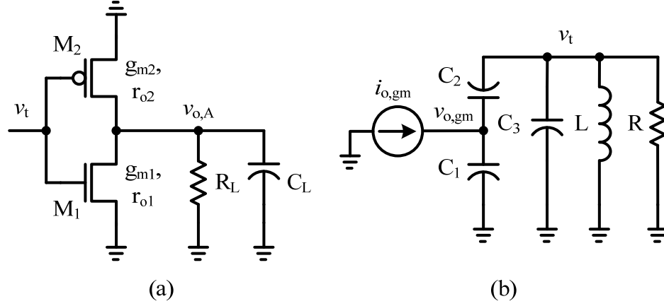
Fig. 2.13. AC equivalent circuits of the A-cell (a) and LC tank (b) for estimating oscillating frequency with phase-balance equation.
