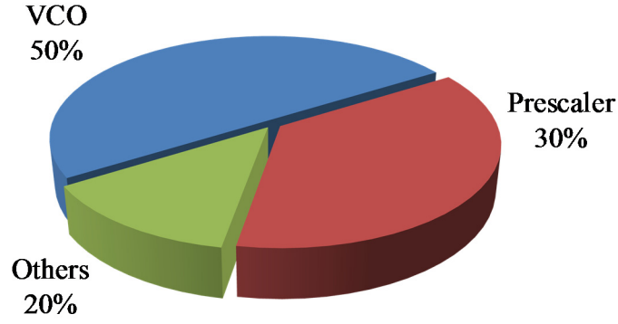
Fig. 1.4. Power budget of the blocks in a PLL [17].
