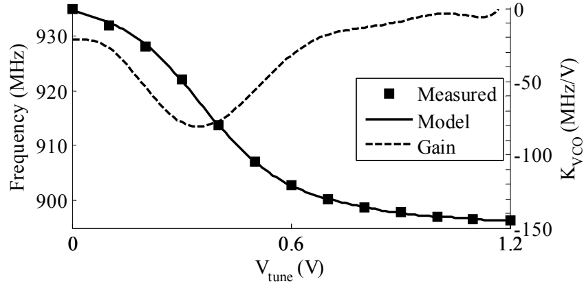
Fig. 5.7. Reduced K_{VCO} variation due to new placement of the tuning capacitor.
