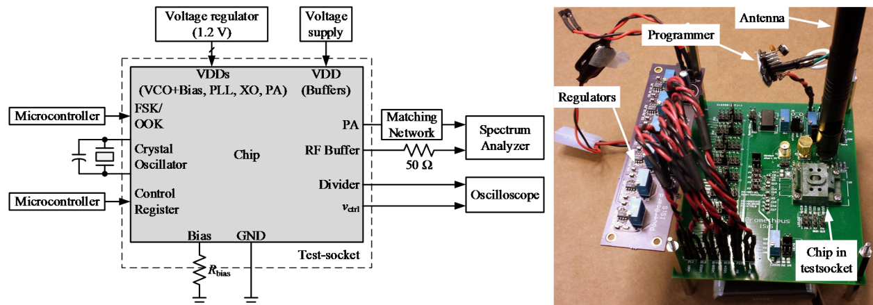
Fig. 6.8. Test setup for the transmitter.
