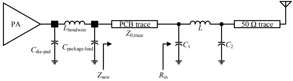
Fig. 4.6. PA output matching network with non-idealities.
