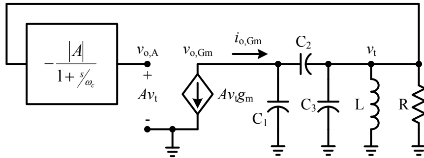
Fig. 2.14. Small-signal equivalent circuit of the GB-LC oscillator core.
