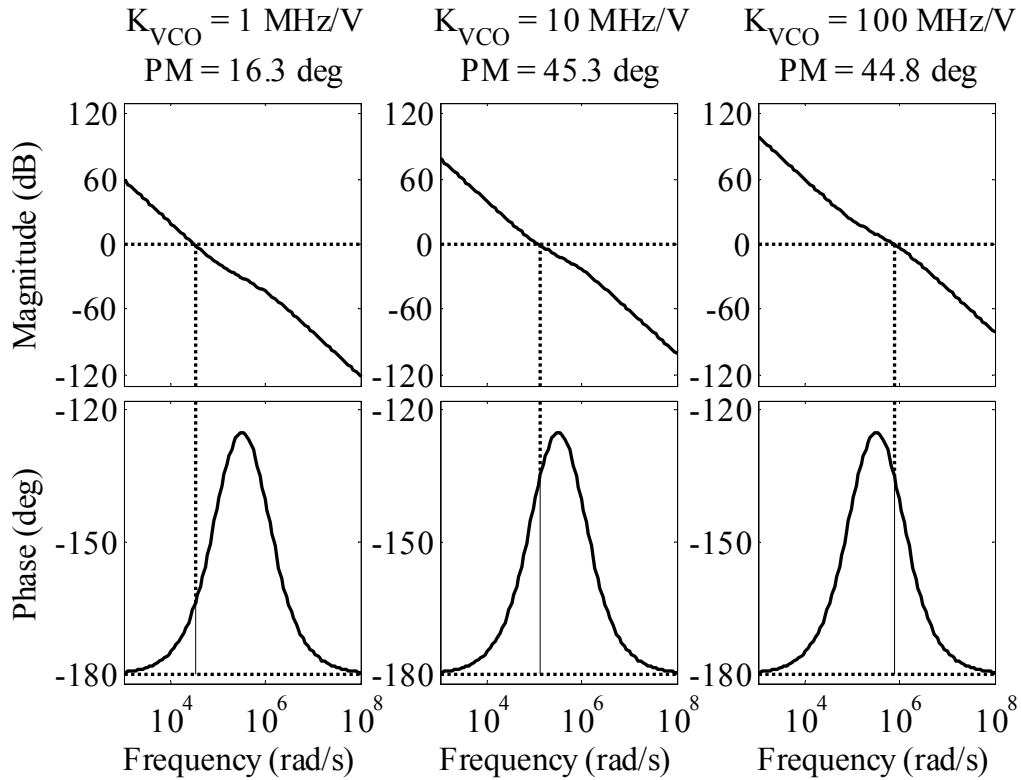
Fig. 5.4. Variation in phase margin of PLL due to variation of VCO gain.
