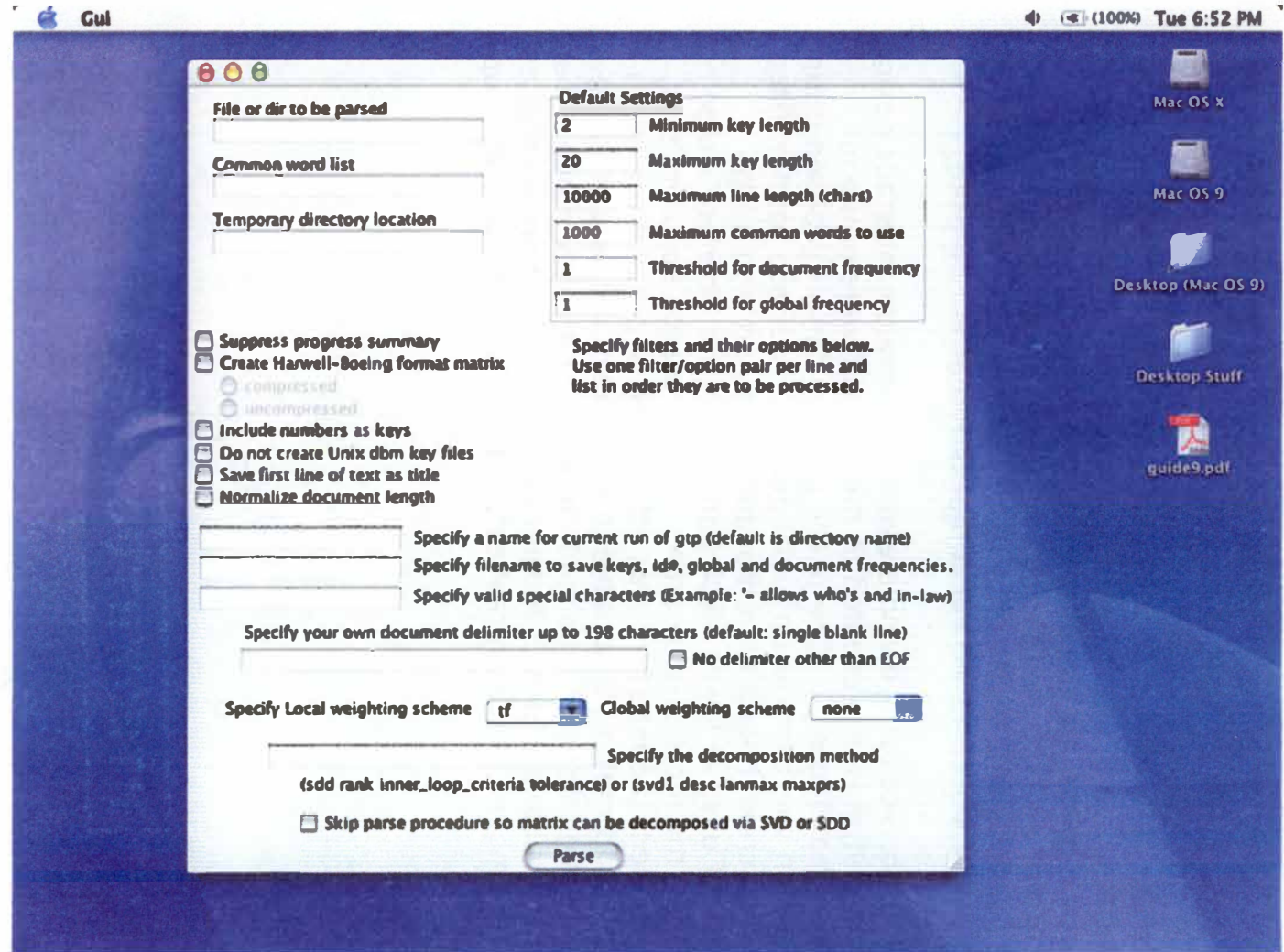
Figure 2. Single expanded window interface
