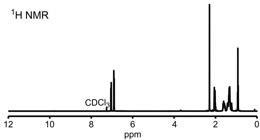
Figure 4.2. ^1\text{H} NMR of 2-octyl-1-(p-tolyl)aziridine in CDCl 3 .
