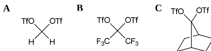
Figure 2.3. (A) Desmarteau's methyl ditriflate, (B) Sterlin's 2,2-ditriflato-perfluoro propane, and (C) Martinez's 7,7'-ditriflato-norbonane.
