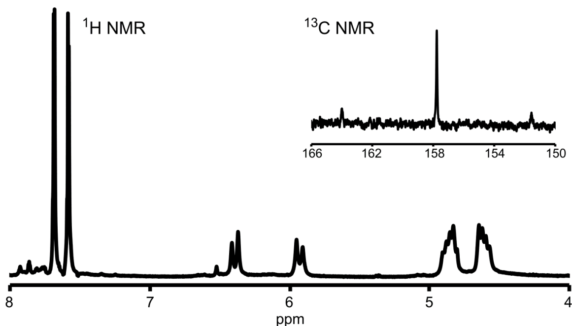
Figure 1.5. ^1\text{H} NMR of [(^{\text{Me,Et}}\text{TC}^{\text{H}})\text{Pt}](\text{OTf})_2 in \text{DMSO-d}_6 , exhibiting geminal AB splitting of the methylene and the ethylene positions, suggesting the rigidity of the complex in solution. The inset is a highlight of the ^{13}\text{C} NMR carbene peak featuring platinum satellites with a ^{195}\text{Pt} -C coupling constant of 942 Hz.
