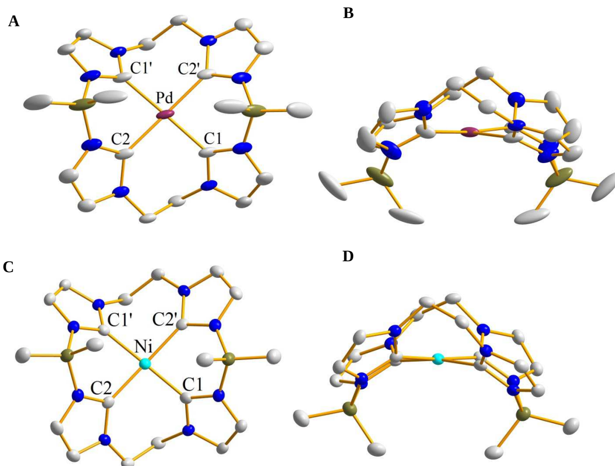
Figure 3.2. Crystal structures of (A) 3 top-down view, (B) 3 side-on view, (C) 4 top-down view, and (D) 4 side-on view. Plum, teal, blue, gray, and olive ellipsoids (50% probability) represent Pd, Ni, N, C, and B respectively. Hydrogens have been omitted for clarity.
