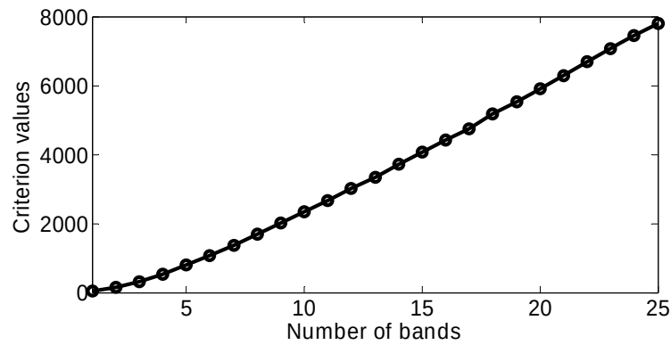
Figure 6.24. Criterion values calculated by ICOMP for different number of bands ranging from 1 to 25 and the top one band (610) with the minimal value.
