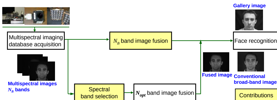
Figure 1.4. Pipeline of the dissertation work.
