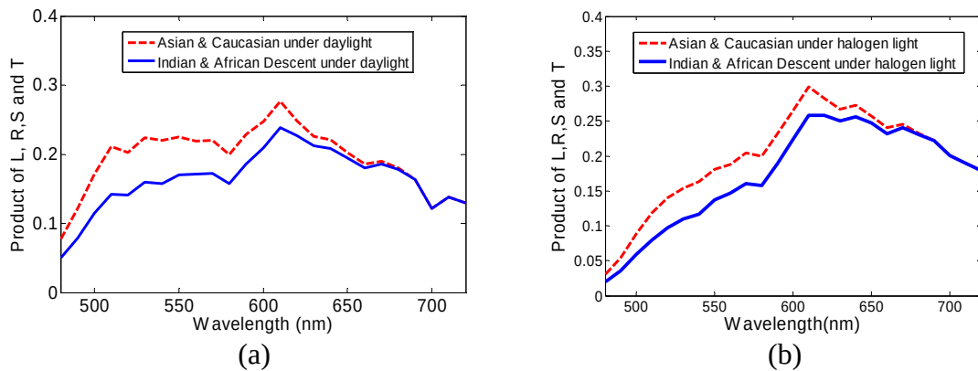
Figure 4.5. The combined spectral behavior of the four factors, spectral response of the camera, transmittance of the LCTF, skin reflectance, and spectral distribution under (a) daylight, and (b) halogen light.
