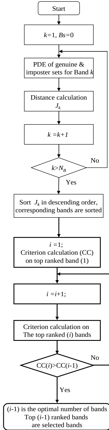
Figure 6.3. Flow-chart of the complexity-guided distance-based band selection algorithm.
