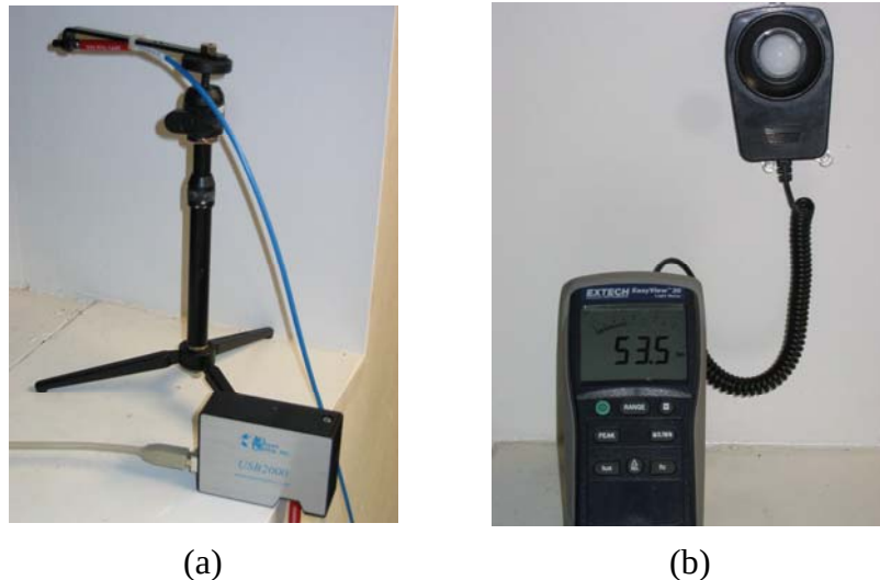
Figure 3.3. Spectrometer and light meter used in our image acquisition, (a) Ocean Optics USB2000 Spectrometer and (b) EasyView30 light meter.
