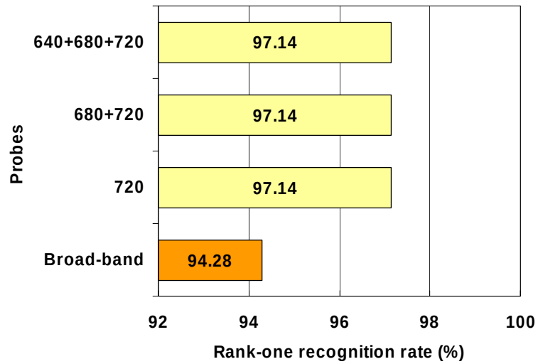
Figure 6.31. Rank-one recognition rates of various probes, including broad-band monochromatic image, narrow-band images of 720nm and fused images from bands (680 720) and (640, 680, 720).
