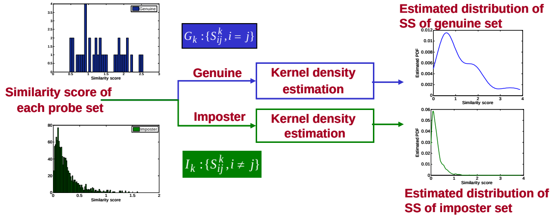
Figure 5.8. Illustration of the probability density estimation by kernel density estimation from discrete similarity scores of a certain probe set.
