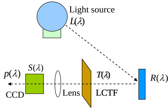
Figure 4.2. The camera response p(\lambda) is the result of integration of all the factors involved, including the spectral distribution of the illumination L(\lambda) , reflectance of the subject R(\lambda) , the transmittance of LCTF T(\lambda) and the spectral response of the camera S(\lambda) .
