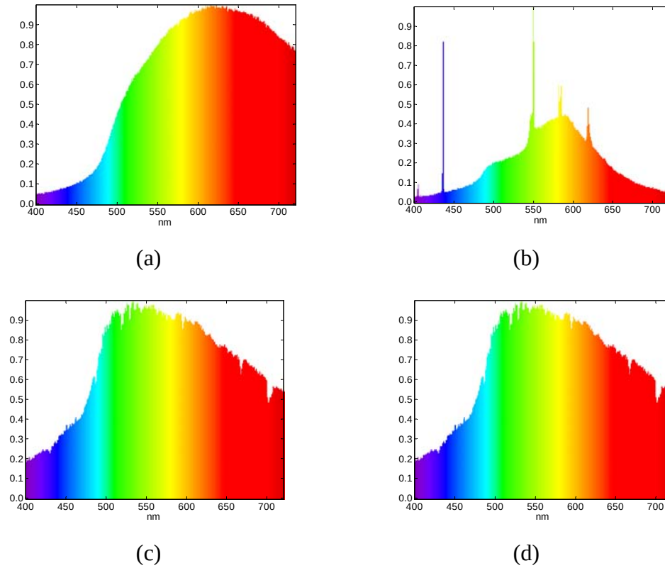
Figure 3.7. Normalized spectral power distribution of (a) halogen light (b) fluorescent light, (c) day light, and (d) another fluorescent light.
