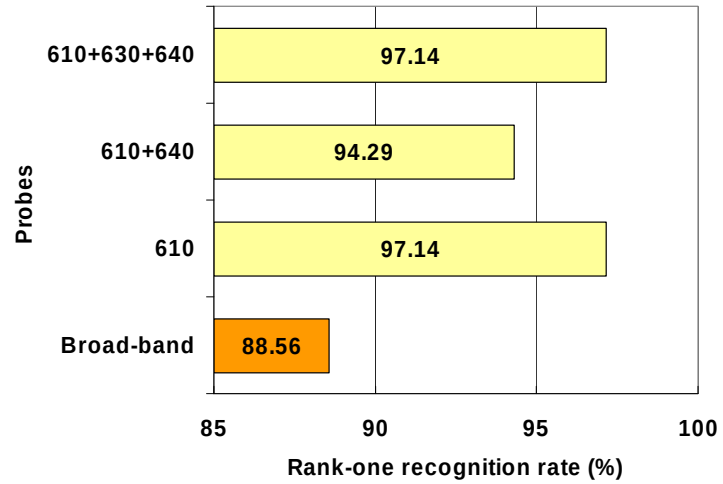
Figure 6.18. Rank-one recognition rate of different probe sets, including conventional broad-band images, single sub-spectral images at 610nm, fused images from selected two bands (610, 640) and selected three bands (610, 630, 640).
