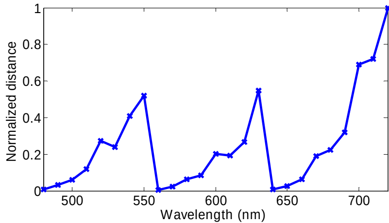
Figure 6.5. Normalized distance measure values for 25 bands with three local peaks.
