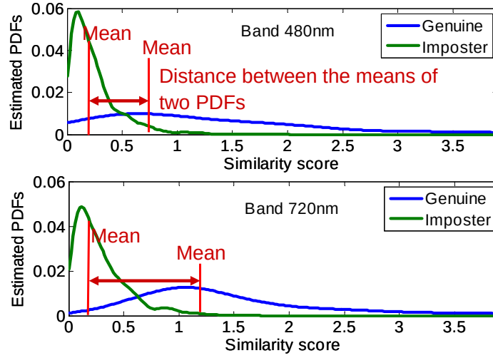
Figure 5.6. Illustration of different separations between the PDFs of the similarity scores from the genuine and imposter sets. More separated PDFs are observed from band 720nm than from band 480nm.
