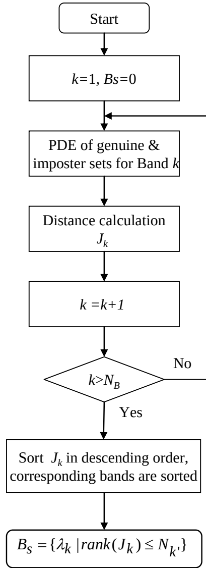
Figure 5.11. The flow chart of the distance-based band selection algorithm.
