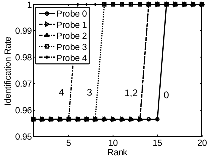
Figure 4.6. CMC plots of probes in Experiment 4.5.1. Physics-based weighted fusion (Probe 1), IA (Probe 2), single band (Probe 3) and wavelet fusion (Probe 4) outperform conventional images (Probe 0).
