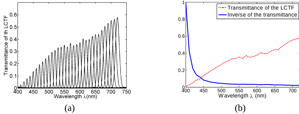
Figure 3.5. (a) The narrow-band transmittances of the LCTF from 400nm to 720nm with the increment of 10nm. (b) The ideal spectral distribution of a light source which can completely compensate the transmittance of the filter (red line) is indicated by the blue line.
