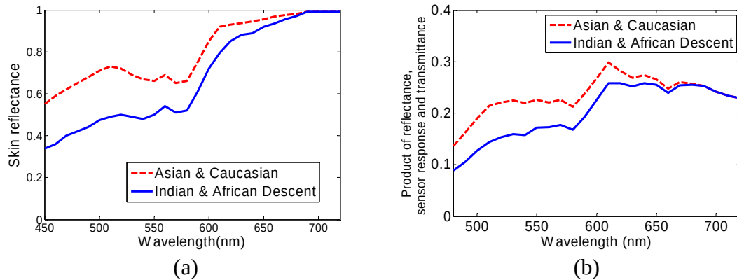
Figure 4.3. (a) Normalized skin reflectance for different skin colors, and (b) the combined spectral characteristics of three factors, skin reflectance, sensor response, and the transmittance of the LCTF.
