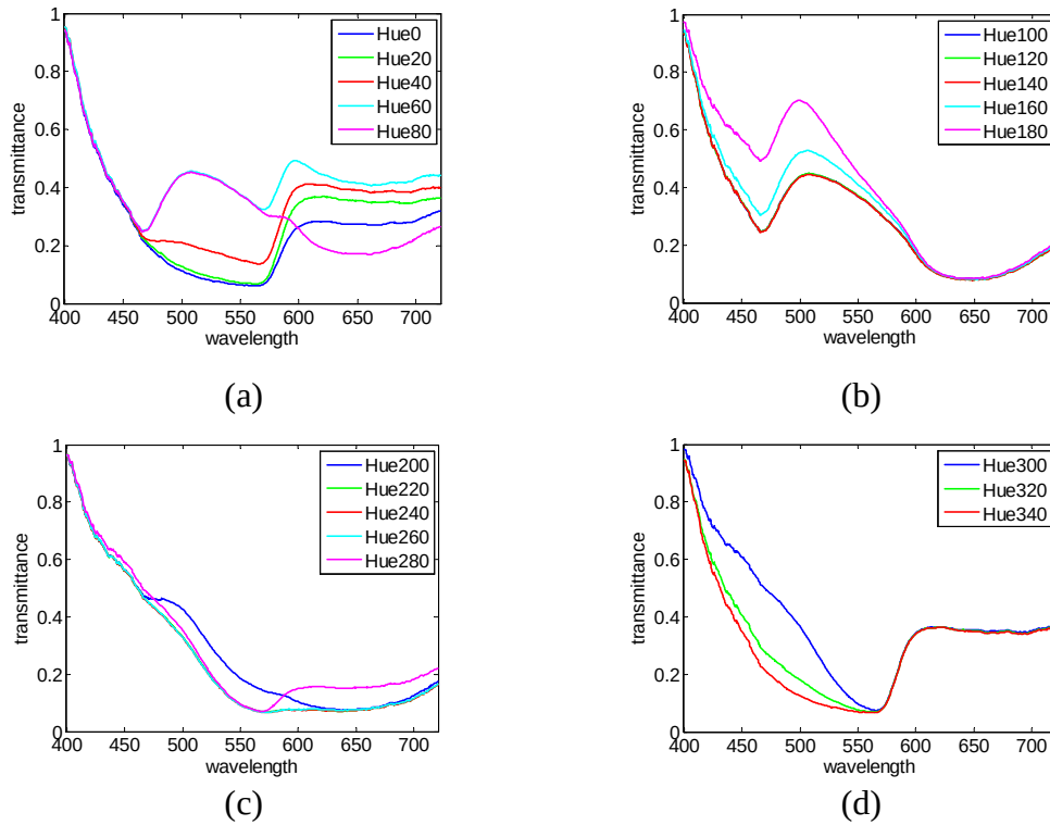
Figure 3.11. The spectral transmittance of the tunable LCD filter with different hue values and fixed value of saturation 255 and brightness 127.
