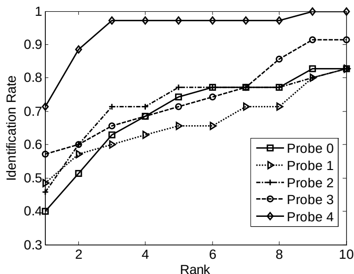
Figure 4.10. The CMC plots of selected probes in Experiment 4.5.3. Physics-based weighted, IA, wavelet and rank-level decision fusions (Probe 1 to Probe 4) all provide higher recognition rates than monochromatic images (Probe 0).
