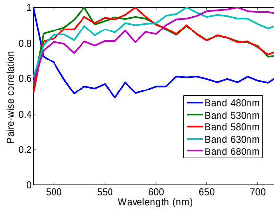
Figure 6.20. Illustration of covariance matrix for band 480nm, 530nm, 580nm, 630nm and 680nm.
