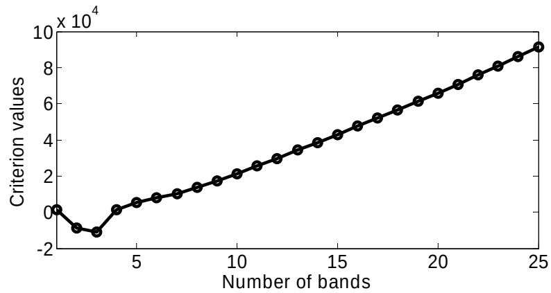
Figure 6.6. Criterion values calculated by ICOMP for different number of bands with 3 bands having the minimal value.
