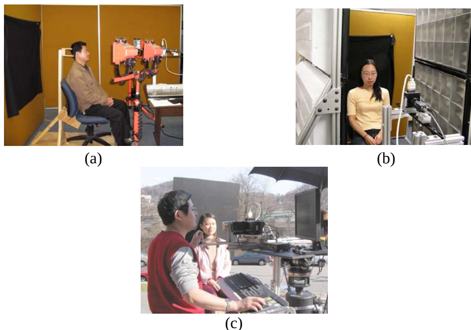
Figure 3.6. Three illumination setups, (a) quadruple halogen lights with a pair on each side halogen lighting setup, (b) a pair of fluorescent light panels, and (c) daylight with side illumination.
