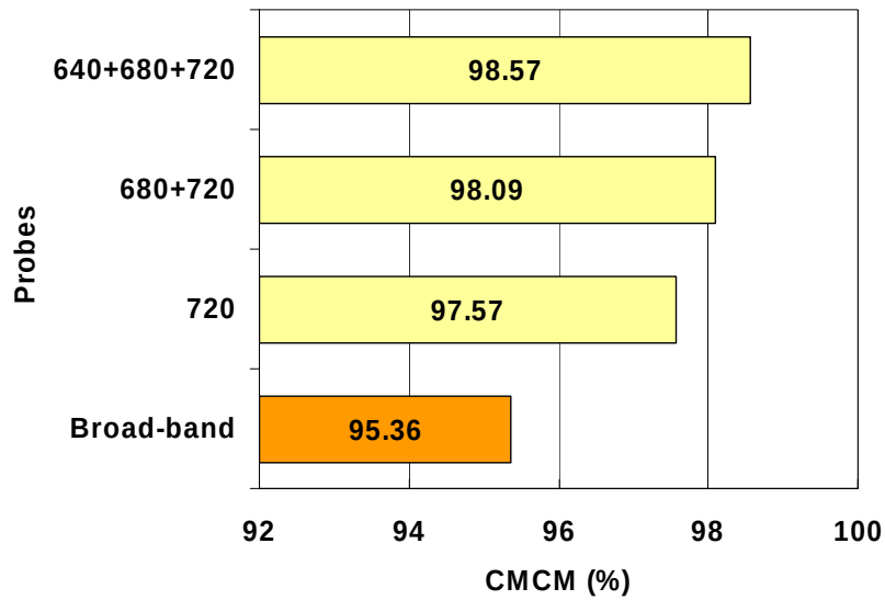
Figure 6.32. CMCM values of various probes, including broad-band monochromatic image, narrow-band images of 720nm and fused images from bands (680 720) and (640, 680, 720).
