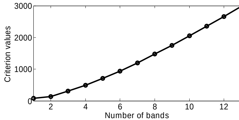
Figure 6.30. Criterion values calculated by ICOMP for different number of bands ranging from 1 to 13 and the top one band (720nm) with the minimal value.
