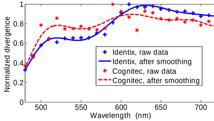
Figure 6.16. Normalized distance measure result of 25 probe sets, including sub-spectral narrow-band images from 480nm to 720 with the increment of 10nm under halogen light while the gallery images are acquired under fluorescent light. The ranking of bands in a descending order as (610, 640, 660, 680, 720, 570, 540, 510, 630, 620, 600, 650, 690, 670, 700, 710, 590, 580, 560, 550, 530, 520, 500, 490, 480).
