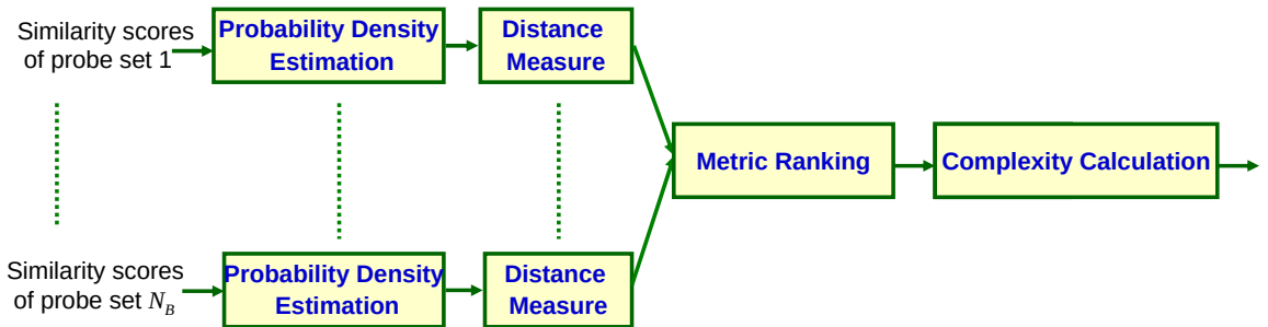
Figure 6.2. Block diagram of complexity guided distance-based band selection.
