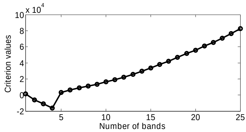
Figure 6.9. Criterion values calculated by ICOMP from different number of bands with 4 as the selected number.
