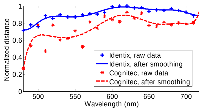
Figure 6.23. Normalized distance of 25 probes including sub-spectral narrow-band images from 480nm to 720nm with the increment of 10nm under halogen light while the gallery images are acquired under daylight.
