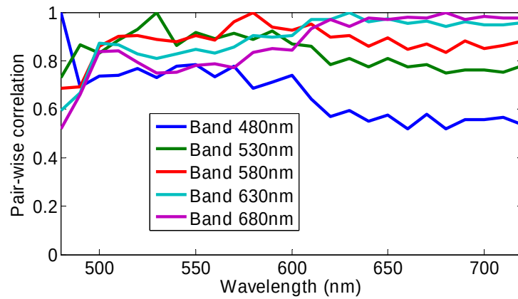
Figure 6.27. Illustration of the pair-wise correlation for band 480nm, 530nm, 580nm, 630nm and 680nm.
