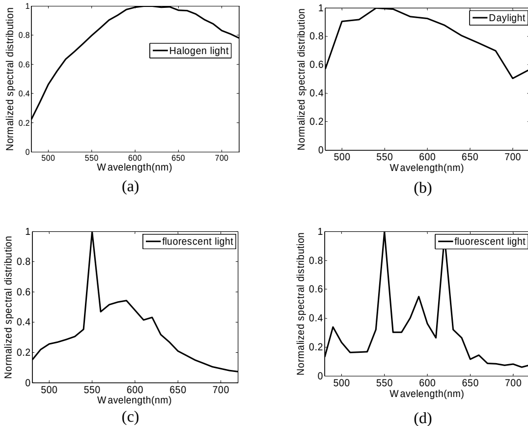
Figure 4.4. Spectral power distribution of (a) halogen light, (b) day light, (c) fluorescent light and (d) another type of fluorescent light.
