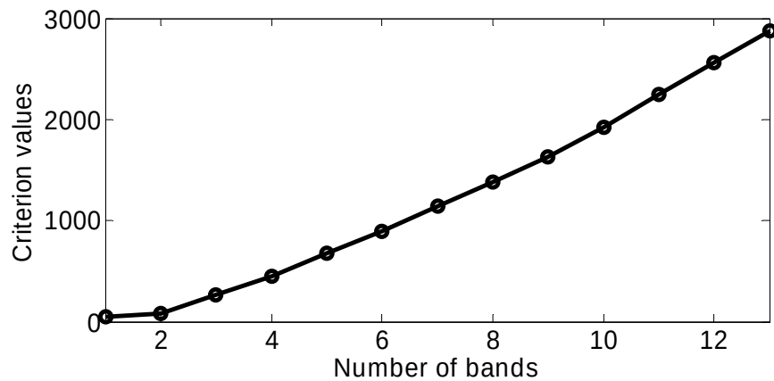
Figure 6.37. Criterion values calculated by ICOMP for different number of bands ranging from 1 to 13 and the top one band (720nm) with the minimal value.
