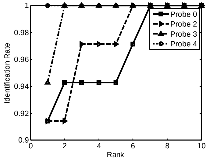
Figure. 4.8. CMC plots of probes in Experiment 4.5.2. Illumination adjustment, wavelet fusion and rank-based decision level fusion (Probe 2, 3 and 4) are more robust to longer time lapse than conventional monochromatic images (Probe 0) and provide better performances.
