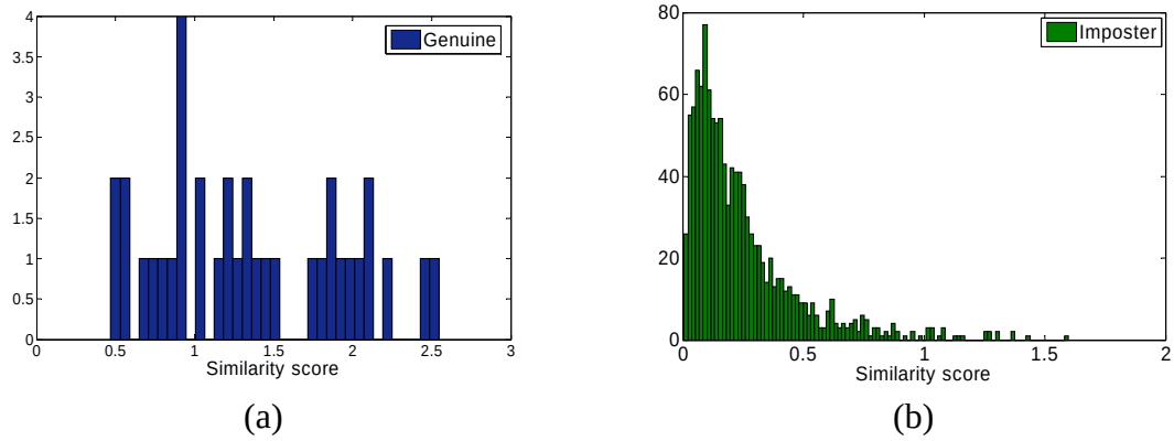
Figure 5.3. Histogram of similarity scores of (a) genuine and (b) imposter data sets from the same probe set. There are 35 subjects in the probe set. Therefore, there are 35 genuine data points and 1190 imposter data points.
