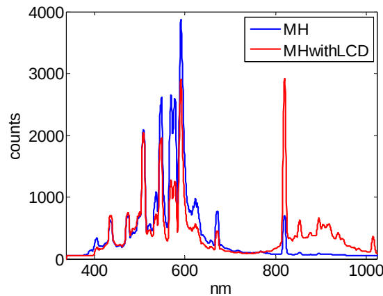
Figure 3.12. Spectral distribution comparison with and without the filter in front of the metal halide light.
