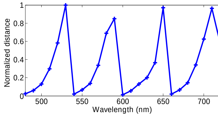
Figure 6.8. Normalized distance measure values for 25 bands with four local peaks.
