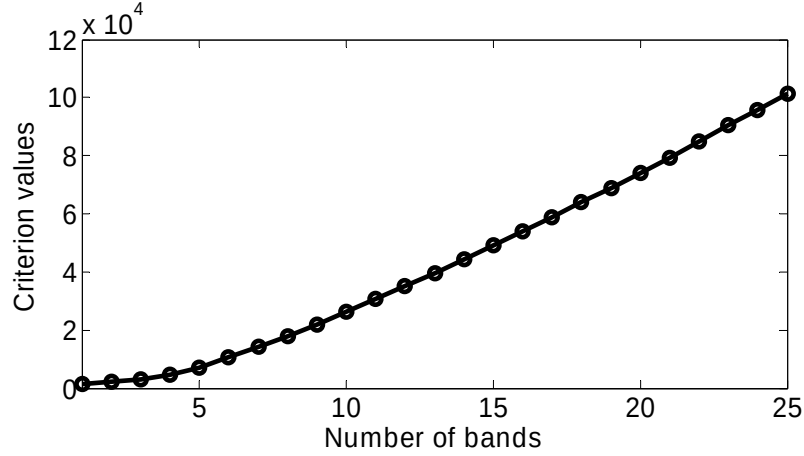
Figure 6.15. Criterion values by ICOMP for different number of selected bands.
