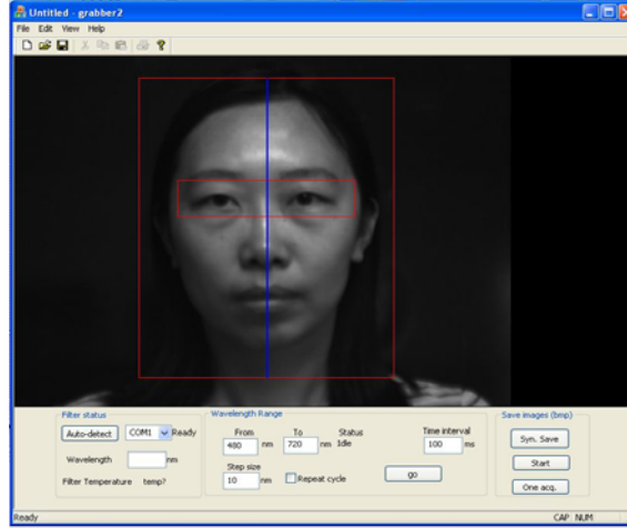
Figure 3.4. Graphical user interface of the software developed to synchronize the tuning of the LCTF with the frame acquisition process.
