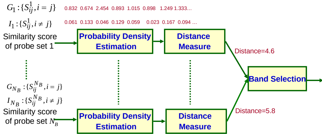
Figure 5.7. Illustration of the algorithm pipeline. The blocks of proposed steps are filled with yellow and the steps are highlighted in blue color.
