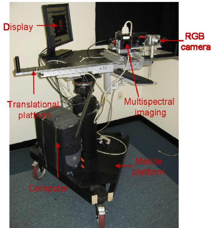
Figure 3.1. The all-inclusive multimodal and multispectral mobile imaging system for indoor and outdoor face data acquisition.
