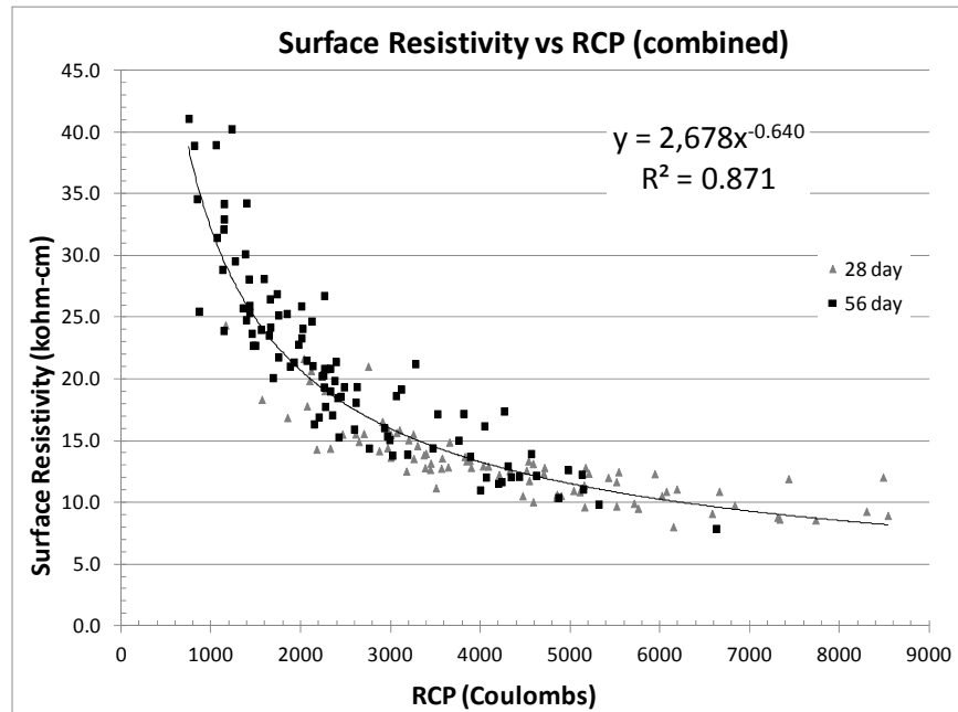
Figure 10: Combined SR versus RCP (28 and 56 Days)
