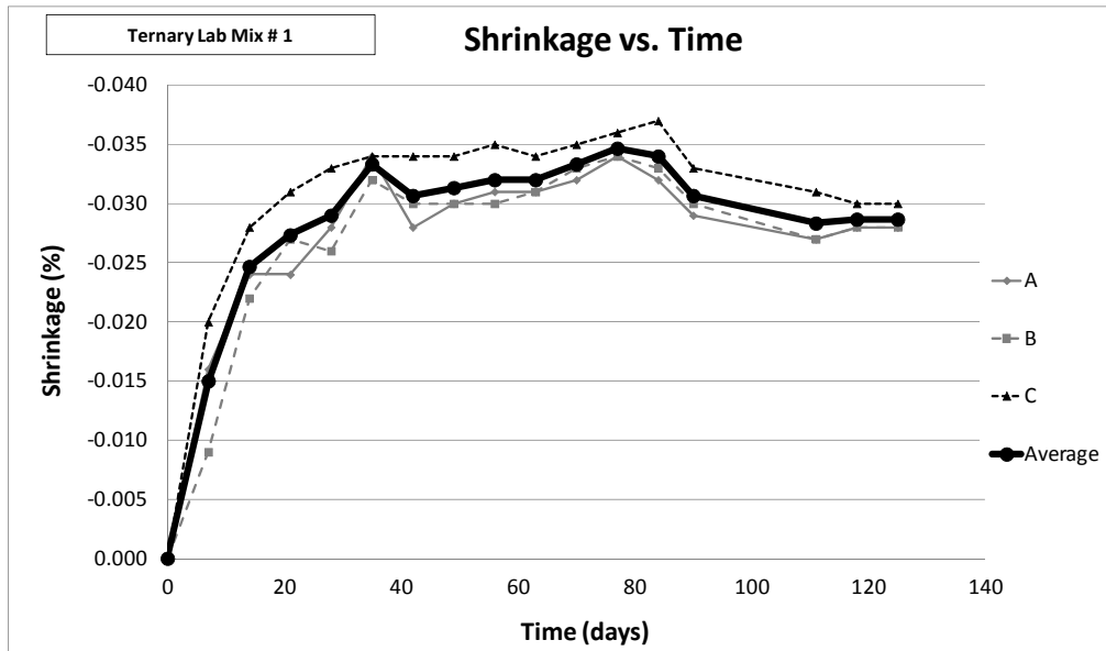
Figure 16: Shrinkage Measurements – Ternary Lab Mixture # 1
