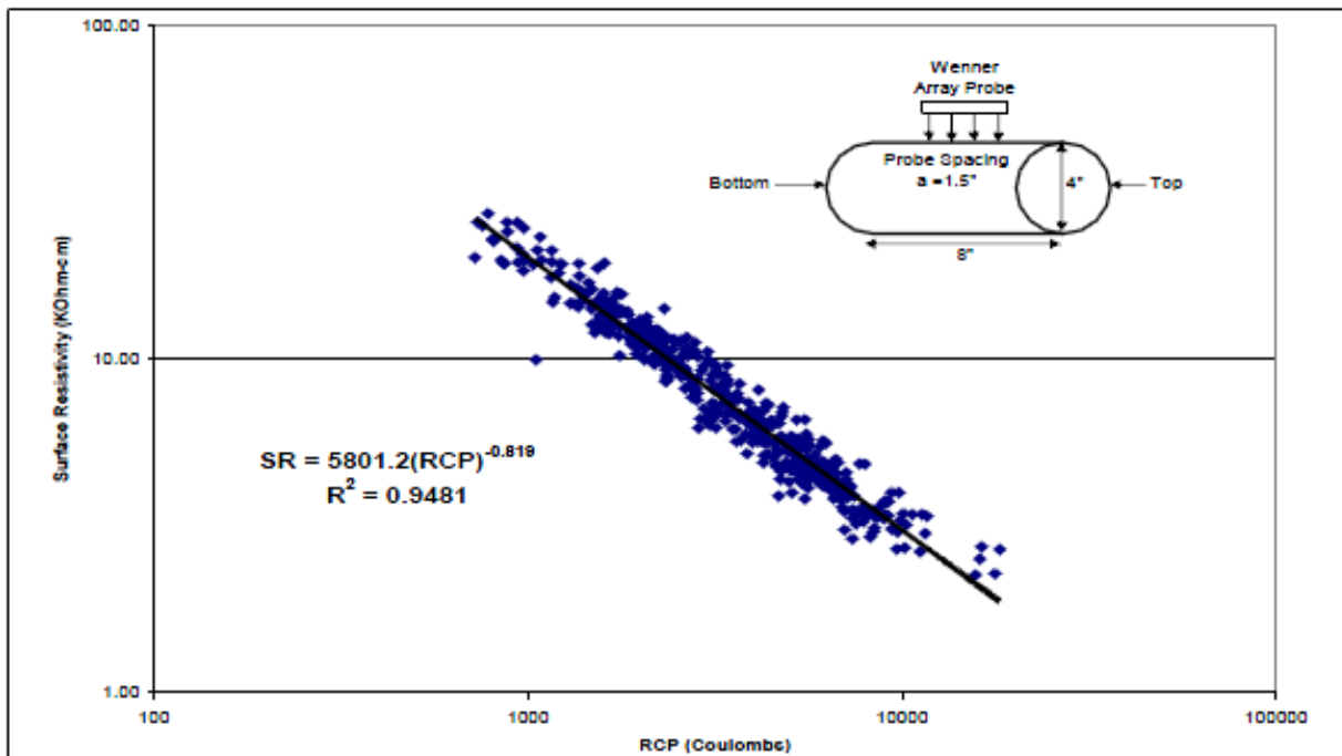
Figure 5: Florida DOT SR vs. RCP results – 28 days (39)
