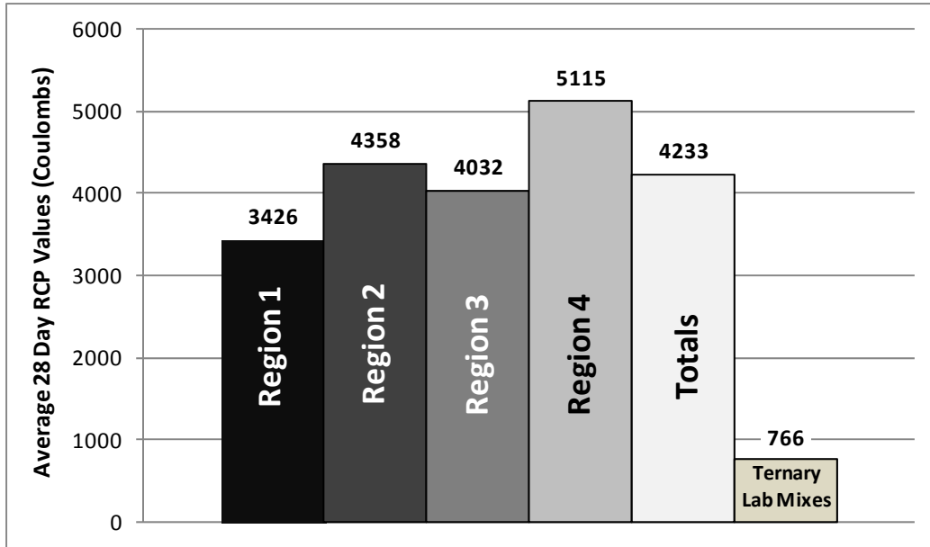
Figure A - 5: Average 28-day RCP Values
