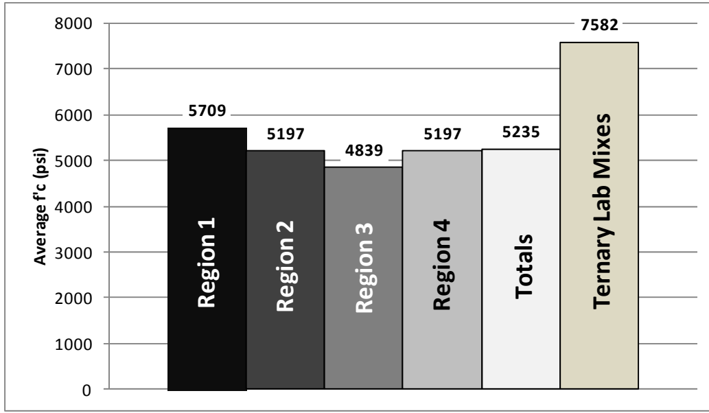
Figure A - 1: Average 28-day Compressive Strengths
