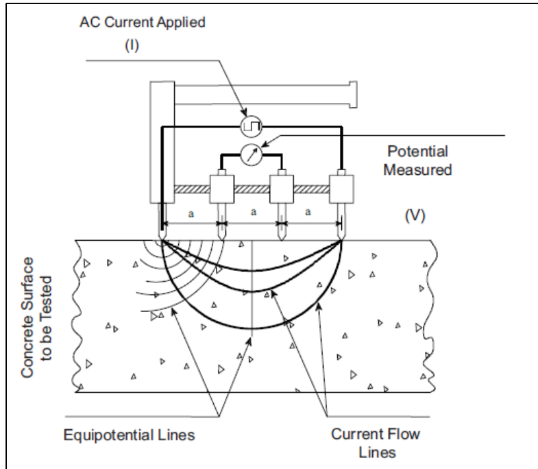
Figure 4: Four-Point Wenner Array Probe Test Setup (8)
