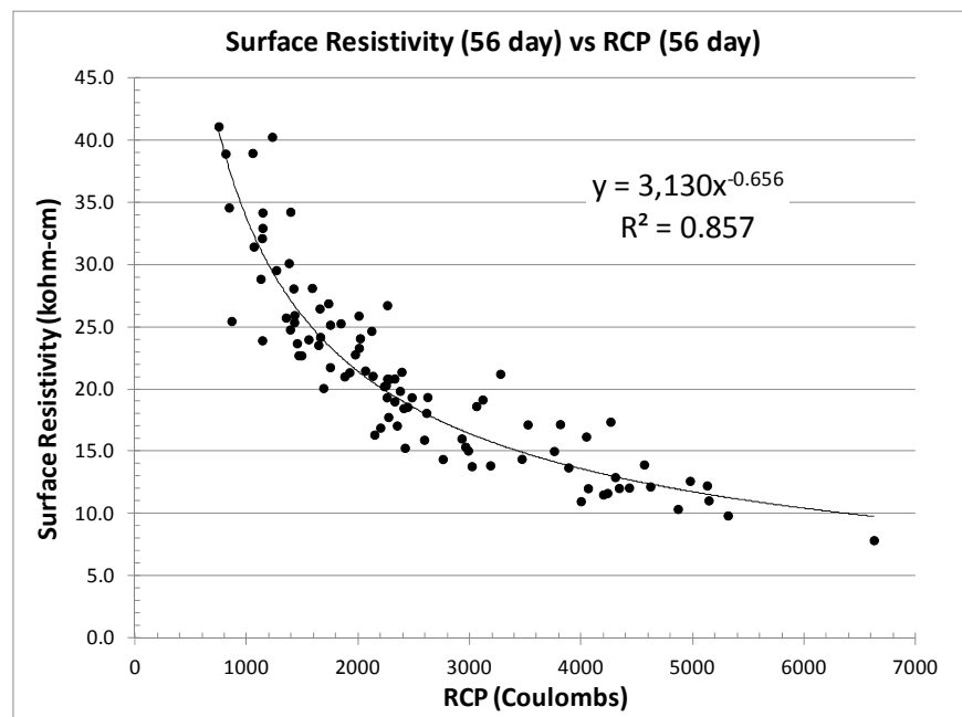
Figure 11: SR versus RCP (56 days)
