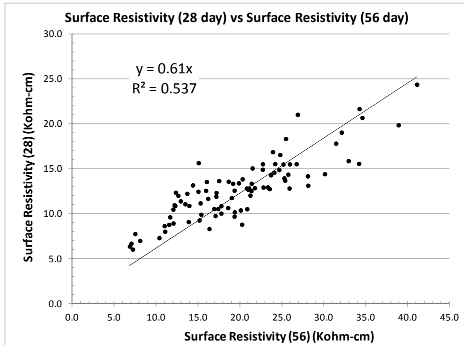
Figure A - 7: 28-day SR Values versus 56-day SR Values
