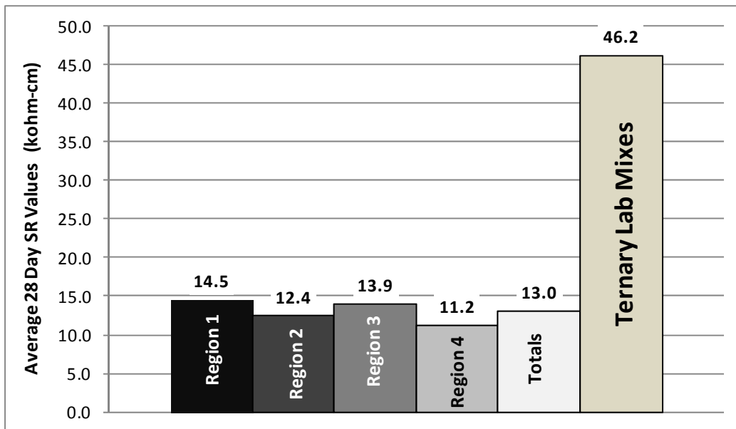
Figure A - 2: Average 28-day SR Values
