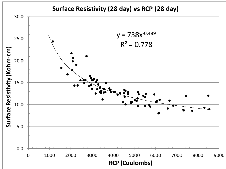
Figure A - 9: 28-day SR Values versus 28-day RCP Values
