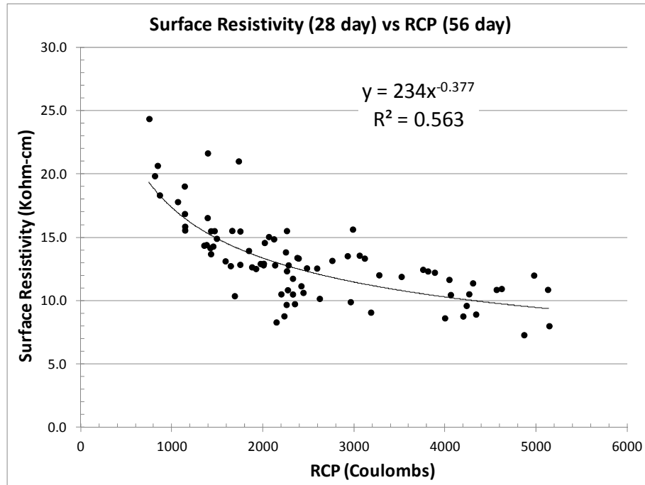
Figure A - 8: 28-day SR Values versus 56-day RCP Values
