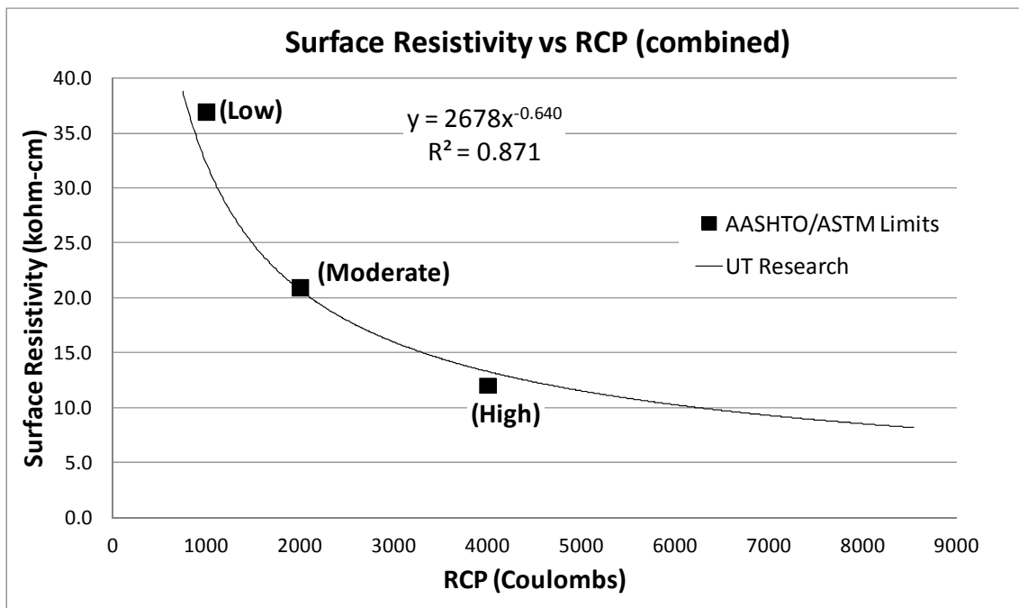
Figure 13: SR versus RCP (28 and 56 days) with AASHTO/ASTM Limits
