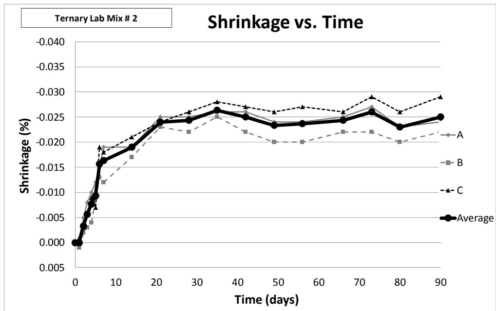
Figure 17: Shrinkage Measurements – Ternary Lab Mixture # 2
