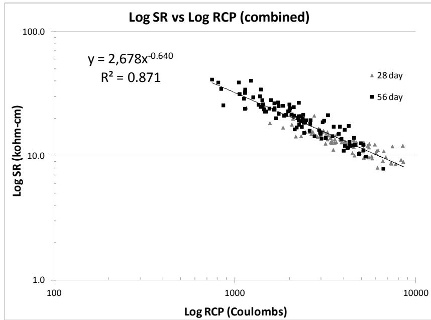
Figure 9: Combined Log SR versus Log RCP (28 and 56 Days)
