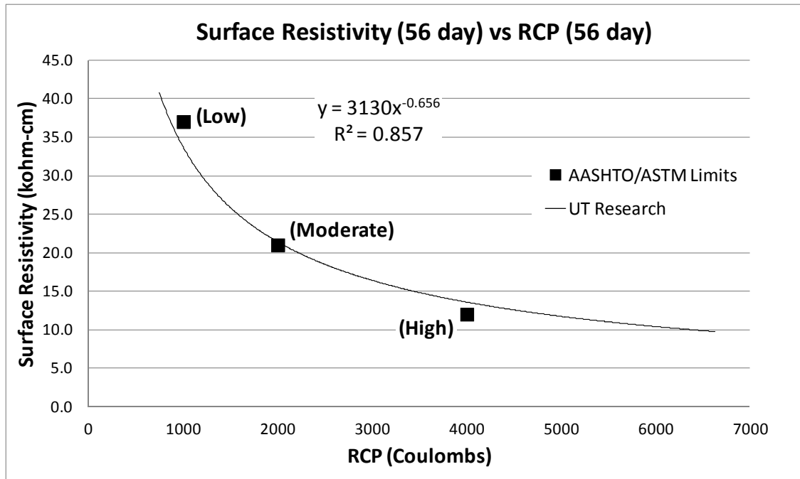
Figure 12: SR versus RCP (56 days) with AASHTO/ASTM Limits
