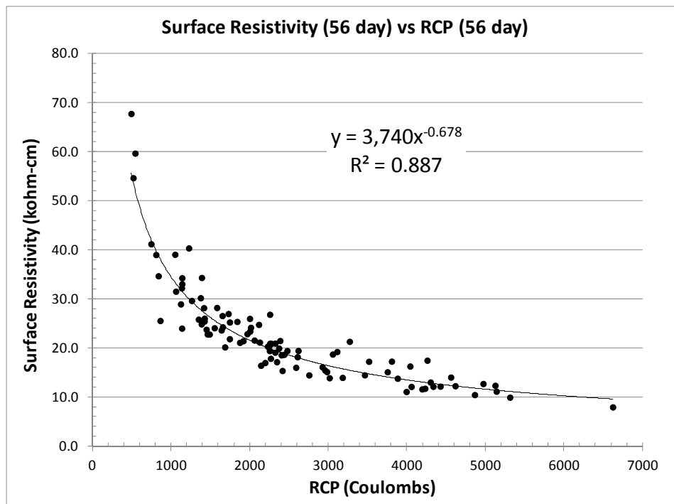
Figure 14: SR versus RCP (56 days) – With Ternary Blend Mixtures
