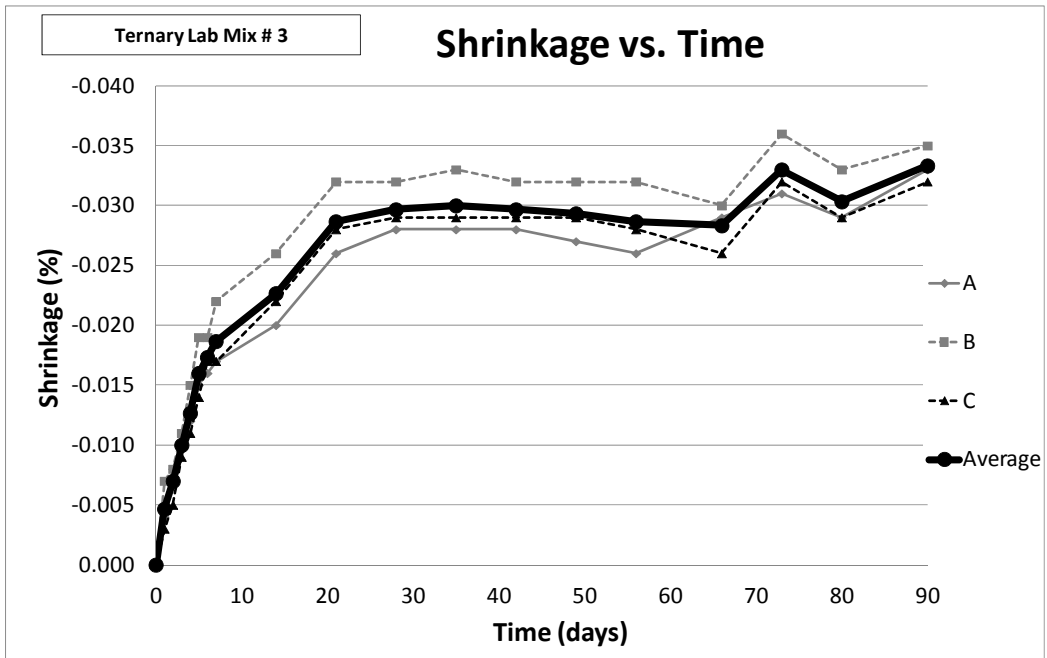
Figure 18: Shrinkage Measurements – Ternary Lab Mixture # 3
