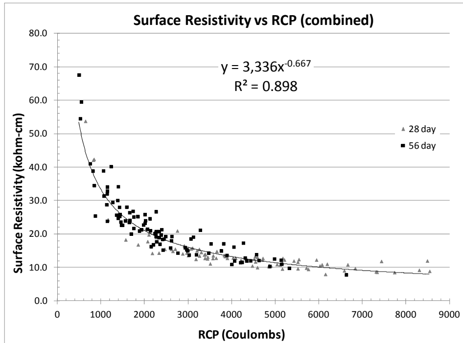
Figure 15: SR versus RCP (28 and 56 days) – With Ternary Blend Mixtures
