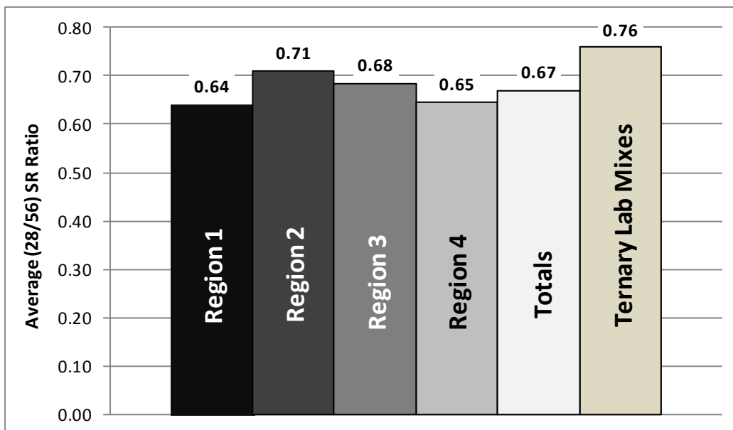
Figure A - 4: Average (28-day/56-day) SR Ratios
