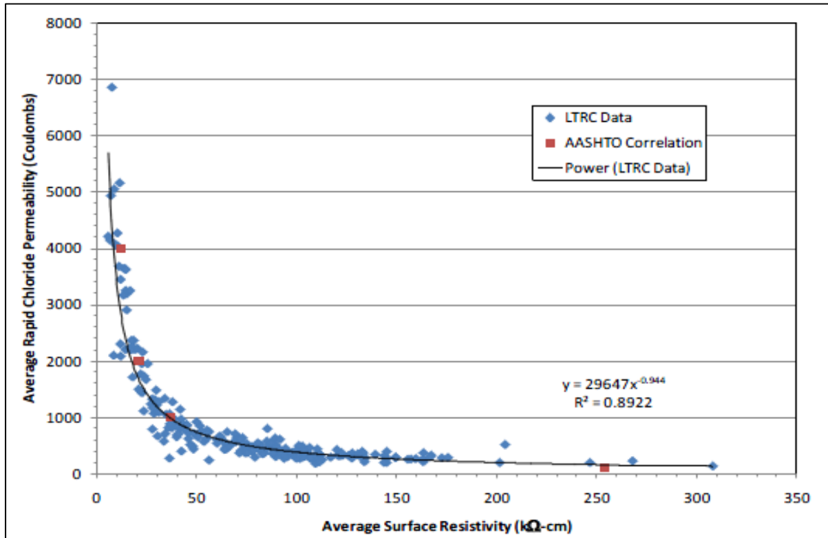
Figure 6: Louisiana DOT SR vs. RCP results – All Test Ages (58)
