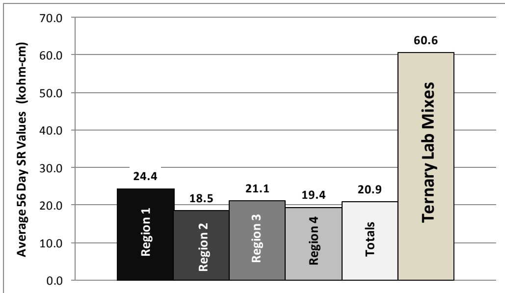
Figure A - 3: Average 56-day SR Values
