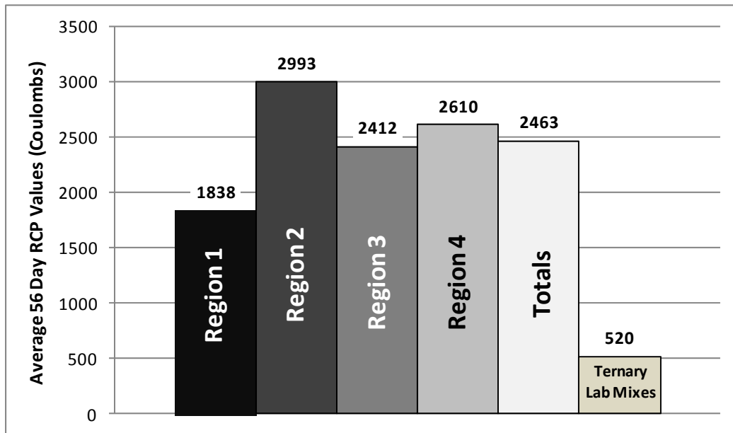
Figure A - 6: Average 56-day RCP Values
