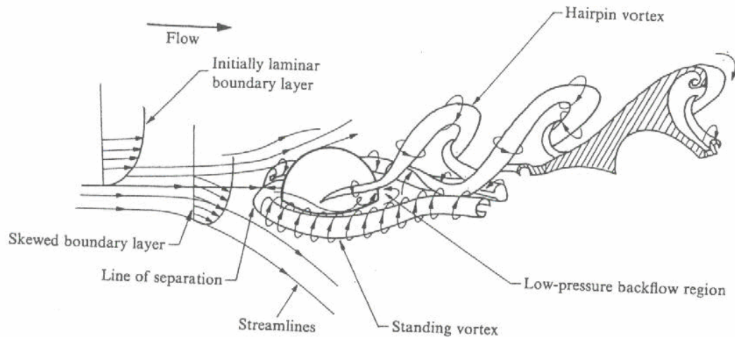
Fig. 1-2 Schematic of near-wake structure in the hemisphere wake
