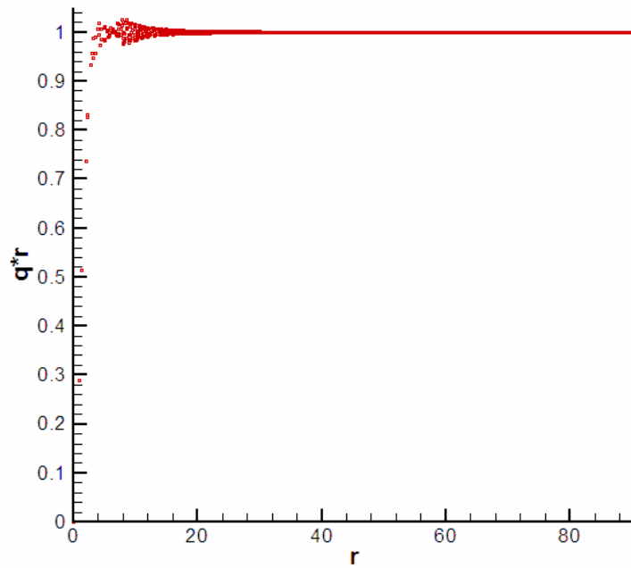
Fig. 3-18 Velocity magnitude distribution for the stationary vortex after 100 time iterations with VC1
