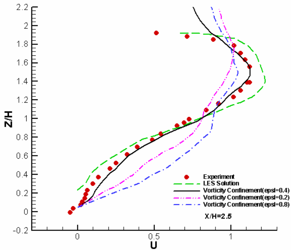
Fig. 4-99 the comparison of mean velocity component U for the different confinement coefficients at X/H=2.5 ( 20 \times 20 \times 20 cube)
