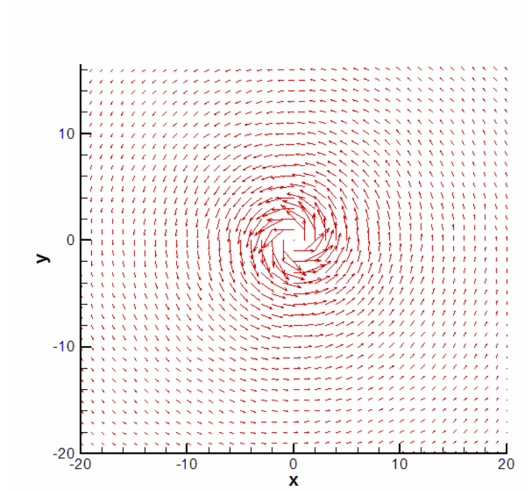
Fig. 3-5 Velocity vector field after 100 time iterations with VC2
