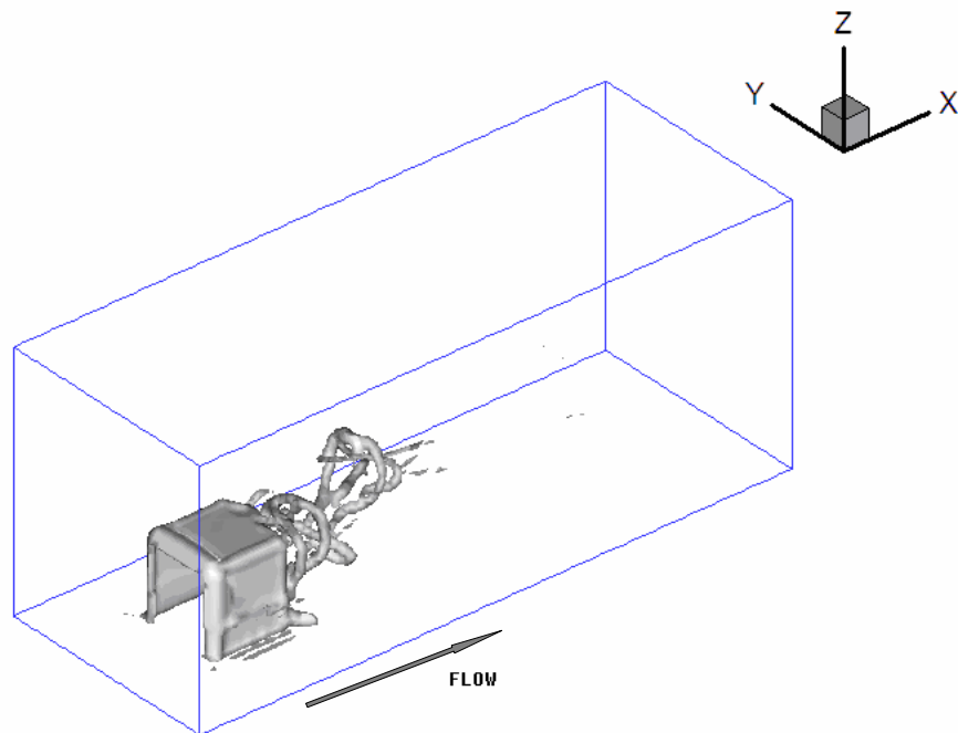
Fig 4-29 Vorticity iso-surface from the different viewing angle, after 700 time steps
