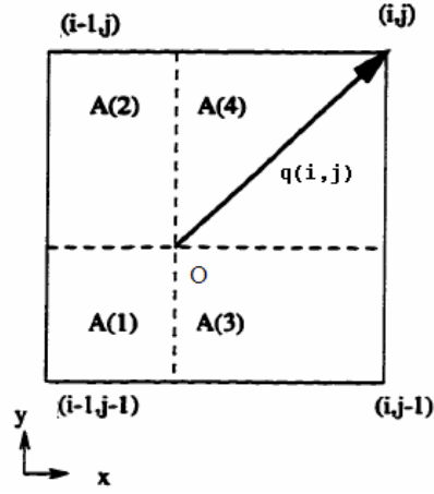
Fig. 2-2 The diagram for the image point location and weighting
