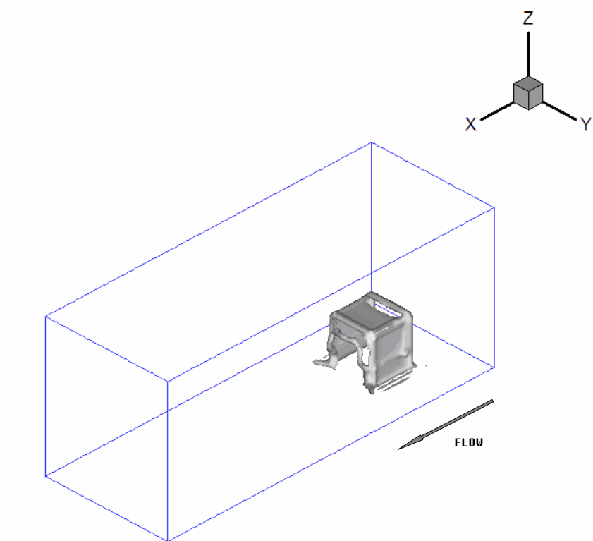
Fig. 4-6 Vorticity iso-surface, after 50 time steps
