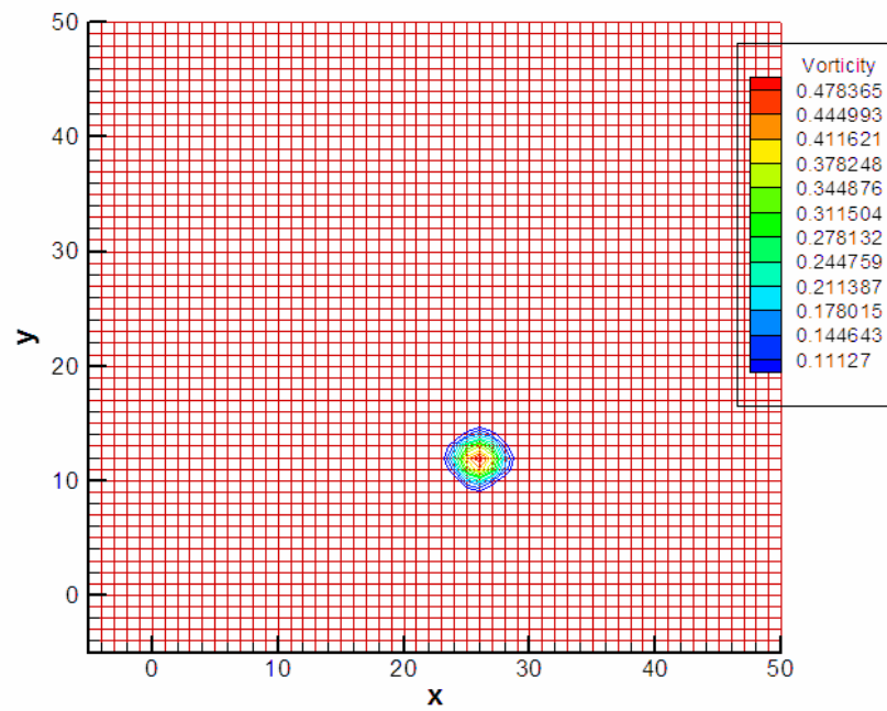
Fig. 3-27 Vorticity contours after 3000 time iterations with VC1
