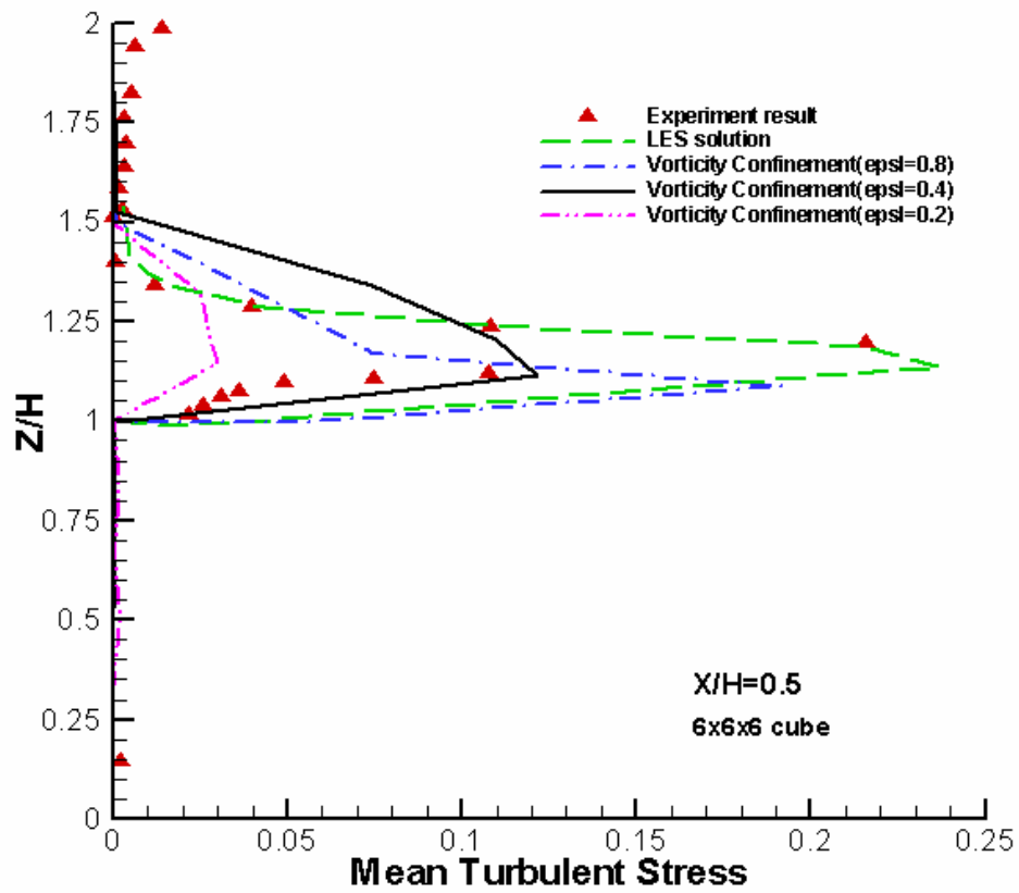
Fig. 4-107 Comparison of mean turbulent stress ( \overline{u'^2} ) for different confinement coefficients at X/H=0.5 ( 6 \times 6 \times 6 cube)
