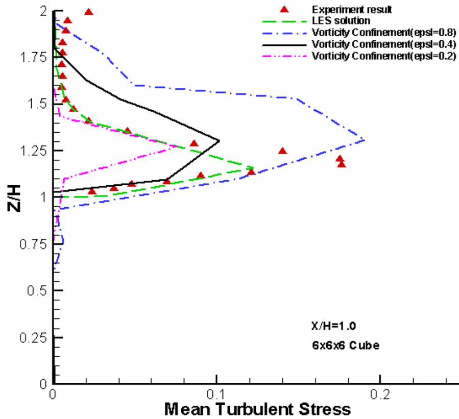
Fig. 4-108 Comparison of mean turbulent stress ( \overline{u'^2} ) for different confinement coefficients at X/H=1.0 ( 6 \times 6 \times 6 cube)
