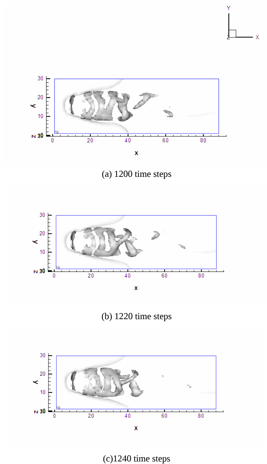
Fig. 4-79 Vorticity iso-surface, top views in a sequence of time steps
