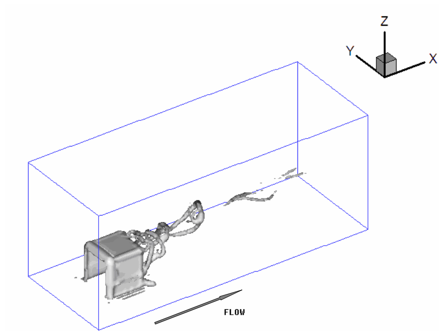
Fig 4-31 Vorticity iso-surface from the different viewing angle, after 1200 time steps
