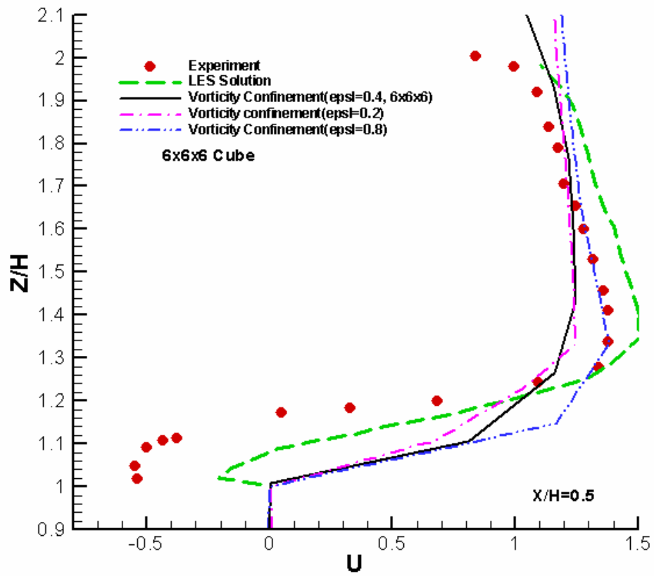
Fig. 4-104 Comparison of mean velocity component U for the different confinement coefficients at X/H=0.5 (6x6x6 Cube)
