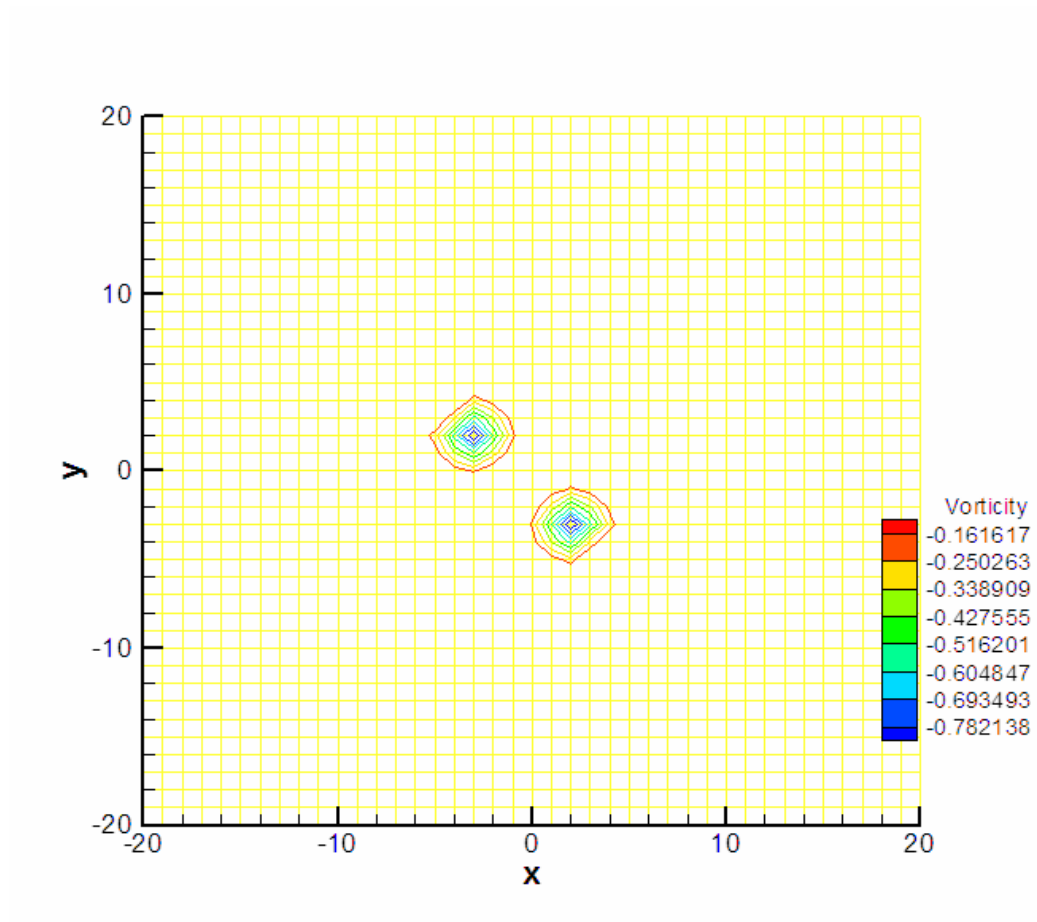
Fig. 3-48 Initial positions of paired vortices of the same signs, 8 cells apart
