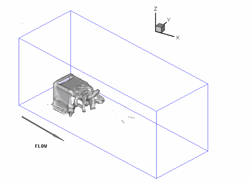
Fig 4-21 Vorticity iso-surface from the different viewing angle, after 600 time steps
