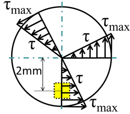
Figure 5.2 Cross section showing shear stress gradient with radial position, and experimental gauge volume location (Robin Woracek et al., 2012)
