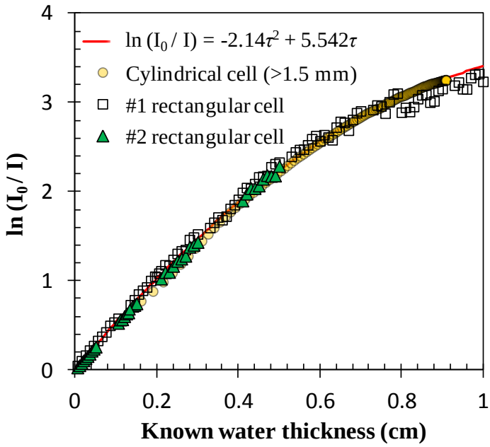
Figure 2- 9 Best fit of Eq. [7] to the measured neutron data versus known water thickness ( \tau ) for all three calibration cell types located 24 cm away from the detector.
