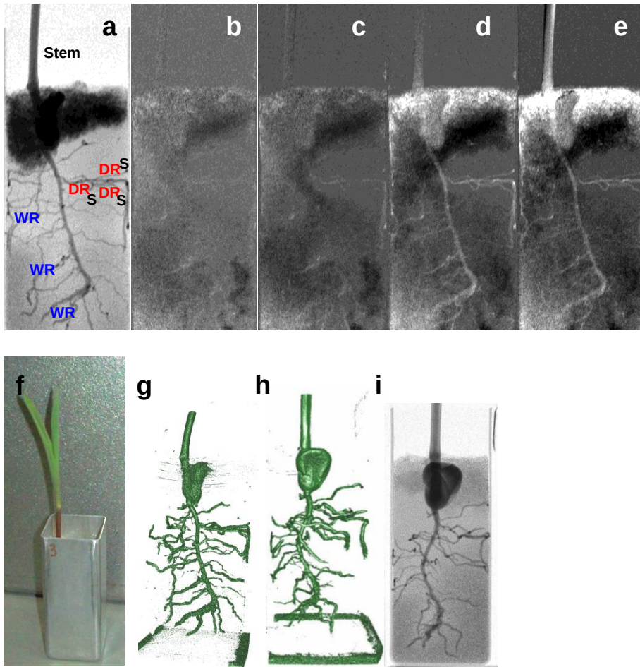
Figure A 5. In situ water uptake and transport in a 10-d old maize seedling. a) Initial neutron radiographic image prior to addition of 3 ml of D 2 O to surface – dark areas represent existing H 2 O within the soil and plant; b-e) the same system 0.25, 0.5, 6 or 12 h after surface irrigation with D 2 O, divided by the initial image – light areas represent displacement of H 2 O and uptake and transport of D 2 O (reference Video S3); f) photograph of sample chamber; g-h) 3D tomographic reconstruction from two different angles, which confirmed identification of individual roots (reference Video S4); (i) One of the 360 2D neutron radiographs used for tomography.
