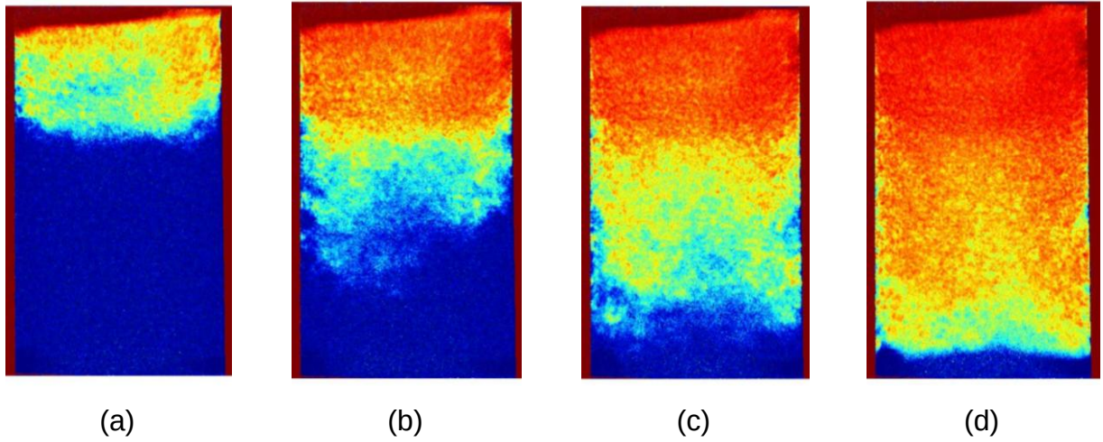
Figure 3- 5 Relative saturation images (1 = blue, 0 = red) for basal matrix potentials of (a) -15.61 cm, (b) -18.47 cm, (c) -20.37 cm, and (d) -21.80 cm in a drying sequence. Note that the filter paper phase barrier at the bottom of sand column remains fully saturated throughout the drainage process.
