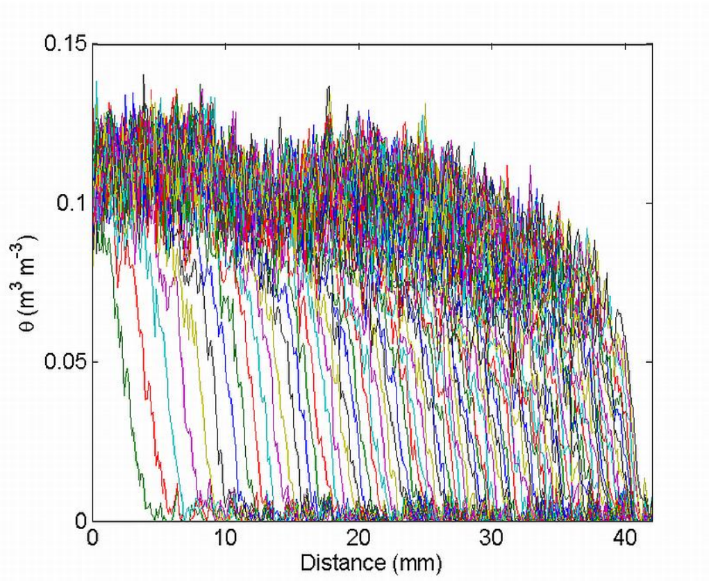
Figure 5- 3 Volumetric water content as a function of distance at different times (identified by different colors) for Berea core sample C3. The volumetric water contents were measured along the central vertical line from a total of 90 images.
