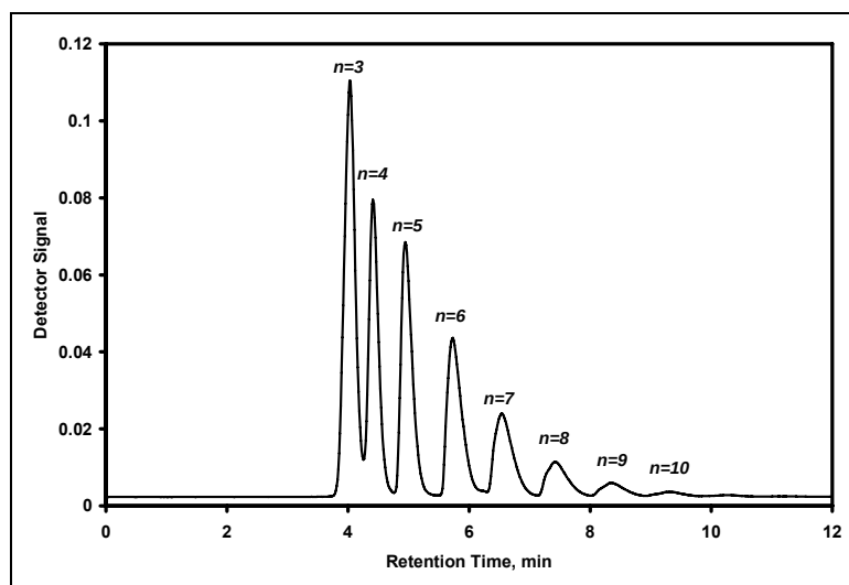
Figure 3.3: Chromatograms of pure CK7. C 18 reverse phase column, isocratic mobile phase of 98 vol% acetone and 2 vol. % acetic acid at 1 mL/min. ELSD detector. n refers to the degree of polymerization of the surfactant molecule's ethoxylate group.
