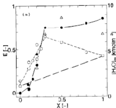
Figure 2.11: Dependence of the fraction of \alpha -chymotrypsinogen A (E) the concentration of water extracted from the aqueous phase on X, the fraction of AOT based on the whole surfactant. \Delta , E about 20 min after the contact; \bullet , E about 2 days after the contact; \circ , [H_2O]_m [4]
