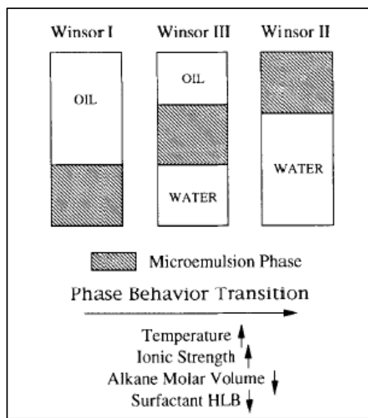
Figure 2.12: Diagram of effects of the variables (legend in the diagram) in the phases of a system composed of oil, water and a non-ionic surfactant [1].
