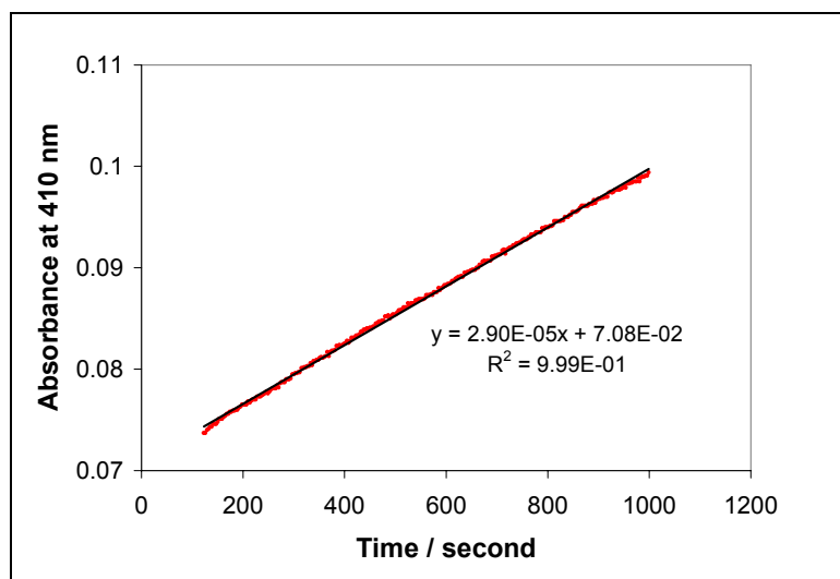
Figure 6.1: Absorbance of light at \lambda=410\text{nm} versus time of the hydrolysis of GNPNA catalyzed by \alpha -chymotrypsin under standard conditions, used to calculate the “standard” activity of \alpha -chymotrypsin (“St” in Eq. 1). 50 \mu\text{L} of 0.5 mg/mL \alpha -chymotrypsin in 5 wt. % NaCl aqueous solution was mixed with 700 \mu\text{L} of GNPNA substrate solution, as described in the Experimental section. (red circles): experimental data; (black line): straight-line fit to the data.
