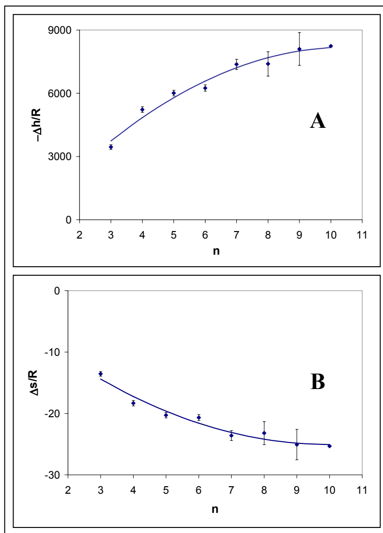
Figure 4.6: Enthalpy and Entropy values divided by the gas constant (R) versus ethoxylate size for the CK7 / CK3 mixed surfactant system. Constants of van't Hoff equation obtained by fitting Equation 4.3 . A) Slopes of fitted lines ( Equation 4.3 ) in Figure 4.5 . B) y-Intercepts of fitted lines ( Equation 4.3 ) in Figure 4.5 . Concentrations in both figures are 3.75 wt. % CK7 and 3.75 wt. % CK3 overall surfactant. Curve represents second-order polynomial fit to the data.
