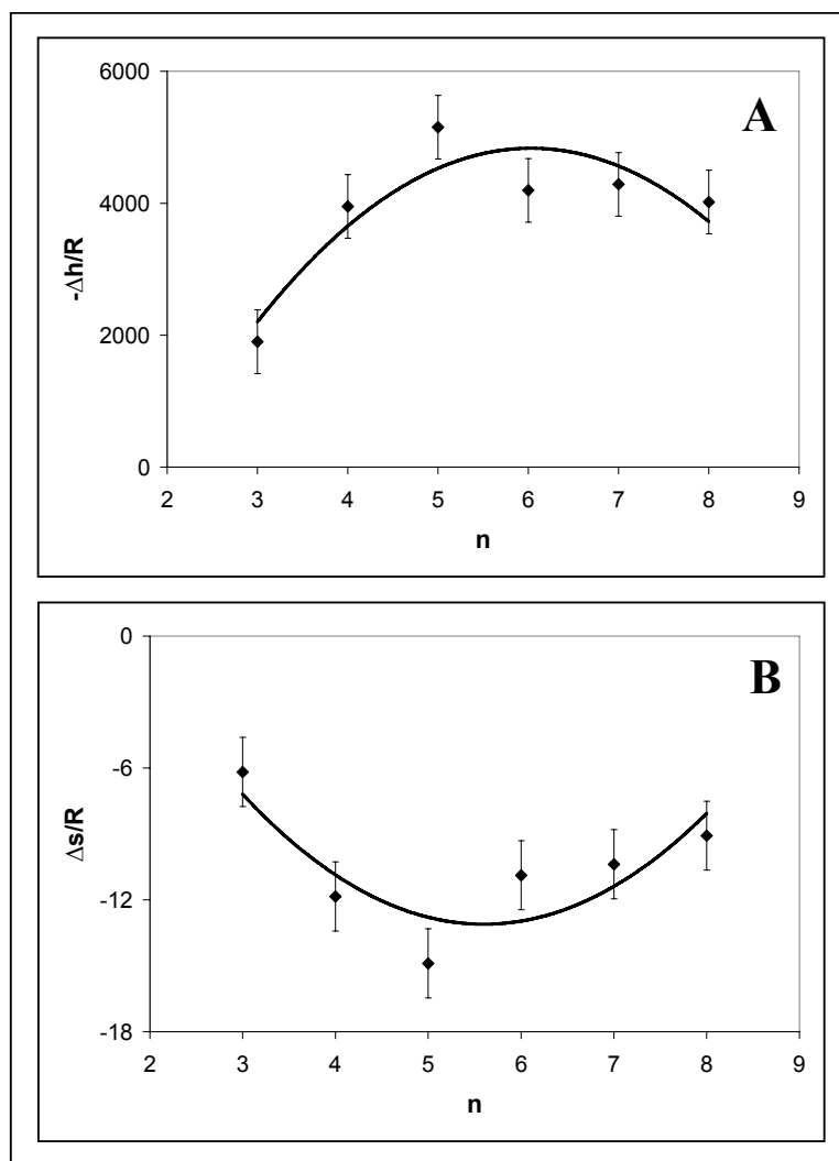
Figure 4.10: Enthalpy and Entropy values divided by the gas constant (R) versus ethoxylate size for the CK7 / AOT mixed surfactant system. Constants of van't Hoff equation obtained by fitting Equation 4.3 to the partitioning data of CK7 for the mixed AOT / CK7 system in the presence of salt. A) Slopes of fitted lines ( Equation 4.3 ) in Figure 4.9 . B) Intercepts of fitted lines ( Equation 4.3 ) in Figure 4.9 . Concentrations are 3.75 wt.% CK7 and 3.75 wt.% AOT. Solvents are isooctane and 1 wt. % NaCl in water solution. Curve represents second-order polynomial fit to the data.
