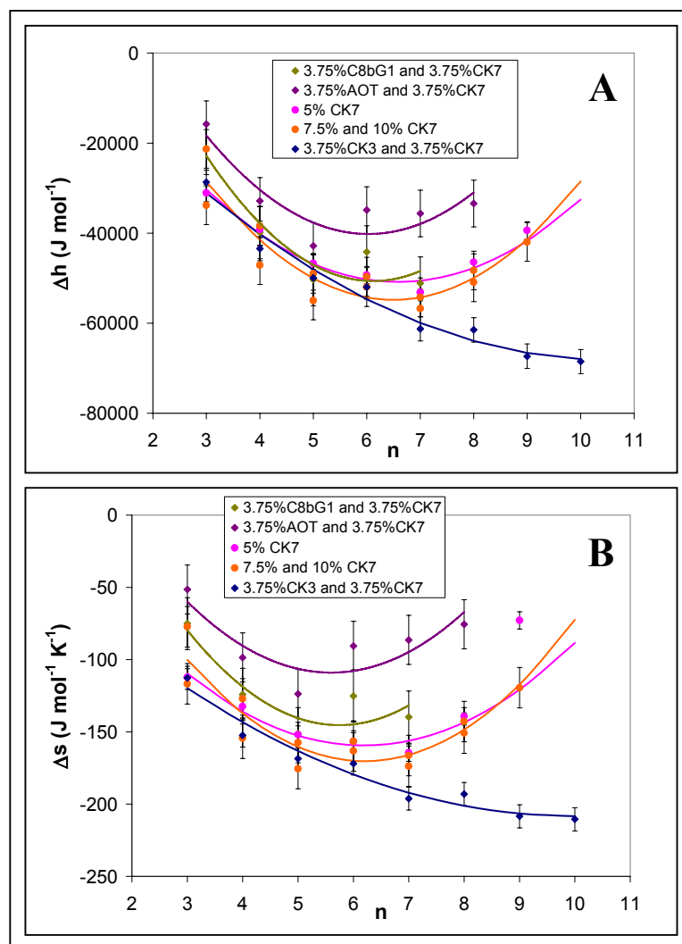
Figure 4.16: A) Enthalpy and B) entropy of transferring a molecule from oil to water. Dots are calculated from measured data and solid lines are second order polynomial fitted to the data. Each color corresponds to the concentration of surfactants described in the legend.
