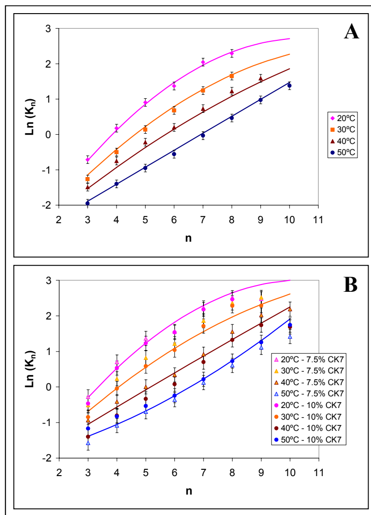
Figure 4.4: The effect of ethoxylate group size, surfactant concentration, and temperature on the partitioning of CK7. Data and values obtained by the semi-empirical model (Section 4.2). Natural logarithm of distribution constant ( K_n = (C_{wn}/C_{on}) ) for CK7 surfactant versus number of ethylene oxide unit as a function of temperature. A) 5 wt. % overall concentration of CK7. B) 7.5 wt. % and 10 wt. % overall concentration of CK7. 20°C is W-I and 30°C to 50°C are W-III system. Curves represent \text{Ln}(K_n) as predicted by the model (Section 4.2).
