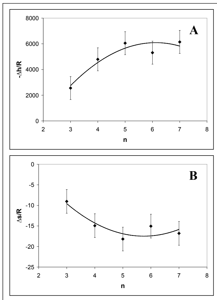
Figure 4.13: Enthalpy and Entropy values divided by the gas constant (R) versus ethoxylate size for the CK7 / C 8 βG 1 mixed surfactant system. Constants of van't Hoff equation obtained by fitting Equation 4.3 to the partitioning data of CK7 for the mixed CK7 / C 8 βG 1 system. A) Slopes of fitted lines (Eq. 4.3) in Figure 4.12 . B) Intercepts of fitted lines (Eq. 4.3) in Figure 4.12 . Concentrations are 3.75 wt. % CK7 and 3.75 wt. % C 8 βG 1 . Solvents are isooctane and water. Curve represents second-order polynomial fit to the data.
