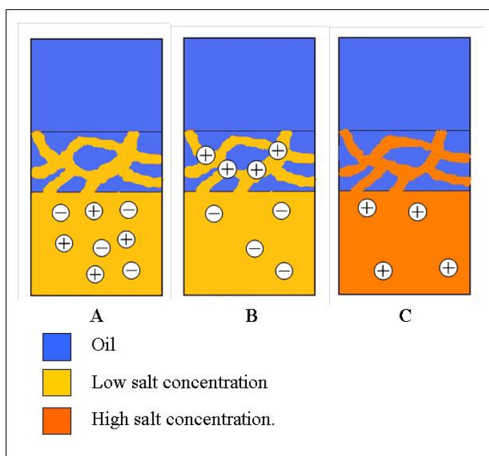
Figure 2.13: Diagram of protein purification by Winsor-III microemulsion system. The sequence from the left to the right is: A) Mixing oil with surfactants and water phase with proteins and low concentration of salt. B) Proteins with charge opposite to surfactant are extracted in bicontinuous phase. C) Bottom solution is replaced by a stripping solution with a concentration of salt high enough to produce Debye shielding and the proteins are released.
