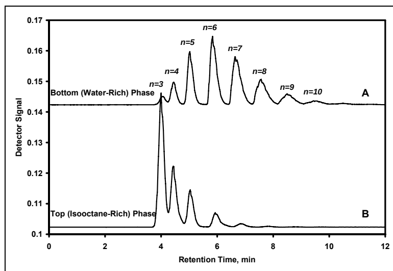
Figure 4.1: Example of chromatograms for the equilibrium partitioning of CK7 in a Winsor-III system obtained from reverse-phase HPLC analysis. A) Aqueous phase (bottom). B) Oil phase (top). The degree of polymerization n corresponding to each peak is indicated in the figure.
