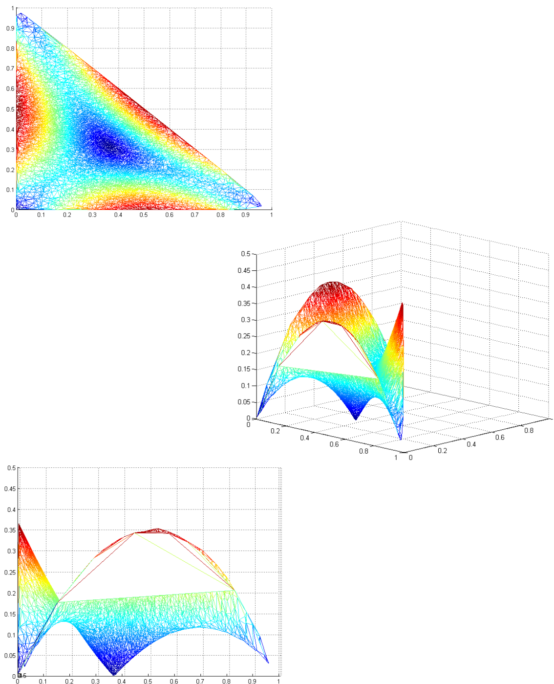
Figure 4-4: 10,000 experiments of the branching distributed between three circles. From top to bottom is a top, angled, and side view.
