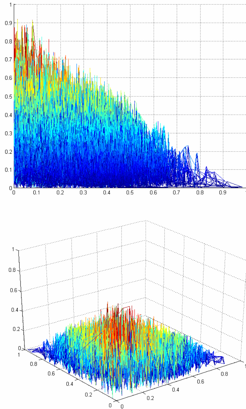
Figure 4-6: A side and angled view of 100,000 experiments on the circle packing in Figure 4-5 with four branch circles.
