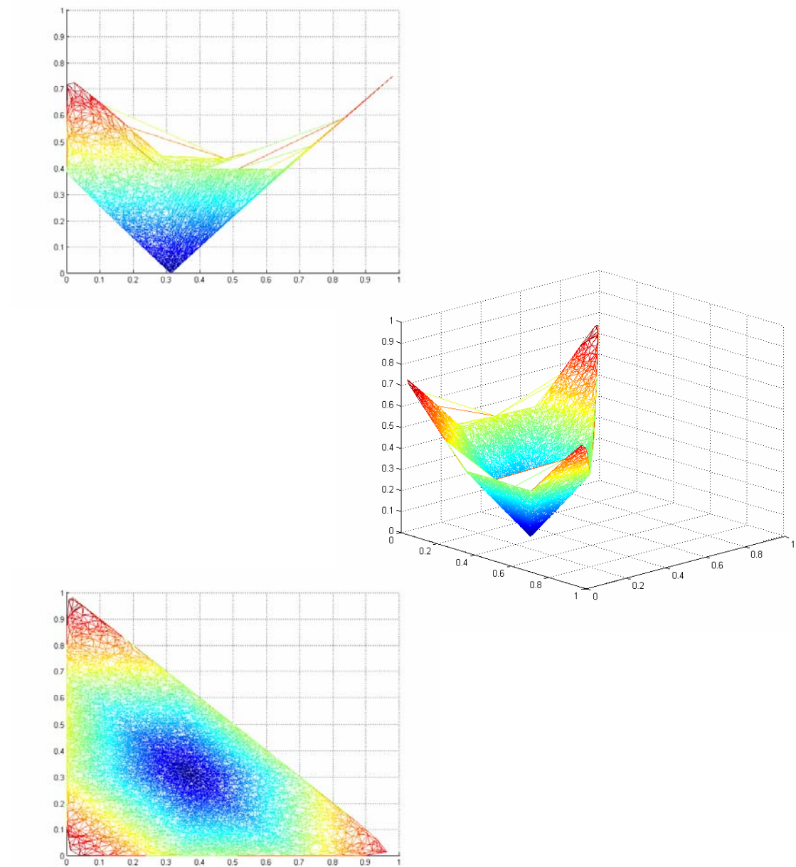
Figure 6-1: A side, top, and angled perspective of 10,000 experiments of the branching distributed between three circles using E to measure incoherency.
