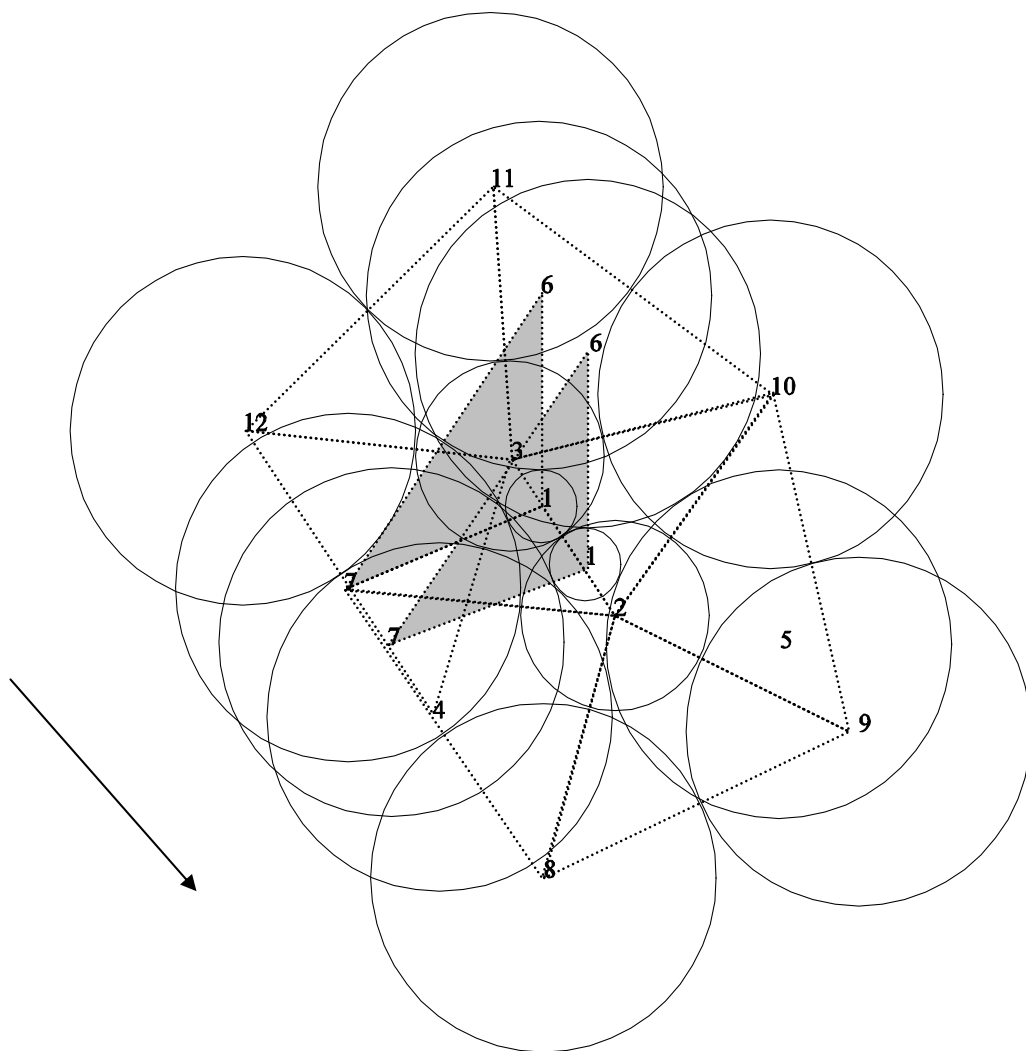
Figure 3-4: Laying down the faces in the closed chain illustrated in Figure 3-2, a holonomy is constructed. The shaded face, f_0 , is the first face of the chain and placed in two different locations. Clearly, this motif is incoherent.
