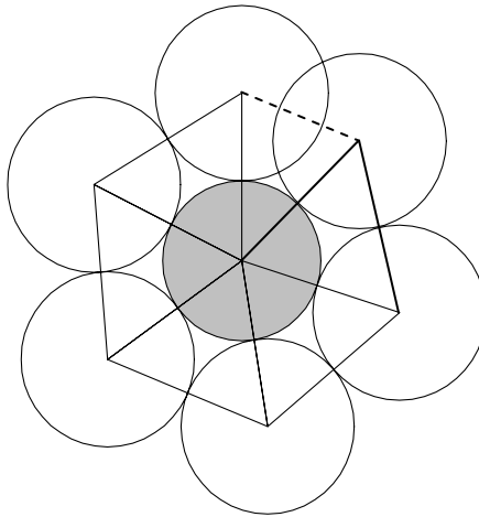
Figure 2-2: The shaded circle has been branched with an angle sum of 2.1\pi
