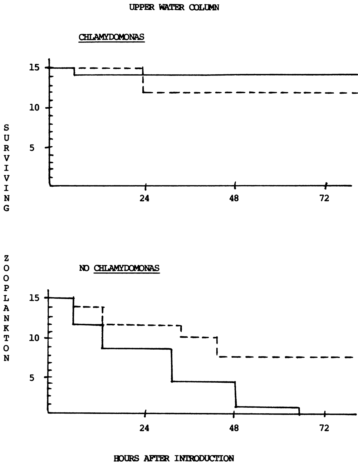
Figure 11. Survival of C. lacustris (—) and D. oregonensis (— —) in supplemented and unsupplemented whole lakewater from Arco's upper 2 m.
