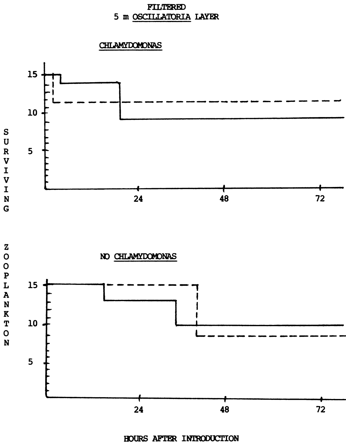
Figure 13. Survival of C. lacustris (—) and D. oregonensis (- -) in supplemented and unsupplemented filtered lakewater from Arco's 5 m Oscillatoria layer.
