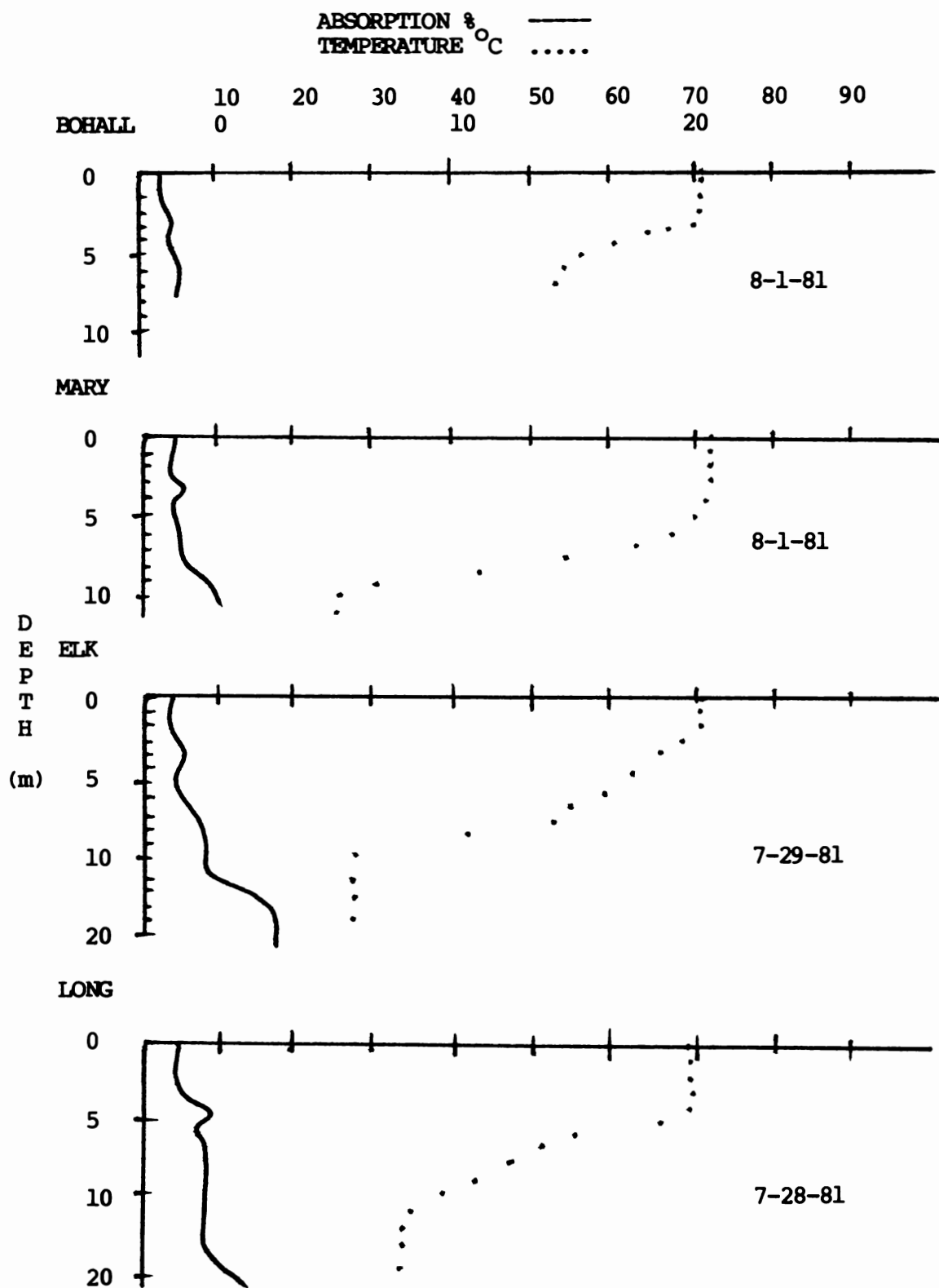
Figure 6. Optical density and temperature profiles of the non- Oscillatoria lakes.
