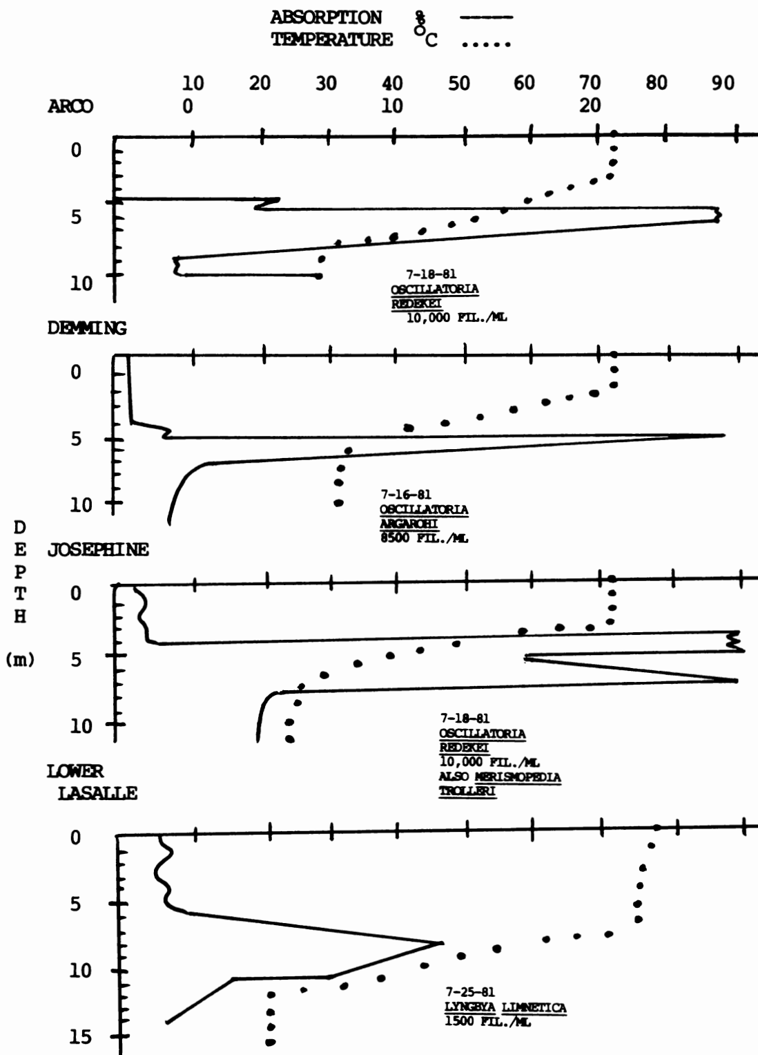
Figure 5. Optical density profiles, identification of Oscillatoria to species, and estimates of filament densities for the stratified Oscillatoria lakes.
