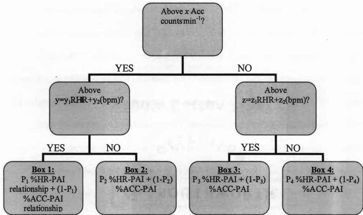
Figure 1. Equation structure for the combination of accelerometry (ACC) and heart rate (HR). All HR values are absolute HR minus resting HR (RHR). All physical activity intensity (PAI) relationships are determined by calibration. Therefore, this study has 2 equation complexes, depending on whether individual or group calibration is used. The equation complexes translate minute-by-minute data into PAI as follows. If Computer Science and Applications (CSA) value is above x , we use box 1 (with P_1 ) if the HR value is above y ; otherwise we use box 2 (with P_2 ). Similarly, if the CSA value is \leq x , we use box 3 (with P_3 ) if the HR value is above z ; otherwise we use box 4 (with P_4 ). Physical activity energy expenditure (PAEE) is obtained by integrating PAI with respect to time. The parameters x , y_{1-2} , z_{1-2} , and P_{1-4} are either assumed a priori or can be estimated post hoc by simulation of all possible models, while the standard error between predicted and measured PAEE is minimized. Reprinted from Brage et al (8).
