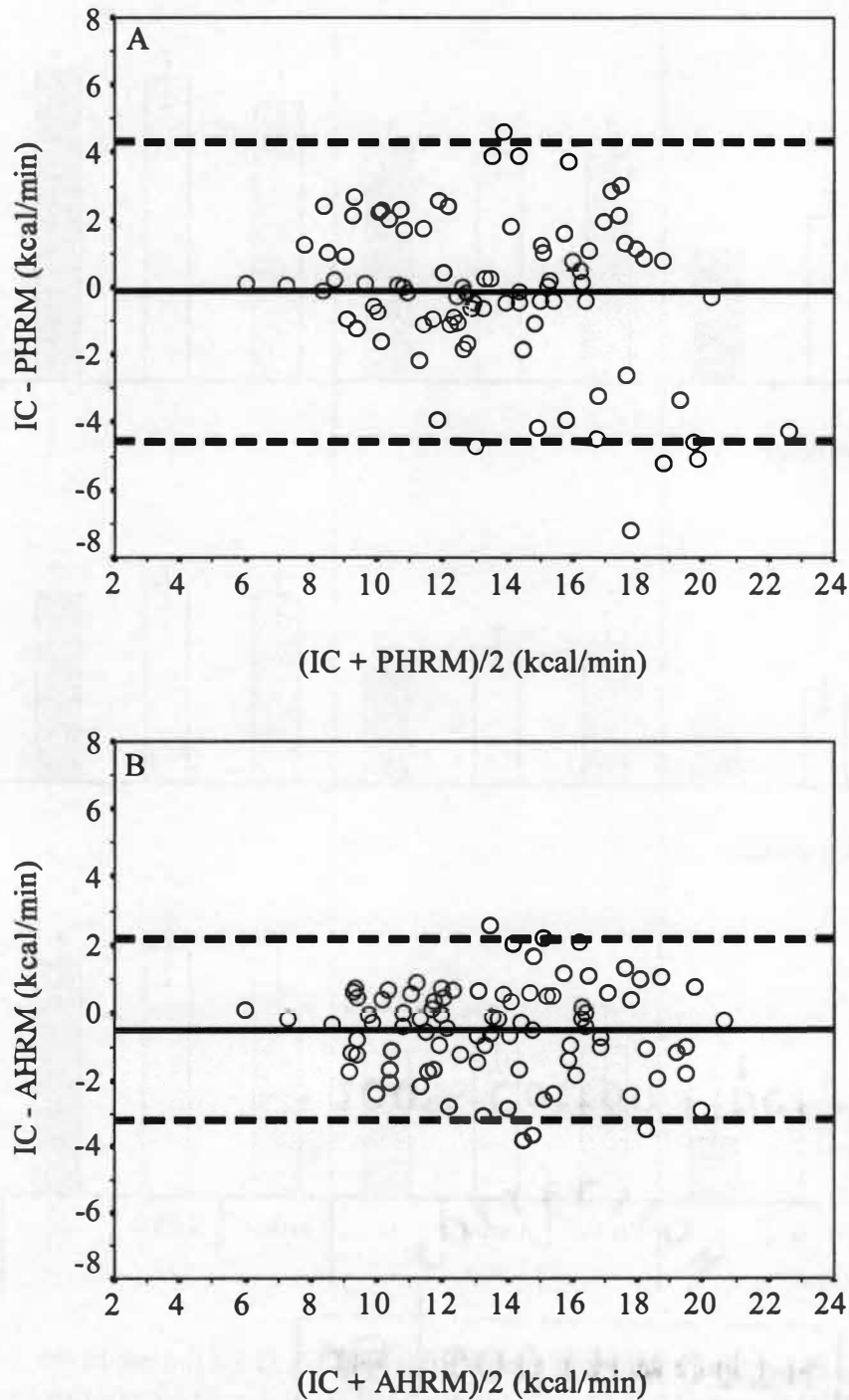
Figure 2. Bland-Altman plots depicting error scores (indirect calorimetry (IC) – device) for each watch in males: (A) Heart rate monitor with the predicted \text{VO}_{2\text{max}} and \text{HR}_{\text{max}} (PHRM), and (B) the heart rate monitor with the actual values (AHRM). Solid line represents mean difference; dashed lines represent 95% prediction intervals.
