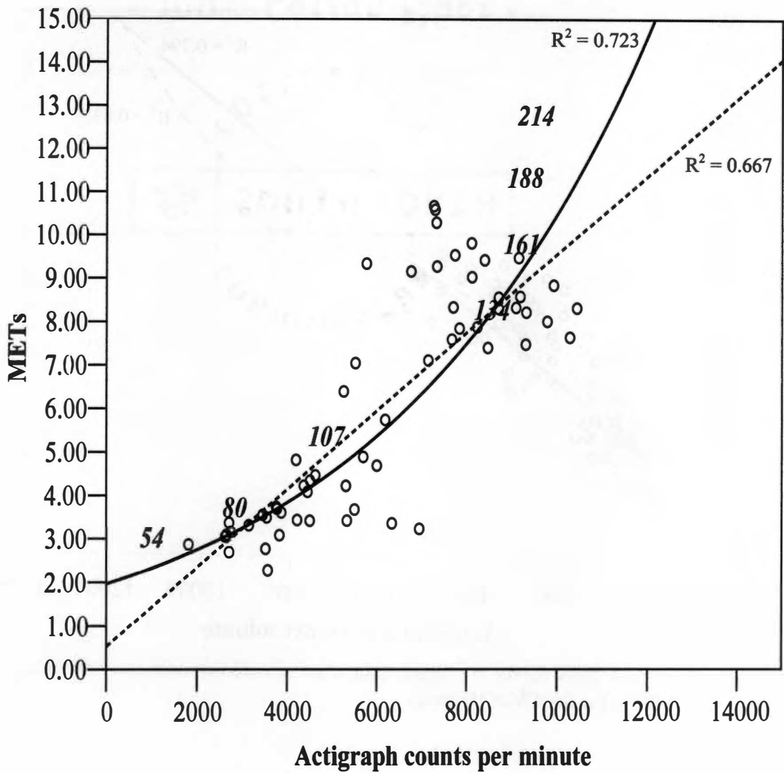
Figure 2. Regression lines for the Actigraph counts·min -1 versus measured energy expenditure (METs) for the CV ≤ 10 group. Numbers on graph represent mean data (N = 10) from King et al. (10).
