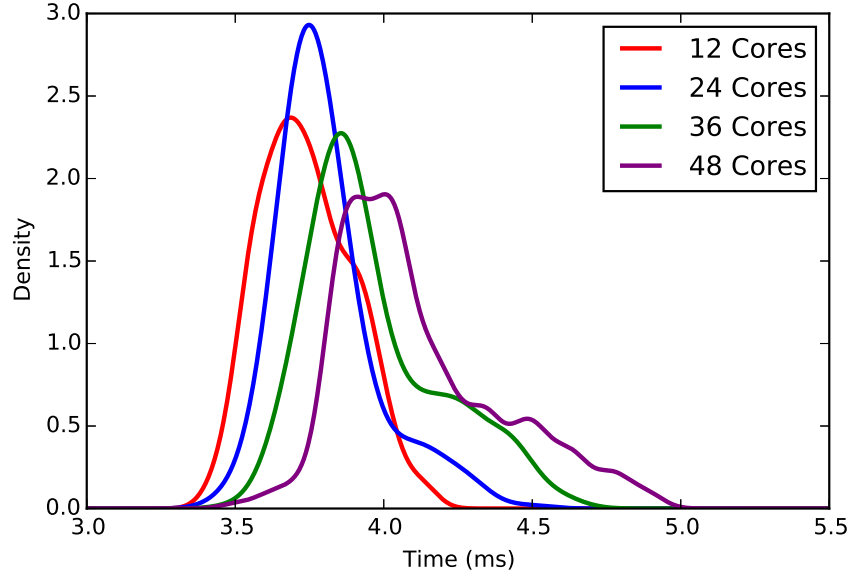
Figure 4.6: Kernel Density Estimation curves for DORMQR tasks
