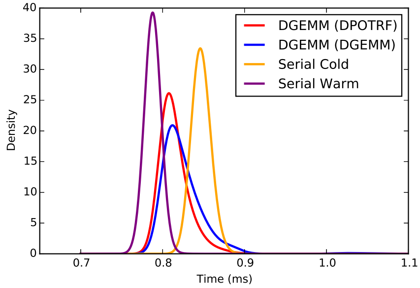
Figure 3.1: Kernel Density Estimation curves for DGEMM including serial benchmark data sets. 2 x 8 Core Intel Xeon E5-2690
