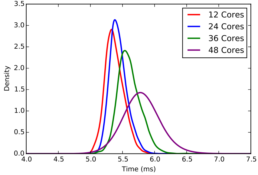
Figure 4.8: Kernel Density Estimation curves for DTSMQR tasks
