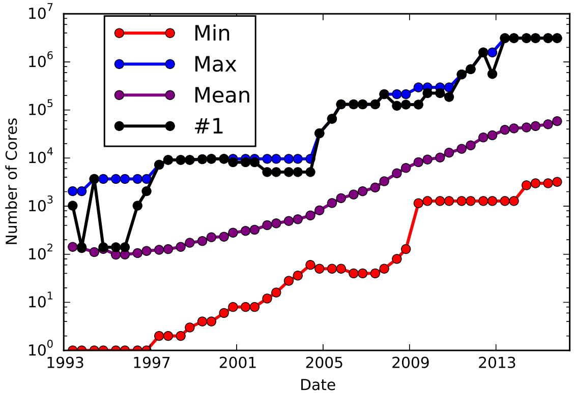
Figure 2.3: The number of cores on the Top 500 supercomputer list begins to dramatically accelerate around 2005.
