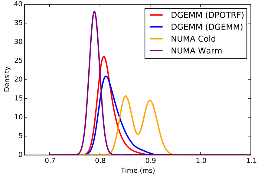
Figure 3.3: Kernel Density Estimation curves for DGEMM including NUMA benchmark data sets. 2 x 8 Core Intel Xeon E5-2690
