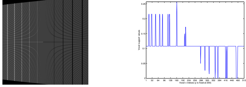
Figure 2.12: Left: Transaxial slice 80 of the line intersection based system matrix column sums corresponding to view angle zero and using the four corners of each detector element as the projection ray terminal points. Right: Line profile with y = 200 .
