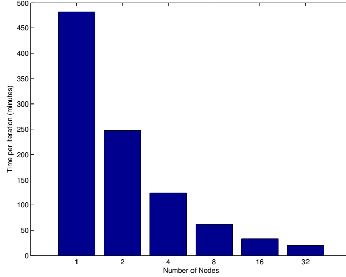
Figure 5.1: Run-times for the first iteration of SIRT using varying numbers of nodes.
