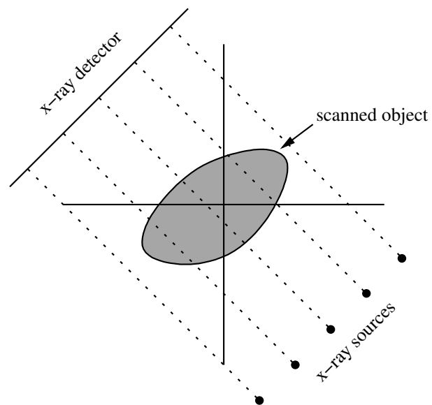
Figure 1.1: Parallel-beam scanner geometry.
