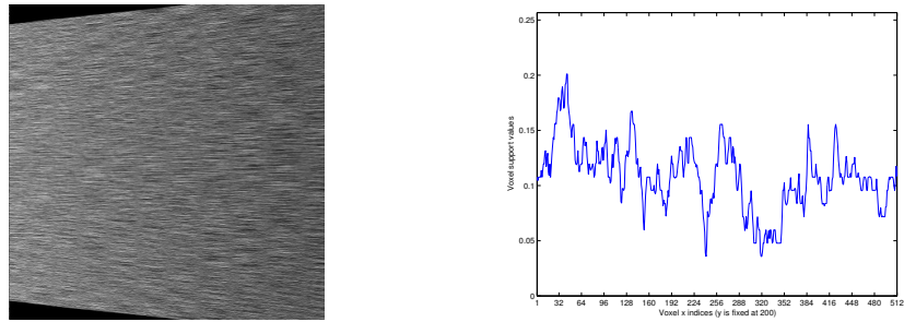
Figure 2.14: Left: Transaxial slice 80 of the line intersection based system matrix column sums corresponding to view angle zero and using nine random points per detector element as the projection ray terminal points. Right: Line profile with y = 200 .
