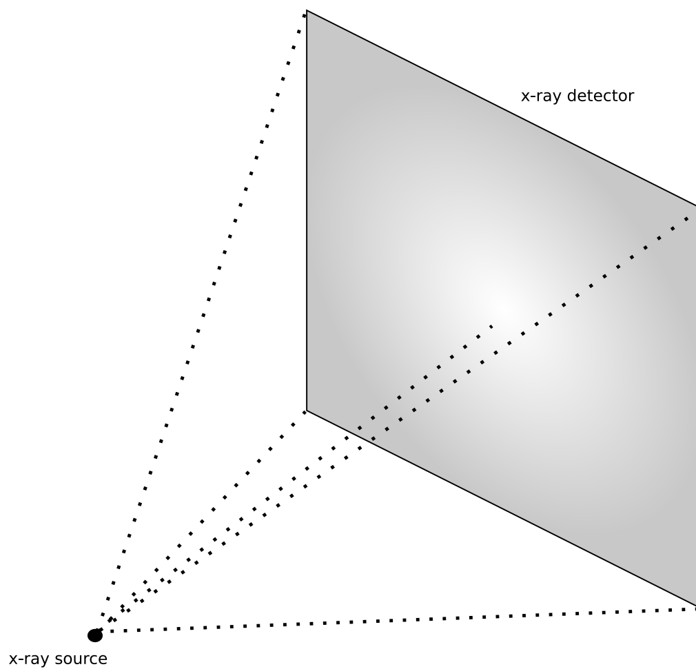
Figure 1.3: Cone-beam scanner geometry.
