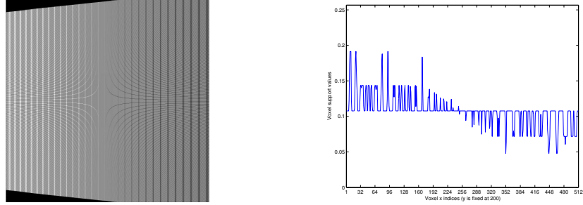
Figure 2.13: Left: Transaxial slice 80 of the line intersection based system matrix column sums corresponding to view angle zero and using nine equally distanced points per detector element as the projection ray terminal points. Right: Line profile with y = 200 .
