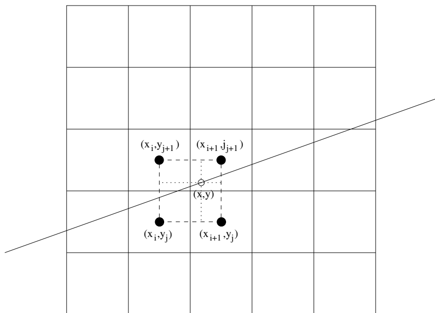
Figure 2.15: Depiction of the process of bilinear interpolation.
