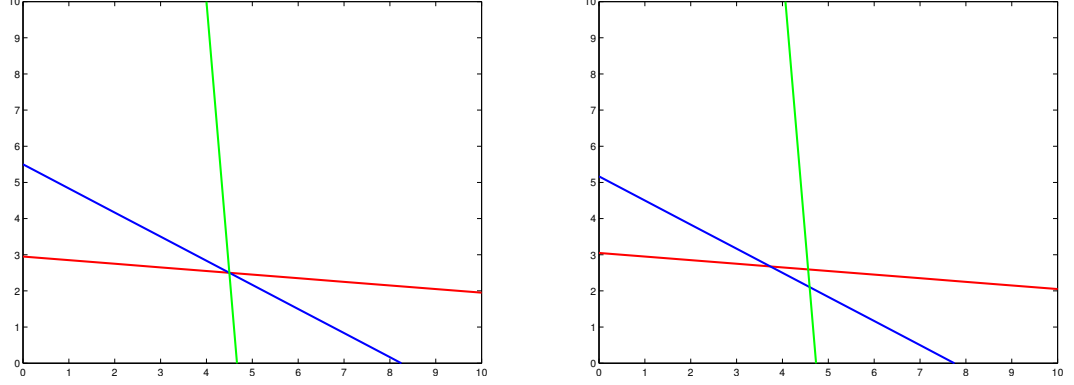
Figure 3.1: Graphs of the lines defined by the linear system examples. The left system has a unique solution where all three lines intersect while the right system has no unique solution.
