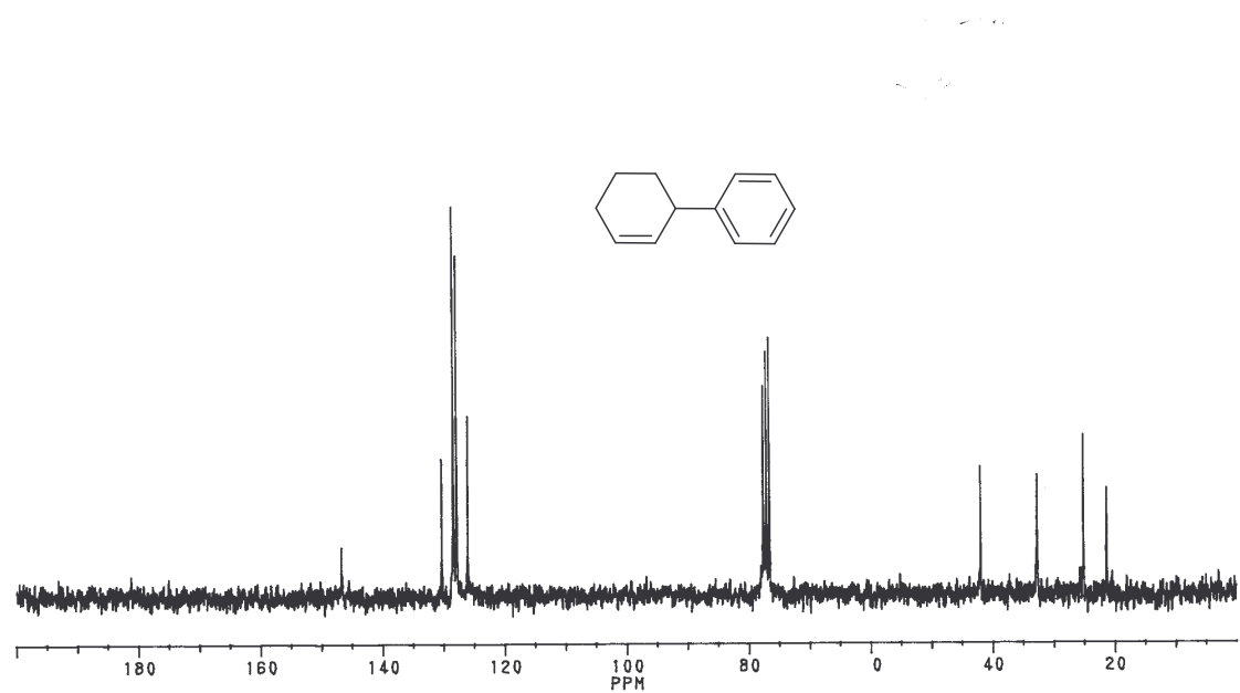
62.5 MHz ^{13}\text{C} NMR of compound 2-209
