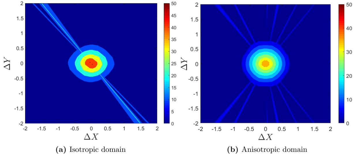
Figure 43: Spatial covariance function for strength field S_N , \text{cov}_{\mathbf{X}_N}
