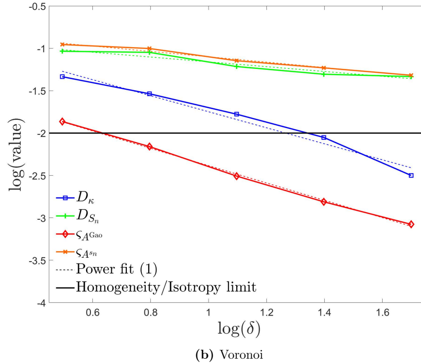
Figure 62: Convergence of SVEs to RVE size for elastic and fracture properties for regular and Voronoi SVEs.
