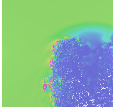
(e) t = 289.2 \mu s , (20.95 MPa), Before Material Failure
