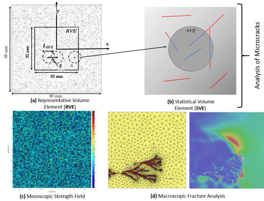
Figure 1: A multi-scale model for fracture analysis of microcracked rock.
