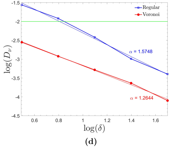
Figure 55: Convergence of VE size to \Delta^{\mathcal{C}_f} for elastic properties \kappa , G , E , and \nu .
