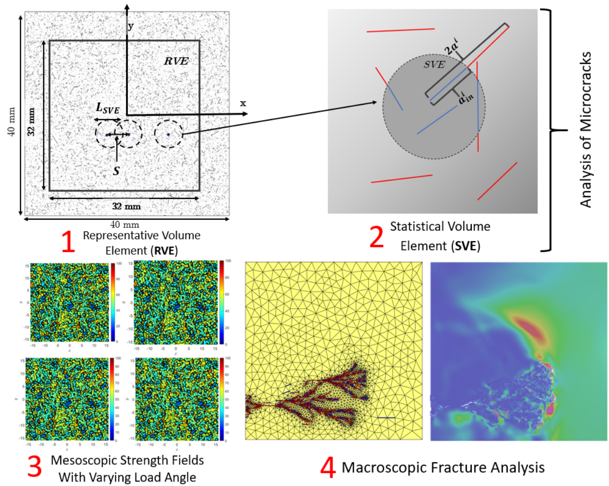
Figure 29: A multi-scale model for anisotropic fracture analysis of microcracked rock.
