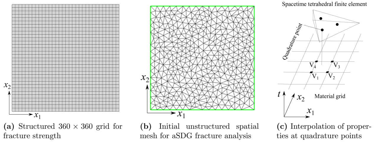
Figure 15: Distinct discrete grids for material properties and fracture analysis.
