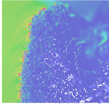
(h) t = 291.2 \mu s , (7.29 MPa), Before Material Failure
