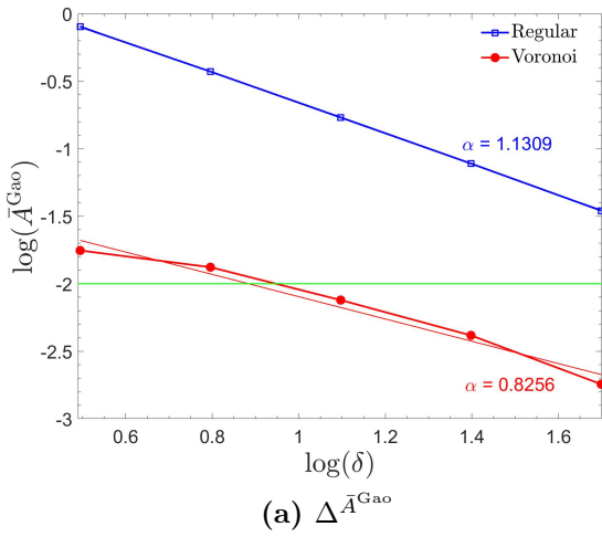
Figure 57: Convergence of VE size to \Delta^{\bar{A}^{\text{Gao}}} and \Delta^{D_{A^{\text{Gao}}}} for elastic anisotropy measure A^{\text{Gao}} .
