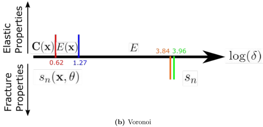
Figure 63: Summary of Convergence to the Homogeneous and Isotropic \Delta limits for regular and Voronoi SVE types. Regular SVEs converge slowly from inhomogeneous/anisotropic \mathbf{C}(\mathbf{x}) elastic field to anisotropic/homogeneous \mathbf{C} before reaching ideal homogeneous/isotropic E , while fracture remains inhomogeneous/anisotropic throughout. Voronoi converges faster from \mathbf{C}(\mathbf{x}) to inhomogeneous elastic modulus E(\mathbf{x}) . For all reasonable sizes \delta strength remains inhomogeneous/anisotropic even for Voronoi. Figure colors match the given properties in Figure 62.
