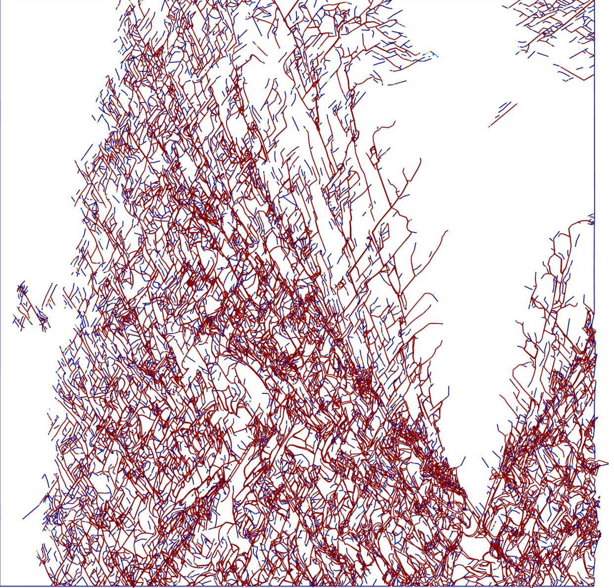
Figure 28: aSDG deformed shape for the compressive loading example at t = 292.0 \mu s
