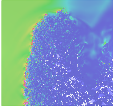
(g) t = 290.8 \mu s , (13.50 MPa), Before Material Failure
