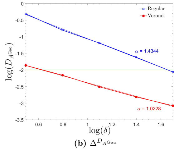
Figure 57: Convergence of VE size to \Delta^{\bar{A}^{\text{Gao}}} and \Delta^{D_{A^{\text{Gao}}}} for elastic anisotropy measure A^{\text{Gao}} .
