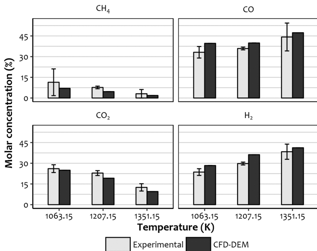
Figure 6.7. Comparison between the predicted and experiment concentration of \text{H}_2 , \text{CO} , \text{CO}_2 , and \text{CH}_4 as affected by gasification temperature. Error bar indicates 95% confidence interval.
