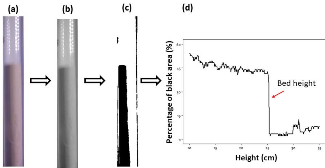
Figure 5.2. Image analysis in R programming (a) original and input bed image in full color, (b) bed image in greyscale, (c) bed image converted to white and black, and (d) graphical representation of color gradient in the bed image to identify bed height.
