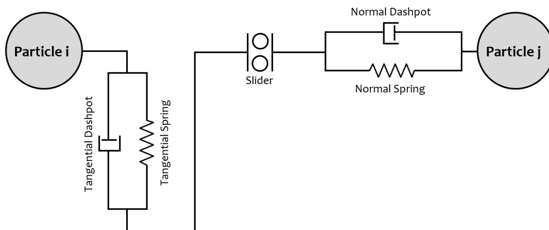
Figure 2.5. Hertz-Mindlin particle contact model.
