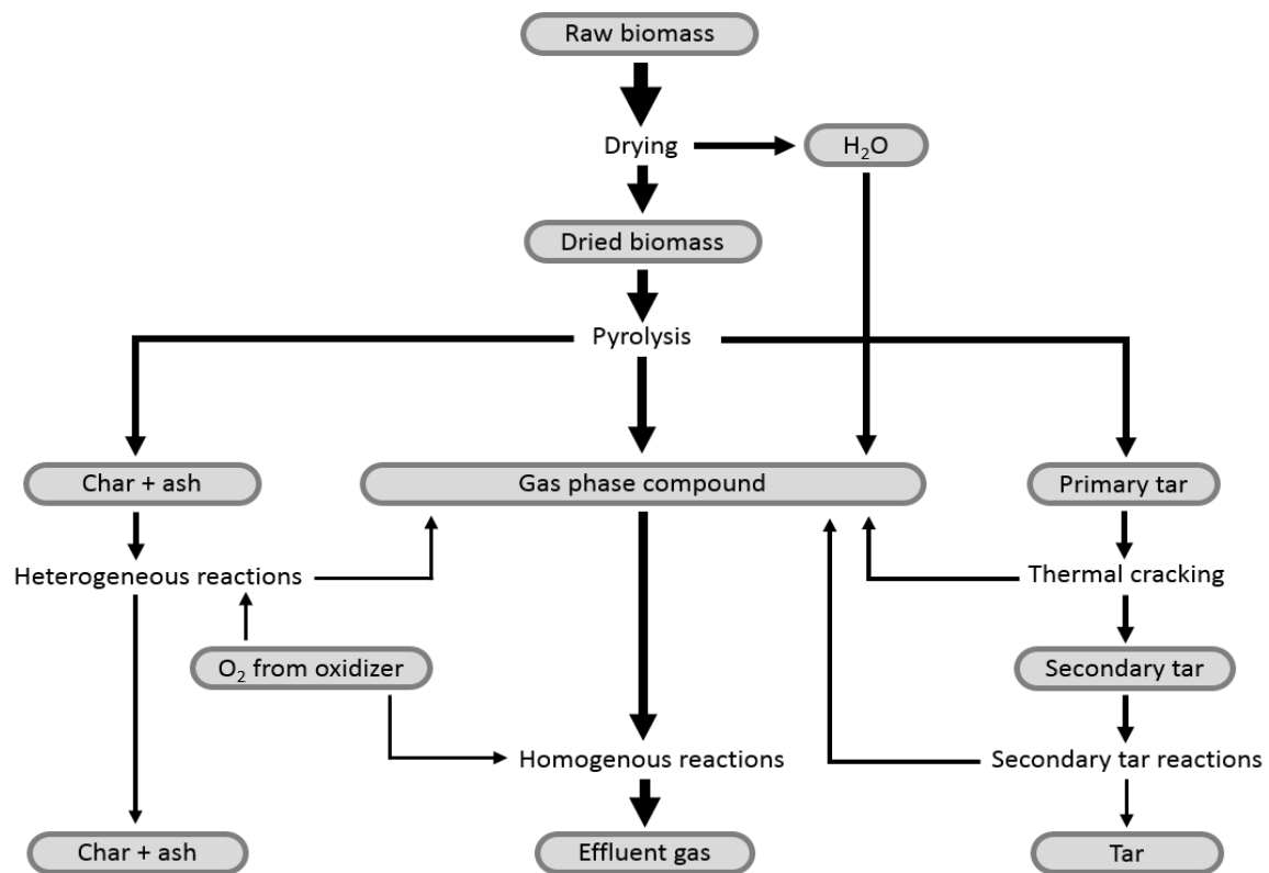
Figure 2.1. A conventional biomass gasification process. The arrow weight qualitatively depicts the mass fraction of intermediate and final products.
