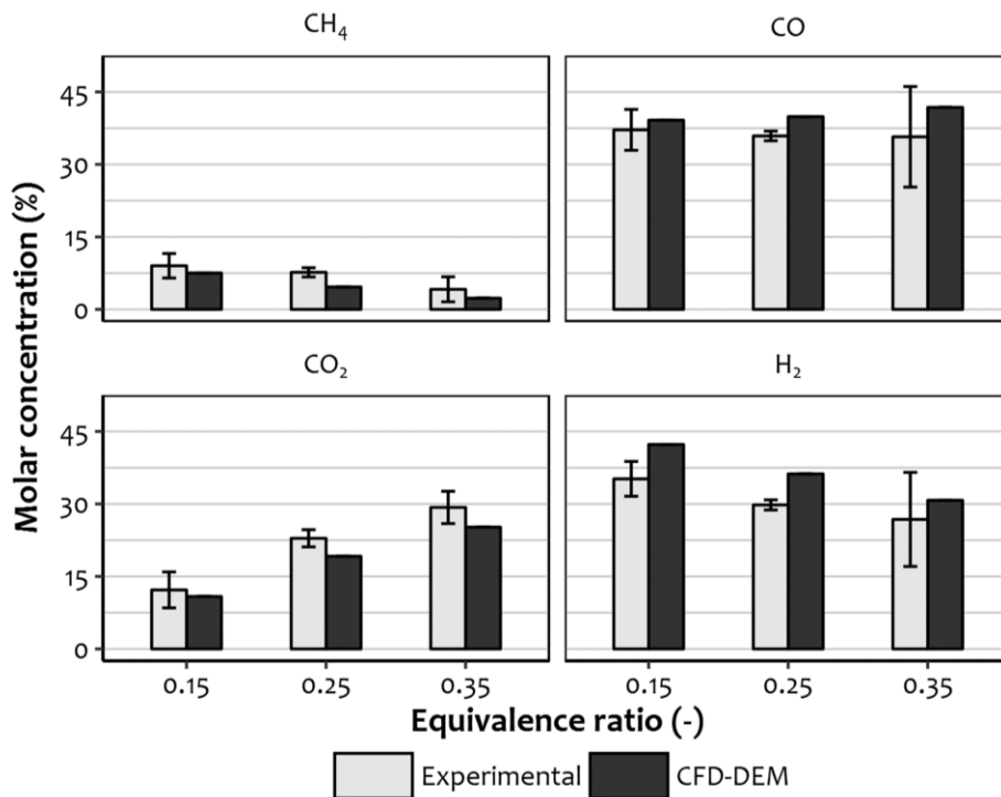
Figure 6.8. Comparison between the predicted and experiment concentration of \text{H}_2 , CO, \text{CO}_2 , and \text{CH}_4 as affected by equivalence ratio. Error bar indicates 95% confidence interval.
