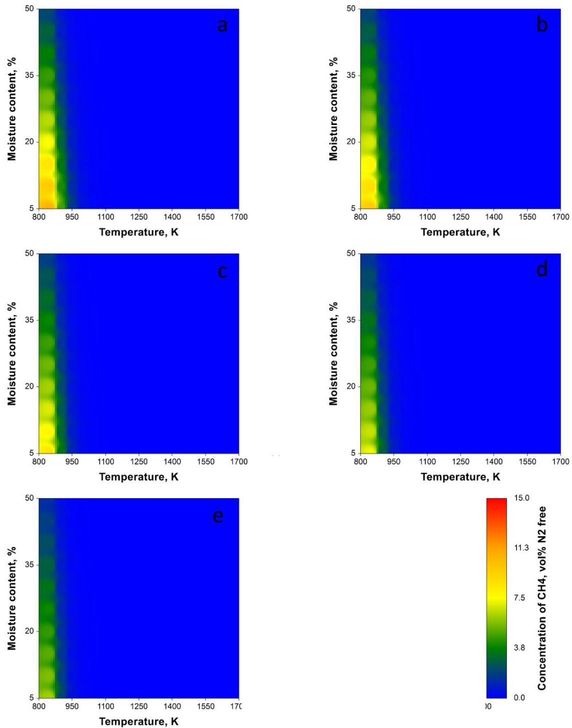
Figure 4.6. Effects of temperature, moisture content, and equivalence ratio on \text{CH}_4 concentration. a) ER = 0.20, b) ER = 0.25, c) ER = 0.30, d) ER = 0.35, and e) ER = 0.40. Values are reported on a % vol/vol dry, \text{N}_2 -free basis.
