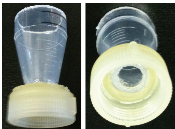
Figure 1 Custom-built 13 mm filter funnel. Funnel was assembled from a Swinnex® inlet bonded to the conical end of a 15 ml polypropylene tube.
