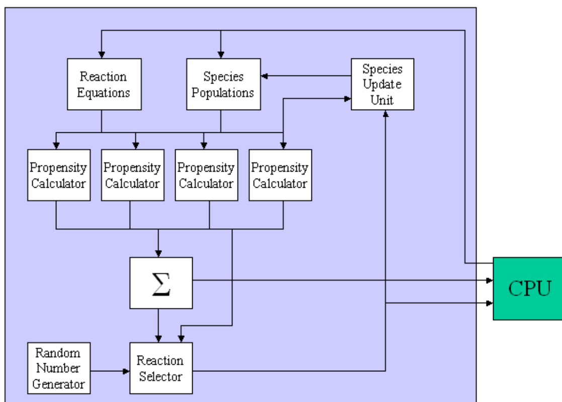
Figure 31. Block Diagram of the Original Hardware Design.
