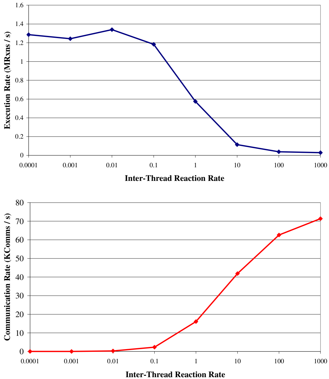
Figure 26. Parallel Execution and Communication Rates. Measurements of simulation speed and communication rate for the artificial model with varying inter-thread reaction rate constants.
