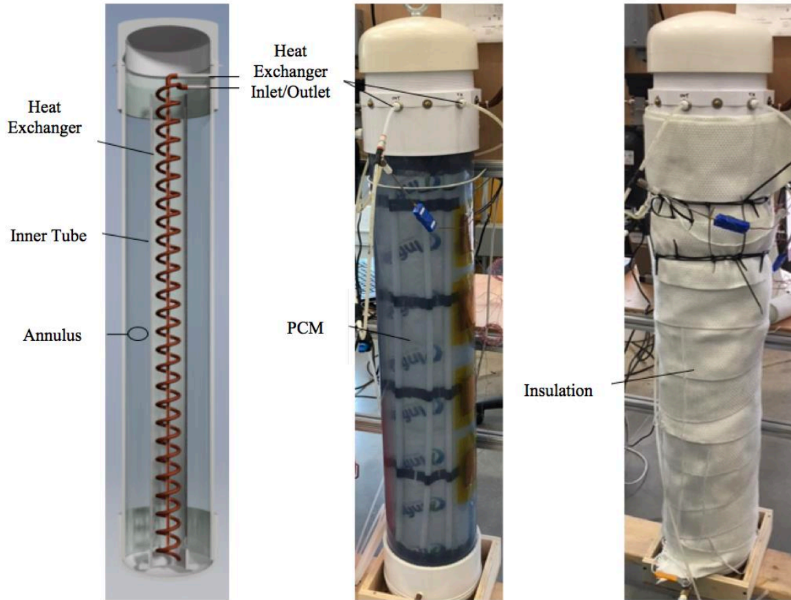
Figure 5. UTB prototype 3-D rendering (left) and actual prototype (center) and insulated prototype (right).
