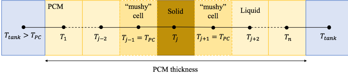
Figure 21. Diagram of PCM domain during phase change process.
