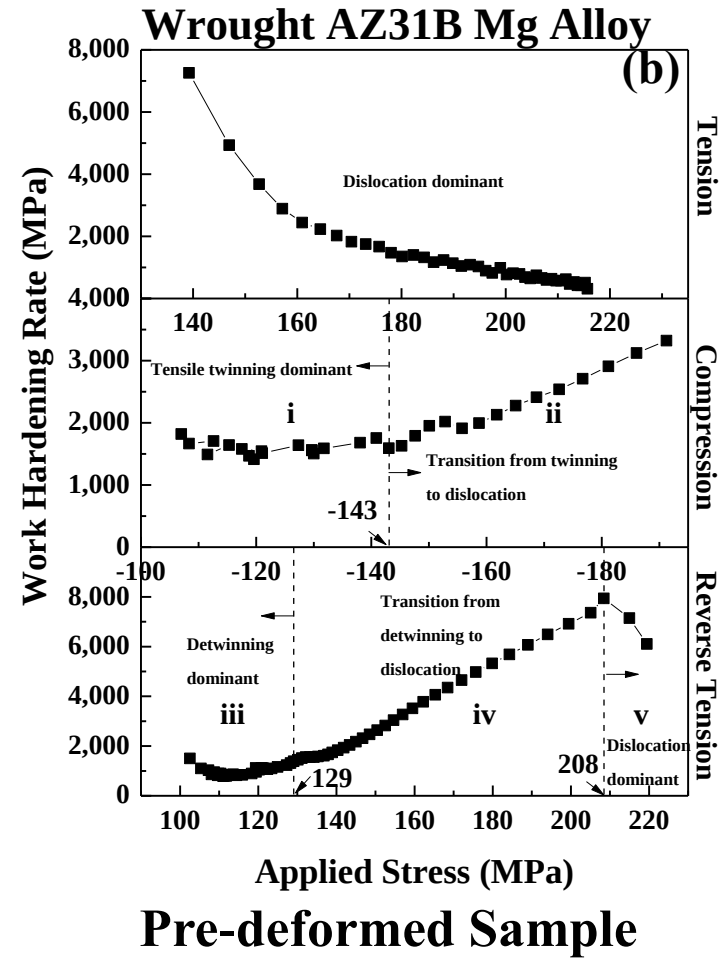
Figure 4.2 The work-hardening rate as a function of stress during the strain-path changes for: (a) the as-received sample and (b) the pre-deformed sample. The stress ranges were divided based on the work-hardening rate changes, denoted by Roman numerals.
