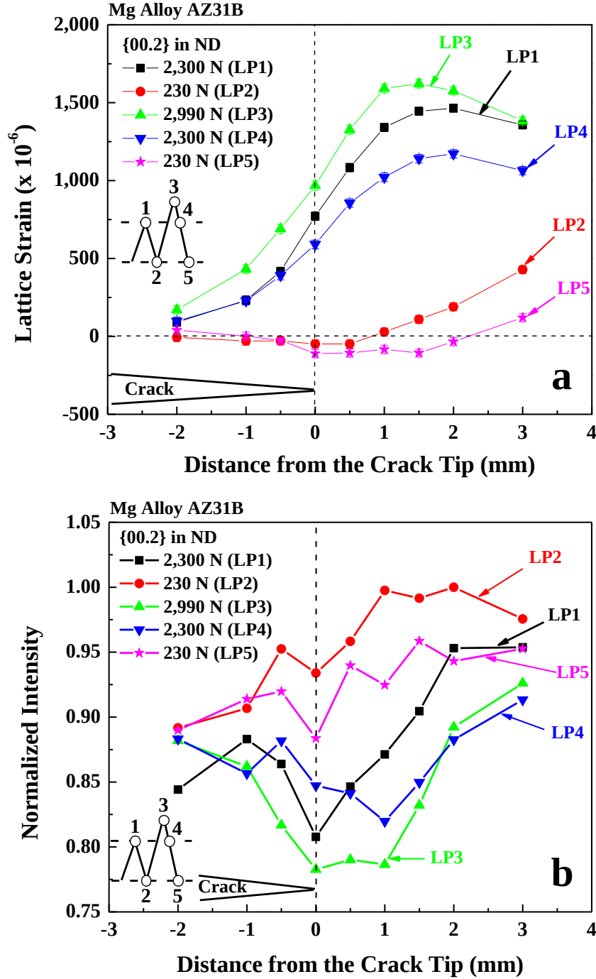
Figure 4.20 In-situ neutron-diffraction results obtained from the \{00.2\} reflection in bank 1: (a) lattice strain and (b) diffraction peak intensity evolution is measured at the five different loadings (marked with a blue circle, Fig. 3.4(d)) during loading-unloading cycles.
