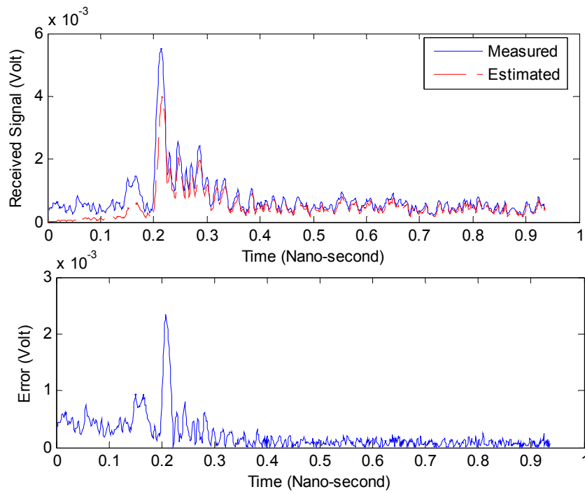
Figure.14 RLS measurement vs. estimation for the 1 st path
