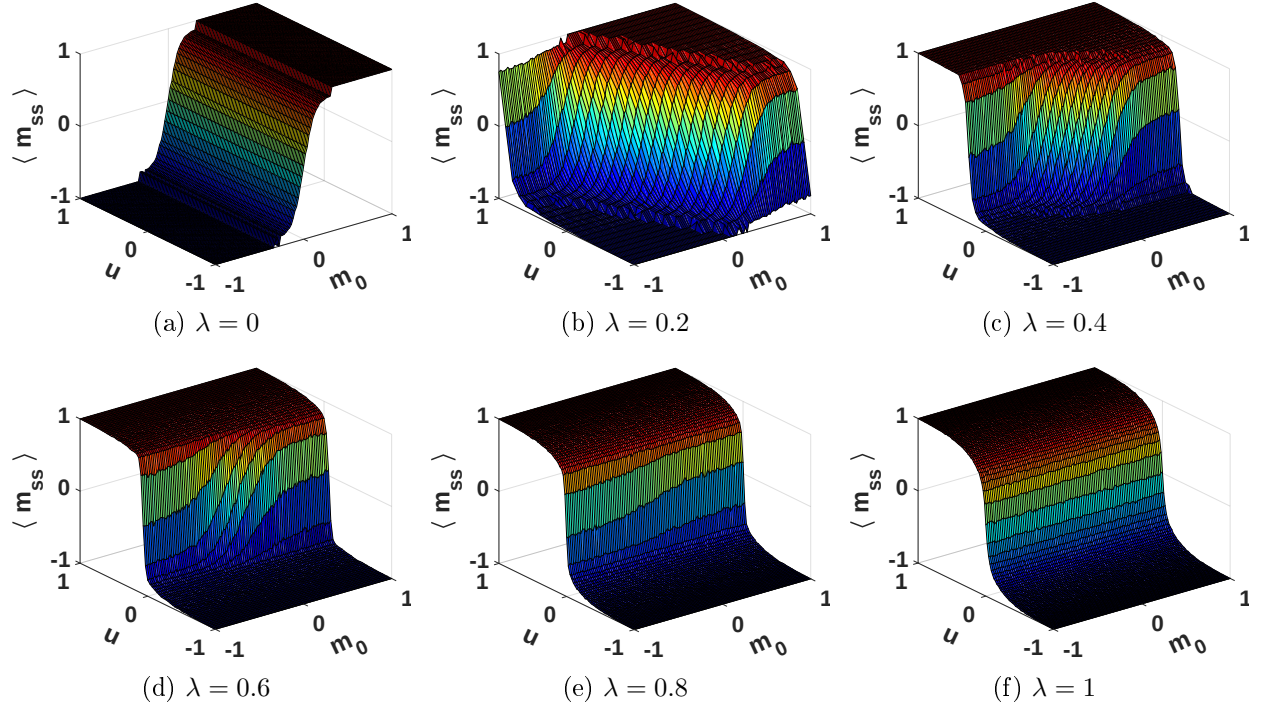
Figure 2.5: Dependency of mean steady state magnetization on initial magnetization and control input for N = 100 .
