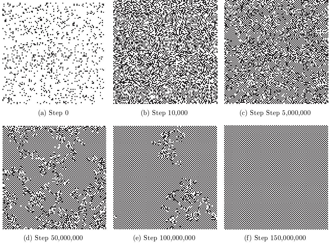
Figure 3.9: Opinion diffusion in a two-dimensional lattice
