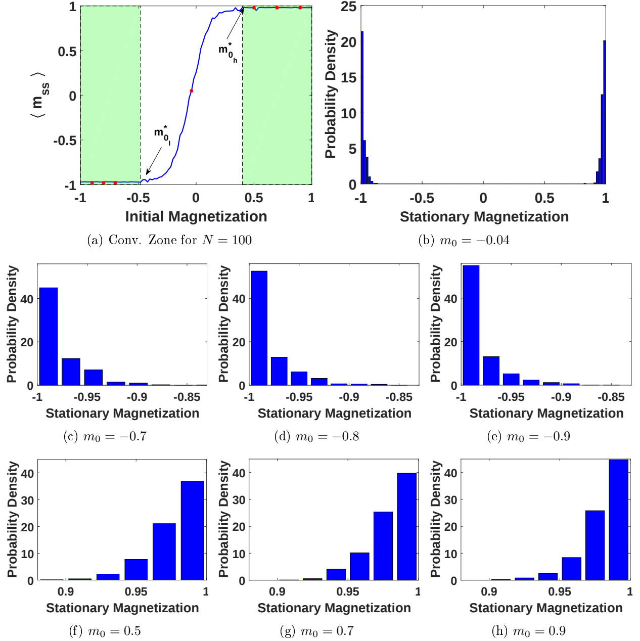
Figure 2.4: Conv. zone and stationary PDF's of a system with N = 100 , I_+ = 12 , I_- = 10 .
