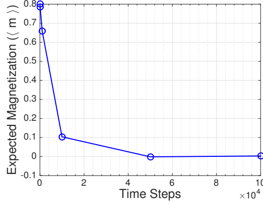
Figure 3.10: Magnetization versus time on the two-dimensional lattice
