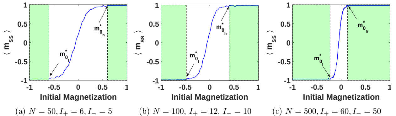
Figure 2.3: Dependency of the mean steady state magnetization on initial magnetization.
