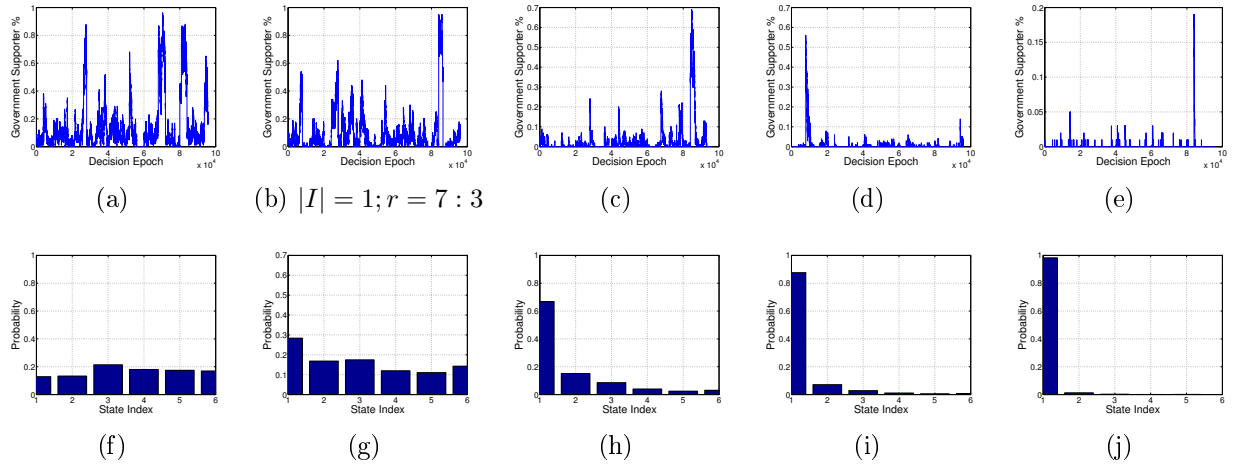
Figure B.4: Evolution of statistical patterns with increasing influence group size
