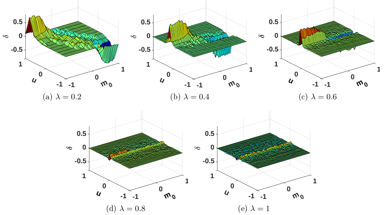
Figure 2.8: Scalability zone for all m_0 s for N = 100 .
