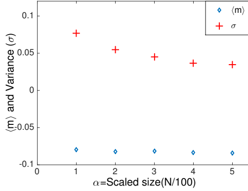
Figure 3.3: Effect of scale factor on the mean and variance of P_e(m)
