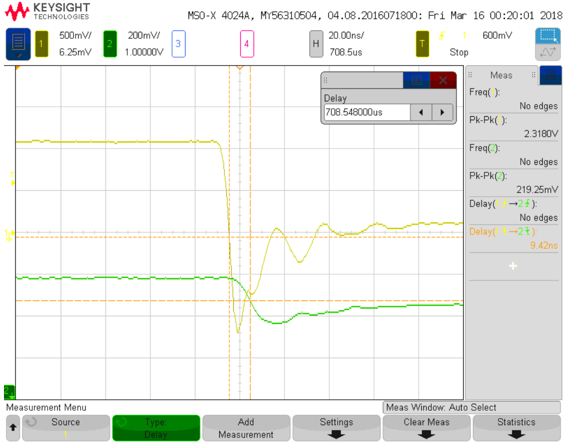
Figure 4.24: Sigmoid Measurement for Falling Edge Propagation Delay.
