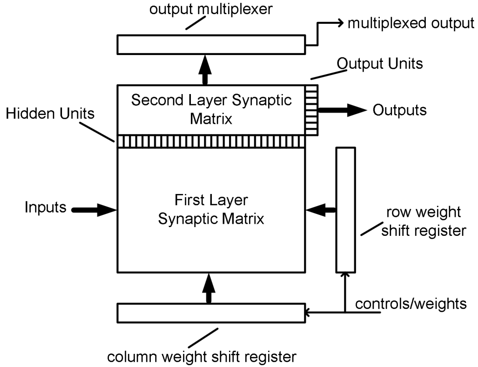
Figure 2.6: Block Diagram of MLP Constructed in [7].
