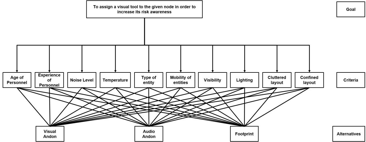
Figure 5.7: Hierarchical structure of visual tool assignment
