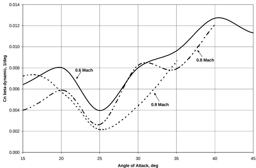
Figure 19 – Departure resistance of the two seat aircraft with the RECCE nose
