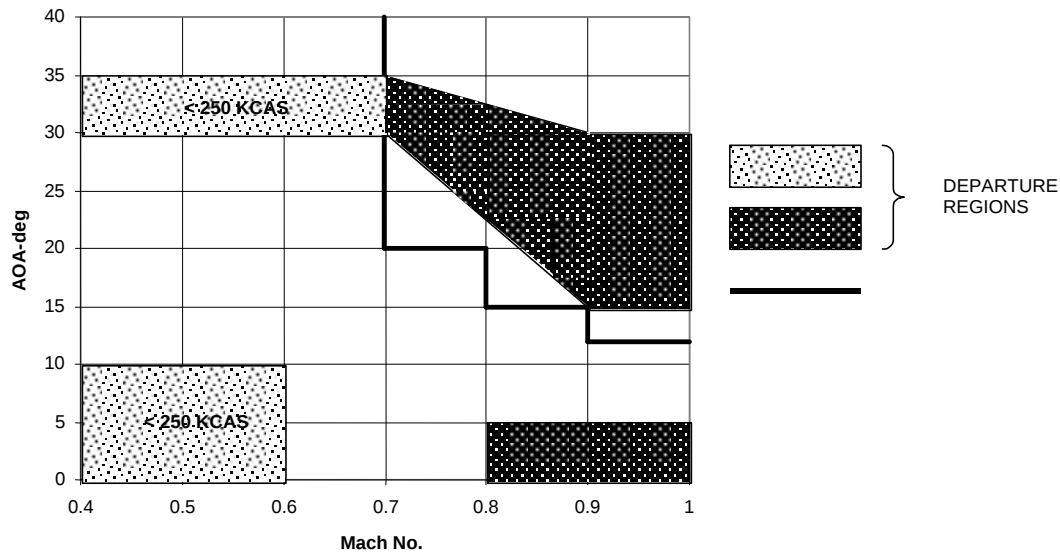
Figure 11 – F/A-18 Departure Susceptibility Regions (Two-Seat with Centerline Tank)
