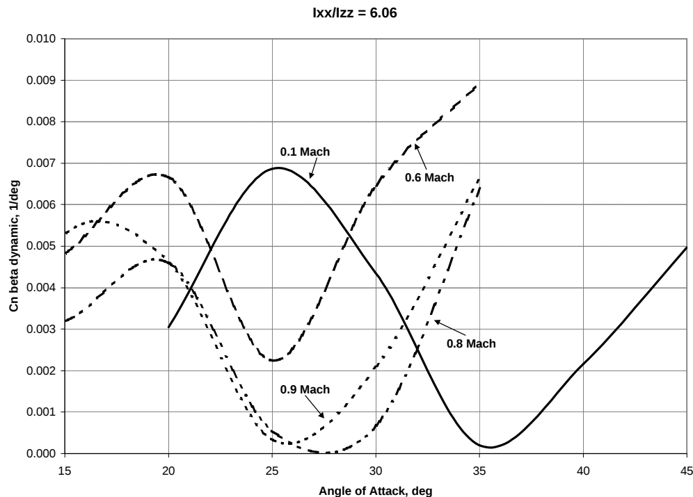
Figure 13 – Departure resistance of the two seat aircraft with centerline tank at various Mach numbers
