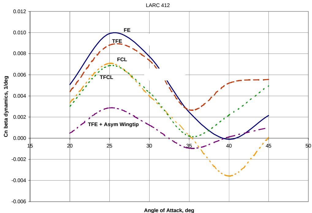
Figure 20 – Departure resistance summary at 0.1 Mach number
