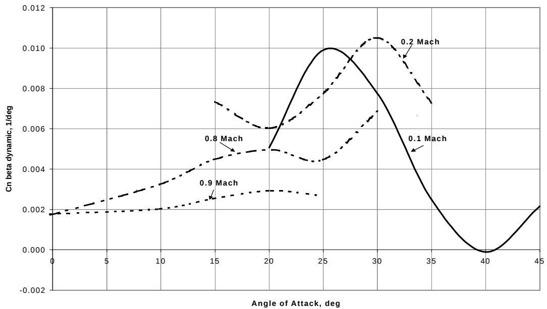
Figure 5 – F/A-18 Single Seat, Clean Departure Resistance (wind tunnel data)
