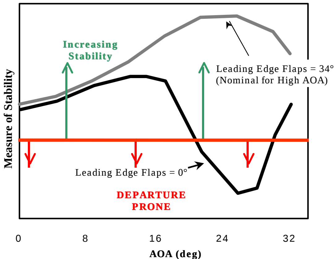
Figure 2 – Lateral-Directional stability levels with leading edge flap deflection
