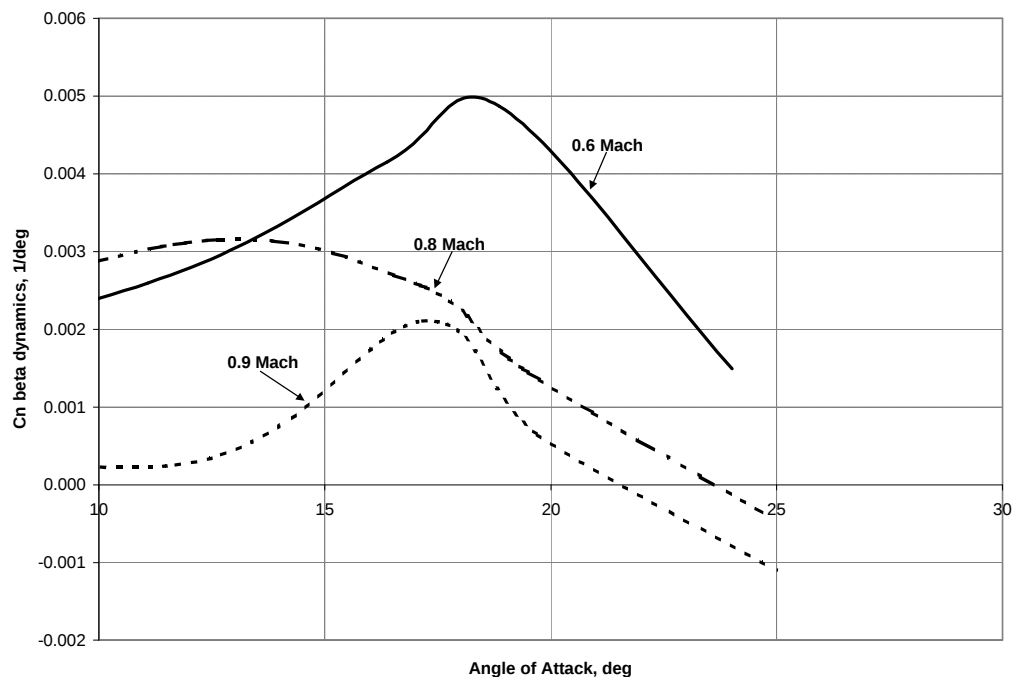
Figure 17 – Departure resistance with stores representing 17,000 ft-lbs asymmetry maneuvering flight in the high subsonic Mach number region and at approximately 15 deg AOA, roll and yaw departures are likely. Aggravated flight control inputs (cross control, forward corner, etc.) can lead to violent departures from controlled flight in this region.
