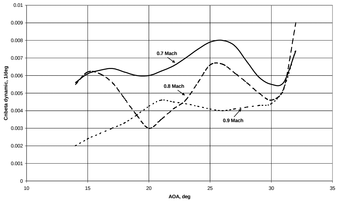
Figure 4 – F/A-18 Single Seat, Clean Departure Resistance (FSD flight test derived)
