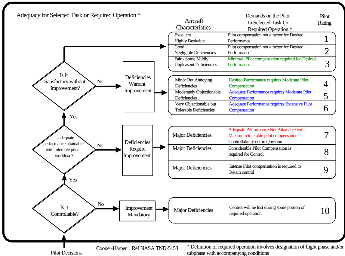
Figure C1 – Pilot Handling Qualities Rating Scale (HQRs)
