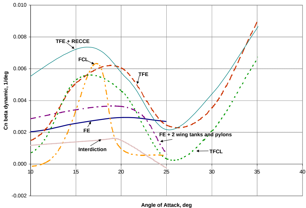
Figure 24 – Departure resistance summary at 0.9 Mach number
