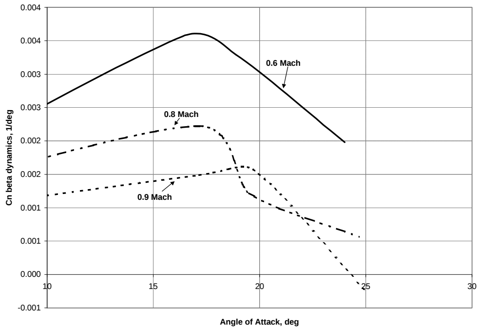
Figure 16 – Departure resistance of the single seat aircraft with Interdiction loading
