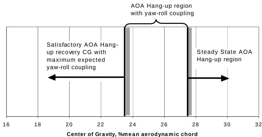
Figure 6 – Example of Center of Gravity Margin Placed on the Hornet due to AOA Hang-up (Fighter Escort with Centerline Tank)
