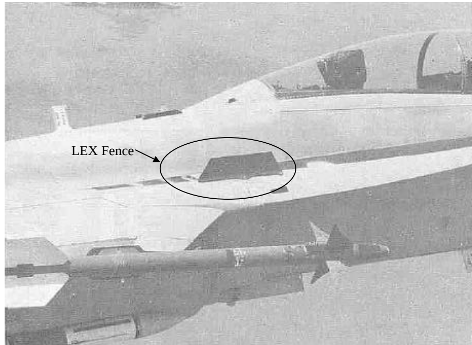
Figure 3 – Leading edge extension fence modification (ref 15)
