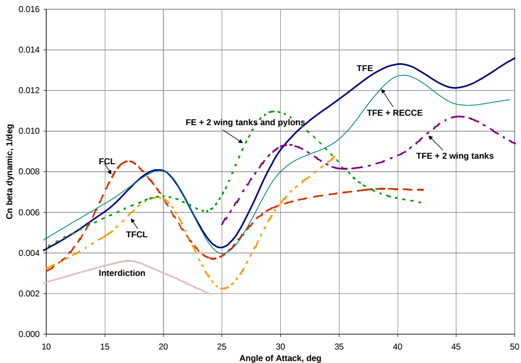
Figure 22 – Departure resistance summary at 0.6 Mach number
