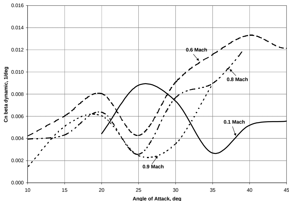
Figure 10 – Departure resistance of the two-seat Hornet at various Mach numbers
