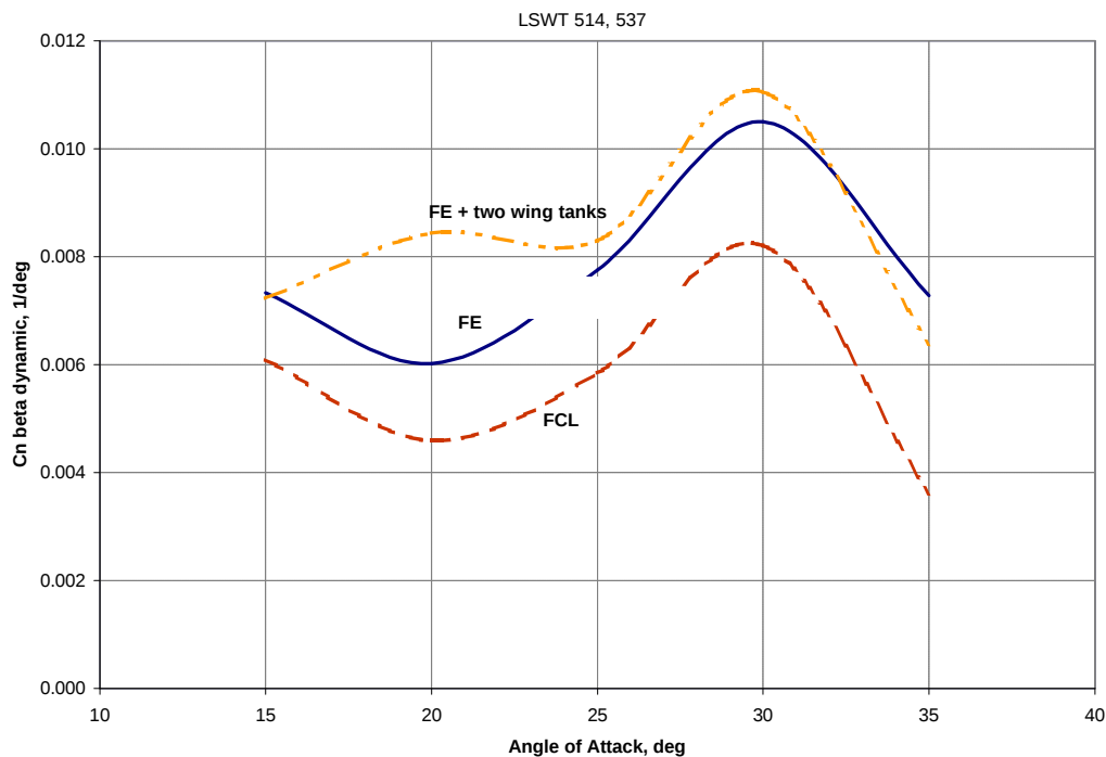
Figure 21 – Departure resistance summary at 0.2 Mach number
