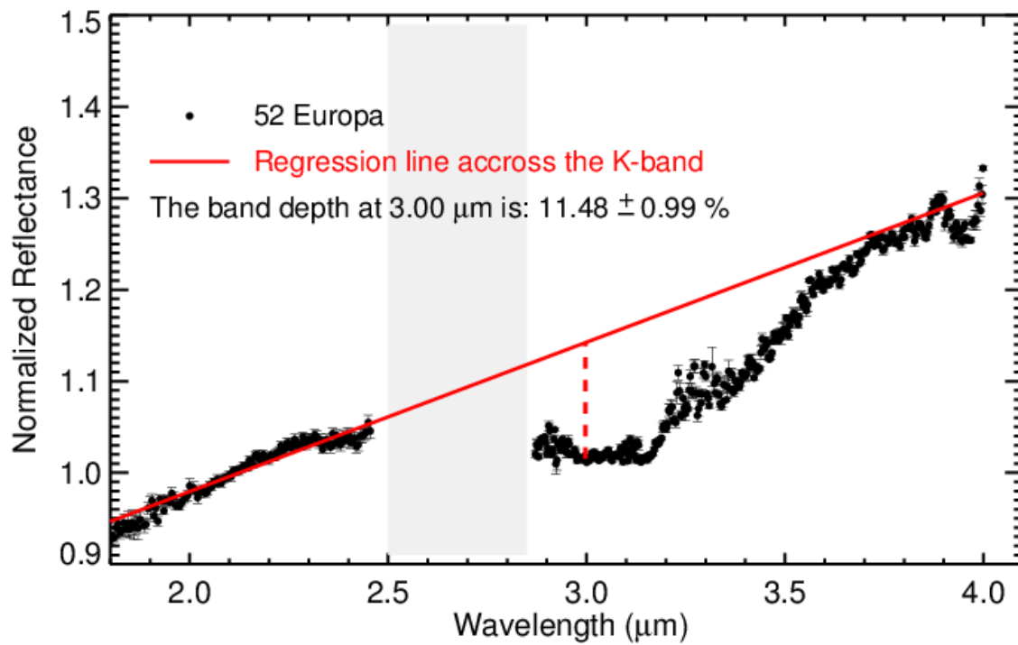
Figure A3. The band depth is calculated by using a regression line across the K-band of the spectrum of 52 Europa. The band depth at 3.00 \mu\text{m} is: 11.48 \pm 0.99 \% . The dashed line shows the band depth at 3.00 \mu\text{m} .
