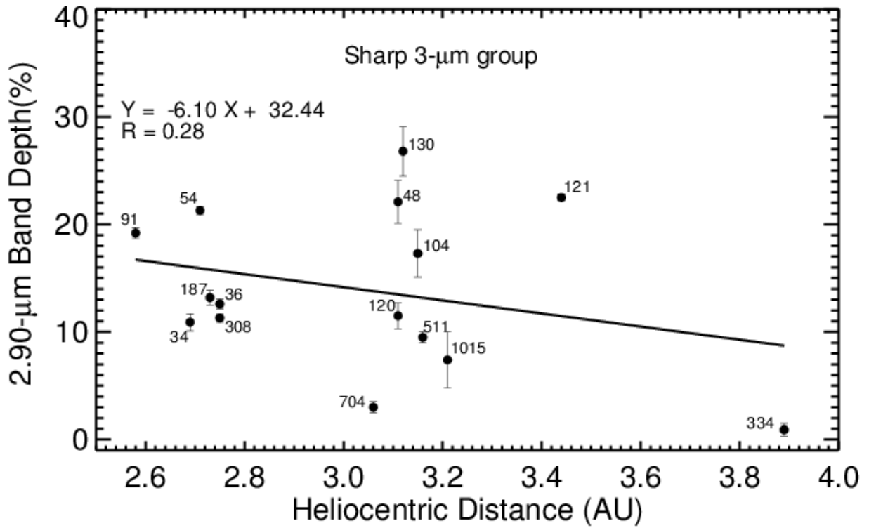
Figure A12. Heliocentric distance vs. the band depth at 2.90 \mu m for asteroids that exhibit the sharp OH 3- \mu m feature. The reflectance was calculated by fitting a linear regression line across the 2.85–3.25- \mu m region. 2.90- \mu m band depth decrease with the increase of the heliocentric distance. The R (linear-correlation coefficient) value of 0.28 corresponds to a probability of \sim 0.60 ( 1\sigma ) that the variables are correlated. If we exclude 121 Hermione and 130 Electra (binaries) from the plot, the R value would be 0.64, corresponding to a probability of \sim 0.95 ( 2\sigma ) that the variables are correlated. However, if we exclude 334 Chicago from the plot we would have a weaker correlation.
