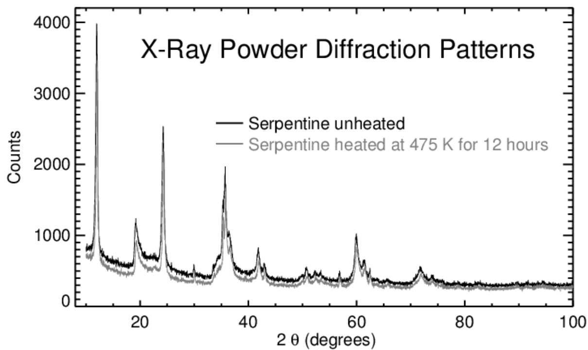
Figure B2. X-ray powder diffraction patterns of serpentine unheated (black) and heated at 475 K for 12 hours (gray). The similarity of the two diffraction patterns indicates that hydroxyl groups are not affected by modest heating.
