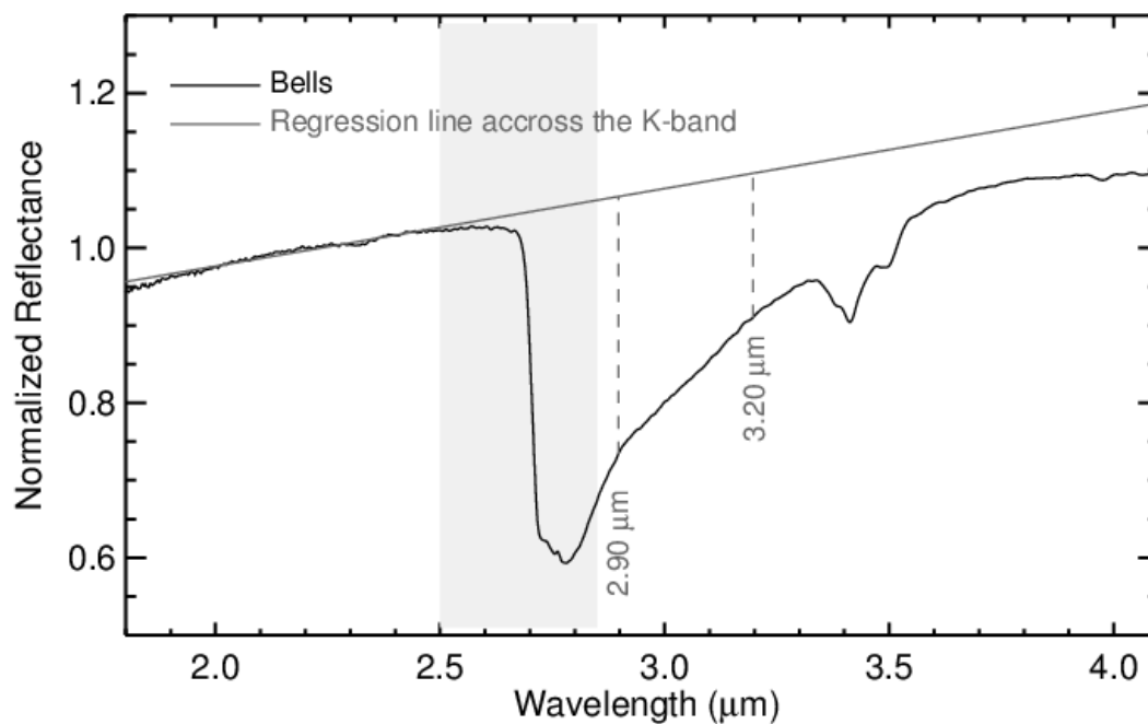
Figure C1. Near-infrared spectrum of the CM carbonaceous chondrite Bells, showing the 3-μm region. The solid gray line is the continuum that is defined as the regression line across the 1.95-2.50-μm region (k-band). The dashed lines show the band depths calculated at 2.90 μm and 3.20 μm, which were chosen as representative wavelengths to characterize the band shape of the 3-μm band.
