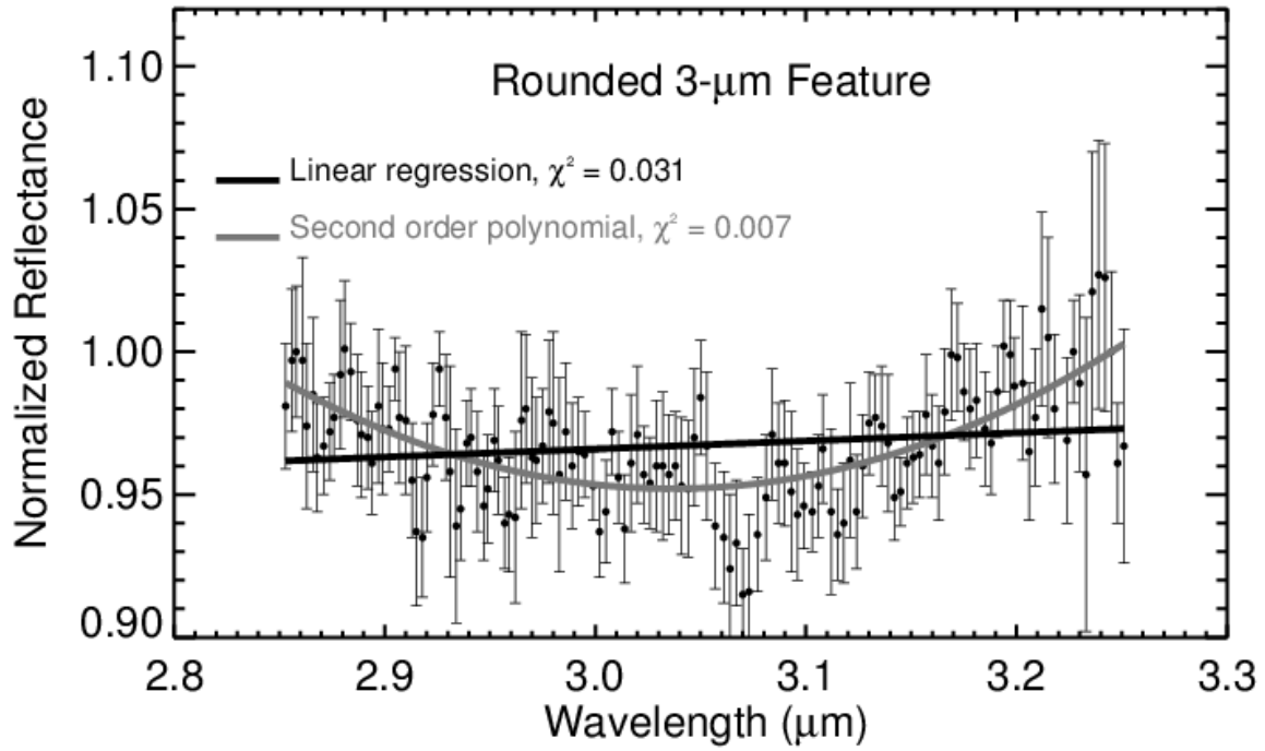
Figure A4. Determination of the best fit for the rounded 3- \mu m feature of 361 Bononia. The calculated chi-squared of the second order polynomial fit (in gray) across the 2.85-3.25- \mu m region has a lower value than one calculated for the linear regression fit (in black). Hence, the former fit is better than the latter. In this chi-squared test, the predicted data are the spectrum data and the observed data are the trendline data. The same technique was used for the sharp 3- \mu m feature.
