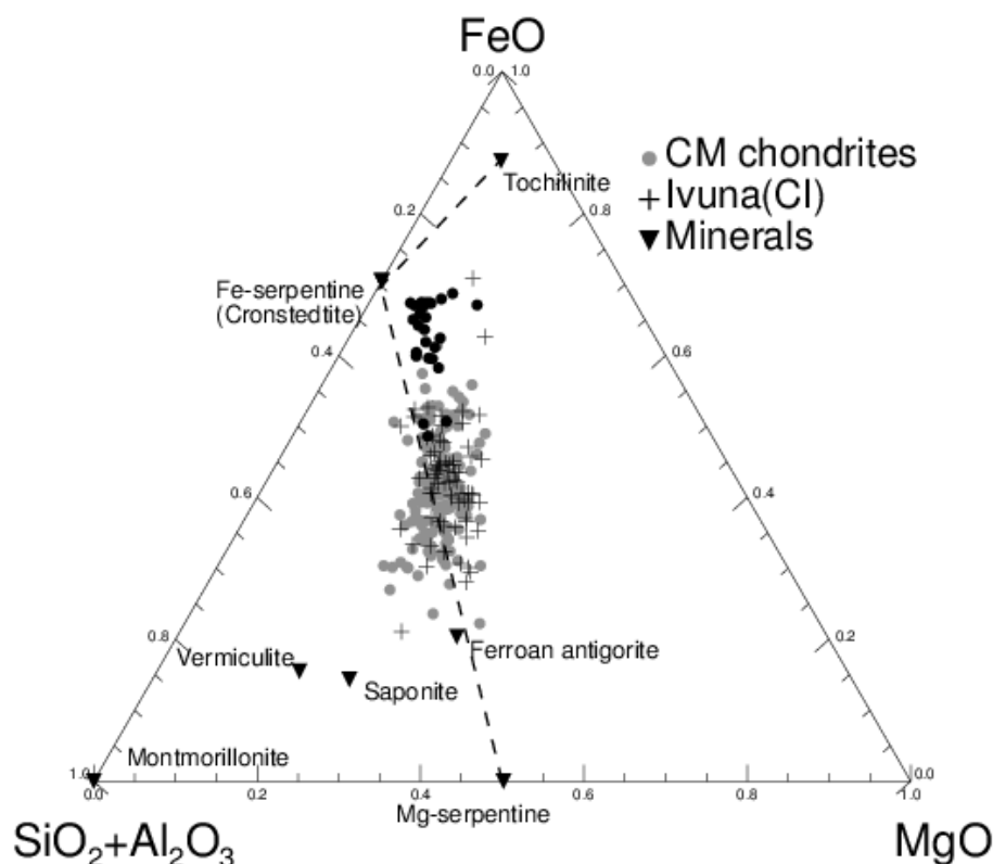
Figure B7. \text{SiO}_2+\text{Al}_2\text{O}_3 -FeO-MgO diagram showing matrix compositions of CM chondrites and Ivuna, as well as some alteration minerals: serpentinite - \text{Mg}_3\text{Si}_2\text{O}_5(\text{OH})_4 , montmorillonite - (\text{Na},\text{Ca})_{0.3}(\text{Al},\text{Mg})_2\text{Si}_4\text{O}_{10}(\text{OH})_2 \cdot n(\text{H}_2\text{O}) , vermiculite - (\text{Mg},\text{Fe}^{2+},\text{Al})_3(\text{Al},\text{Si})_4\text{O}_{10}(\text{OH})_2 \cdot 4(\text{H}_2\text{O}) , saponite - (\text{Ca}/2,\text{Na})_{0.3}(\text{Mg},\text{Fe}^{2+})_3(\text{Si},\text{Al})_4\text{O}_{10}(\text{OH})_2 \cdot 4(\text{H}_2\text{O}) , ferroan antigorite - (\text{Mg},\text{Fe}^{2+})_3\text{Si}_2\text{O}_5(\text{OH})_4 , and cronstedtite - \text{Fe}^{2+}_2\text{Fe}^{3+}(\text{SiFe}^{3+})\text{O}_5(\text{OH})_4 . Tochilinite data from Tomeoka and Buseck (1985). The matrix compositions lie along an approximately linear trend that extends from near the composition of cronstedtite (representing the least altered material) towards the \text{SiO}_2 -MgO join near the composition of Mg-serpentine (representing the most altered material). The black filled circles represent QUE 97990 (the least altered sample in the present study). See Appendix B2 for more diagrams of matrix compositions of CM chondrites and Ivuna.
