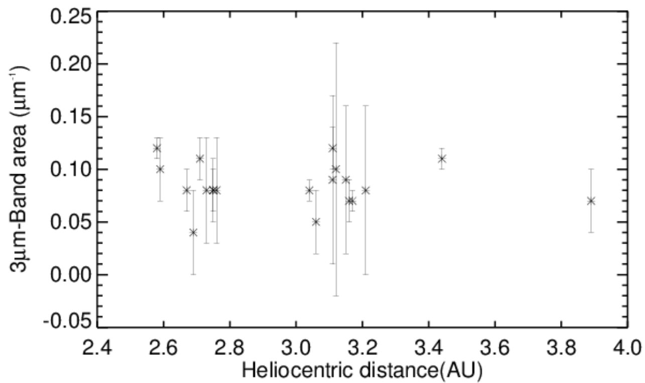
Figure C7. No correlation found between the helioncentric distance and the band area in asteroids that show the sharp OH 3-μm features.
