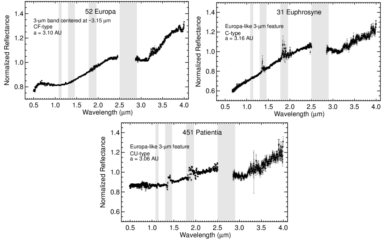
Figure A10. The Europa-like group with a 3- \mu\text{m} feature centered at 3.15 \pm 0.01 \mu\text{m} . All spectra have been normalized to unity at 2.2 \mu\text{m} . The gray bars on each plot mark wavelengths of strong absorption by water vapor in Earth's atmosphere.
