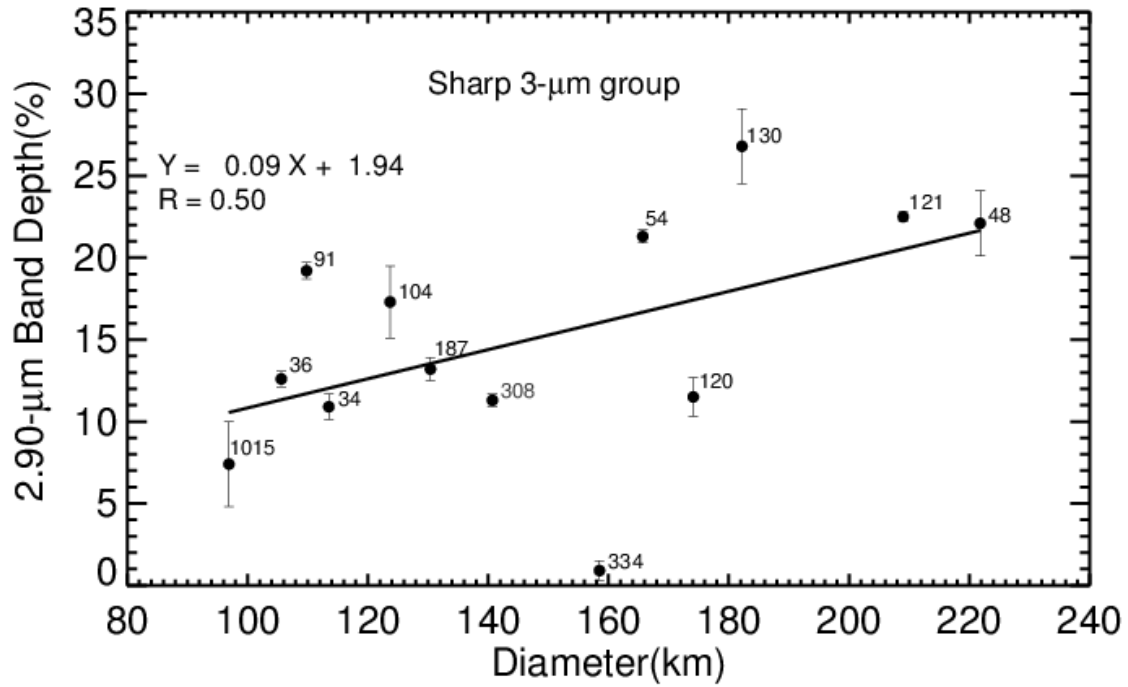
Figure A15. Diameter vs. the band depth at 2.90 \mu m for asteroids ( D < 300 km) exhibit the sharp OH 3- \mu m feature. The reflectance was calculated by fitting a linear regression line across the 2.85-3.25- \mu m region. 2.90- \mu m band depth increases with the increase of the diameter. The R (linear-correlation coefficient) value of 0.50 corresponds to a probability of \sim 0.95 ( 2\sigma ) that the variables are correlated.
