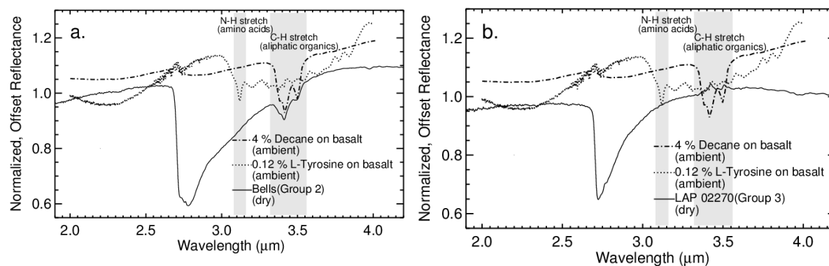
Figure B9a. Spectra of Bells (Group 2), and of decane alkane (4%) and L-Tyrosine amino acid (0.12%) mixed with basalt (BHVO-2F). The 3.1-μm feature in Tyrosine spectrum is the N-H fundamental stretch of amino acids. If Tyrosine were in the meteorite sample with similar grain sizes, our detectability would be around 0.01 wt % (100 ppm). The absorptions at 3.4-3.5 μm are the C-H stretch of aliphatic organics. B9b. LAP 02770 (Group 3) does not show the N-H stretch feature nor the C-H stretch feature.
