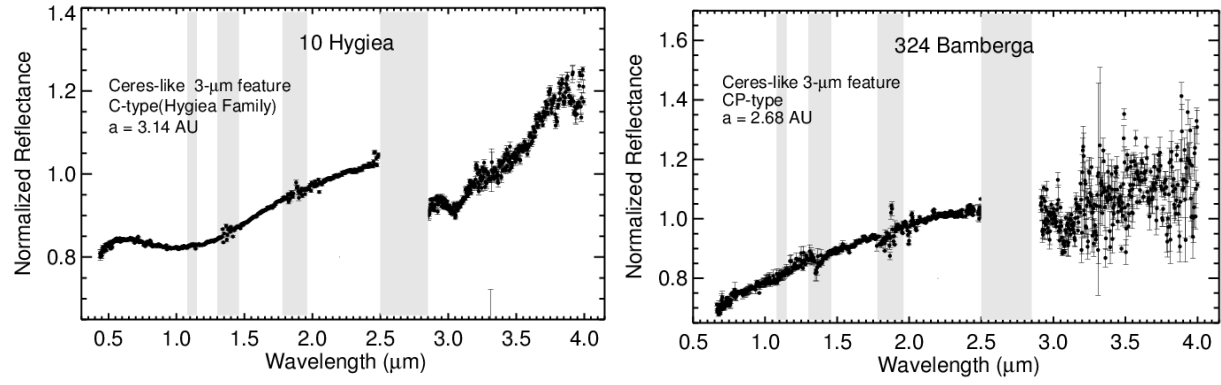
Figure A9. The Ceres-like group with a 3-μm feature centered at 3.05 \pm 0.01 μm. All spectra have been normalized to unity at 2.2 μm. The gray bars on each plot mark wavelengths of strong absorption by water vapor in Earth's atmosphere.
