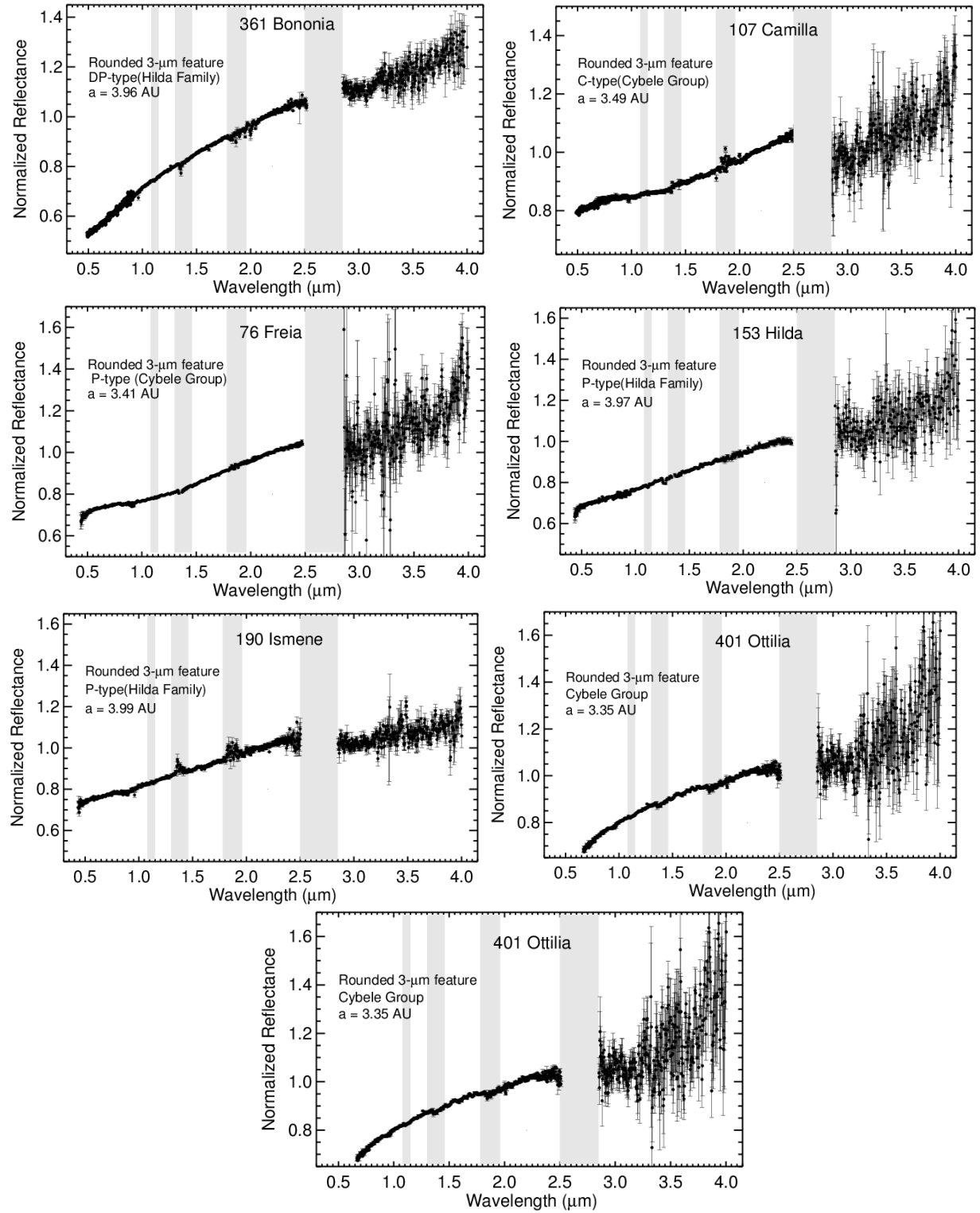
Figure A11. The rounded 3- \mu m feature. All spectra have been normalized to unity at 2.2 \mu m. The gray bars on each plot mark wavelengths of strong absorption by water vapor in Earth's atmosphere.
