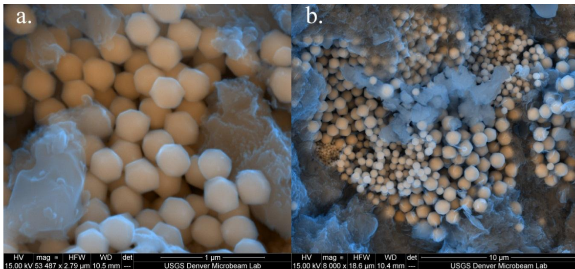
Figure B10a. Magnetite grains have been identified in Bells (Group 2) as framboidal aggregates with polygonal morphology. B10b. Similar framboidal aggregates of magnetite grains have also been found in Ivuna (CI).
