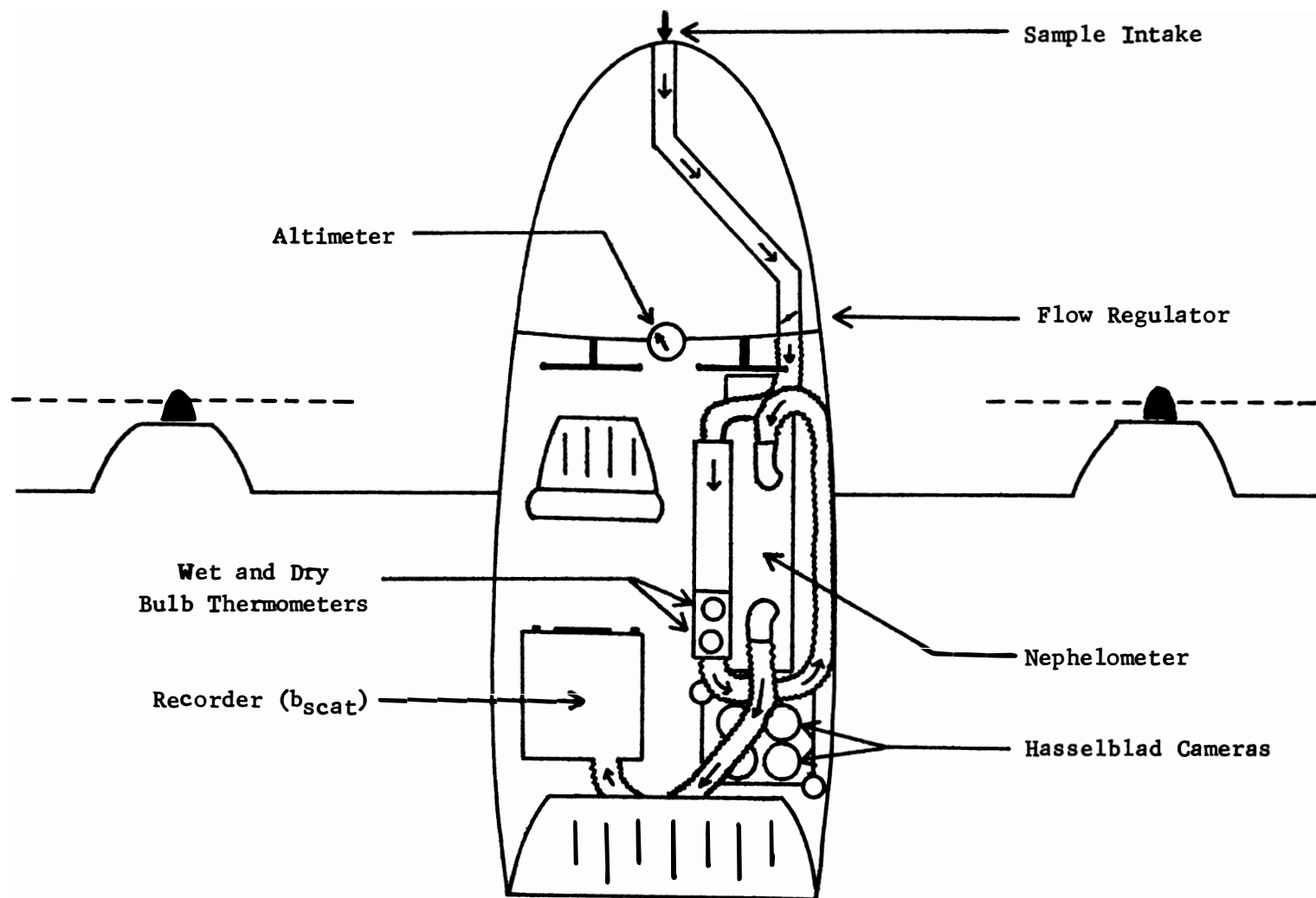
FIGURE IV-1. View of Airplane and the Experimental Apparatus.
