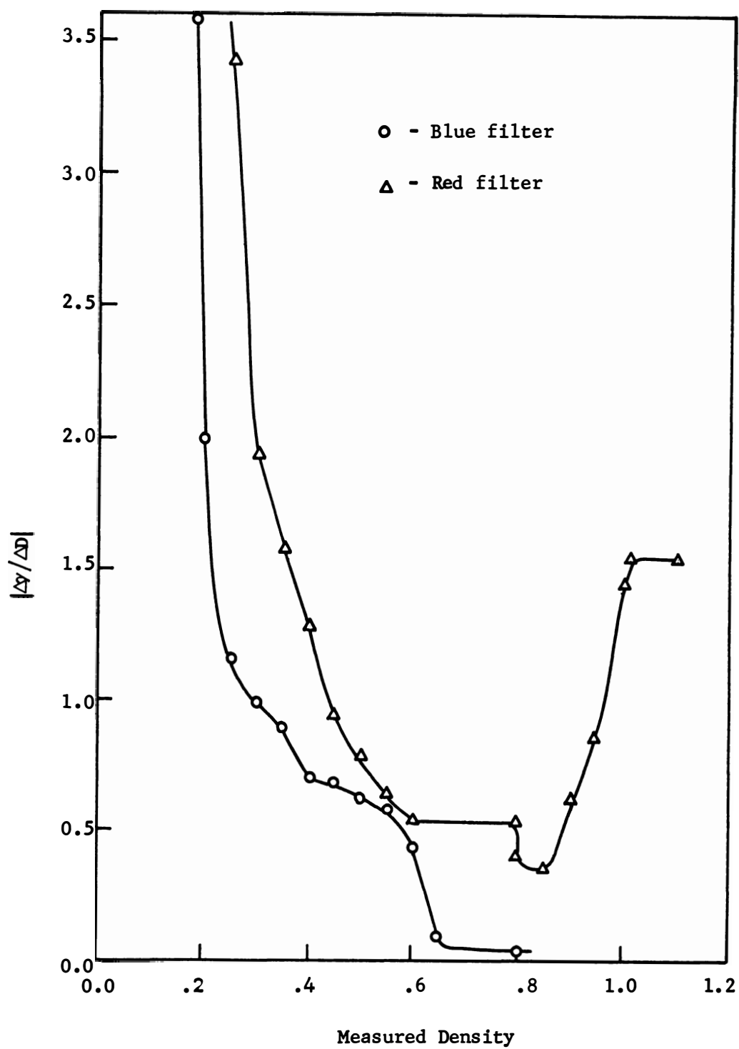
Figure V-15. Graph of |\Delta\gamma/\Delta D| versus Measured Density for November 6, 1972 Flight.
