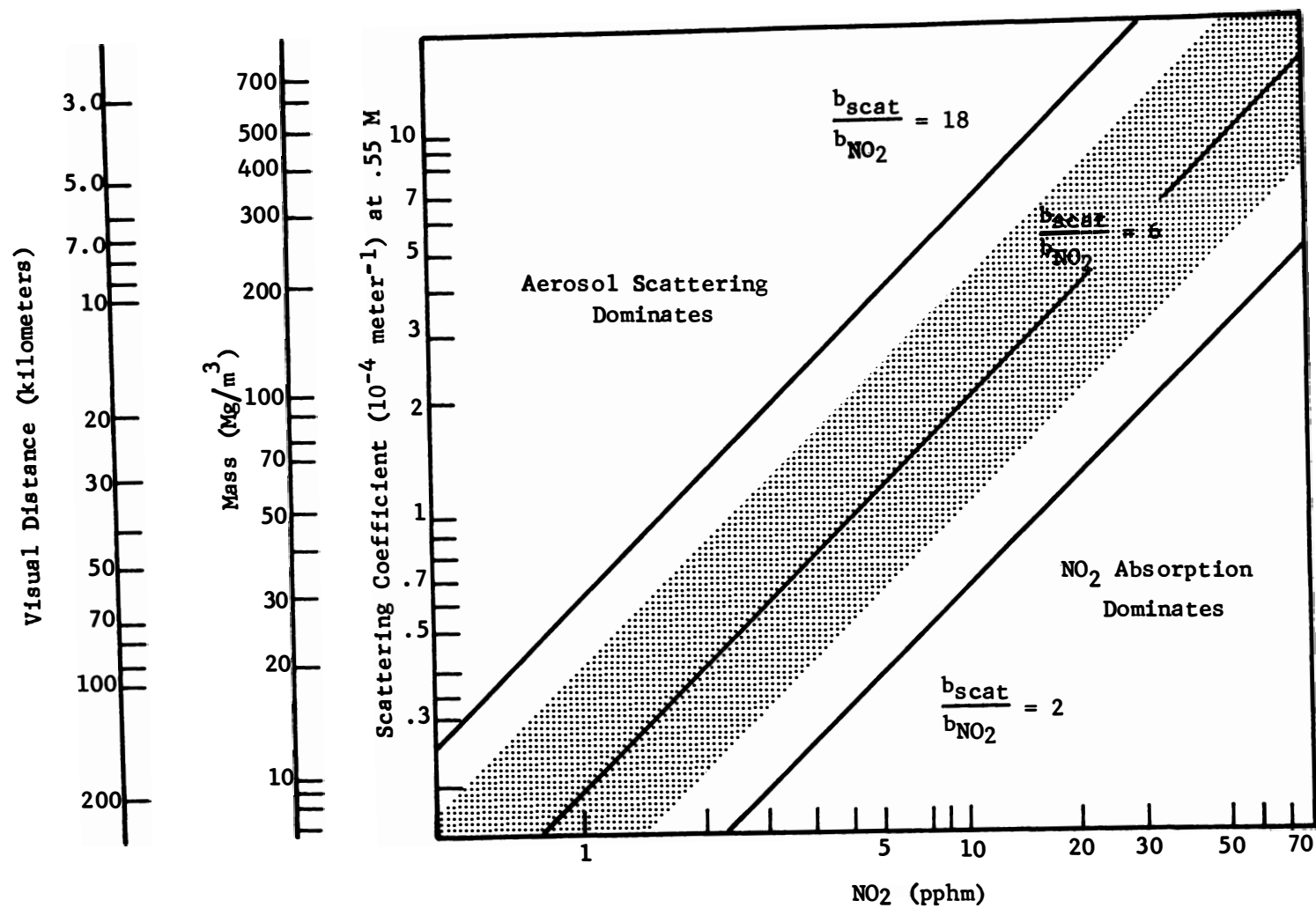
FIGURE II-1. Graph of b_{scat} Versus b_{NO_2} .
