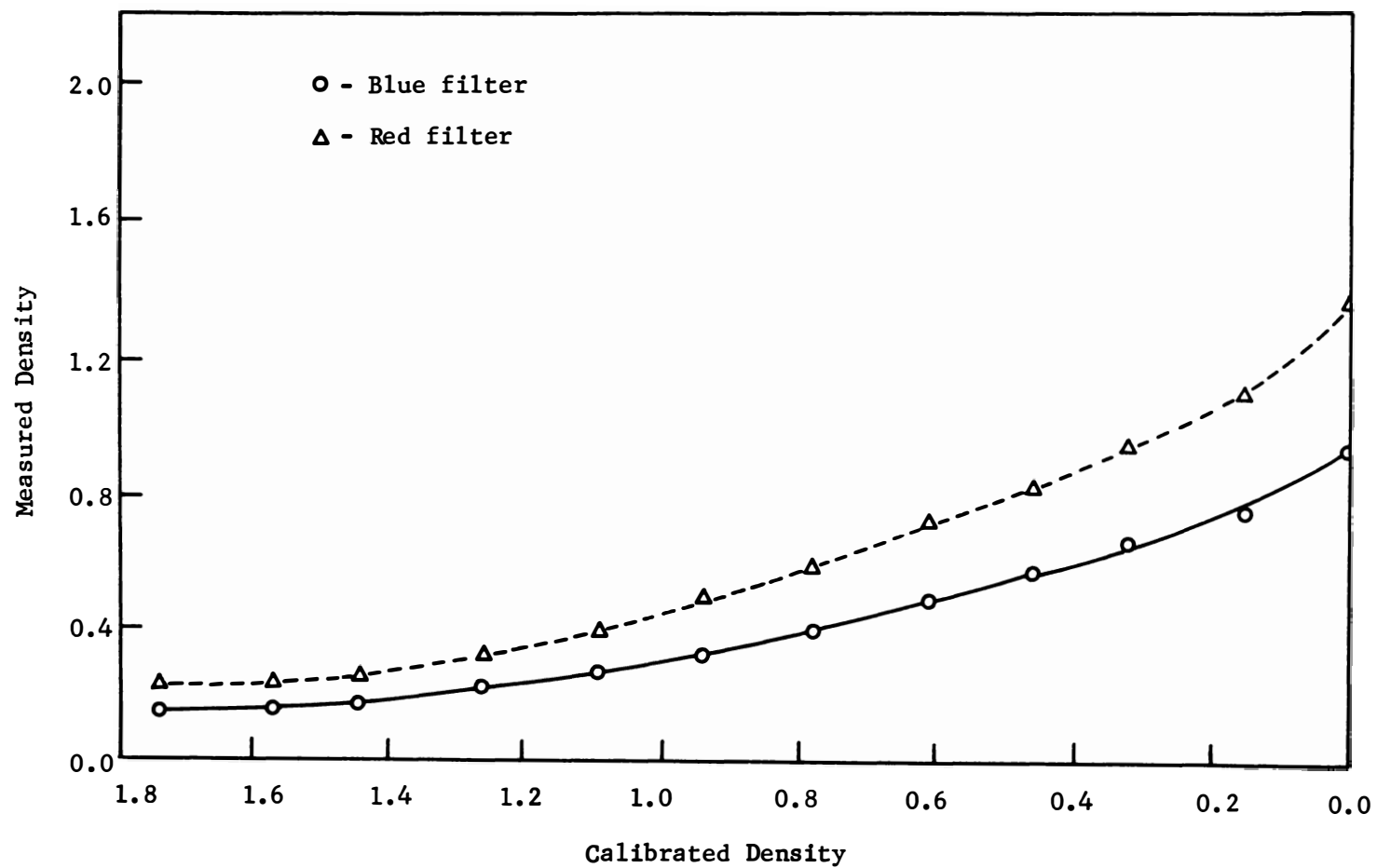
Figure V-8. The \gamma -Curves for the November 6, 1972 Flight.
