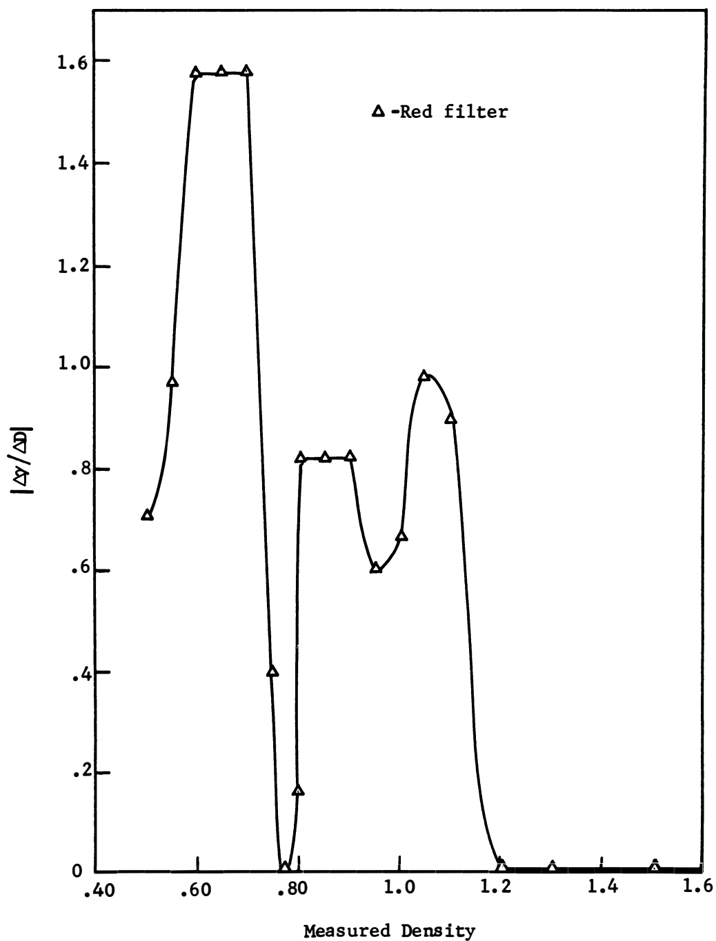
Figure V-14. Graph of |\Delta y / \Delta D| versus Measured Density for July 12, 1972 Flight.
