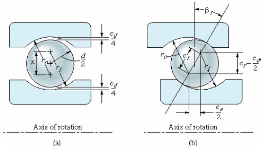
Figure 42. Contact Angles.
