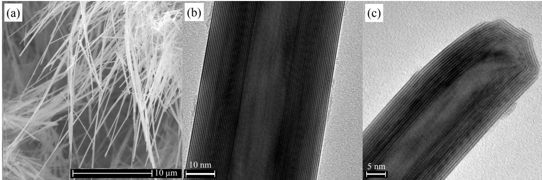
Figure 1: Ambient condition (a) scanning and (b,c) high resolution transmission electron microscopy images of the \text{WS}_2 nanotubes used in this work.
