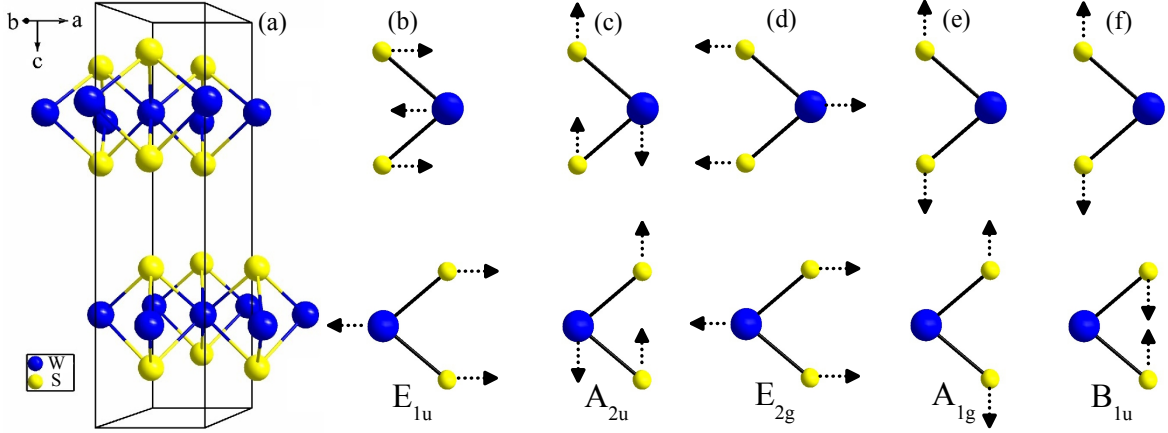
Figure 3: (a) The unit cell of \text{WS}_2 consists of two layers; in each layer W is covalently bonded to six S atoms in trigonal prismatic coordination, 49 which form the walls of the tubes. These layers comprise the ab -plane, and are stacked along the c axis. Displacement patterns for the (b,c) infrared- and (d-f) Raman-active phonons. 41,42 While these mode patterns and symmetries formally apply only to the single crystal, they are regularly extended to describe nanoscale analogs.
