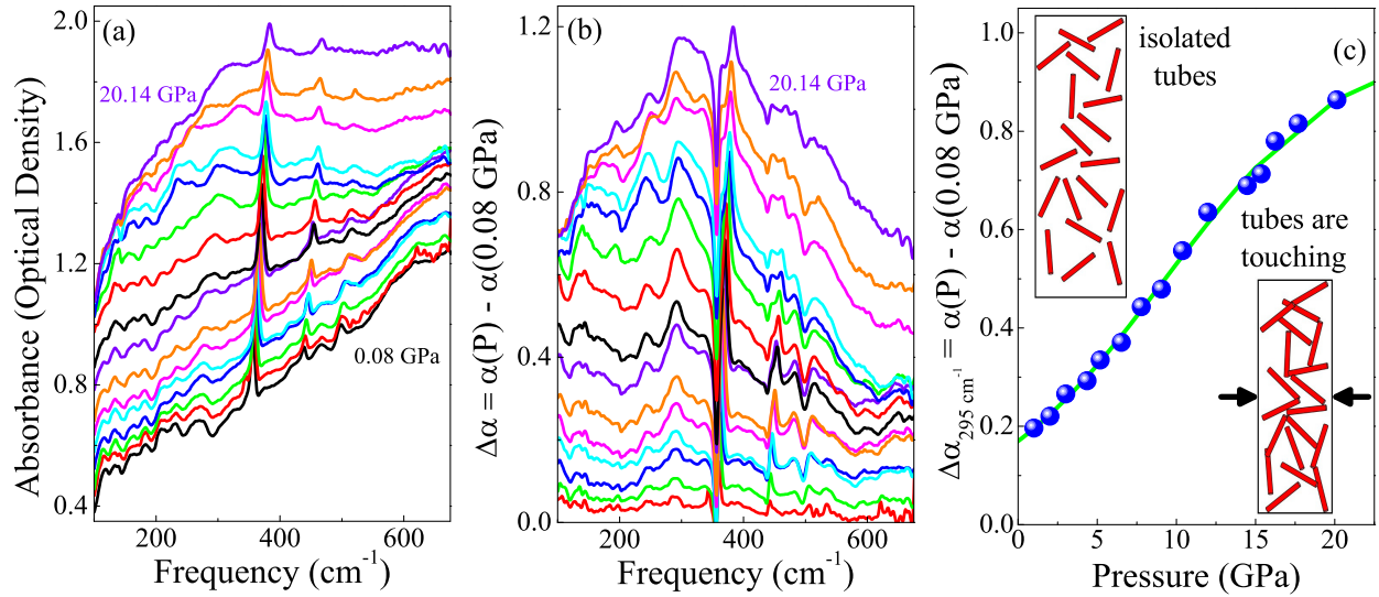
Figure 5: (a) Infrared spectra at increasing pressures. (b) Absorption difference, \Delta\alpha = \alpha(P) - \alpha(0.08 \text{ GPa}) , showing the increasing background due to improved conductivity under pressure caused by percolation effects. (c) Absorption difference at 295 cm -1 versus pressure. The green line is a fit to the percolation model described in the text. Insets: schematic views of the diamond anvil cell at low and high pressure showing the conductive pathway that forms as the tubes begin to touch.
