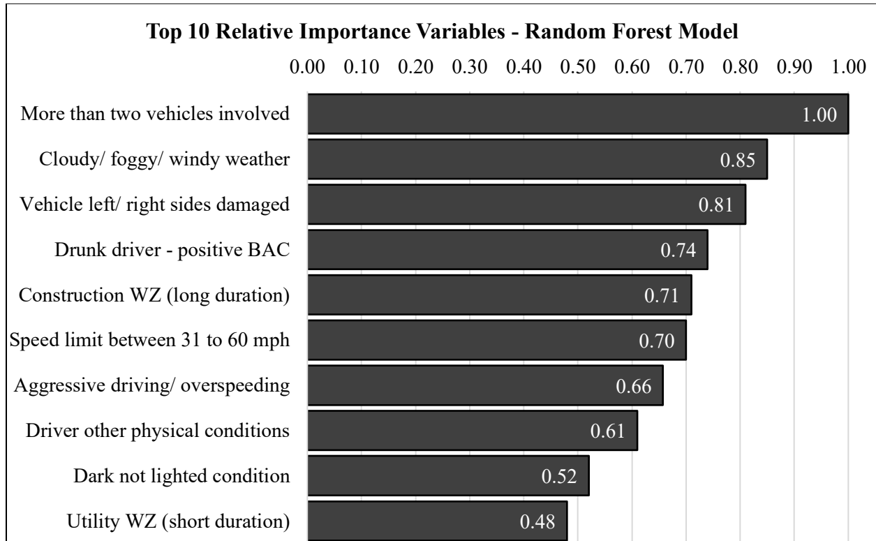
3 Figure 3 Top 10 Relative Importance Variables – Original Data Random Forest Model
