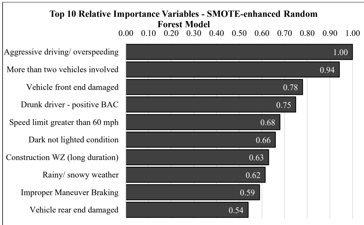
5 Figure 4 Top 10 Relative Importance Variables – SMOTE-enhanced Random Forest Model
