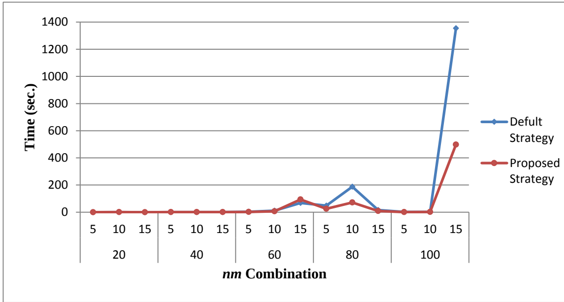
Figure 28: The Effect of the MATLAB Default and the Proposed Branching Strategies on the Average CPU Time in Model 2
