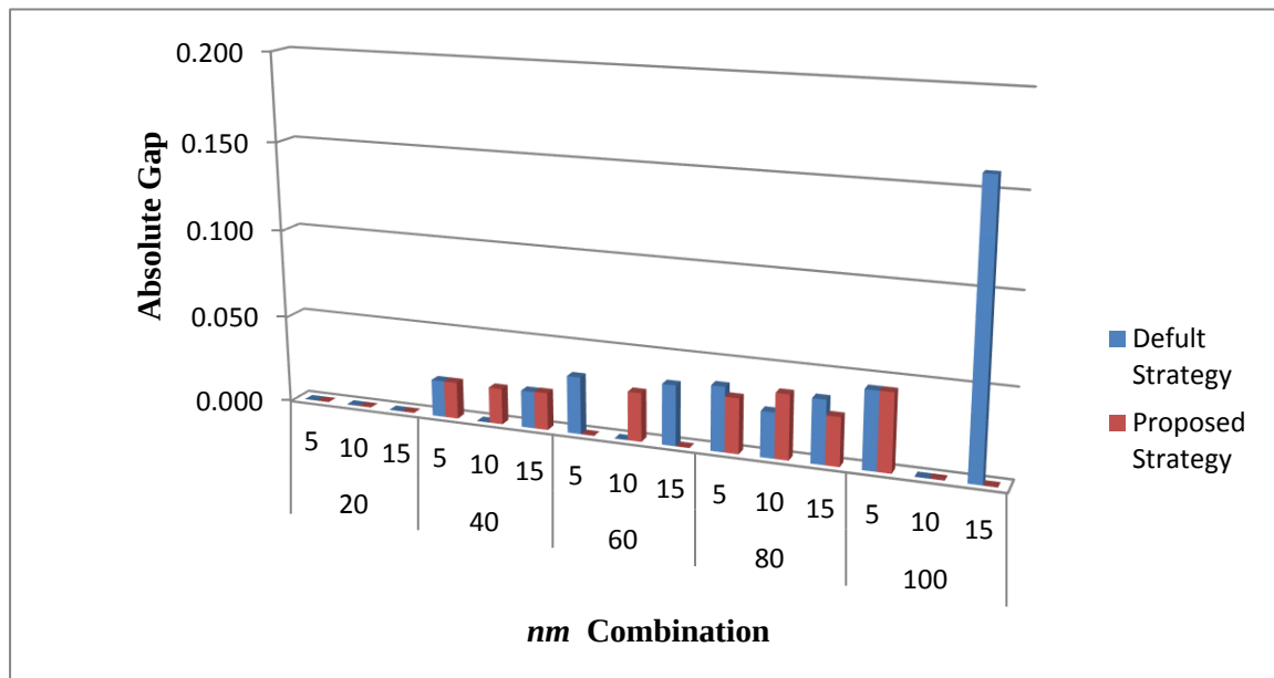
Figure 29: The Effect of the MATLAB Default and the Proposed Branching Strategies on the Absolute Gap in Model 2
