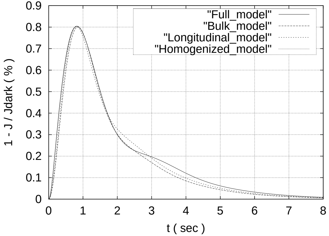
Figure 5.10: Histories of the normalized response from all models. The activation parameter \nu_{\text{RE}} = 355 \text{ s}^{-1} in the bulk model, 412.5 \text{ s}^{-1} in the longitudinal model and 675 \text{ s}^{-1} in the full model and the homogenized model.
