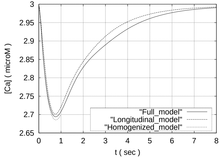
Figure 5.12: Histories of \text{Ca}^{2+} concentration (at activated disc) from all models. The activation parameter \nu_{\text{RE}} = 355 \text{ s}^{-1} in the bulk model, 412.5 \text{ s}^{-1} in the longitudinal model and 675 \text{ s}^{-1} in the full model and the homogenized model.
