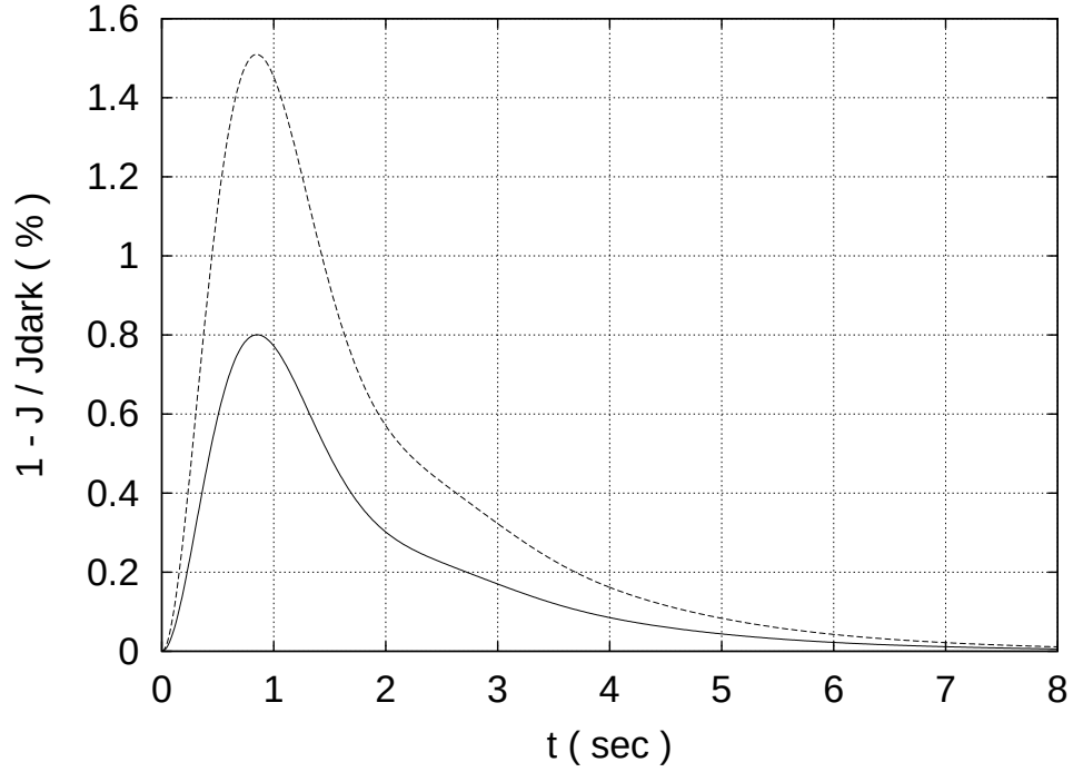
Figure 5.6: Bulk model simulation: normalized response versus time; upper curve with \nu_{\text{RE}} = 675 \text{ s}^{-1} and lower curve with \nu_{\text{RE}} = 355 \text{ s}^{-1} .
