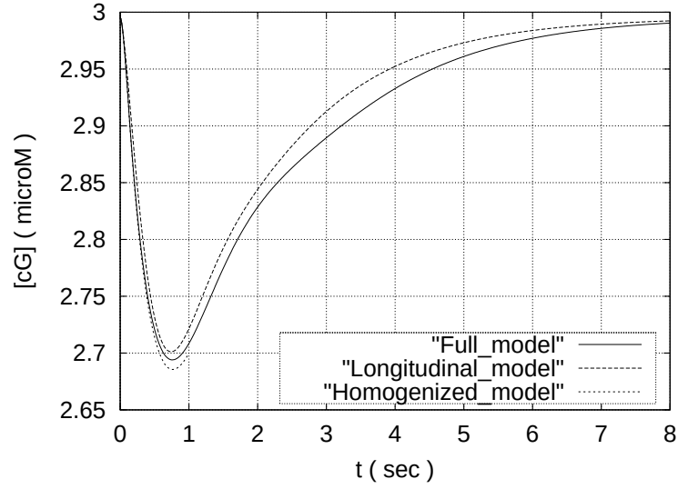
Figure 5.11: Histories of cGMP concentration (at activated disc) from all models. The activation parameter \nu_{\text{RE}} = 355 \text{ s}^{-1} in the bulk model, 412.5 \text{ s}^{-1} in the longitudinal model and 675 \text{ s}^{-1} in the full model and the homogenized model.
