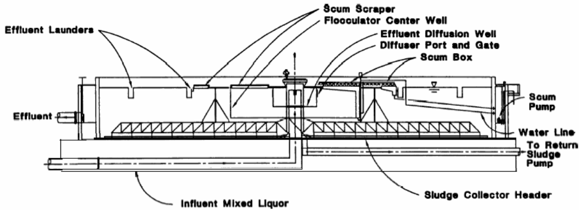
Figure 1: Cross sectional view of flocculator clarifier
