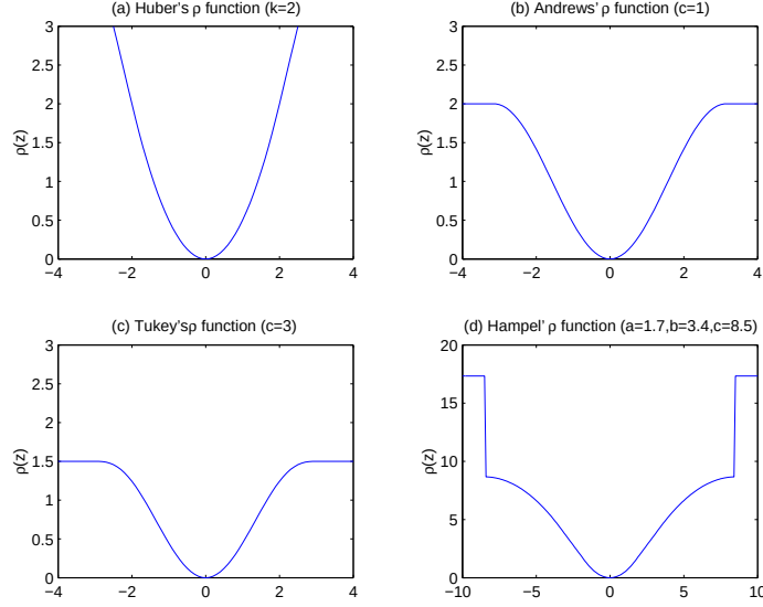
Figure 2.1: Example \rho Functions of M-estimation: (a) Huber's \rho function with k=2 ; (b) Andrews' \rho function with c=1 ; (c) Tukey's \rho function with c=3 ; (d) Hampel's \rho function with a=1.7 , b=3.4 , c=8.5 .
