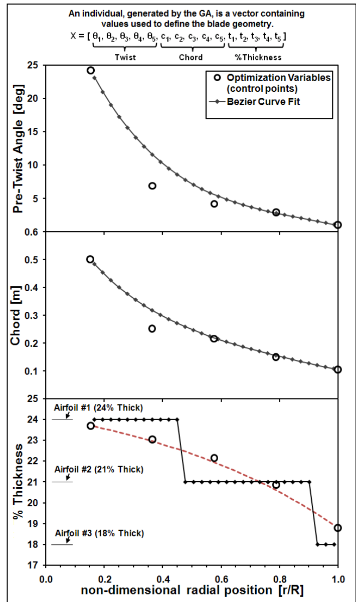
Figure 3 - The blade geometry distributions are each defined by a Bezier curve fit through the control points.
