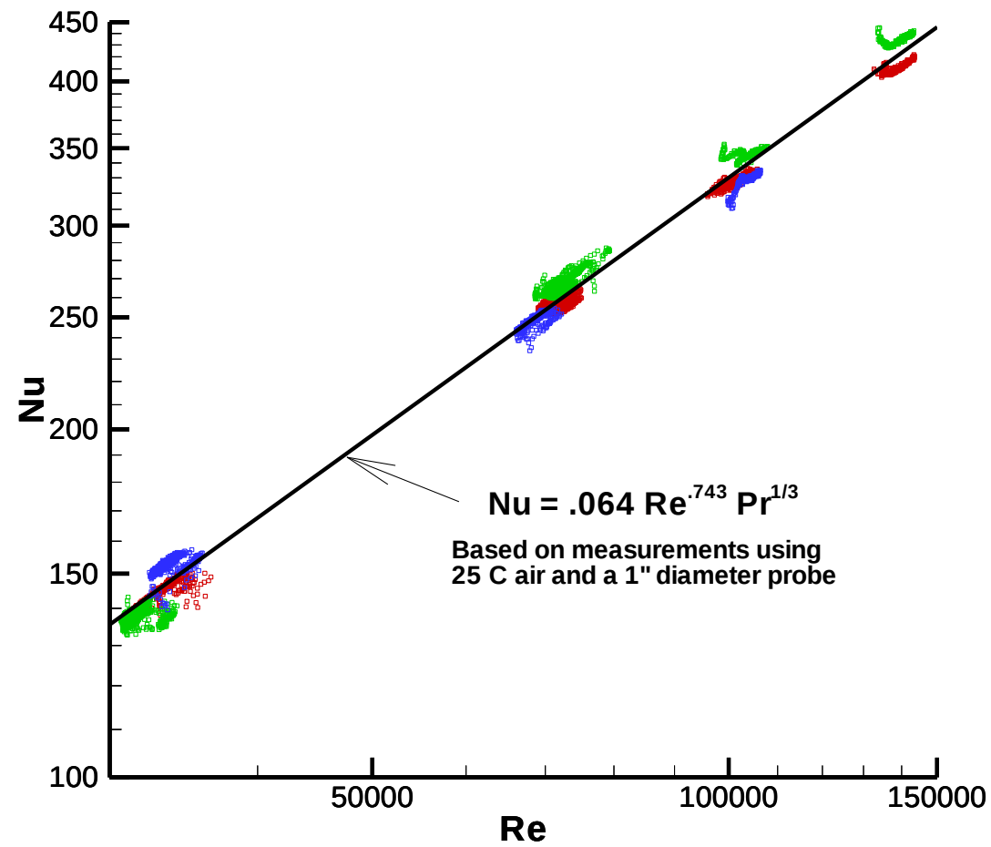
Figure 14: Nussult Number Relationship for the High Temperature Simulated Temperature Probe.
