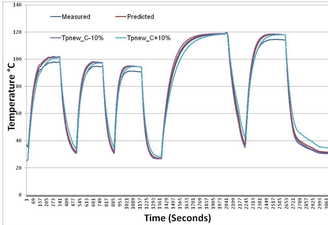
Figure 22: Temperature Model Results for dT/dt Coefficient \pm 10\% vs. Predicted and Measured Temperature.
